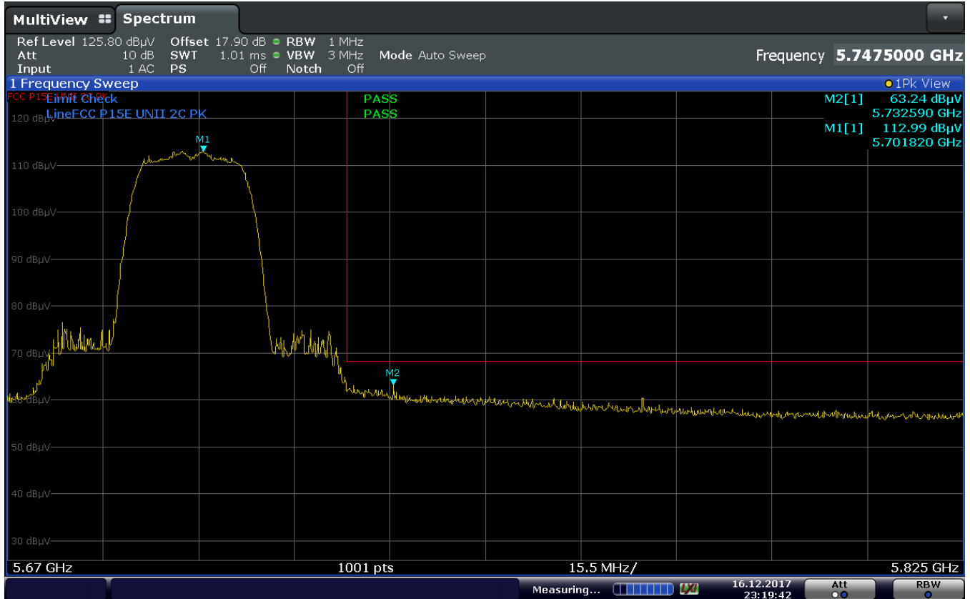
Plot 7-333. Radiated Restricted Upper Band Edge Measurement SISO ANT2 (Average & Peak UNII Band 2C)
