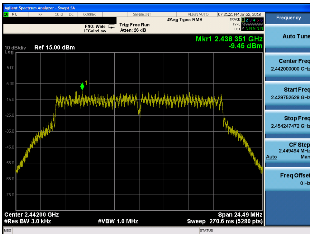
Plot 7-77. Power Spectral Density Plot MIMO ANT2 (802.11g – Ch. 7)
