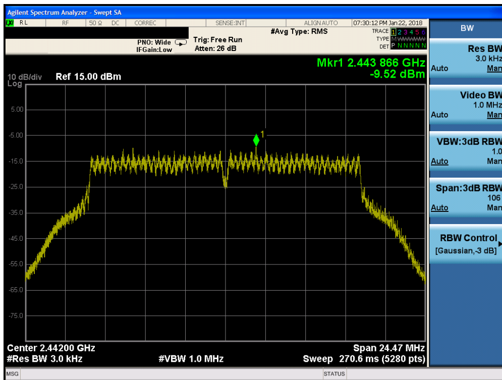
Plot 7-76. Power Spectral Density Plot MIMO ANT1 (802.11g – Ch. 7)
