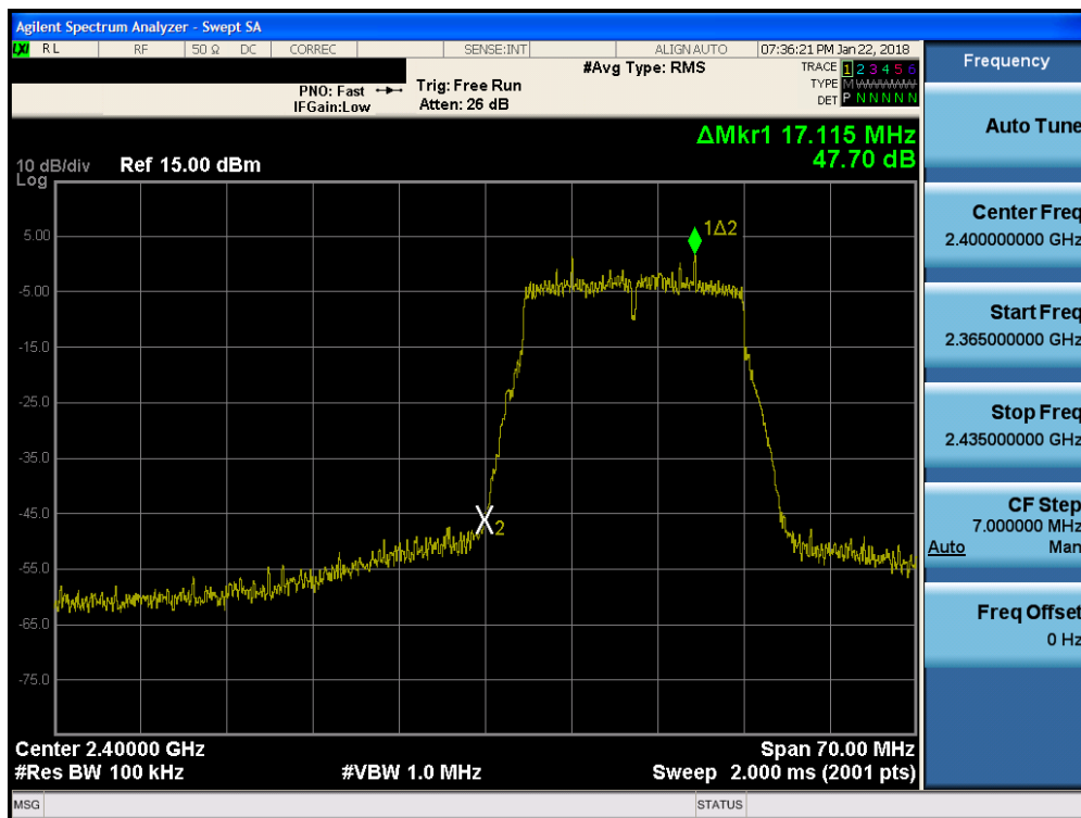
Plot 7-124. Band Edge Plot MIMO ANT1 (802.11n (2.4GHz) – Ch. 1)
