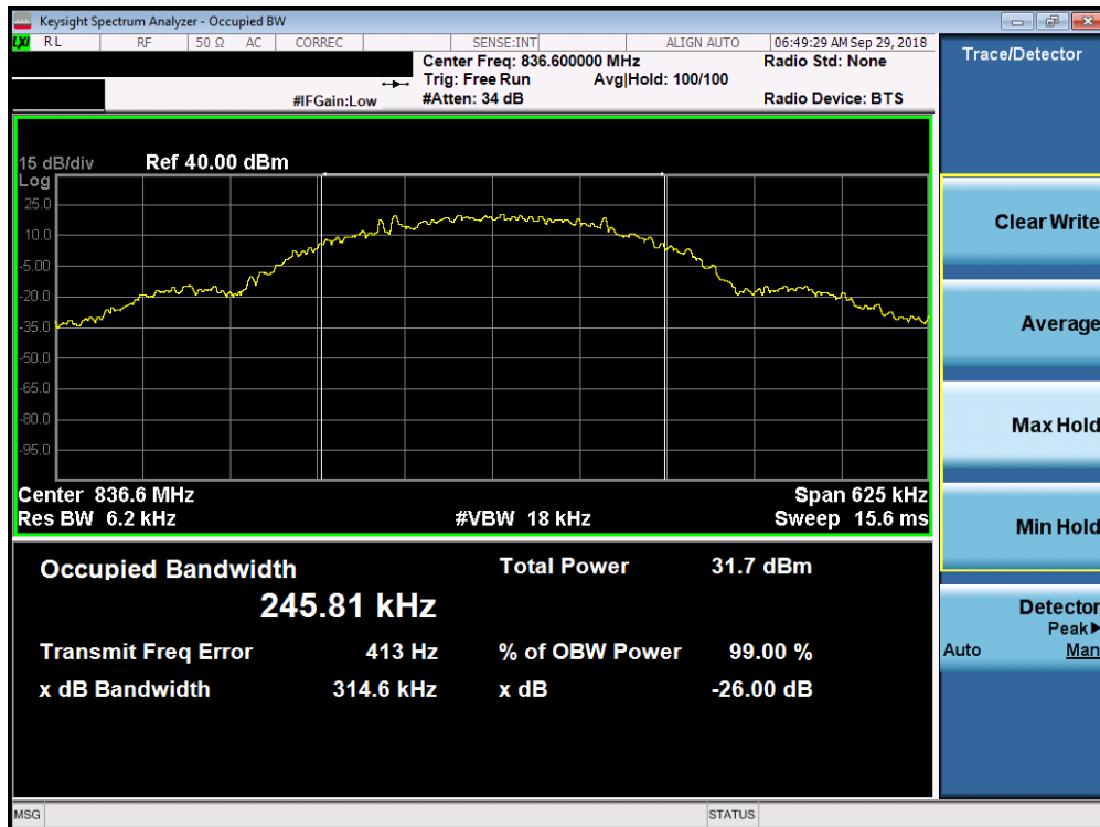
Plot 7-2. Occupied Bandwidth Plot (Cellular EDGE Mode)
