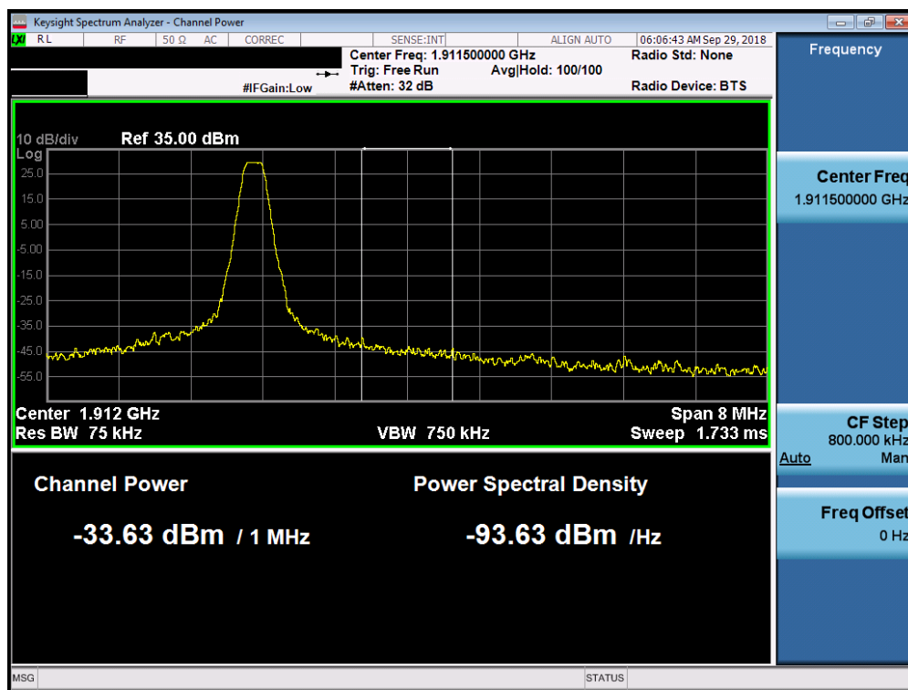
Plot 7-58. Extended Band Edge Plot (PCS GPRS Mode - High Channel)
