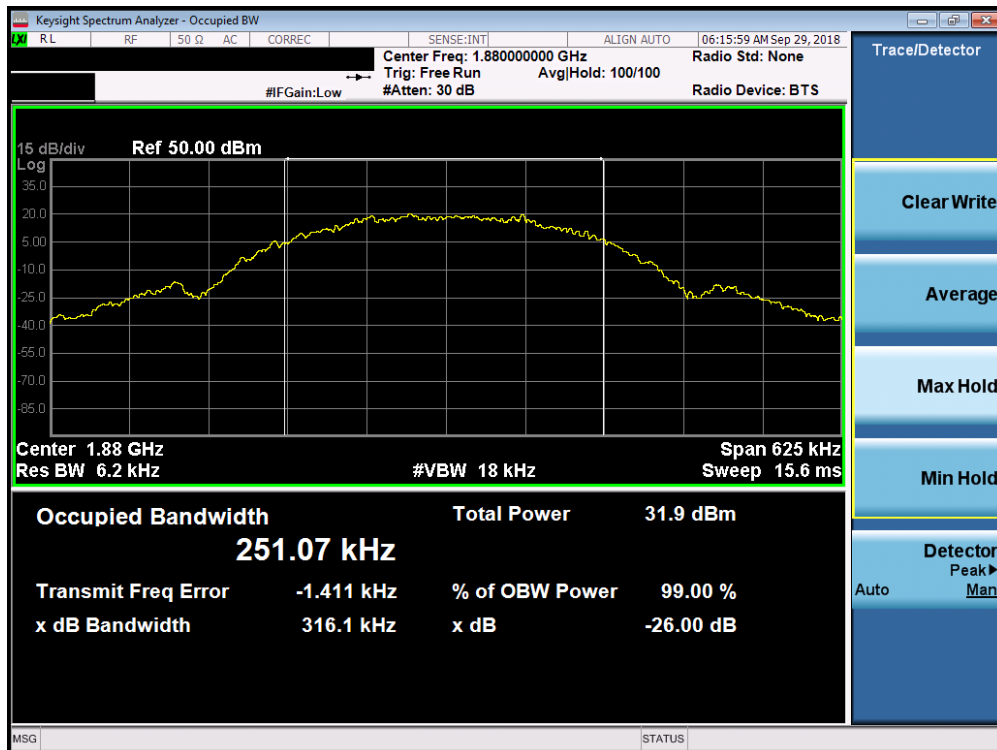
Plot 7-4. Occupied Bandwidth Plot (PCS EDGE Mode)
