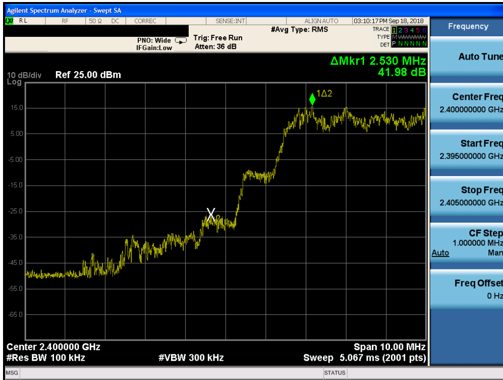
Plot 7-25. Band Edge Plot ANT0 (Bluetooth with Hopping Enabled, 8DPSK, ePA – Ch. 0)
