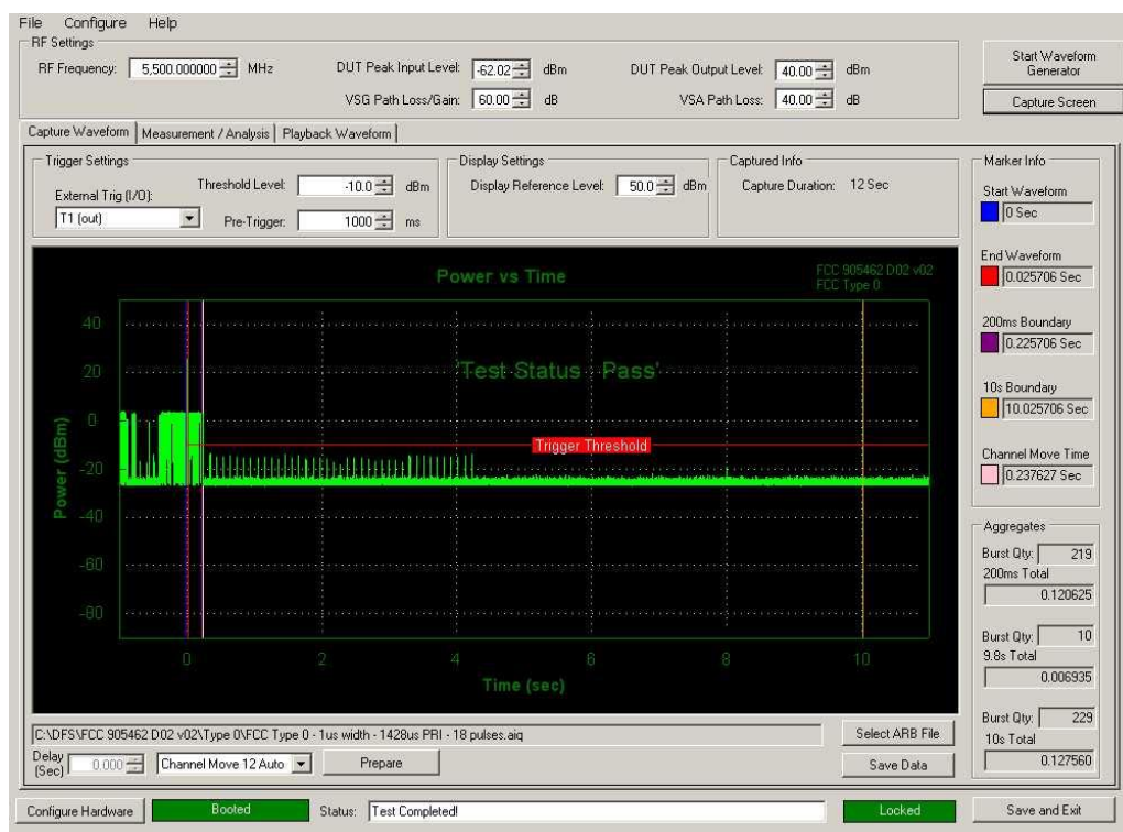
Figure 8-4. 5500MHz - Move Time and Aggregate Time (20 MHz)
