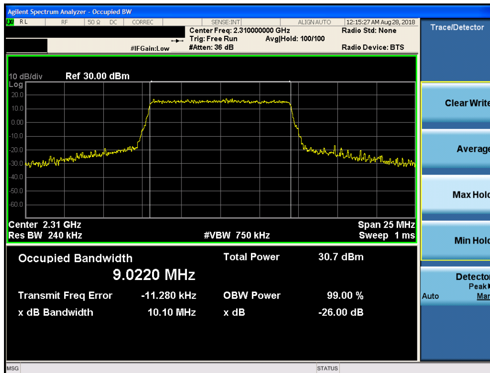
Plot 7-72. Occupied Bandwidth Plot (Band 30 – 10.0MHz 64-QAM – RB Size 50)
