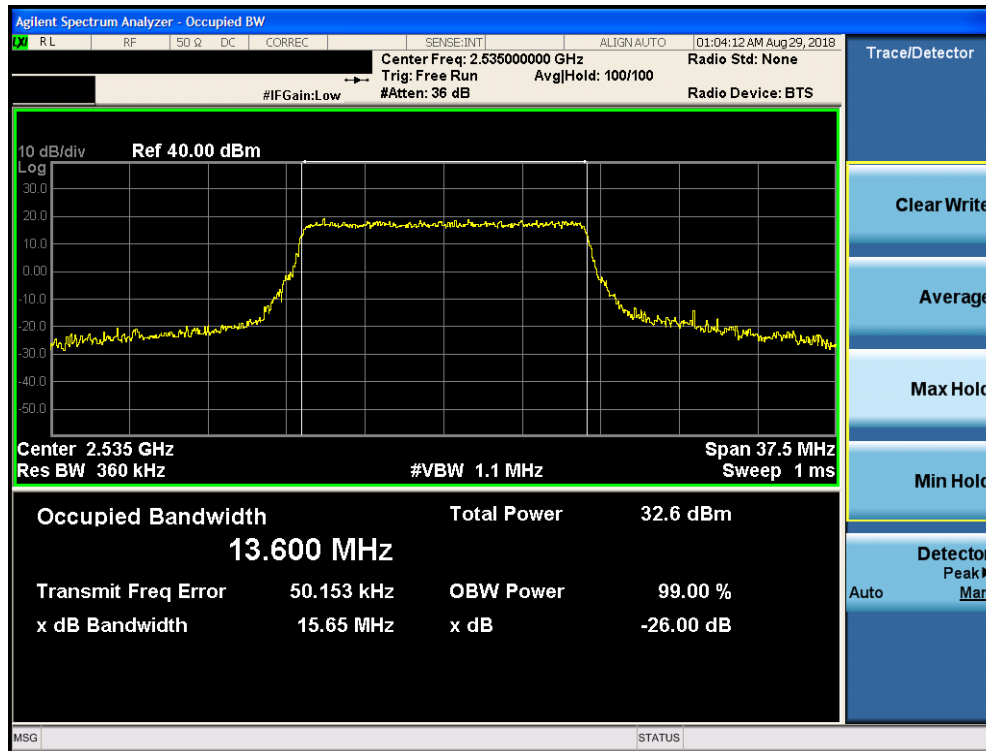
Plot 7-79. Occupied Bandwidth Plot (Band 7 – 15.0MHz QPSK – RB Size 75)
