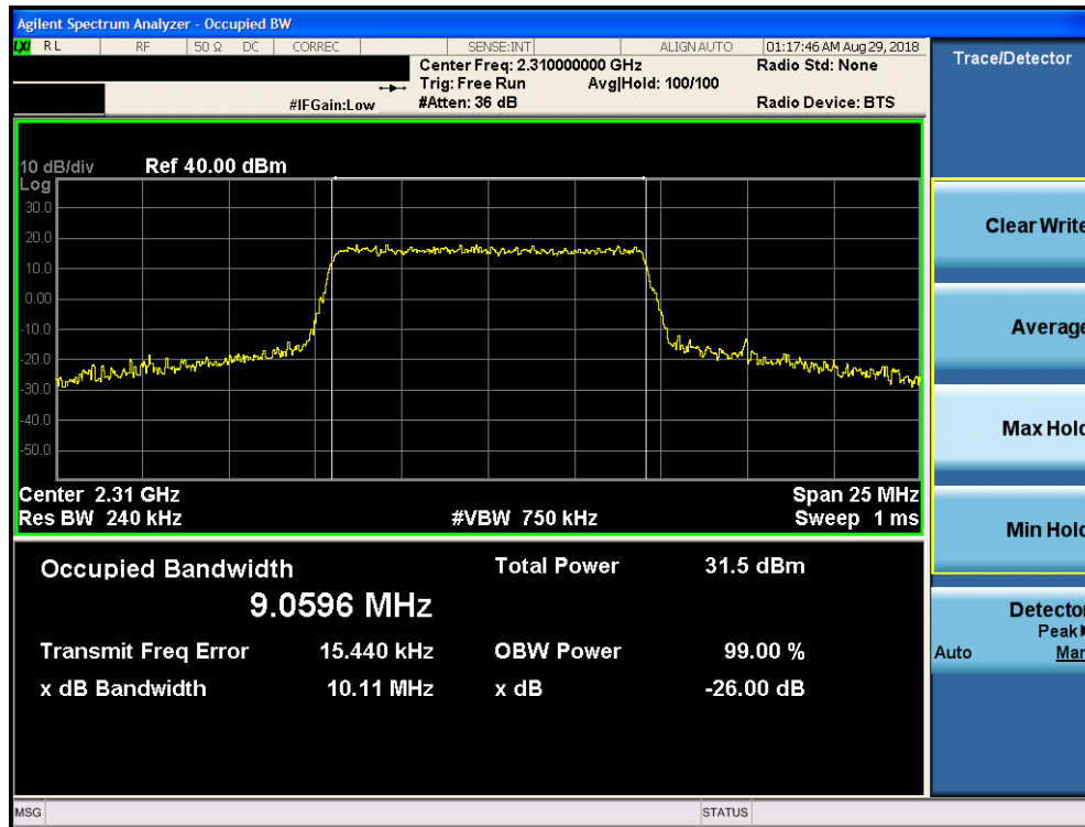
Plot 7-71. Occupied Bandwidth Plot (Band 30 – 10.0MHz 16-QAM – RB Size 50)
