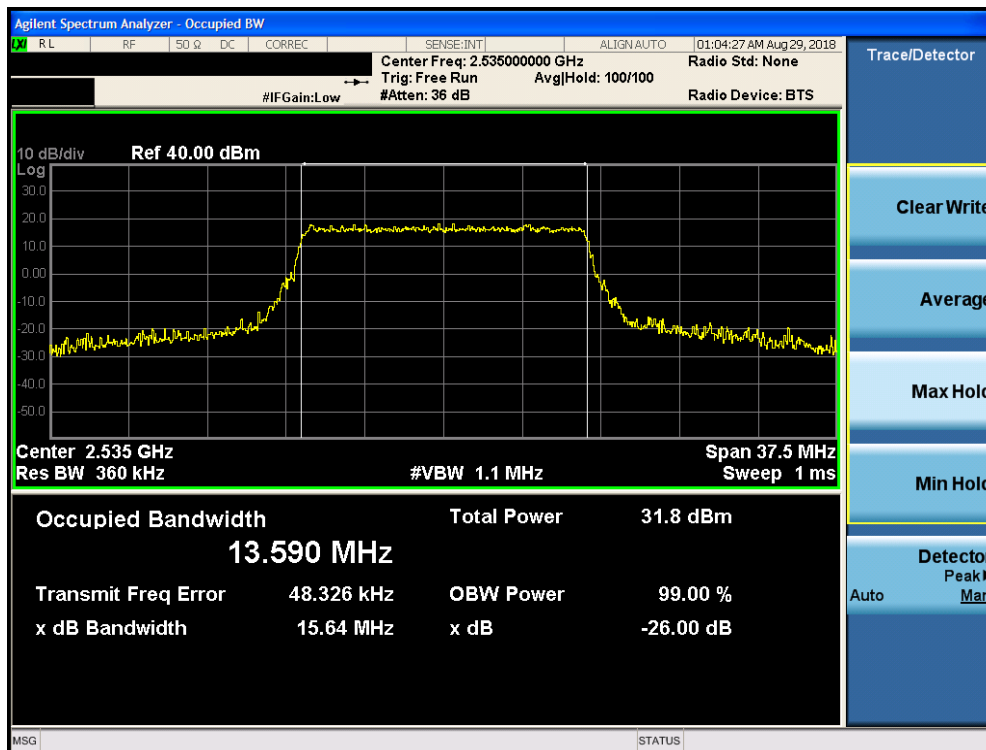
Plot 7-80. Occupied Bandwidth Plot (Band 7 – 15.0MHz 16-QAM – RB Size 75)
