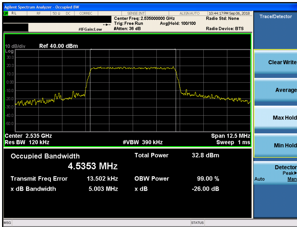
Plot 7-74. Occupied Bandwidth Plot (Band 7 – 5.0MHz 16-QAM – RB Size 25)
