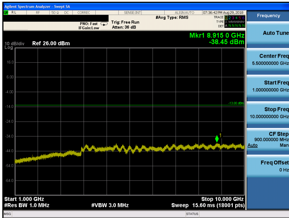
Plot 7-117. Conducted Spurious Plot (Band 26/5 – 10.0MHz QPSK – RB Size 1, RB Offset 0 – High Channel)
