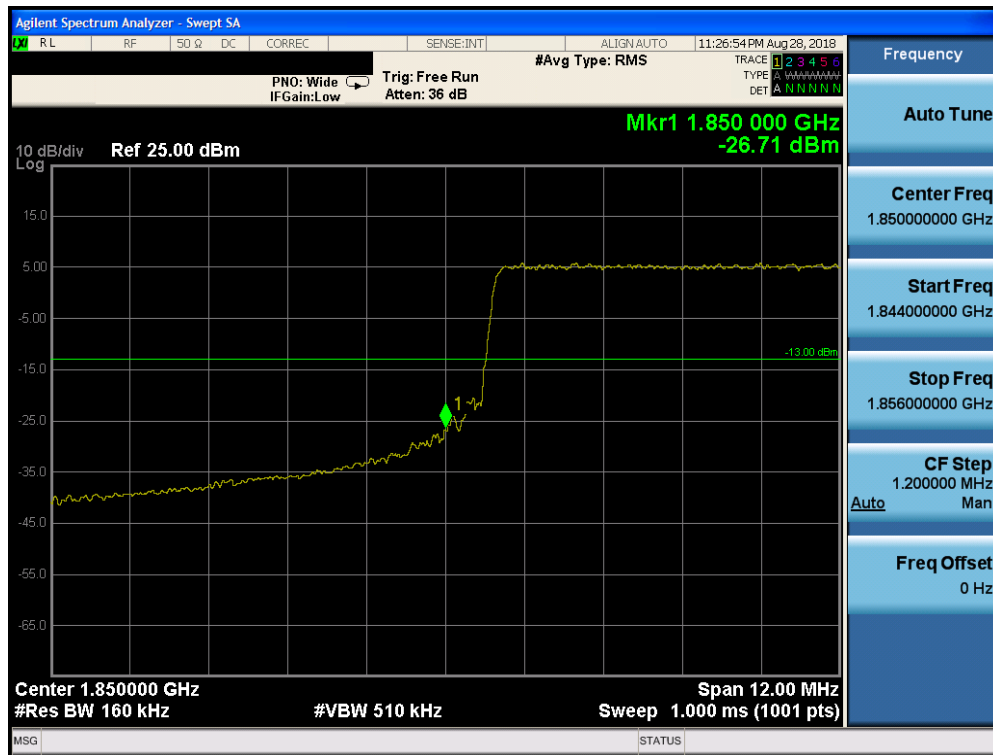
Plot 7-284. Lower Band Edge Plot (Band 25 – 15.0MHz QPSK – RB Size 75)
