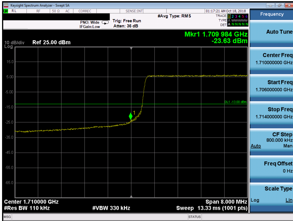
Plot 7-232. Lower Band Edge Plot (Band 66 – 10.0MHz QPSK – RB Size 50)
