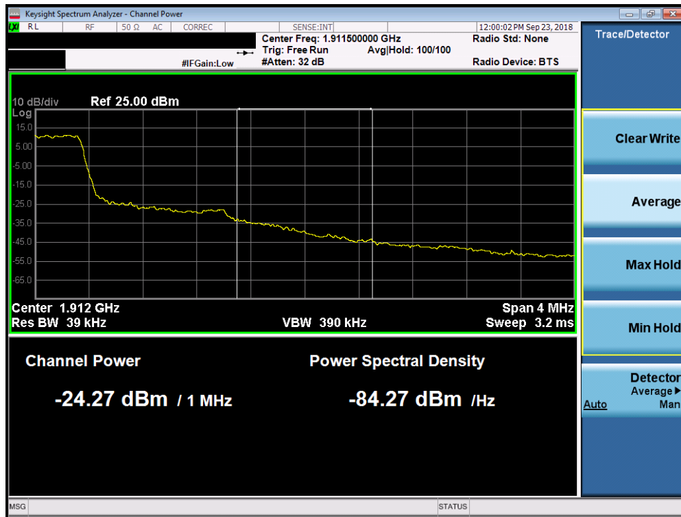
Plot 7-247. Upper Extended Band Edge Plot (Band 2 – 1.4MHz QPSK – RB Size 6)
