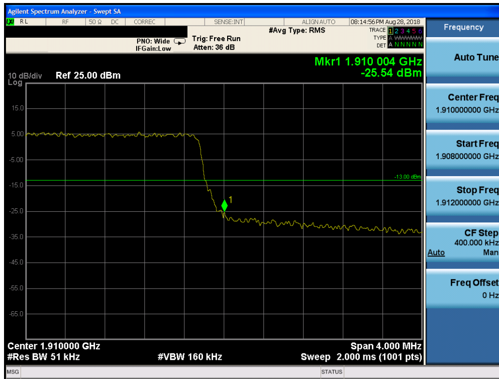
Plot 7-254. Upper Band Edge Plot (Band 2 – 5.0MHz QPSK – RB Size 25)
