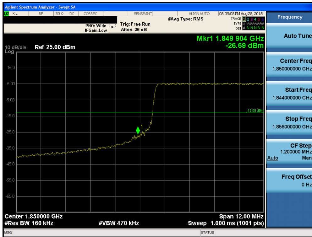
Plot 7-260. Lower Band Edge Plot (Band 2 – 15.0MHz QPSK – RB Size 75)
