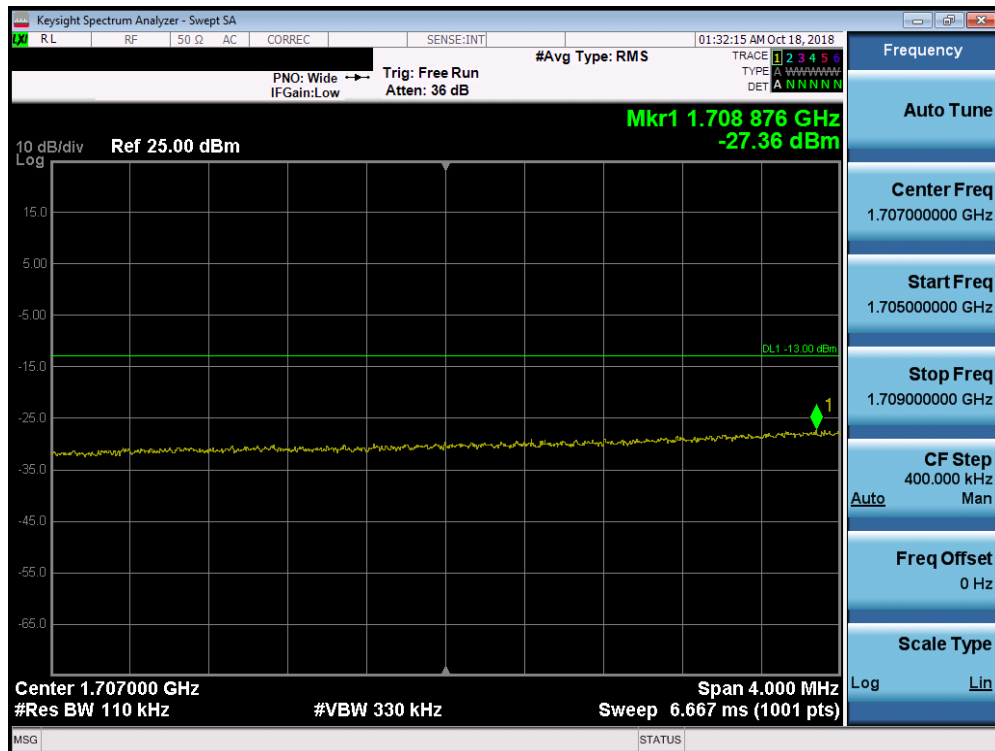
Plot 7-233. Lower Extended Band Edge Plot (Band 66 – 10.0MHz QPSK – RB Size 50)
