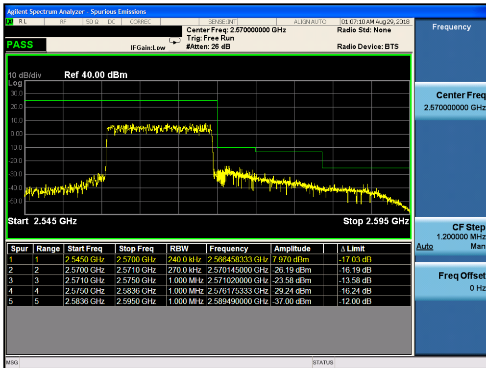
Plot 7-305. Upper ACP Plot (Band 7 – 15.0MHz QPSK – RB Size 75)
