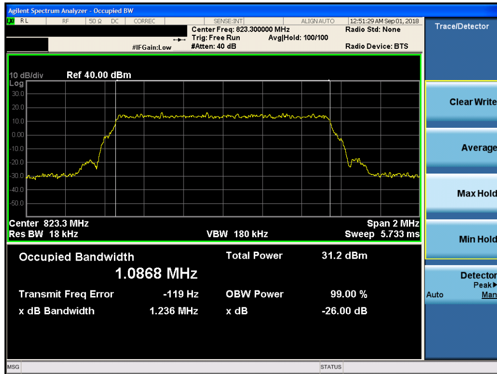
Plot 7-3. Occupied Bandwidth Plot (LTE Band 26, 1.4MHz 64-QAM – RB Size 6– High Channel)
