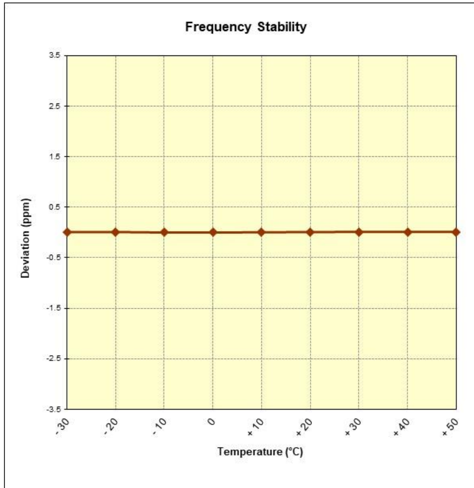
Figure 7-8. LTE Band 14 Frequency Stability Data
