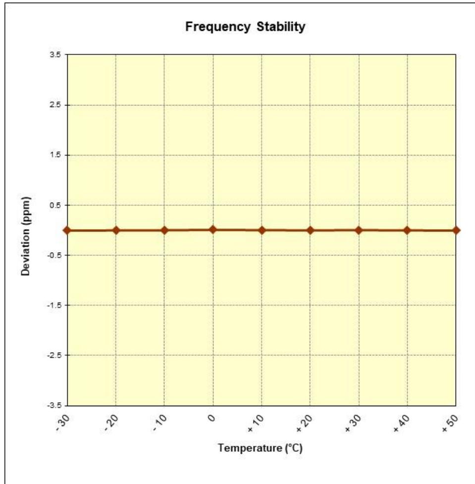
Figure 7-7. LTE Band 26 Frequency Stability Data
