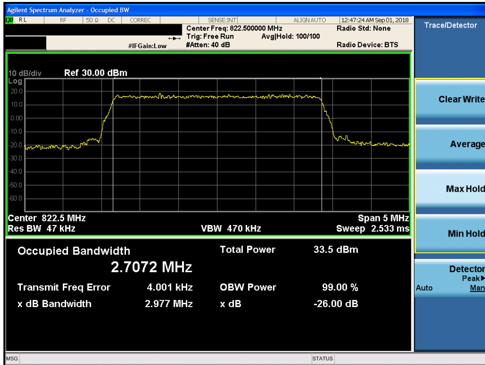
Plot 7-5. Occupied Bandwidth Plot (LTE Band 26, 3MHz 16-QAM – RB Size 15– High Channel)
