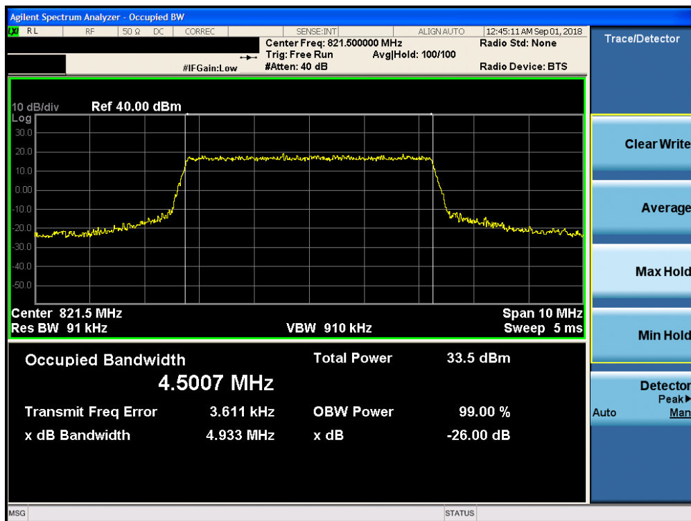
Plot 7-7. Occupied Bandwidth Plot (LTE Band 26, 5MHz QPSK – RB Size 25– High Channel)
