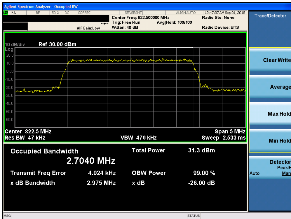
Plot 7-6. Occupied Bandwidth Plot (LTE Band 26, 3MHz 64-QAM – RB Size 15– High Channel)
