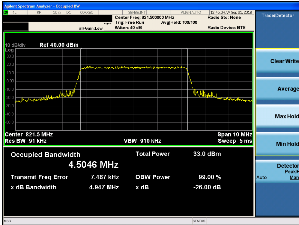
Plot 7-9. Occupied Bandwidth Plot (LTE Band 26, 5MHz 64-QAM – RB Size 25– High Channel)
