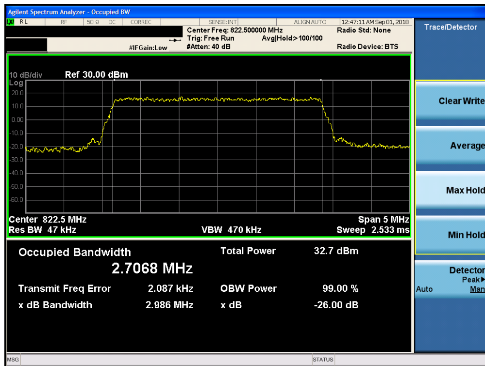
Plot 7-4. Occupied Bandwidth Plot (LTE Band 26, 3MHz QPSK – RB Size 15– High Channel)
