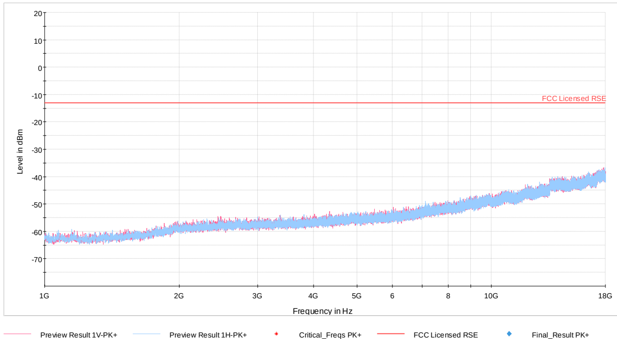
Plot 7-49. Radiated Spurious Plot above 1GHz (Band 26)
