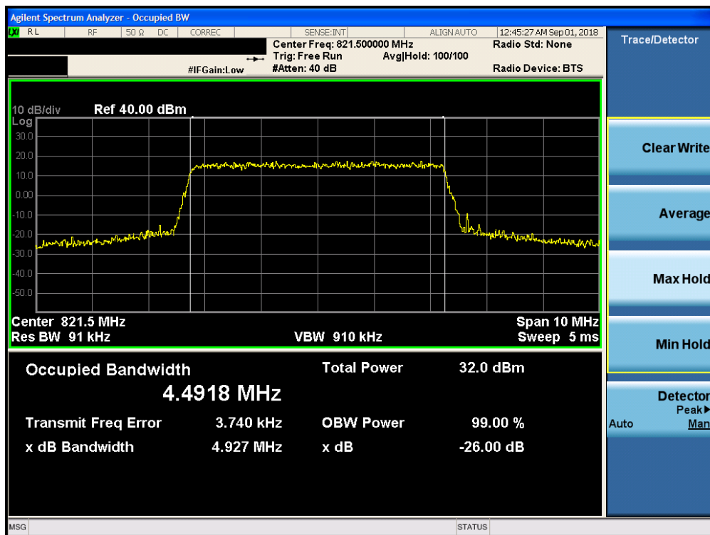
Plot 7-8. Occupied Bandwidth Plot (LTE Band 26, 5MHz 16-QAM – RB Size 25– High Channel)
