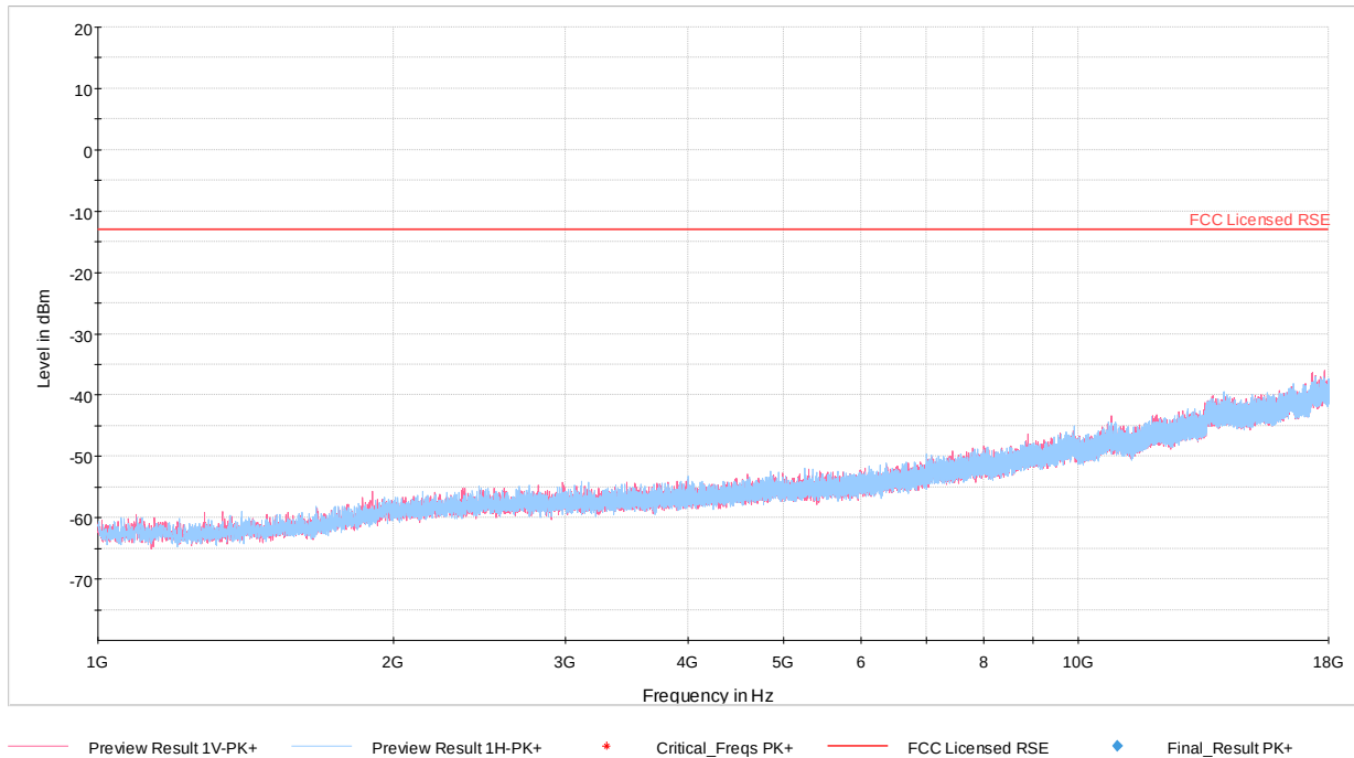
Plot 7-50. Radiated Spurious Plot above 1GHz (Band 14)
