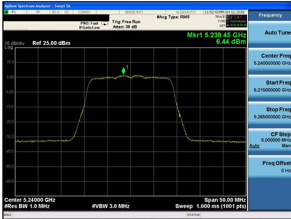
Plot 7-55. Power Spectral Density Plot SISO CORE0 (20MHz BW 802.11n (UNII Band 1) – Ch. 48) - ISED
