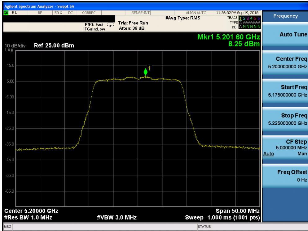
Plot 7-57. Power Spectral Density Plot SISO CORE0 (20MHz BW 802.11n (UNII Band 1) – Ch. 40)
