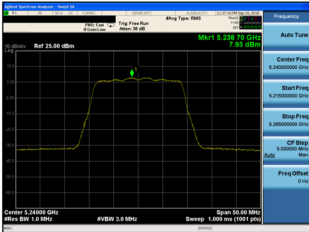
Plot 7-58. Power Spectral Density Plot SISO CORE0 (20MHz BW 802.11n (UNII Band 1) – Ch. 48)
