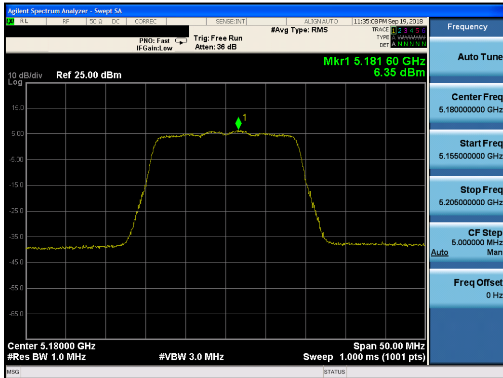
Plot 7-56. Power Spectral Density Plot SISO CORE0 (20MHz BW 802.11n (UNII Band 1) – Ch. 36)
