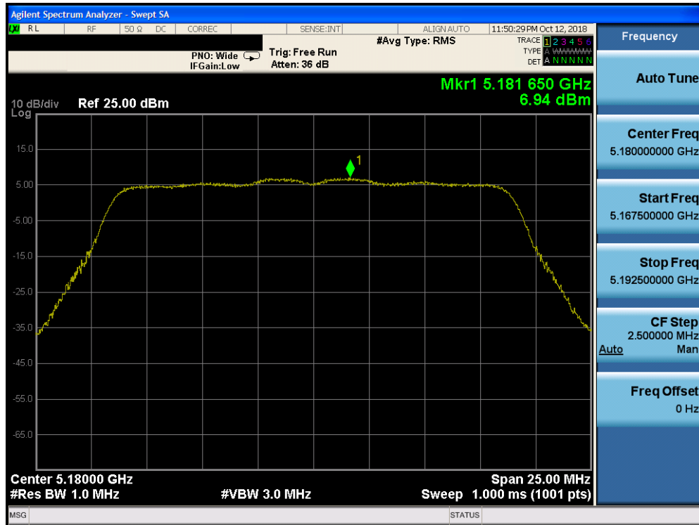
Plot 7-53. Power Spectral Density Plot SISO CORE0 (20MHz BW 802.11n (UNII Band 1) – Ch. 36) - ISED
