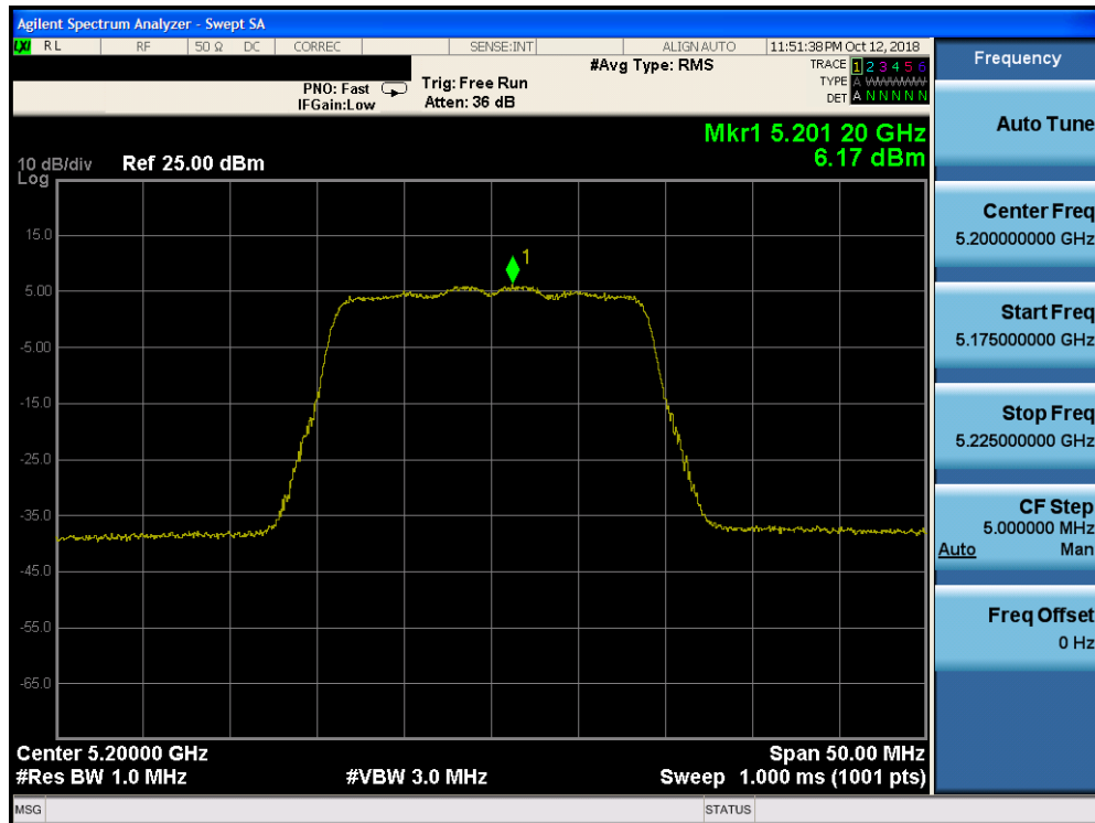
Plot 7-54. Power Spectral Density Plot SISO CORE0 (20MHz BW 802.11n (UNII Band 1) – Ch. 40) - ISED
