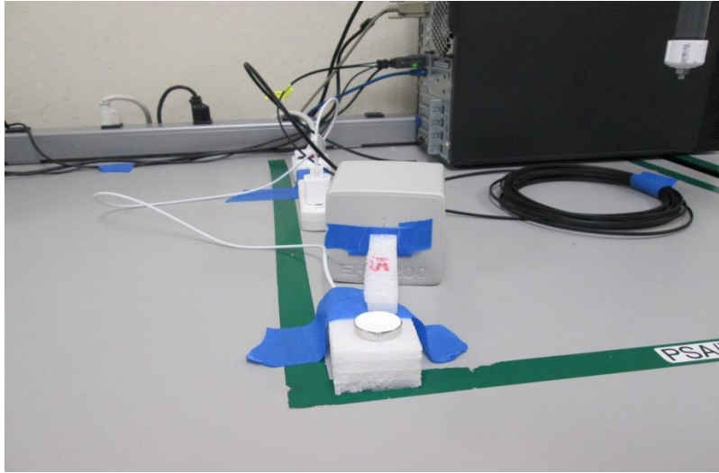
S1, RF EXPOSURE SETUP PHOTO 15cm
