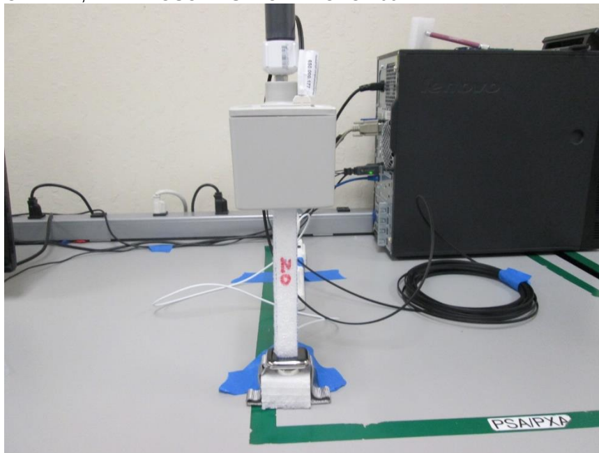
CENTER, RF EXPOSURE SETUP PHOTO 20cm
