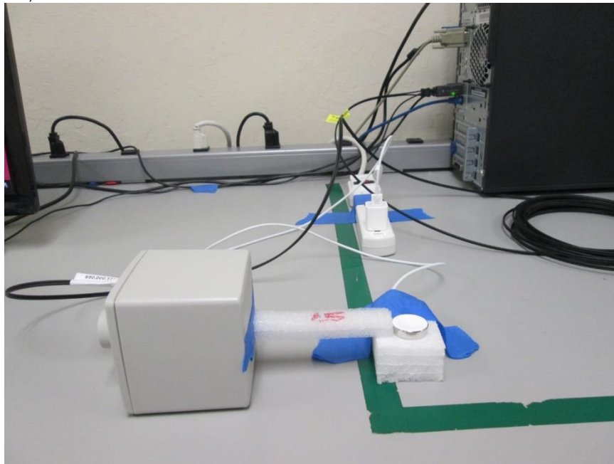
S4, RF EXPOSURE SETUP PHOTO 15cm
