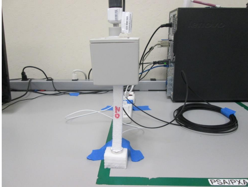
CENTER, RF EXPOSURE SETUP PHOTO 20cm
