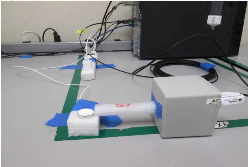
S2, RF EXPOSURE SETUP PHOTO 15cm
