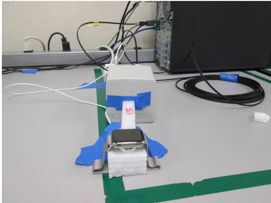
S1, RF EXPOSURE SETUP PHOTO 15cm
