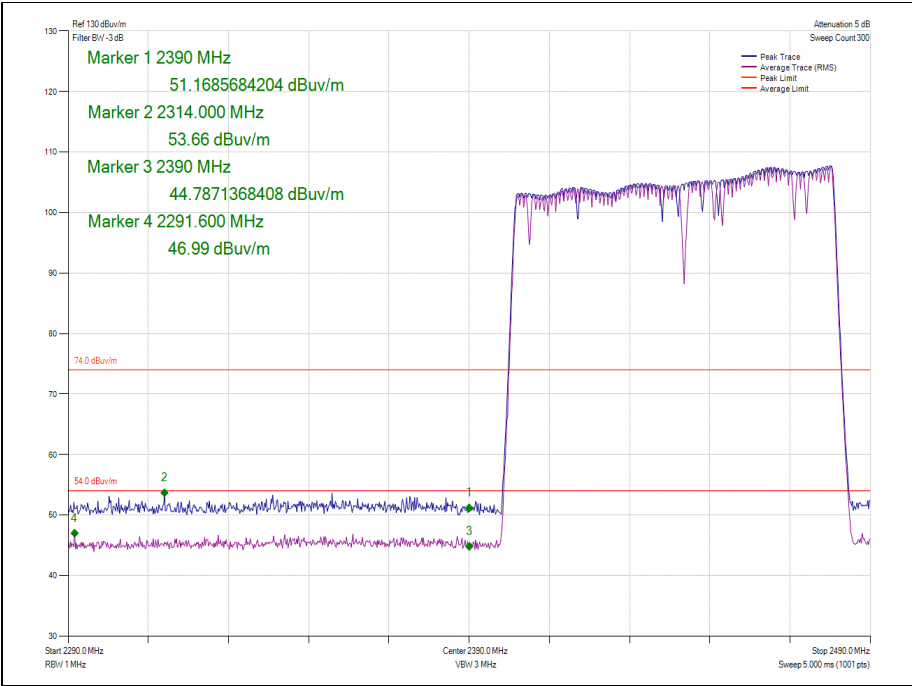
Figure 46 - Hopping - GFSK/DH5 - Measured Frequency 2390.0 MHz
