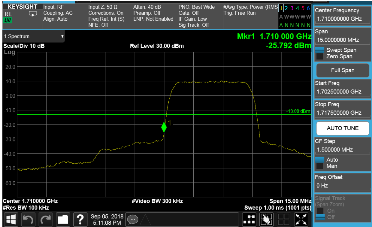
Plot 7-61. Band Edge Plot (AWS WCDMA Mode - Low Channel)
