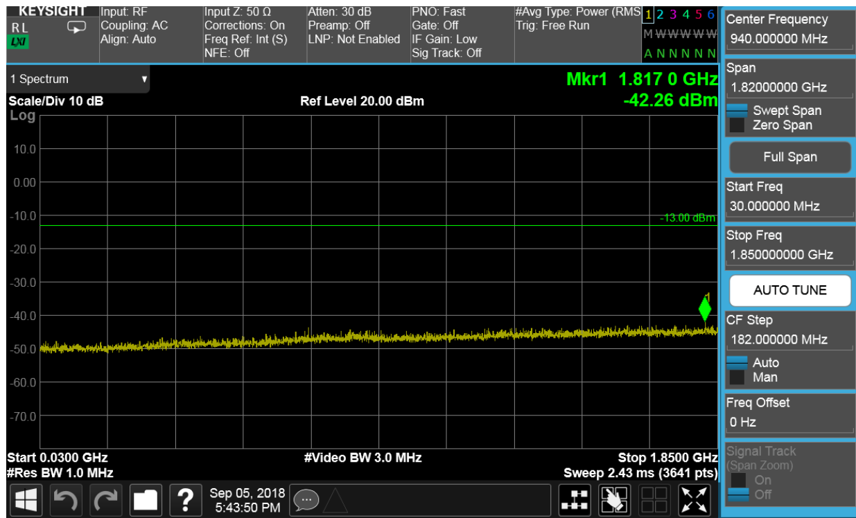
Plot 7-20. Conducted Spurious Plot (PCS GPRS Mode - Mid Channel)
