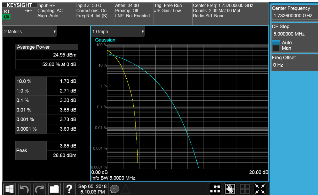
Plot 7-74. Peak-Average Ratio Plot (AWS WCDMA Mode)
