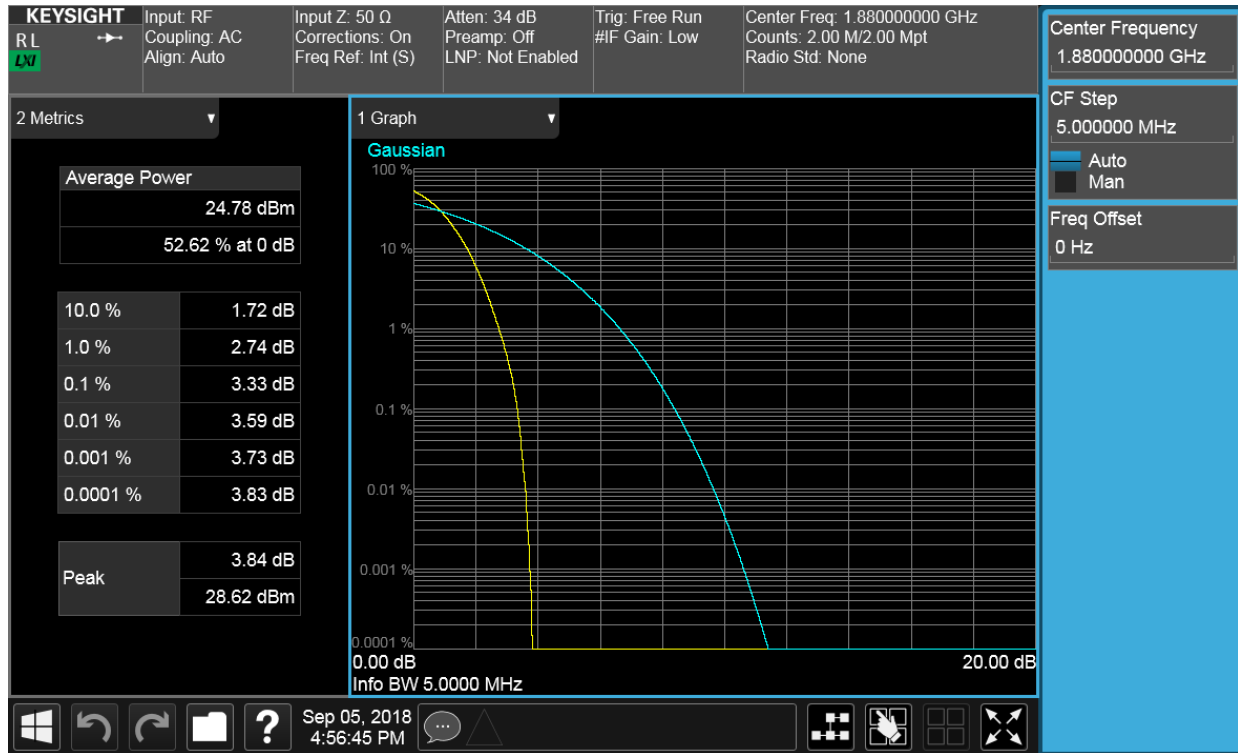
Plot 7-75. Peak-Average Ratio Plot (PCS WCDMA Mode)
