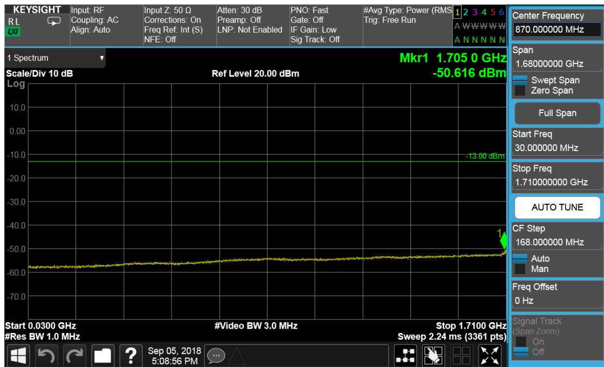
Plot 7-38. Conducted Spurious Plot (AWS WCDMA Mode - Mid Channel)
