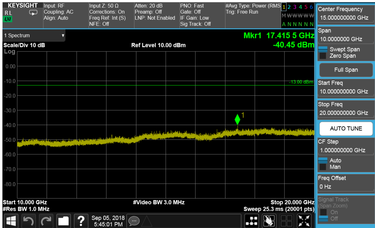
Plot 7-22. Conducted Spurious Plot (PCS GPRS Mode - Mid Channel)
