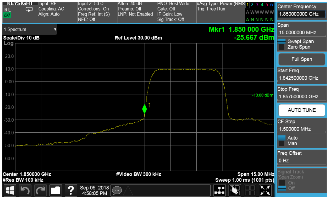
Plot 7-65. Band Edge Plot (PCS WCDMA Mode - Low Channel)
