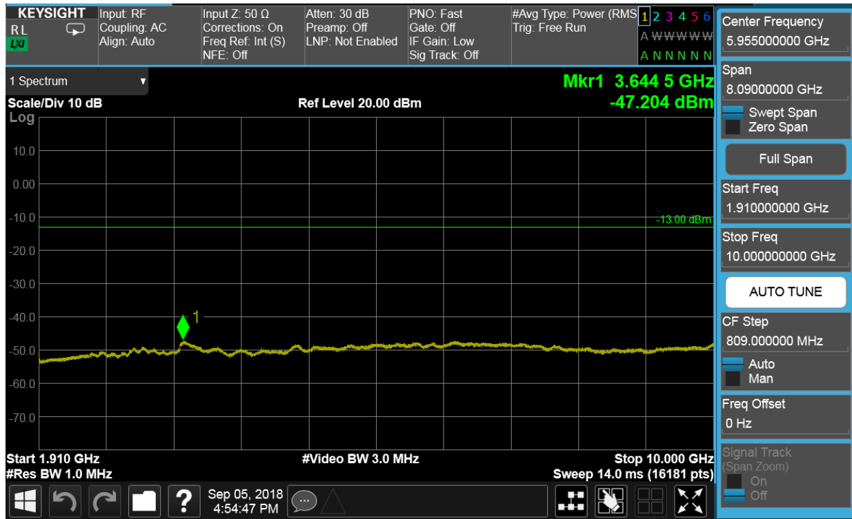
Plot 7-48. Conducted Spurious Plot (PCS WCDMA Mode - Mid Channel)
