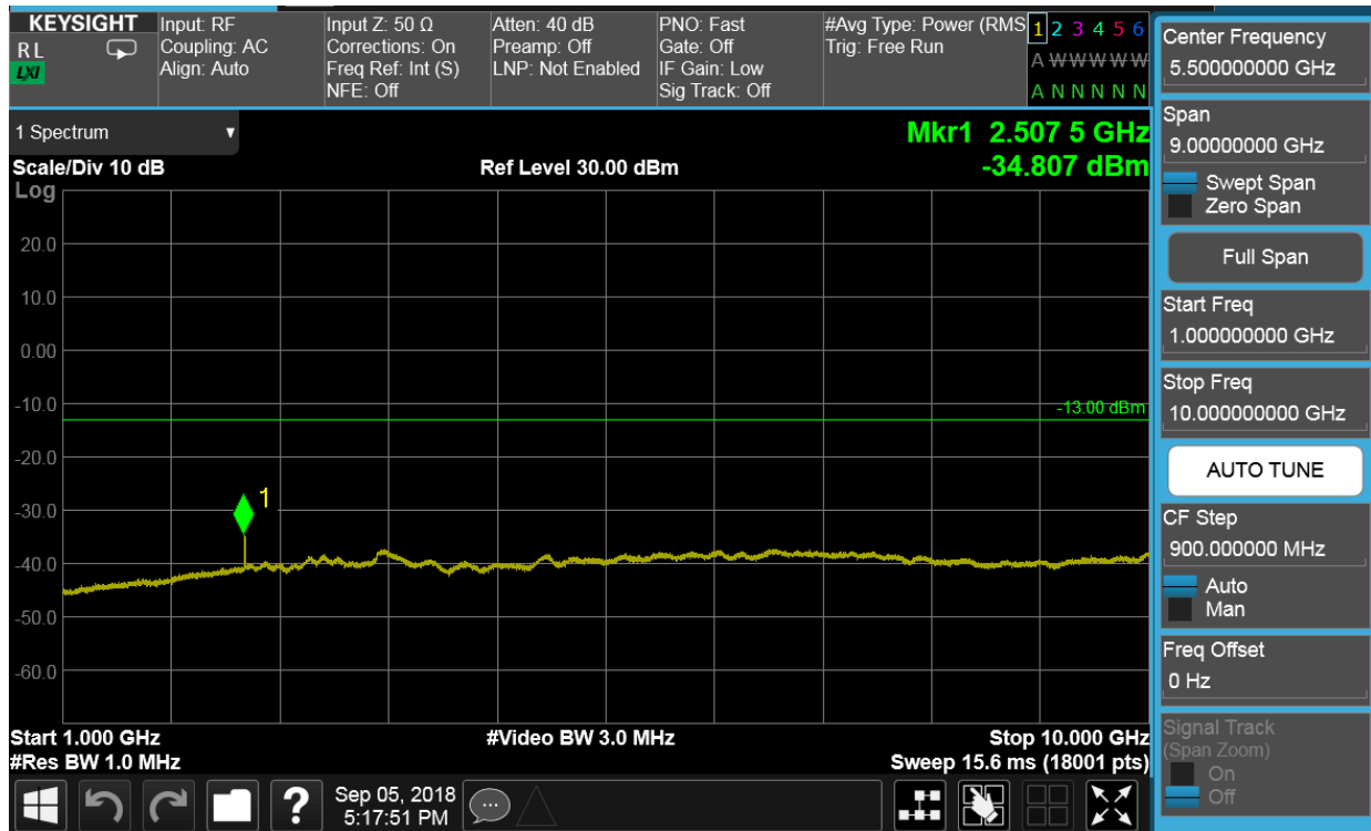
Plot 7-31. Conducted Spurious Plot (Cellular WCDMA Mode - Mid Channel)
