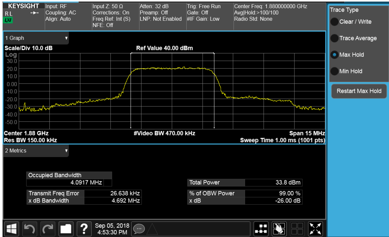
Plot 7-7. Occupied Bandwidth Plot (PCS WCDMA Mode)
