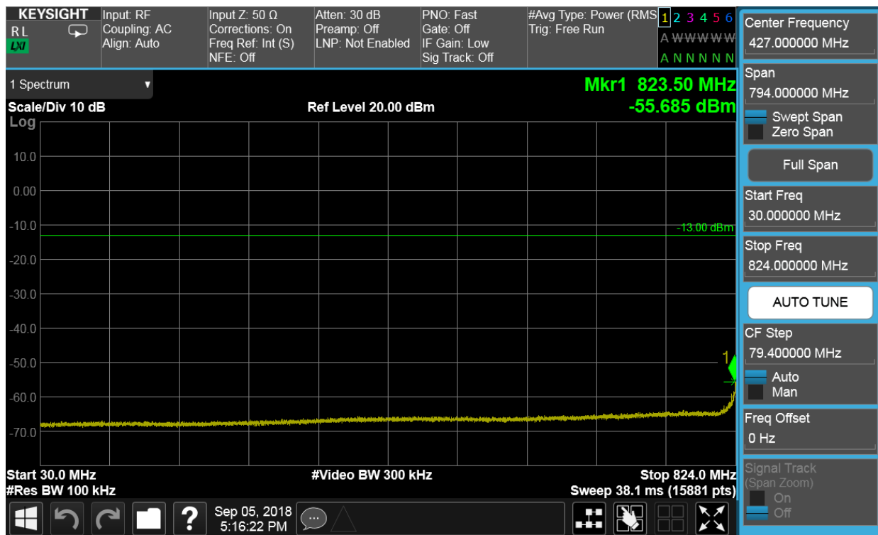
Plot 7-29. Conducted Spurious Plot (Cellular WCDMA Mode - Mid Channel)
