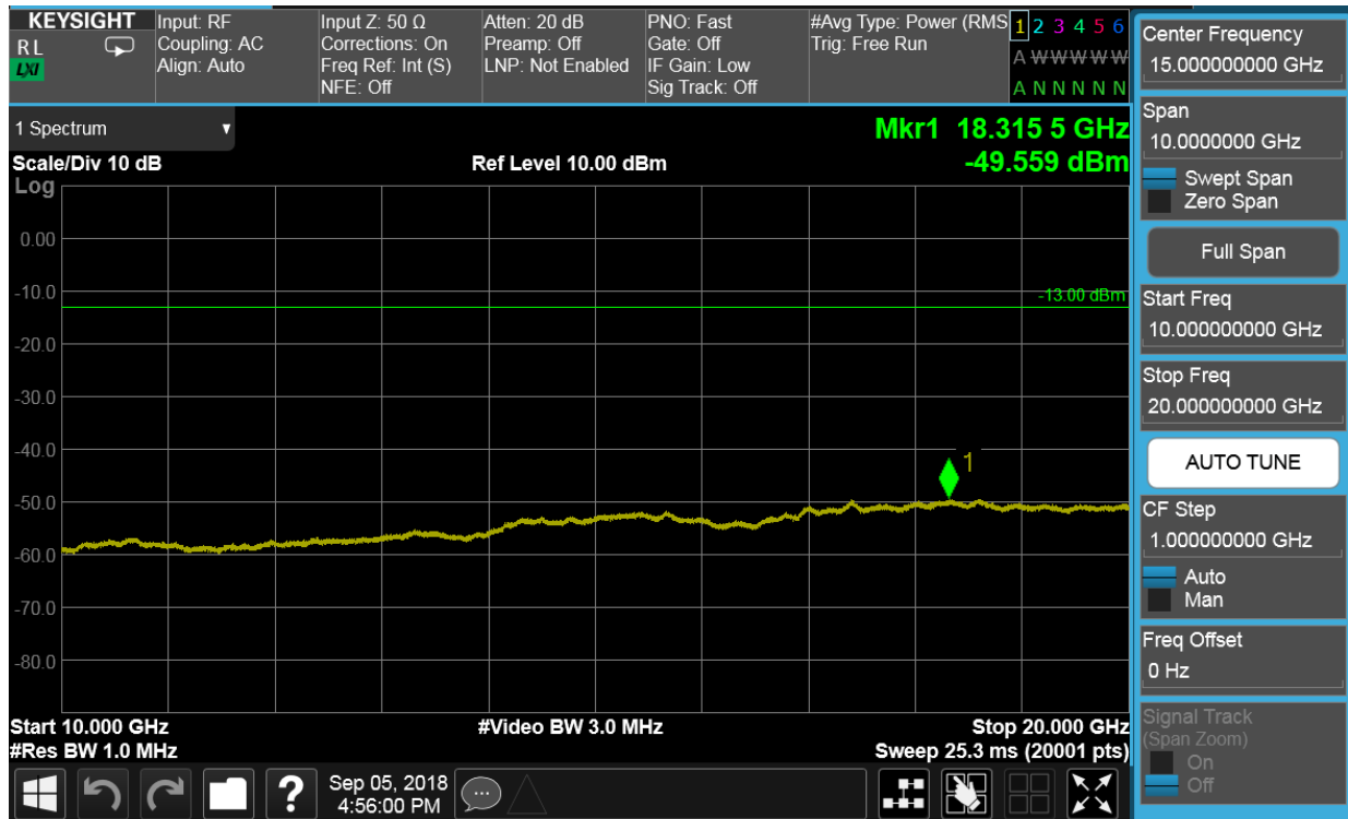
Plot 7-49. Conducted Spurious Plot (PCS WCDMA Mode - Mid Channel)
