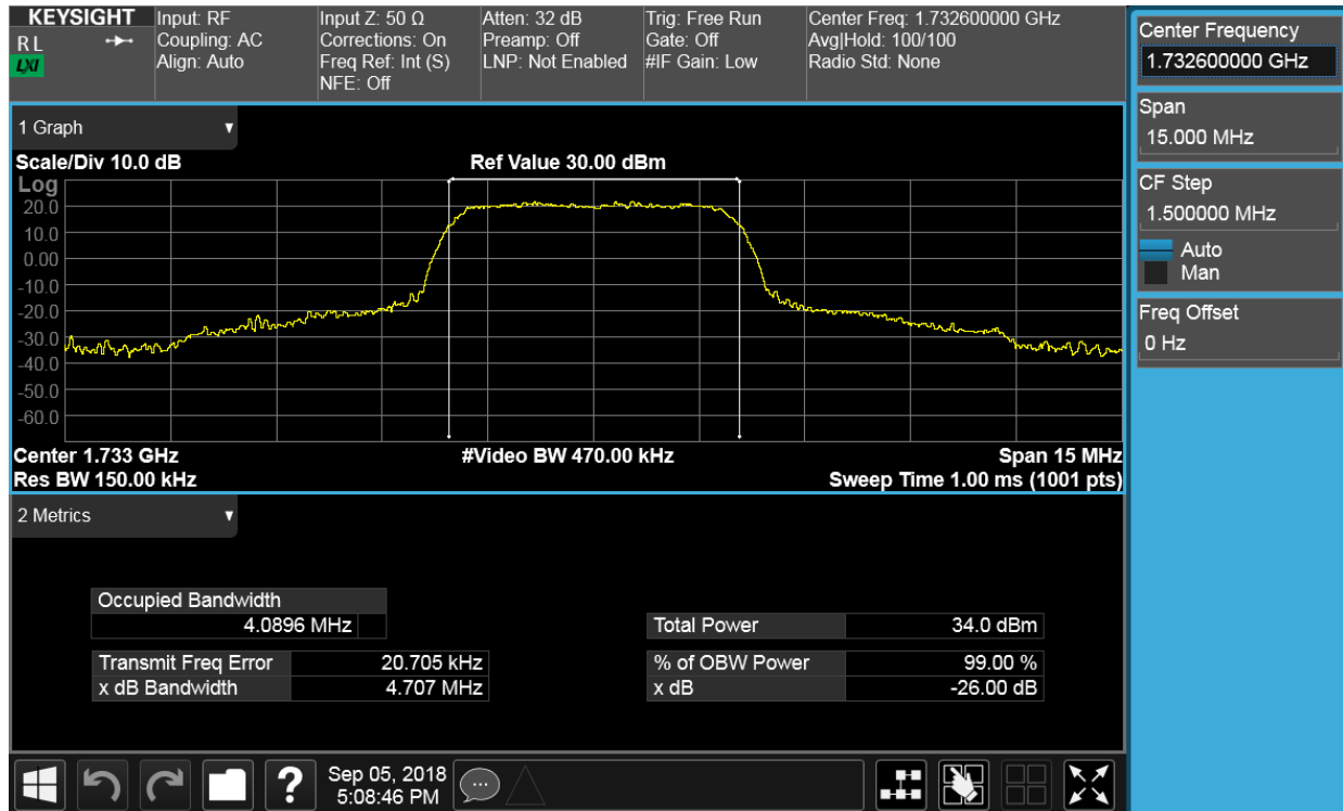
Plot 7-6. Occupied Bandwidth Plot (AWS WCDMA Mode)
