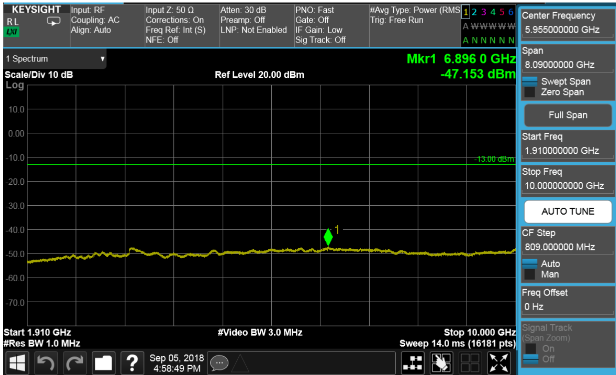
Plot 7-45. Conducted Spurious Plot (PCS WCDMA Mode - Low Channel)
