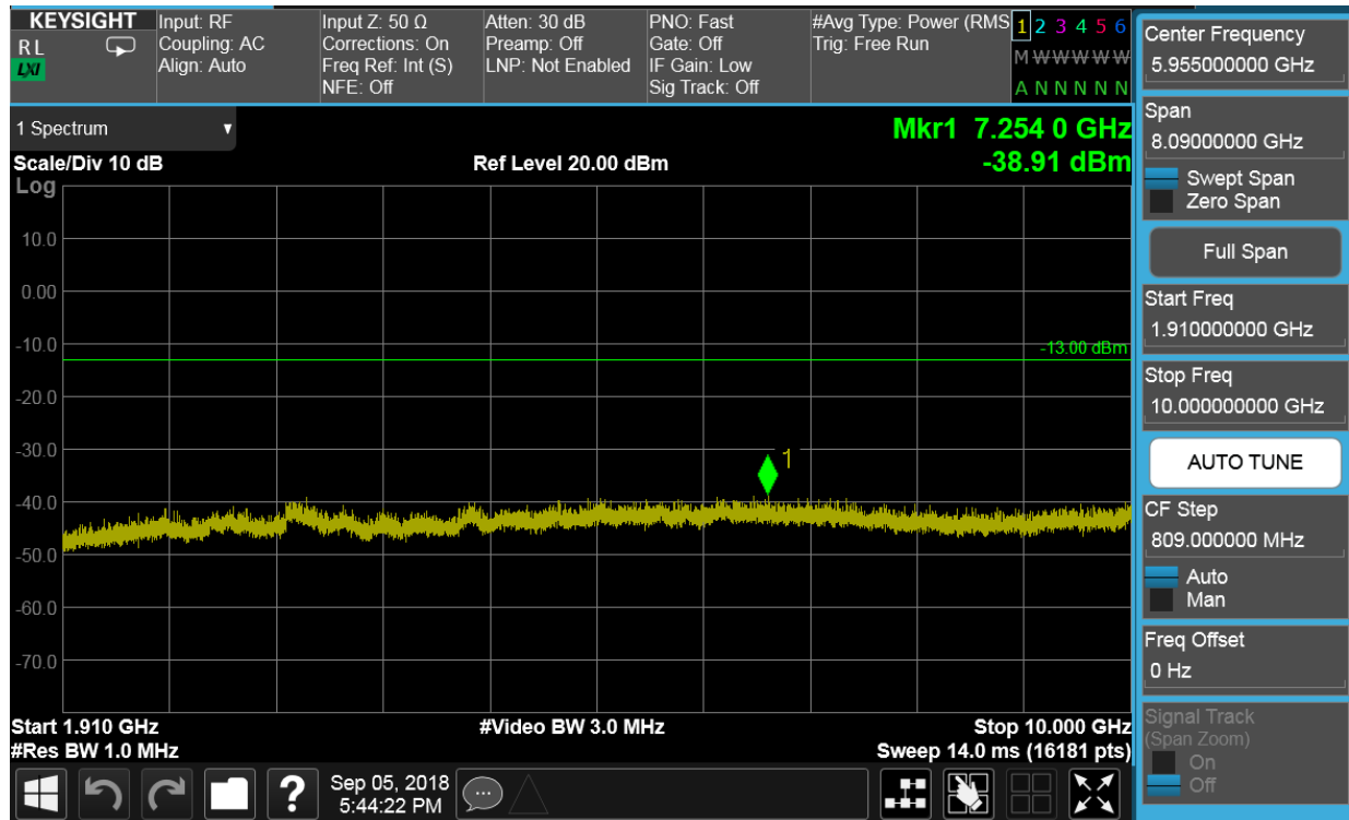
Plot 7-21. Conducted Spurious Plot (PCS GPRS Mode - Mid Channel)
