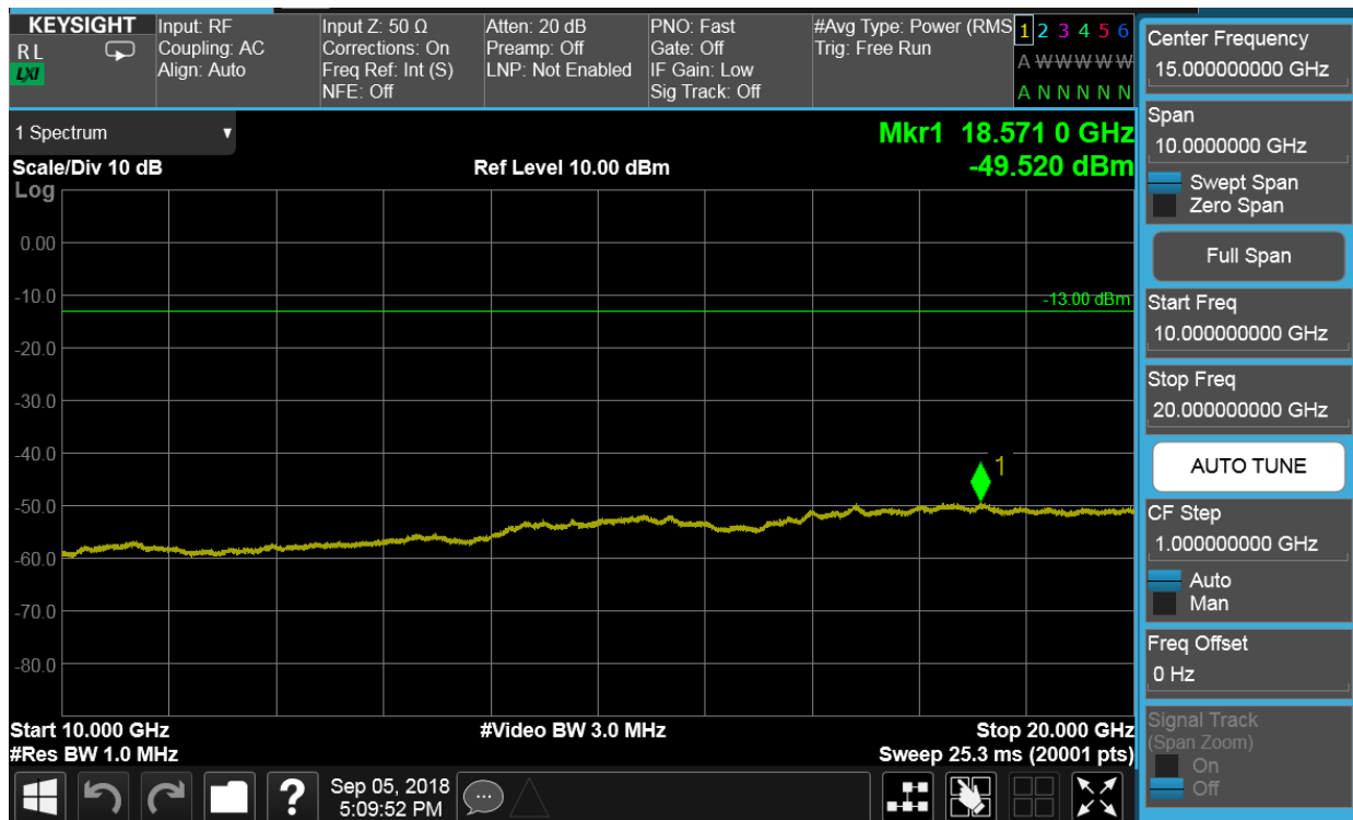
Plot 7-40. Conducted Spurious Plot (AWS WCDMA Mode - Mid Channel)
