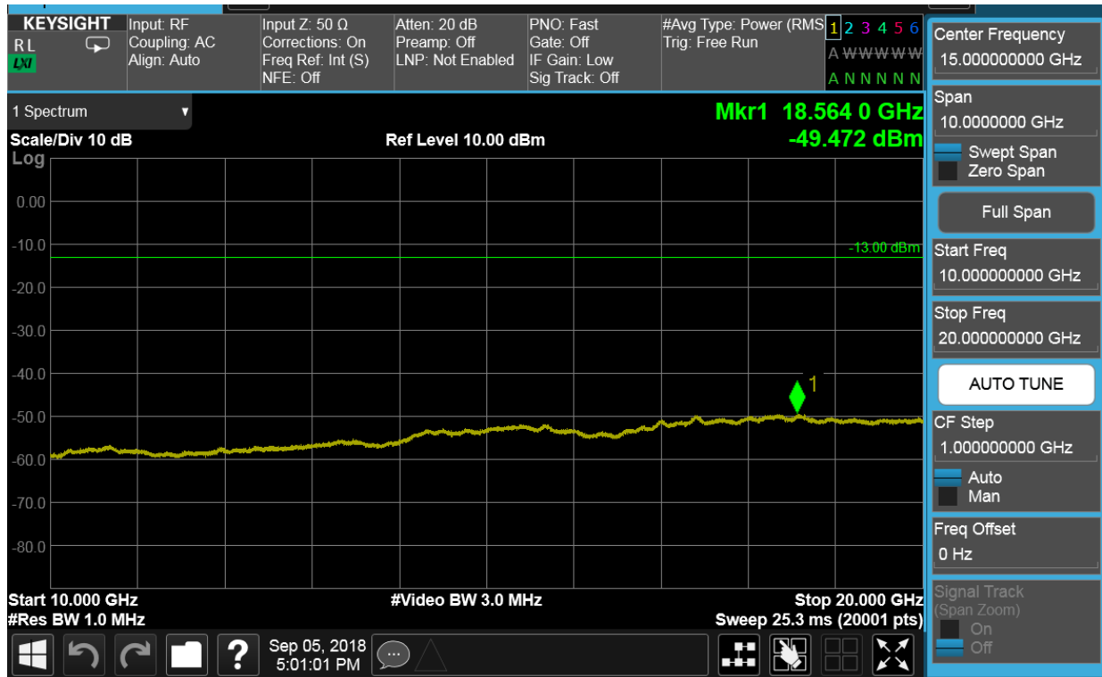
Plot 7-46. Conducted Spurious Plot (PCS WCDMA Mode - Low Channel)
