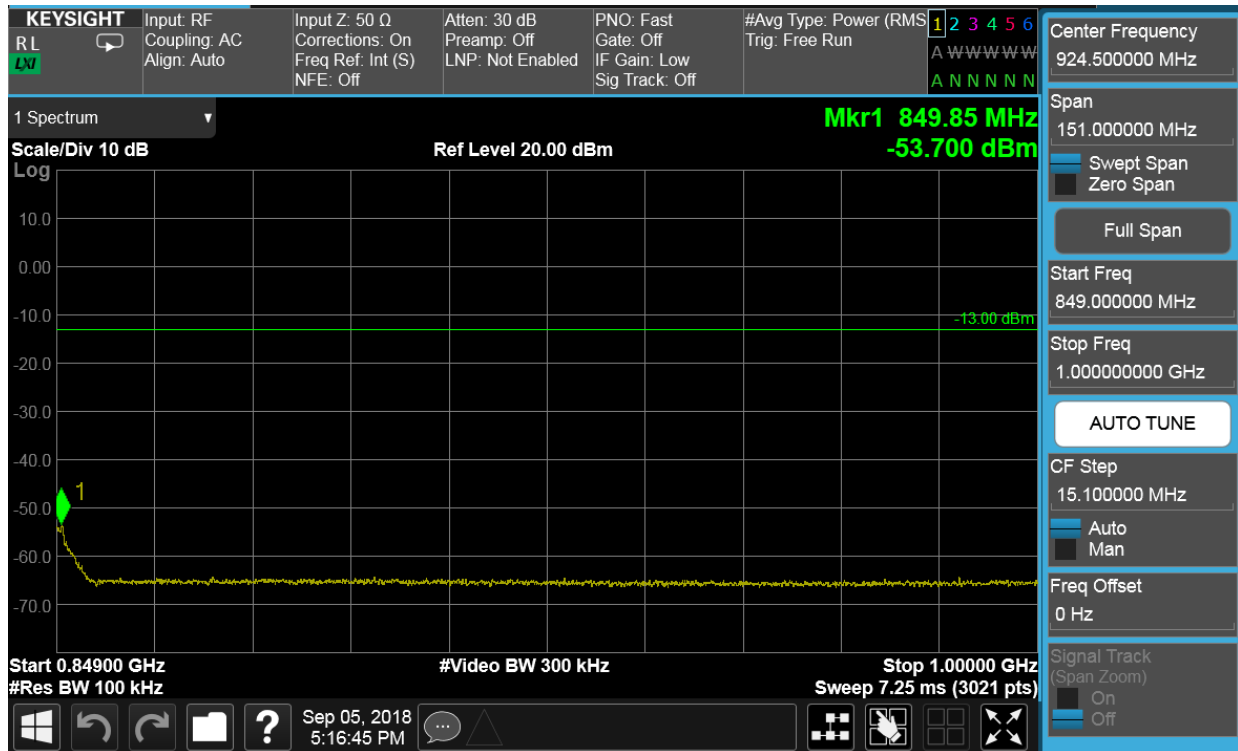
Plot 7-30. Conducted Spurious Plot (Cellular WCDMA Mode - Mid Channel)
