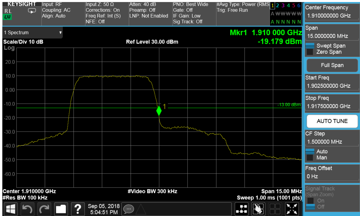
Plot 7-67. Band Edge Plot (PCS WCDMA Mode - High Channel)
