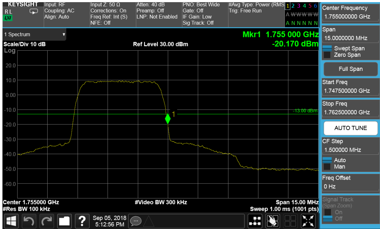
Plot 7-63. Band Edge Plot (AWS WCDMA Mode - High Channel)
