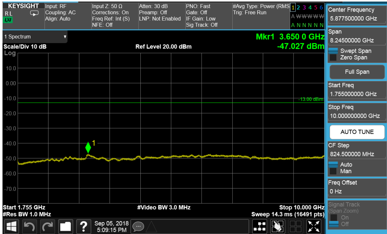
Plot 7-39. Conducted Spurious Plot (AWS WCDMA Mode - Mid Channel)
