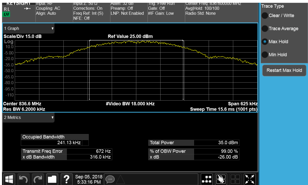
Plot 7-1. Occupied Bandwidth Plot (Cellular GPRS Mode)
