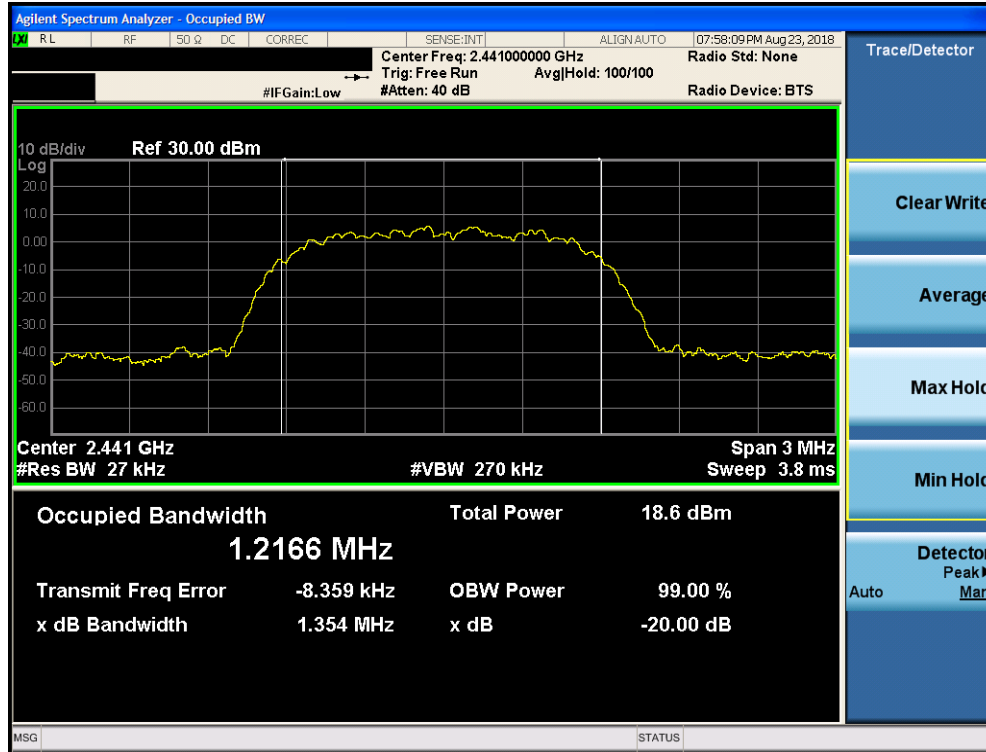
Plot 7-11. 20dB Bandwidth Plot ANT 1 (Bluetooth, 8DPSK, ePA – Ch. 39)
