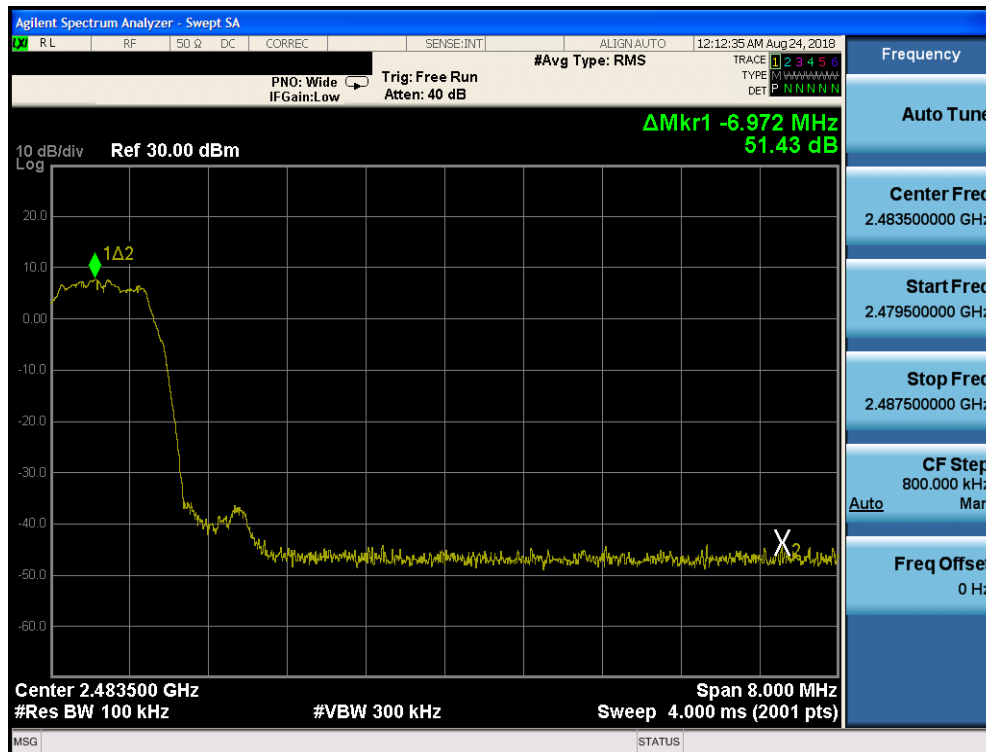
Plot 7-40. Band Edge Plot ANT 2 (Bluetooth with Hopping Disabled, 8DPSK, ePA – Ch. 78)
