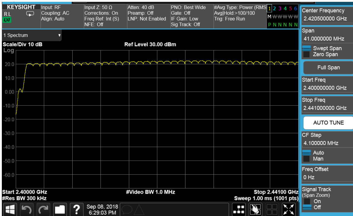
Plot 7-57. Low End Spectrum Channel Hopping Plot ANT0 (Bluetooth, 8DPSK, ePA)
