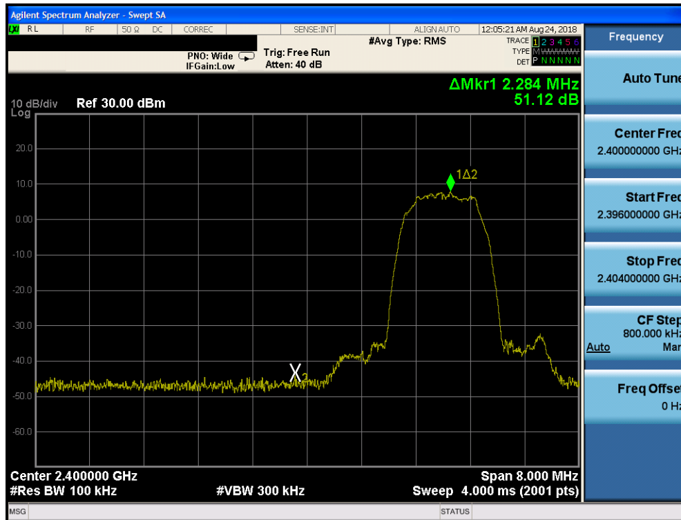
Plot 7-39. Band Edge Plot ANT 2 (Bluetooth with Hopping Disabled, 8DPSK, ePA – Ch. 0)
