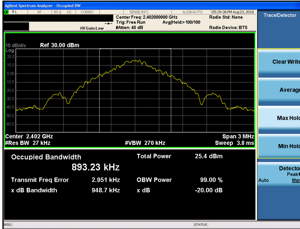
Plot 7-1. 20dB Bandwidth Plot ANT 0 (Bluetooth, GFSK, ePA – Ch. 0)
