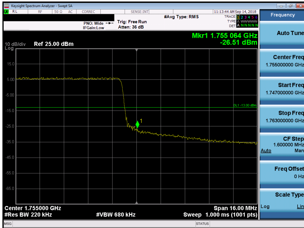
Plot 7-221. Upper Band Edge Plot (Band 4 – 20.0MHz QPSK – RB Size 100)
