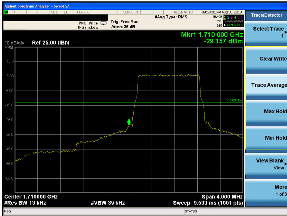
Plot 7-223. Lower Band Edge Plot (Band 66 – 1.4MHz QPSK – RB Size 6)
