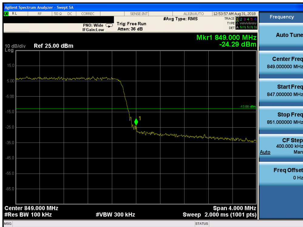
Plot 7-188. Upper Band Edge Plot (Band 5 - 5.0MHz QPSK - RB Size 25)
