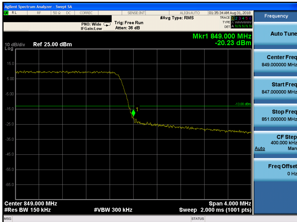
Plot 7-196. Upper Band Edge Plot (Band 26 – 5.0MHz QPSK – RB Size 25)
