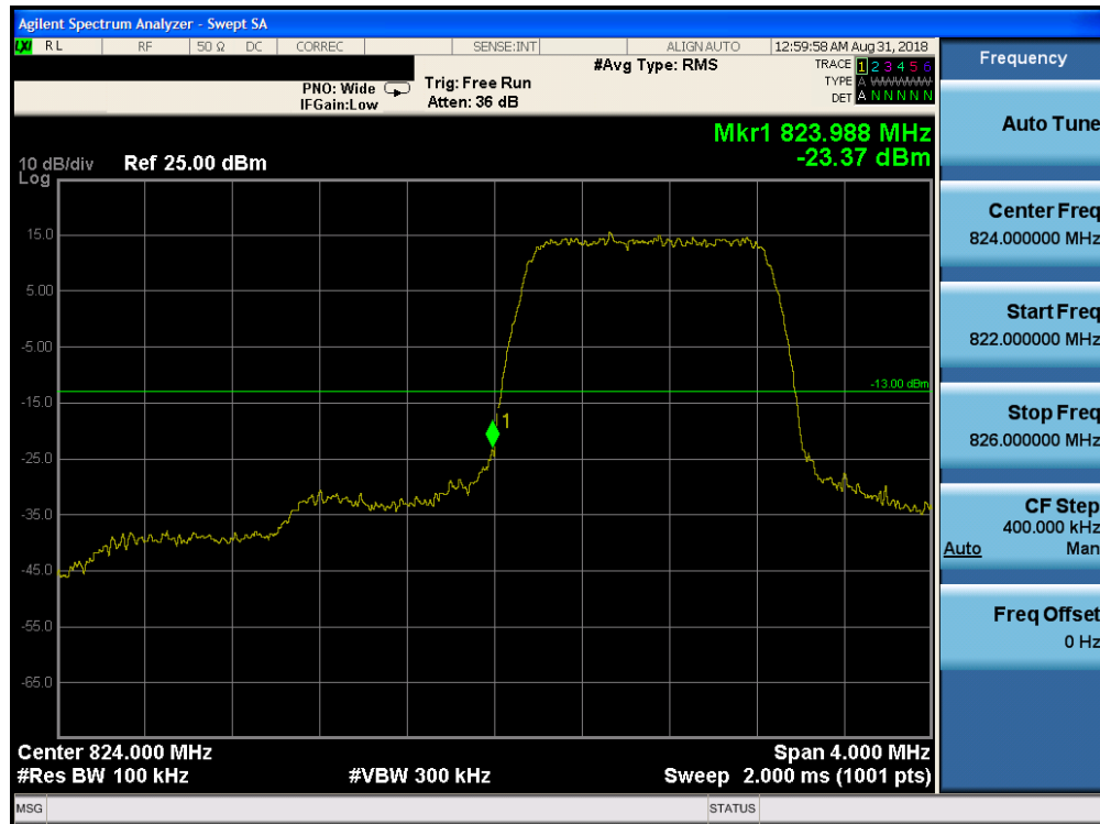
Plot 7-183. Lower Band Edge Plot (Band 5 – 1.4MHz QPSK – RB Size 6)
