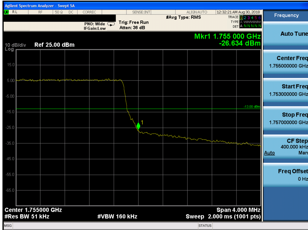
Plot 7-209. Upper Band Edge Plot (Band 4 – 5.0MHz QPSK – RB Size 25)
