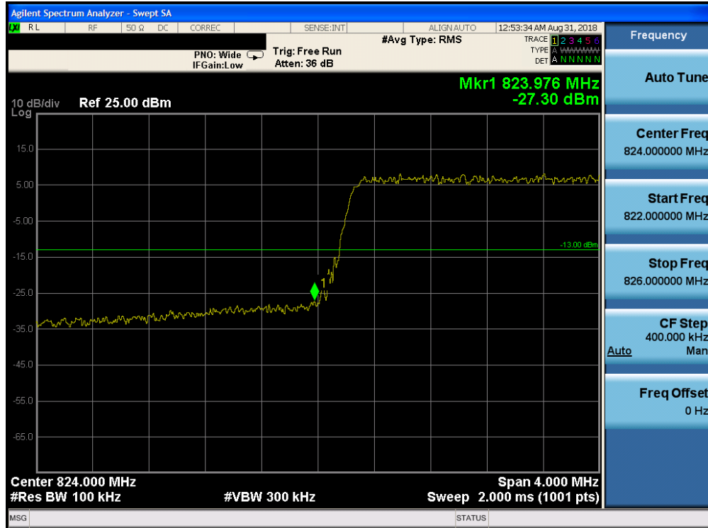
Plot 7-187. Lower Band Edge Plot (Band 5 - 5.0MHz QPSK - RB Size 25)
