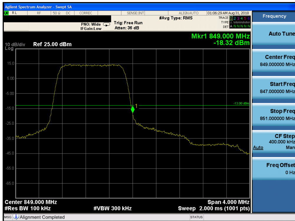
Plot 7-184. Upper Band Edge Plot (Band 5 – 1.4MHz QPSK – RB Size 6)
