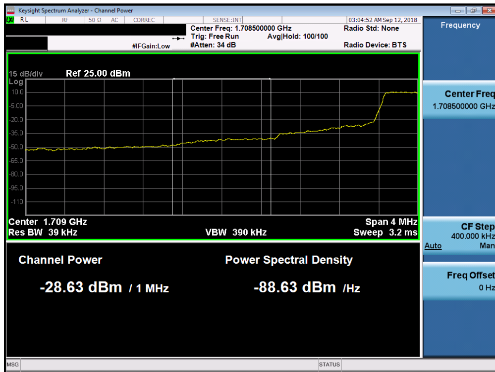
Plot 7-224. Lower Extended Band Edge Plot (Band 66 – 1.4MHz QPSK – RB Size 6)
