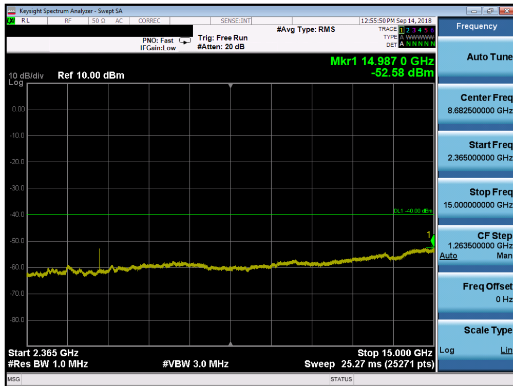
Plot 7-143. Conducted Spurious Plot (Band 30 – 10.0MHz QPSK – RB Size 1, RB Offset 0 – Mid Channel)
