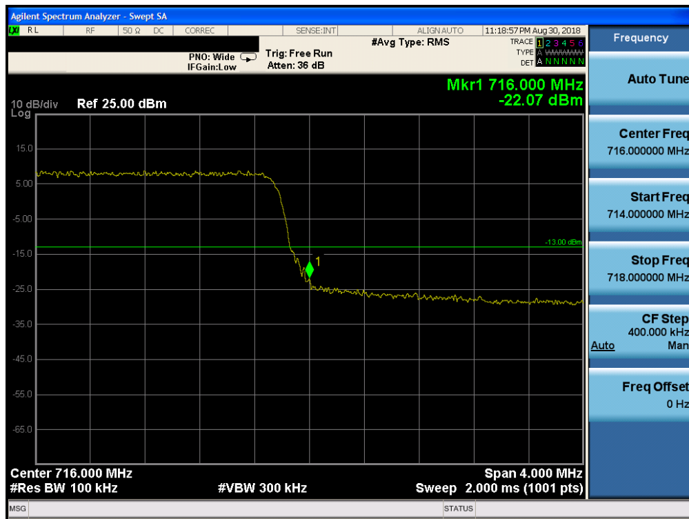
Plot 7-172. Upper Band Edge Plot (Band 17 – 5.0MHz QPSK – RB Size 25)
