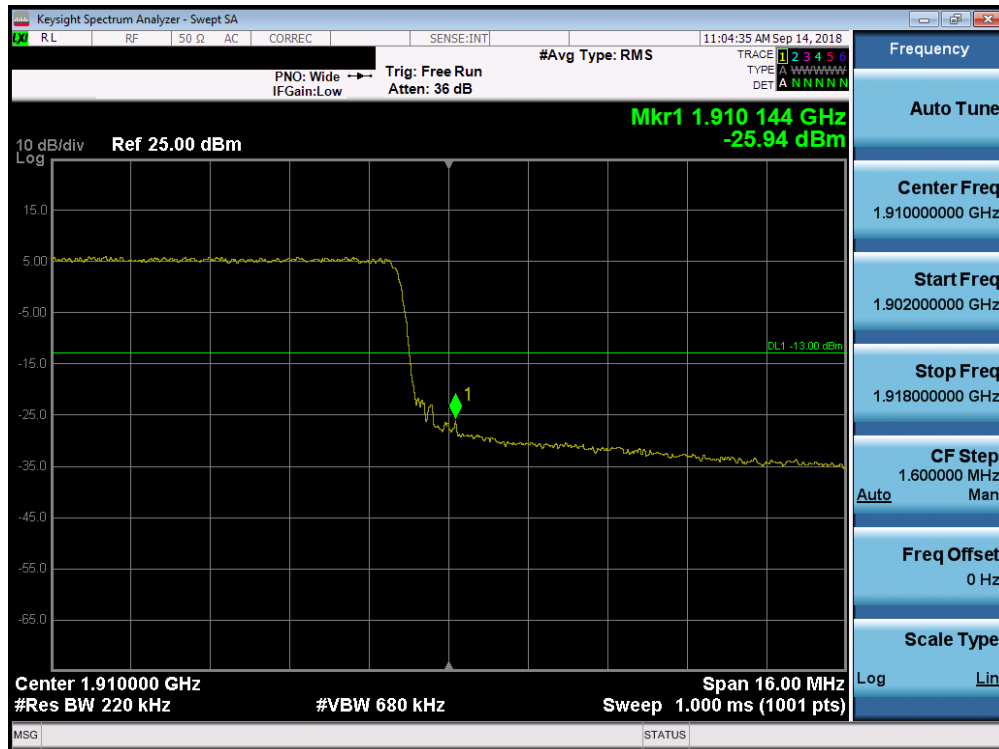
Plot 7-269. Upper Band Edge Plot (Band 2 - 20.0MHz QPSK - RB Size 100)
