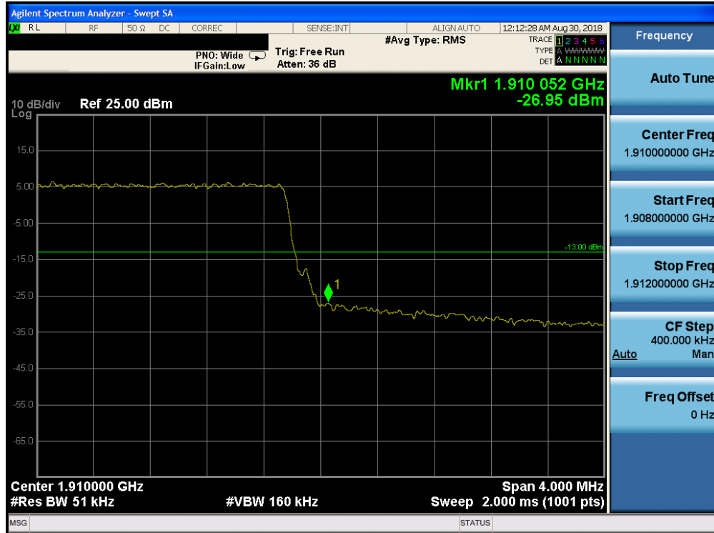
Plot 7-257. Upper Band Edge Plot (Band 2 – 5.0MHz QPSK – RB Size 25)
