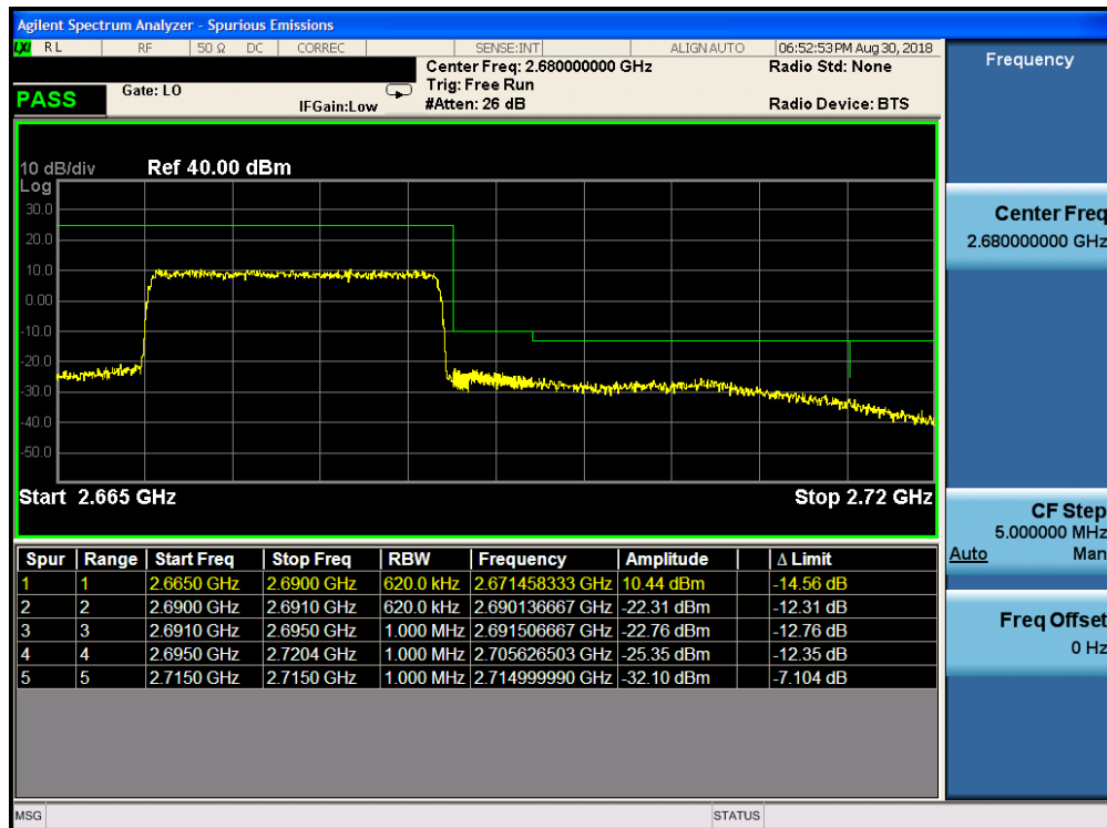
Plot 7-319. Upper ACP Plot (Band 41 – 20.0MHz QPSK – RB Size 100)
