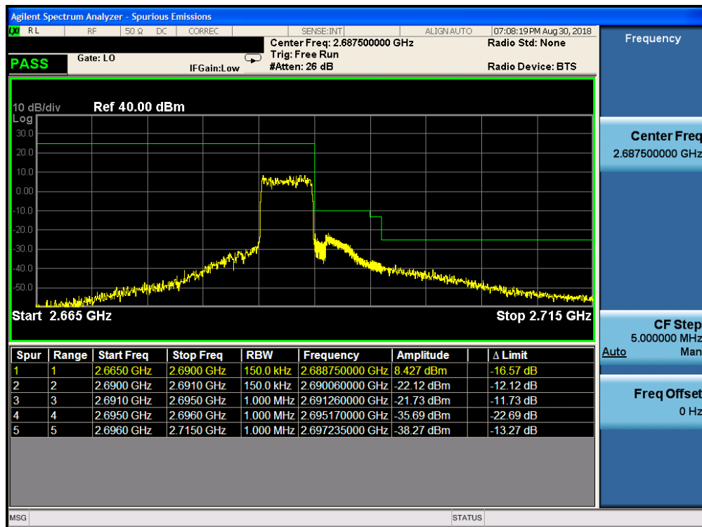
Plot 7-313. Upper ACP Plot (Band 41 – 5.0MHz QPSK – RB Size 25)
