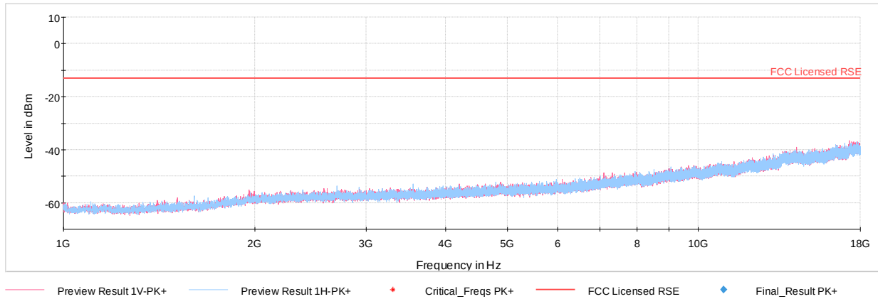
Plot 7-48. Radiated Spurious Plot above 1GHz (Band 14)
