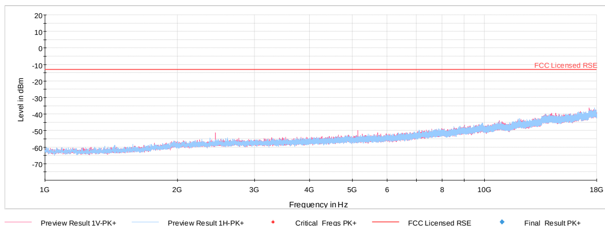
Plot 7-47. Radiated Spurious Plot above 1GHz (Band 26)
