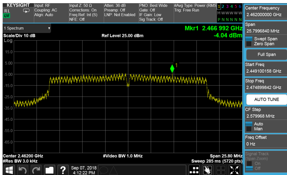
Plot 7-54. Power Spectral Density Plot SISO CORE1 DIVERSITY (802.11n (2.4GHz) – Ch. 11)
