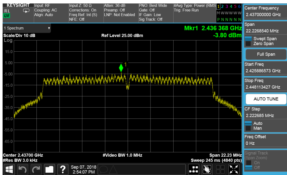
Plot 7-32. Power Spectral Density Plot SISO CORE0 (802.11g - Ch. 6)
