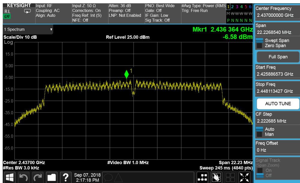
Plot 7-41. Power Spectral Density Plot SISO CORE1 PRIMARY (802.11g – Ch. 6)
