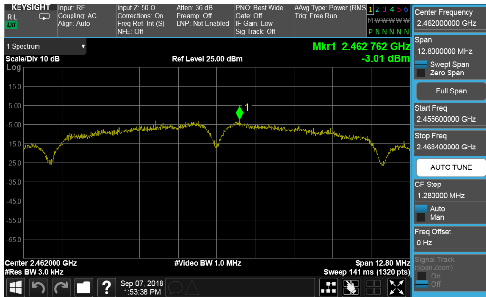
Plot 7-39. Power Spectral Density Plot SISO CORE1 PRIMARY (802.11b – Ch. 11)
