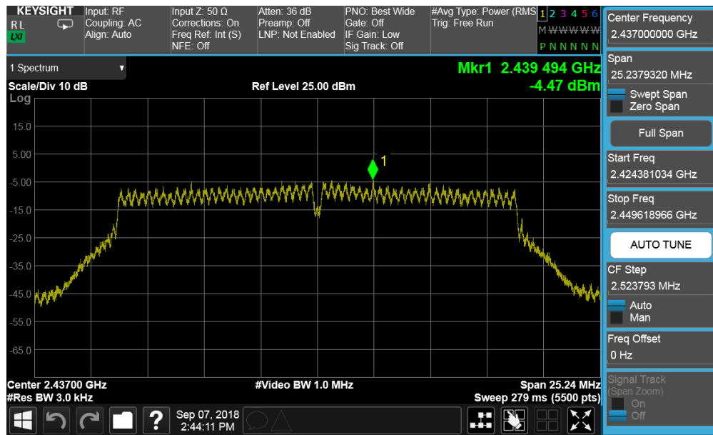
Plot 7-35. Power Spectral Density Plot SISO CORE0 (802.11n (2.4GHz) – Ch. 6)
