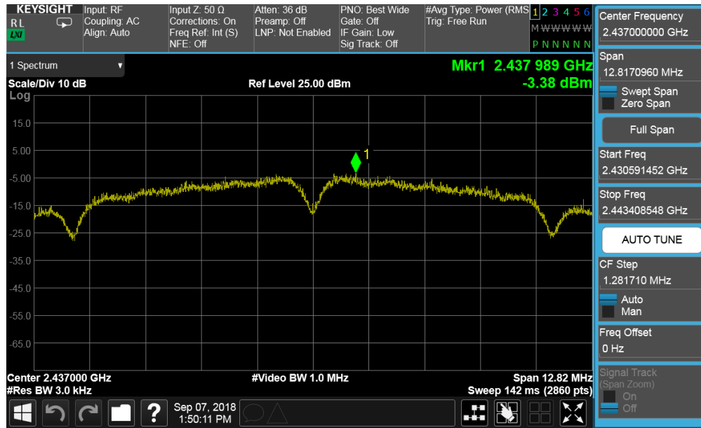
Plot 7-38. Power Spectral Density Plot SISO CORE1 PRIMARY (802.11b – Ch. 6)
