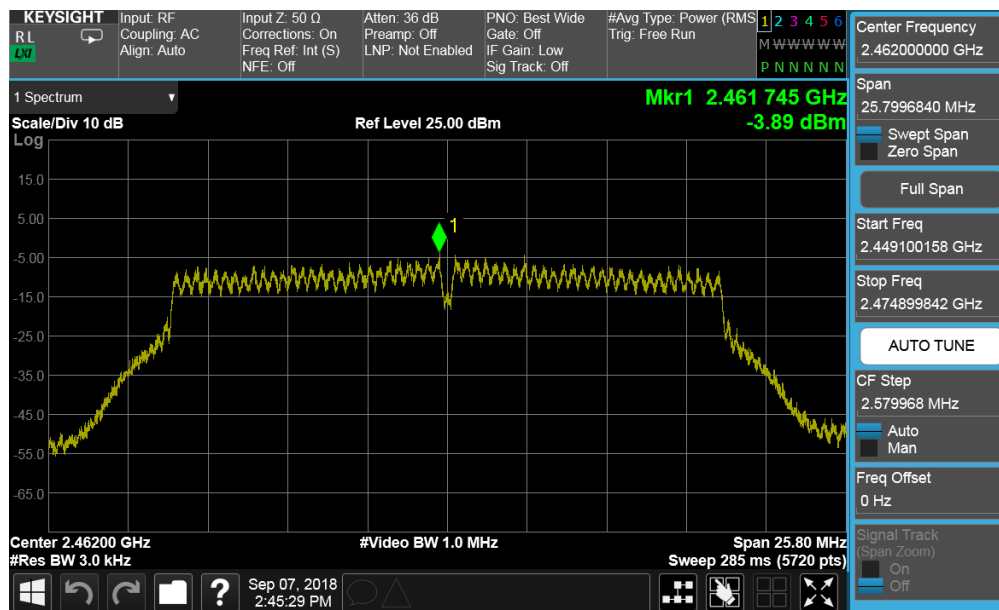
Plot 7-36. Power Spectral Density Plot SISO CORE0 (802.11n (2.4GHz) – Ch. 11)
