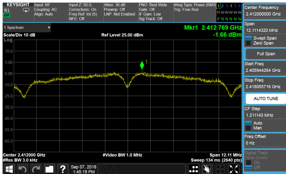
Plot 7-37. Power Spectral Density Plot SISO CORE1 PRIMARY (802.11b – Ch. 1)
