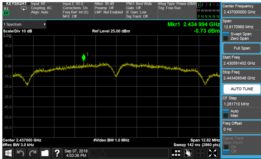
Plot 7-47. Power Spectral Density Plot SISO CORE1 DIVERSITY (802.11b – Ch. 6)
