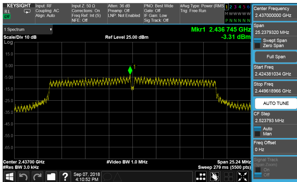
Plot 7-53. Power Spectral Density Plot SISO CORE1 DIVERSITY (802.11n (2.4GHz) – Ch. 6)
