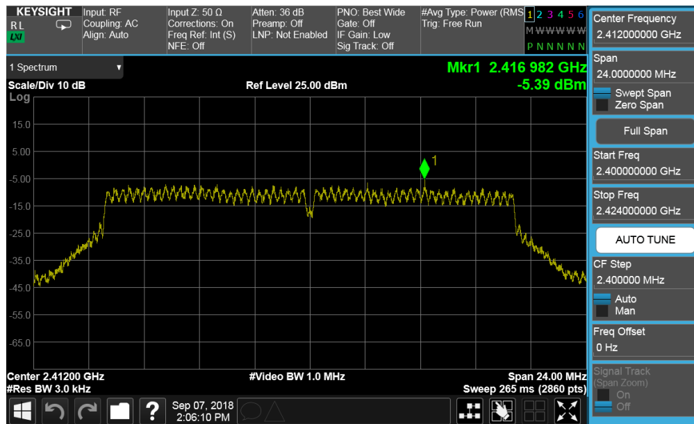
Plot 7-43. Power Spectral Density Plot SISO CORE1 PRIMARY (802.11n (2.4GHz) – Ch. 1)
