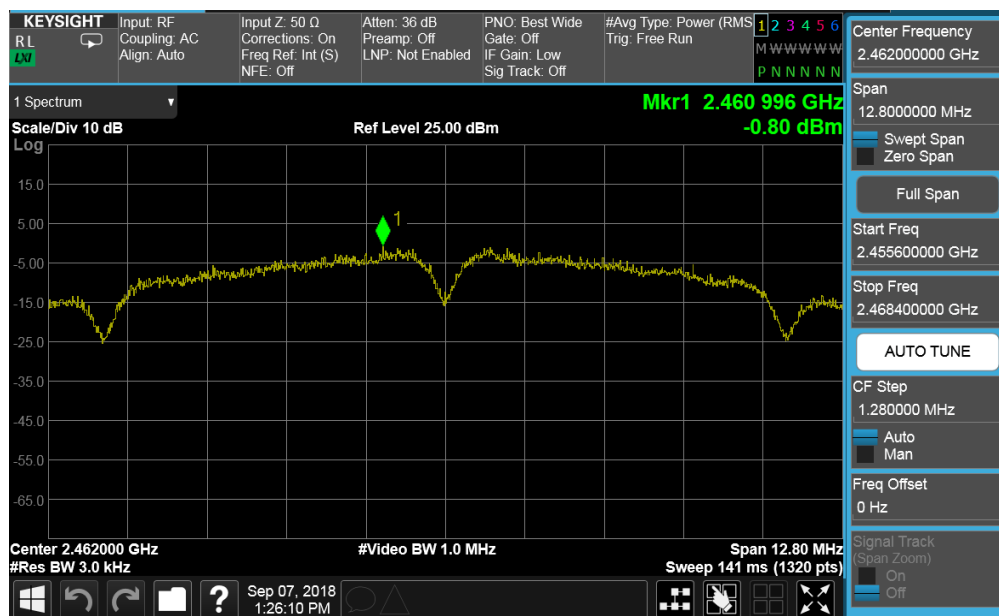
Plot 7-30. Power Spectral Density Plot SISO CORE0 (802.11b – Ch. 11)
