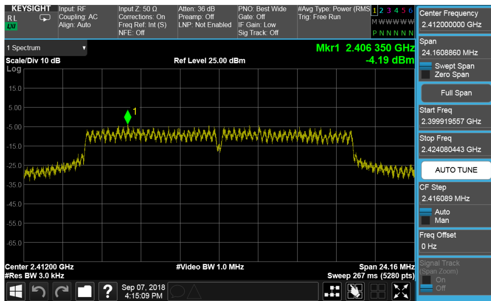
Plot 7-49. Power Spectral Density Plot SISO CORE1 DIVERSITY (802.11g – Ch. 1)
