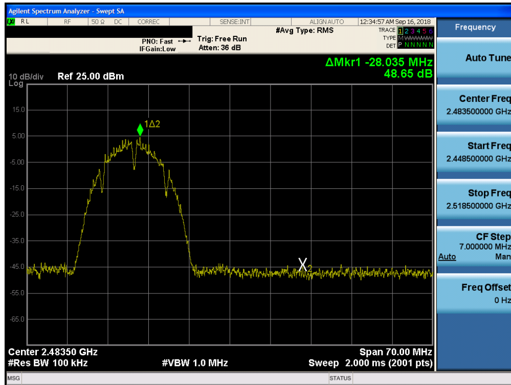
Plot 7-81. Band Edge Plot SISO CORE0 (802.11b - Ch. 12)
