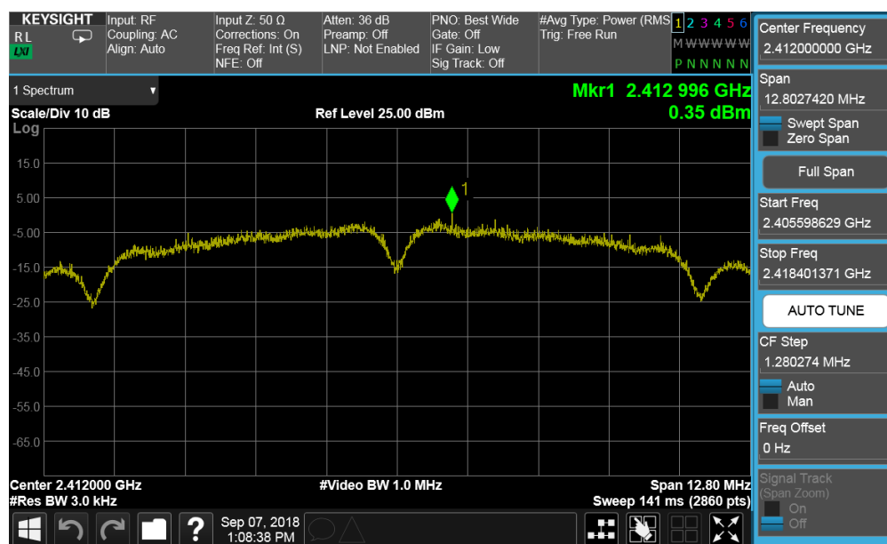
Plot 7-28. Power Spectral Density Plot SISO CORE0 (802.11b – Ch. 1)
