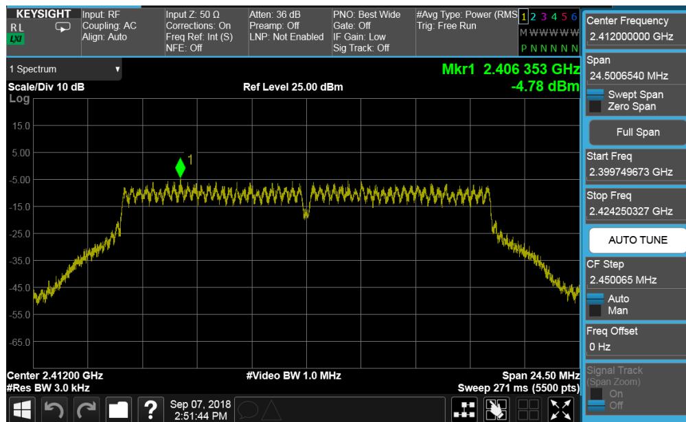
Plot 7-31. Power Spectral Density Plot SISO CORE0 (802.11g - Ch. 1)
