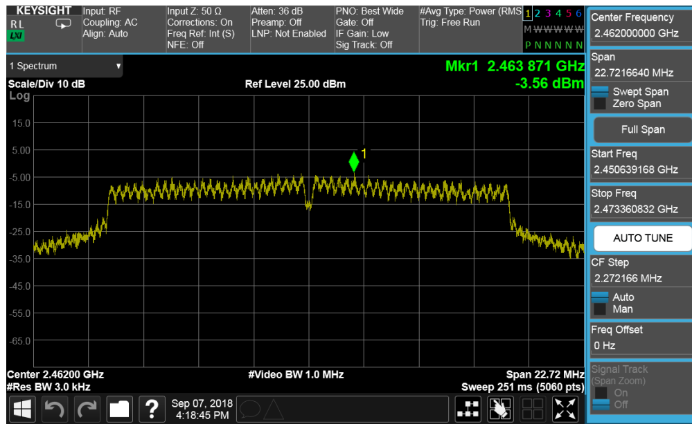
Plot 7-51. Power Spectral Density Plot SISO CORE1 DIVERSITY (802.11g – Ch. 11)
