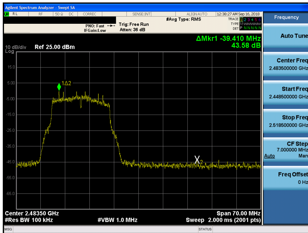
Plot 7-85. Band Edge Plot SISO CORE0 (802.11g - Ch. 12)
