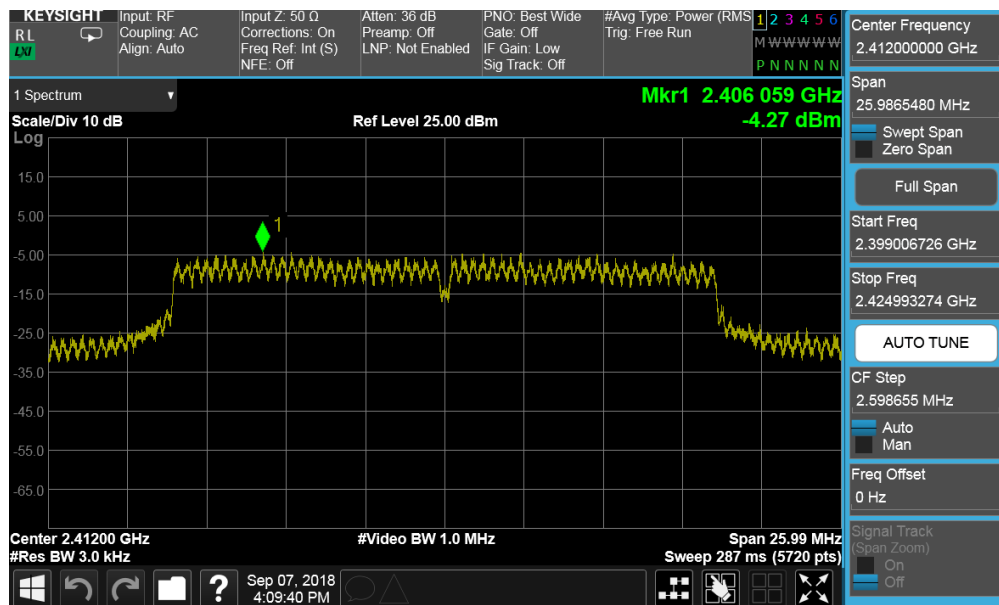
Plot 7-52. Power Spectral Density Plot SISO CORE1 DIVERSITY (802.11n (2.4GHz) – Ch. 1)
