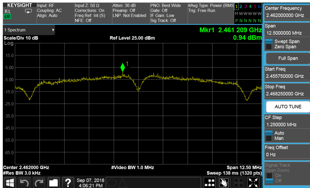
Plot 7-48. Power Spectral Density Plot SISO CORE1 DIVERSITY (802.11b – Ch. 11)
