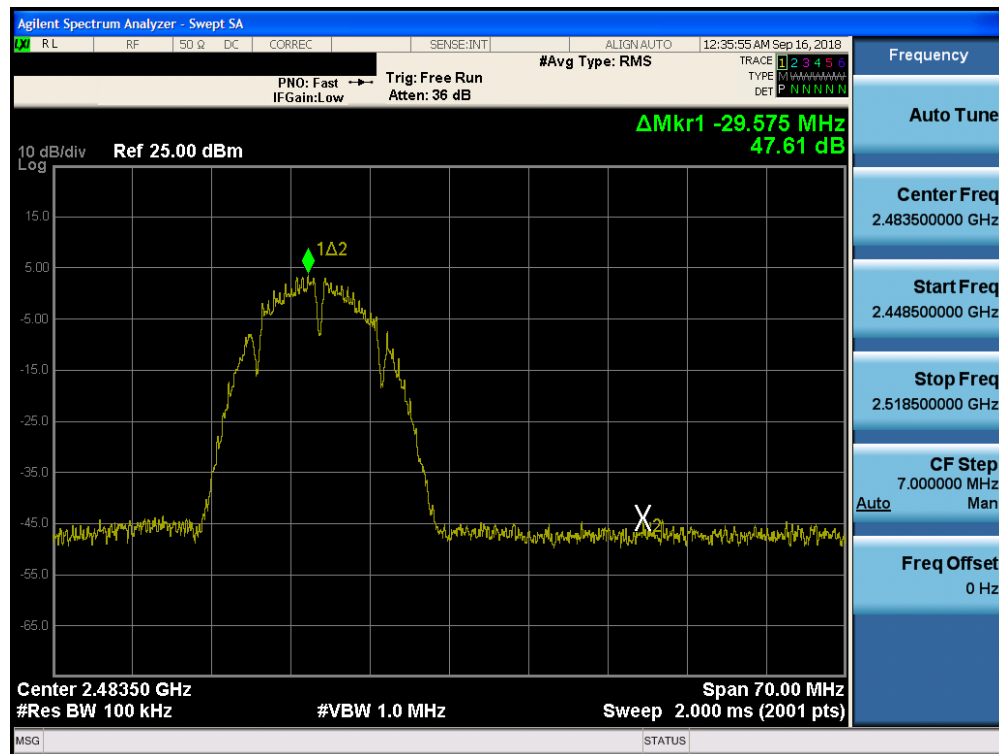
Plot 7-82. Band Edge Plot SISO CORE0 (802.11b - Ch. 13)
