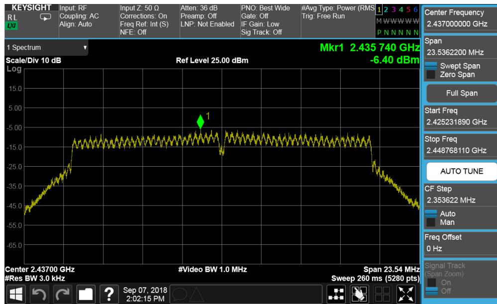
Plot 7-44. Power Spectral Density Plot SISO CORE1 PRIMARY (802.11n (2.4GHz) – Ch. 6)
