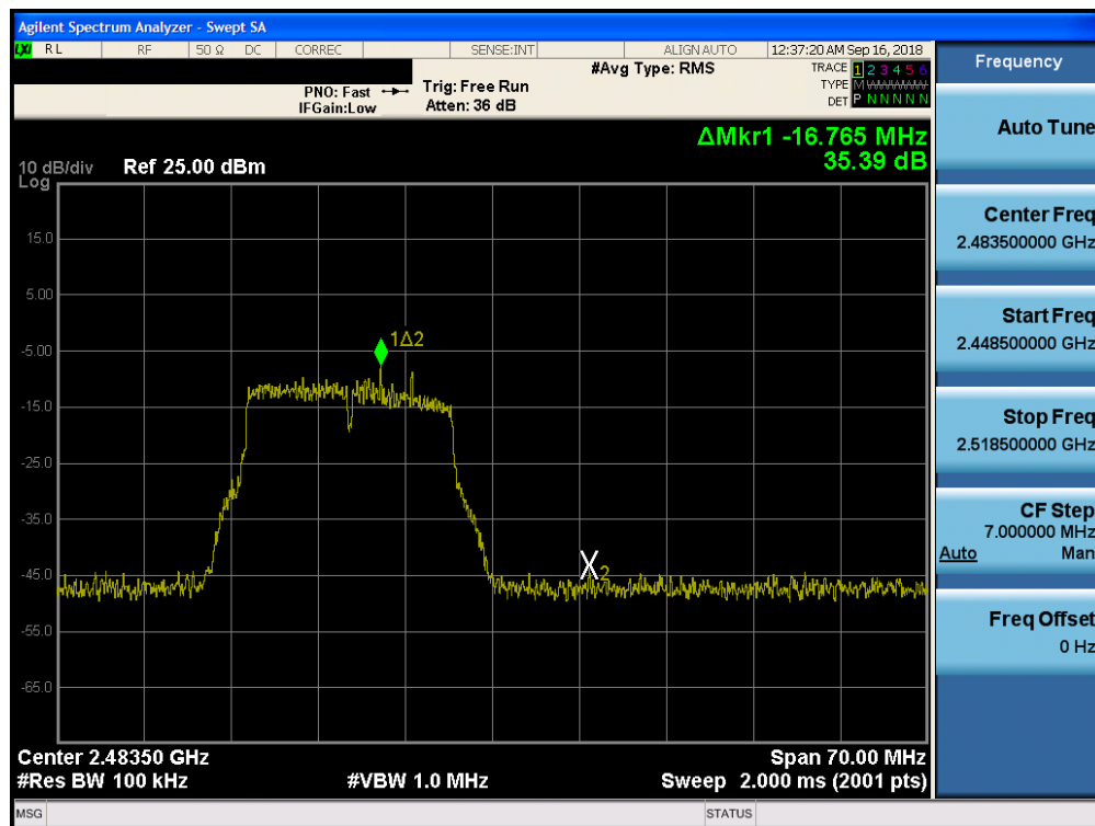
Plot 7-86. Band Edge Plot SISO CORE0 (802.11g - Ch. 13)
