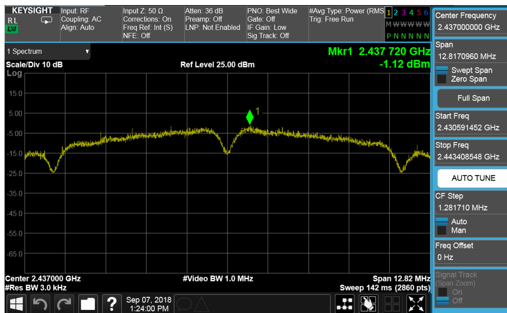
Plot 7-29. Power Spectral Density Plot SISO CORE0 (802.11b – Ch. 6)
