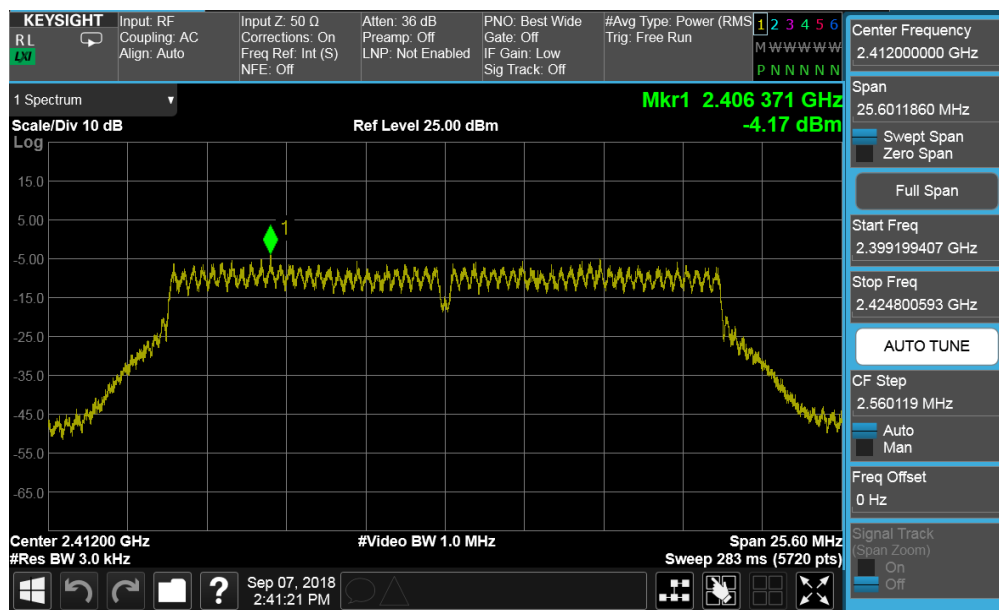
Plot 7-34. Power Spectral Density Plot SISO CORE0 (802.11n (2.4GHz) – Ch. 1)
