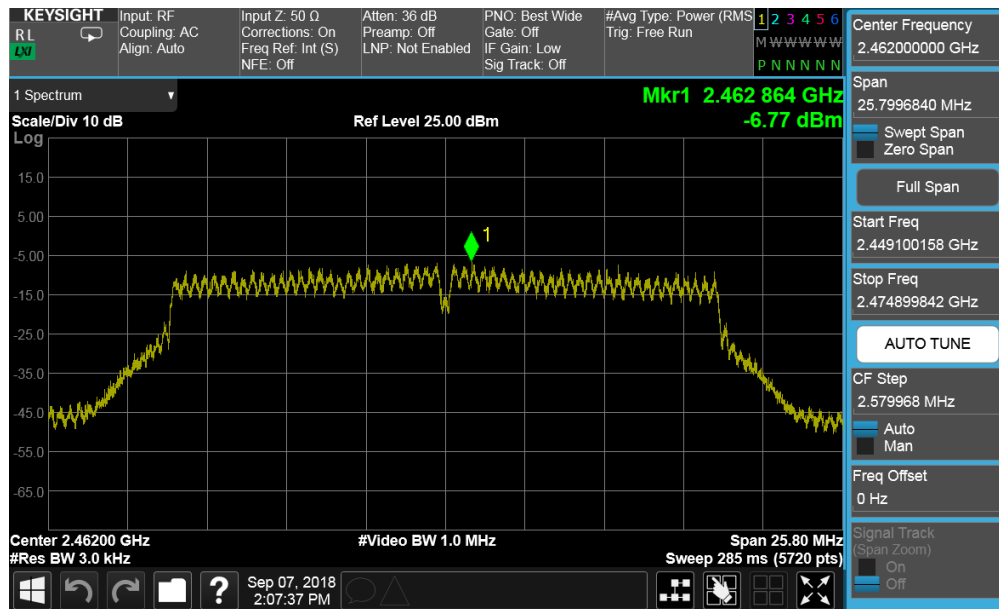
Plot 7-45. Power Spectral Density Plot SISO CORE1 PRIMARY (802.11n (2.4GHz) – Ch. 11)
