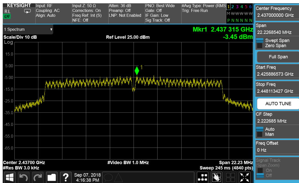
Plot 7-50. Power Spectral Density Plot SISO CORE1 DIVERSITY (802.11g – Ch. 6)
