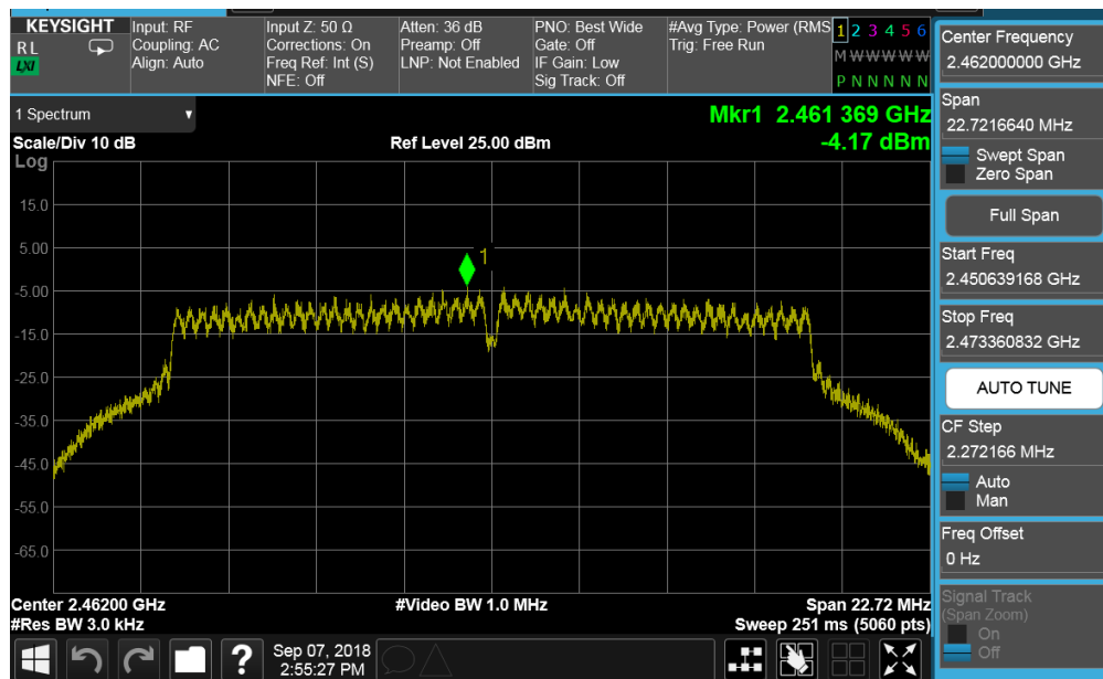
Plot 7-33. Power Spectral Density Plot SISO CORE0 (802.11g – Ch. 11)
