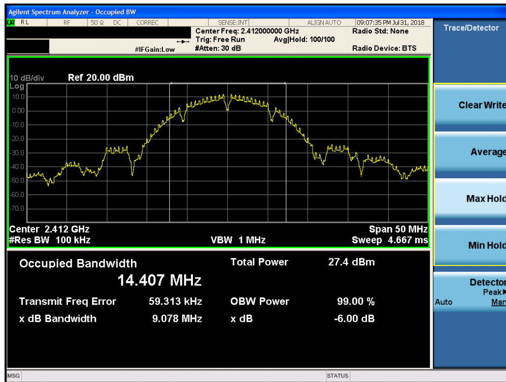
Plot 7-10. 6dB Bandwidth Plot SISO CORE1 PRIMARY (802.11b – Ch. 1)
