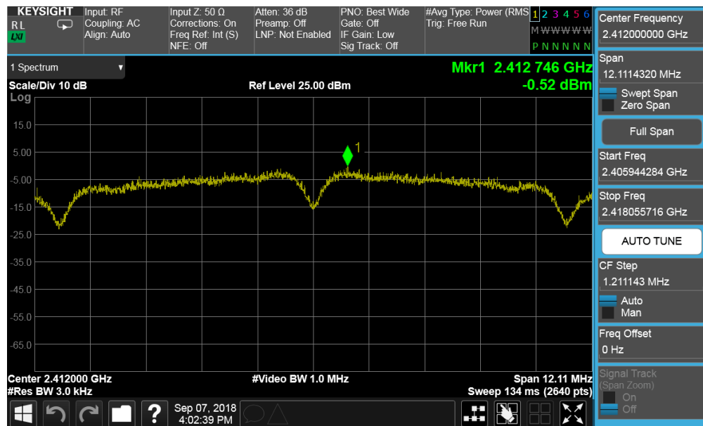
Plot 7-46. Power Spectral Density Plot SISO CORE1 DIVERSITY (802.11b – Ch. 1)
