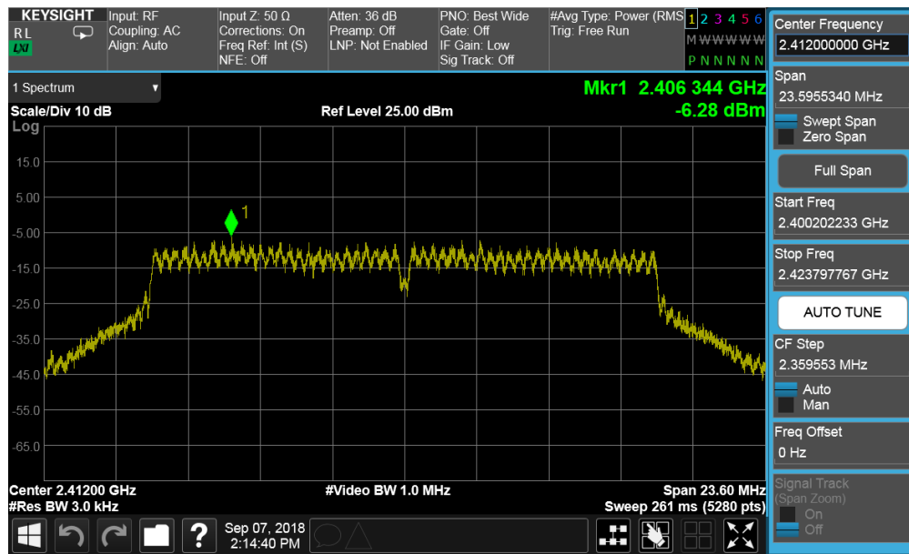
Plot 7-40. Power Spectral Density Plot SISO CORE1 PRIMARY (802.11g – Ch. 1)
