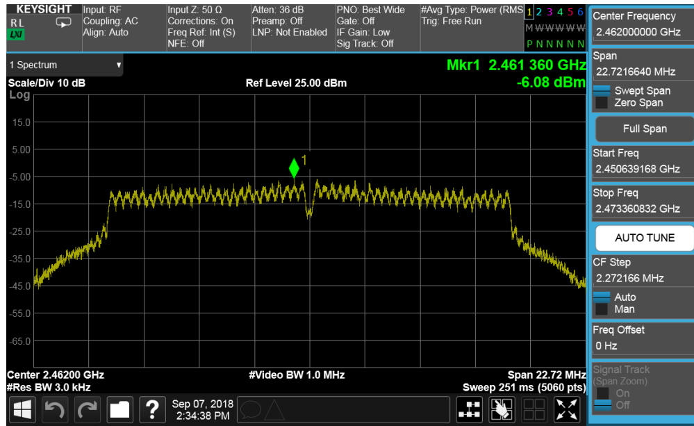
Plot 7-42. Power Spectral Density Plot SISO CORE1 PRIMARY (802.11g – Ch. 11)
