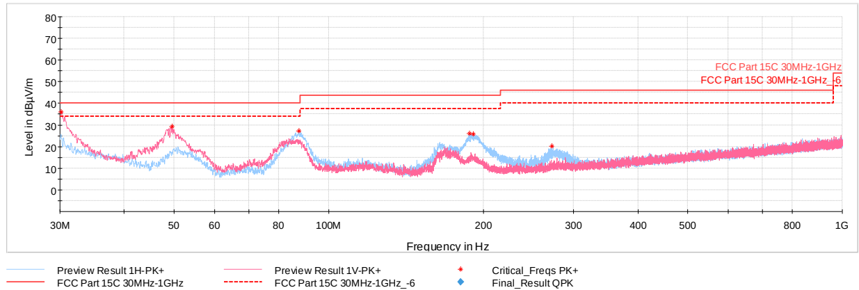
Plot 7-183. Radiated Spurious Plot below 1GHz CDD Primary
