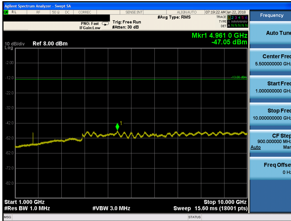
Plot 7-36. Conducted Spurious Plot (Cellular CDMA Mode - High Channel)
