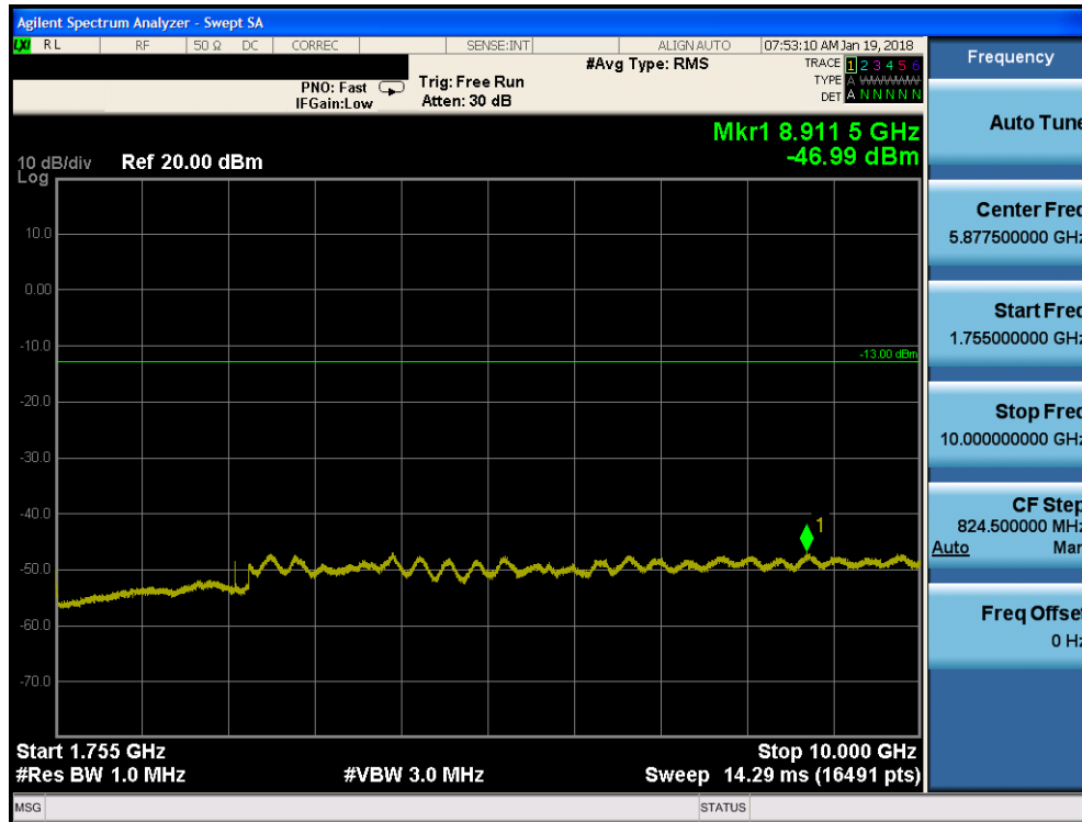
Plot 7-59. Conducted Spurious Plot (AWS WCDMA Mode - Mid Channel)
