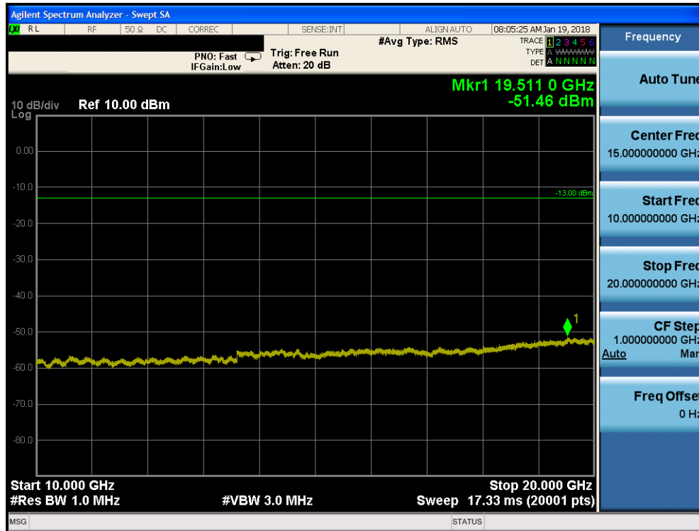
Plot 7-63. Conducted Spurious Plot (AWS WCDMA Mode - High Channel)
