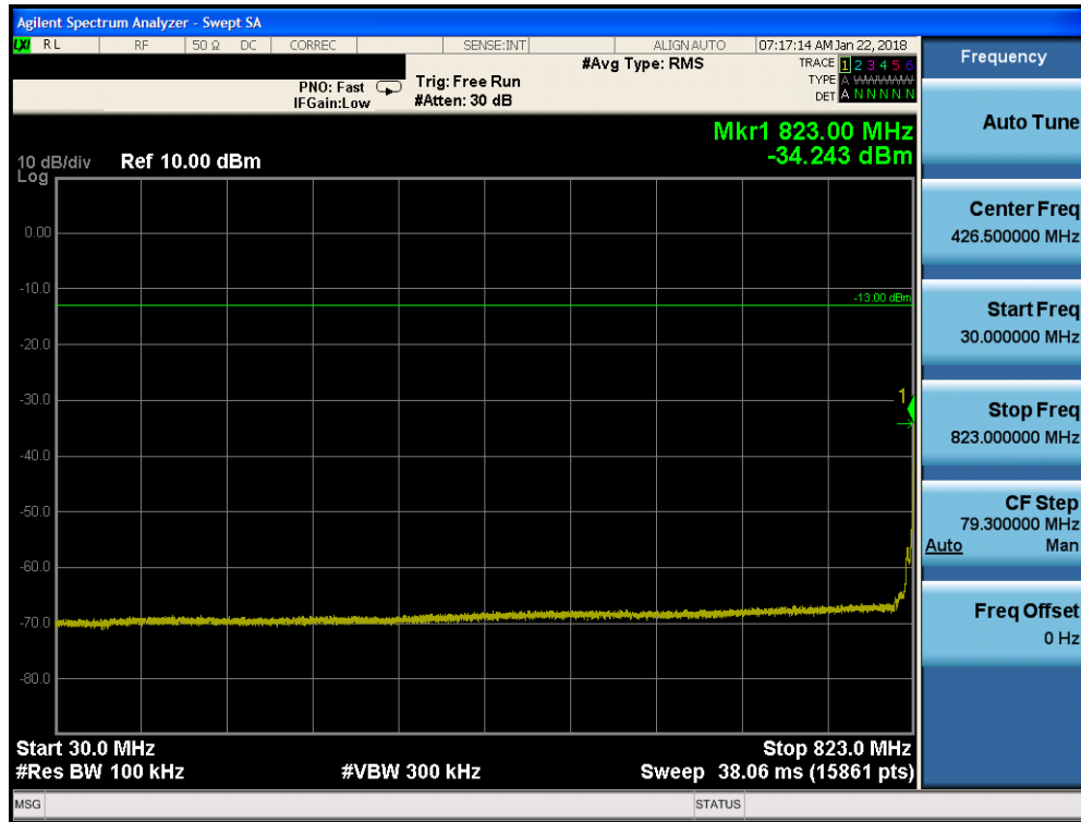
Plot 7-28. Conducted Spurious Plot (Cellular CDMA Mode - Low Channel)
