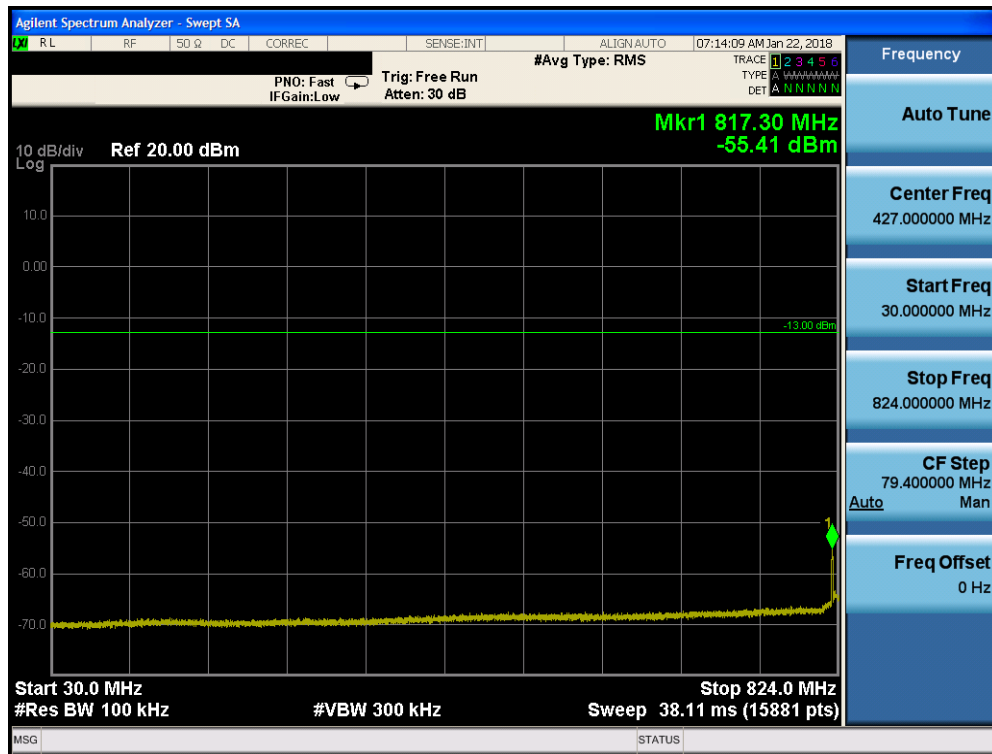
Plot 7-31. Conducted Spurious Plot (Cellular CDMA Mode - Mid Channel)
