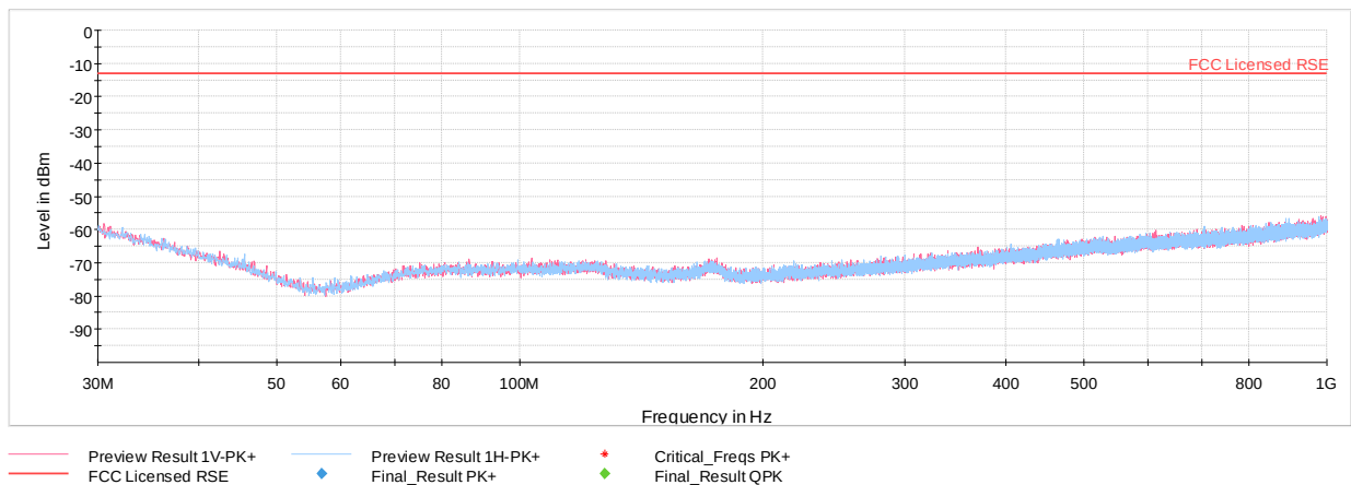
Plot 7-32. Radiated Spurious Plot (WCDMA 1900)
