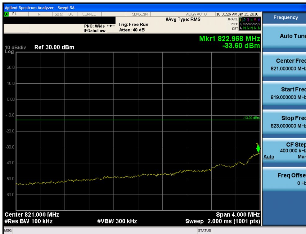
Plot 7-80. 4MHz Span Plot (Cellular CDMA Mode - Low Channel)
