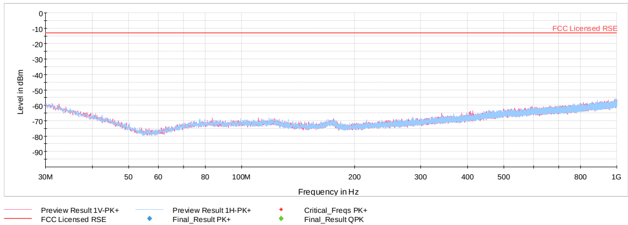
Plot 7-31. Radiated Spurious Plot (CDMA 1900)
