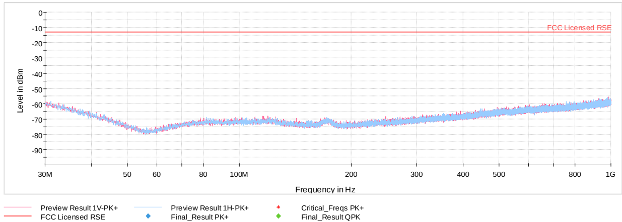
Plot 7-30. Radiated Spurious Plot (GPRS 1900)
