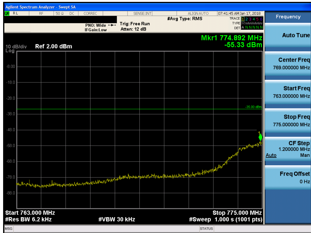
Plot 7-201. Lower Emission Mask Edge Plot (Band 13 - 5.0MHz QPSK - Full RB Configuration)
