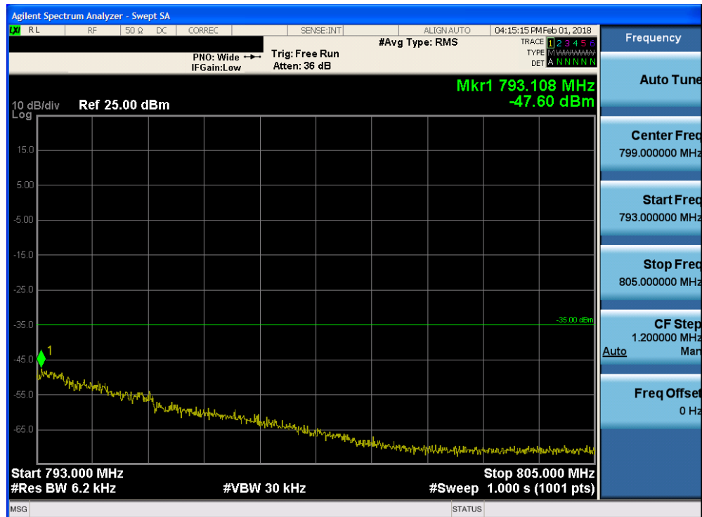
Plot 7-207. Upper Emission Mask Edge Plot (Band 13 - 10.0MHz QPSK - Full RB Configuration)
