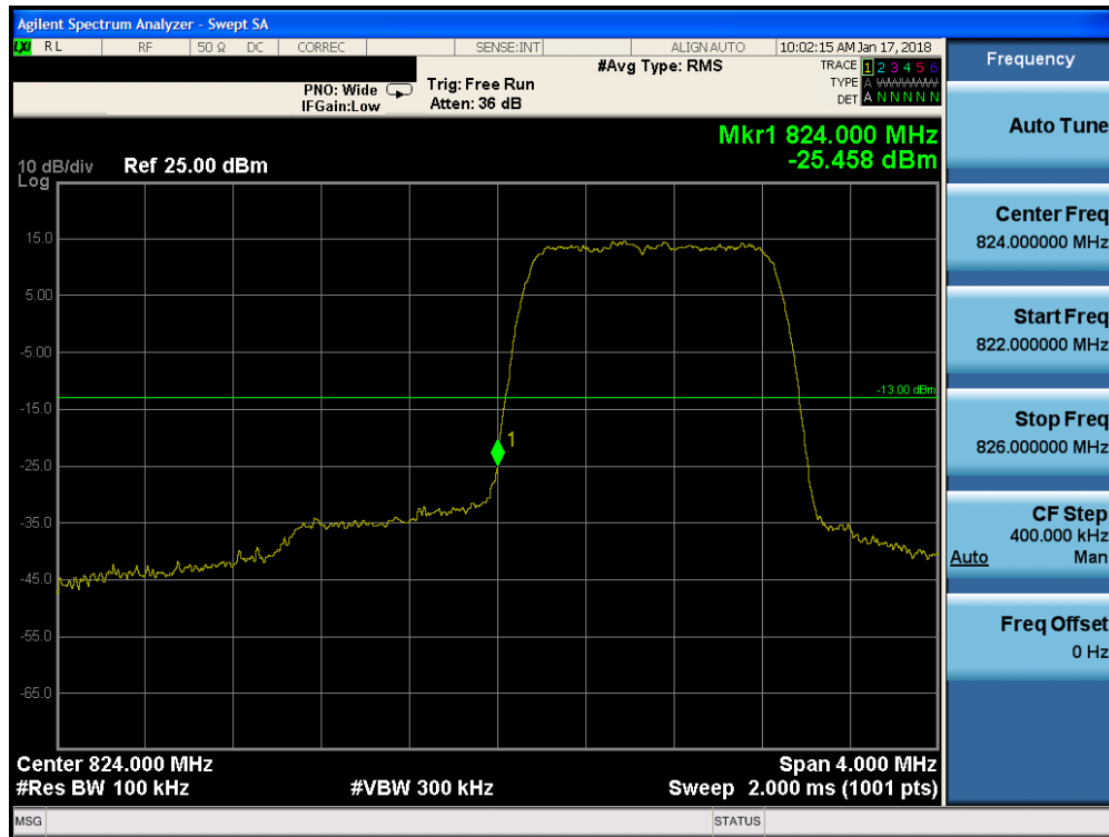
Plot 7-208. Lower Band Edge Plot (Band 26 - 1.4MHz QPSK - Full RB Configuration)
