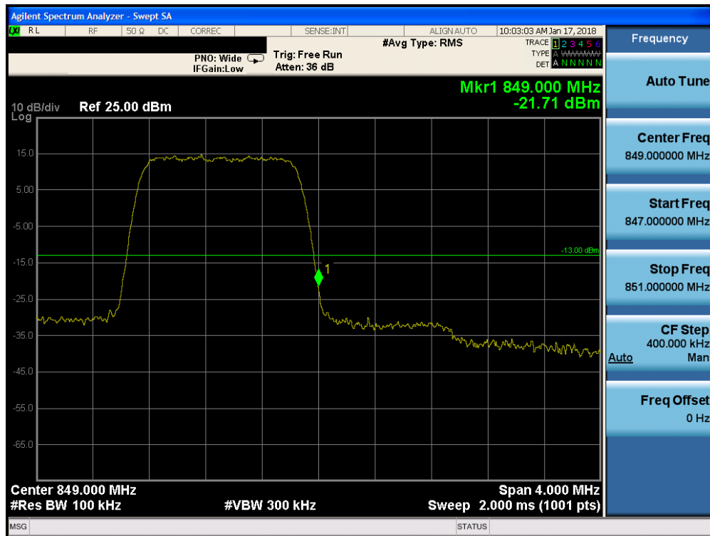
Plot 7-209. Upper Band Edge Plot (Band 26 - 1.4MHz QPSK - Full RB Configuration)
