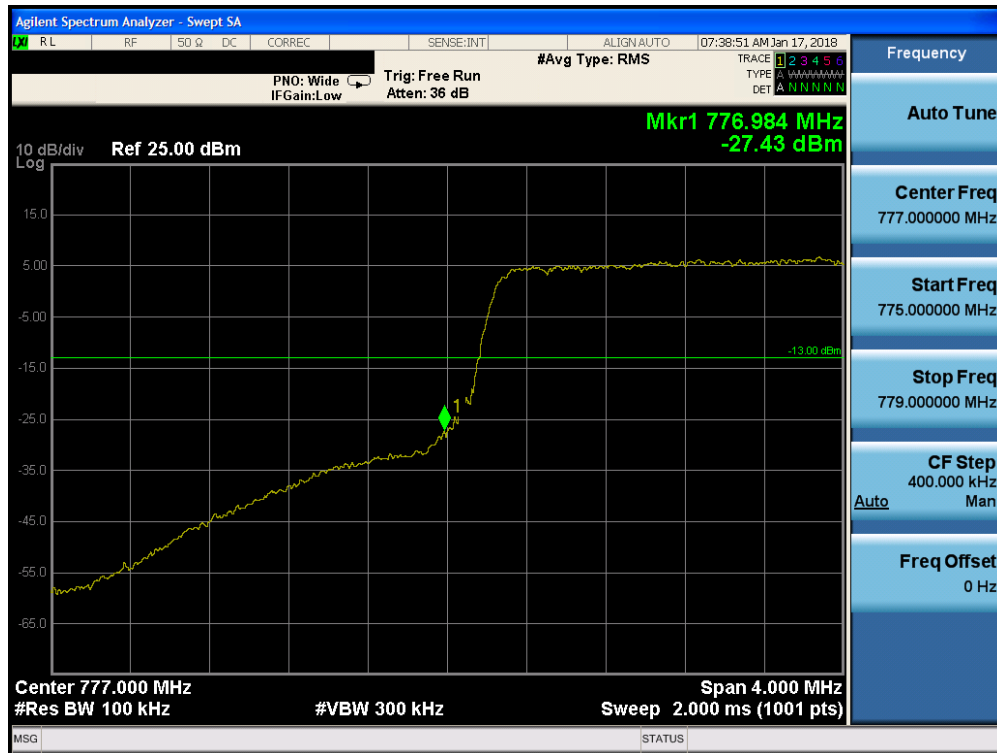
Plot 7-200. Lower Band Edge Plot (Band 13 - 5.0MHz QPSK - Full RB Configuration)
