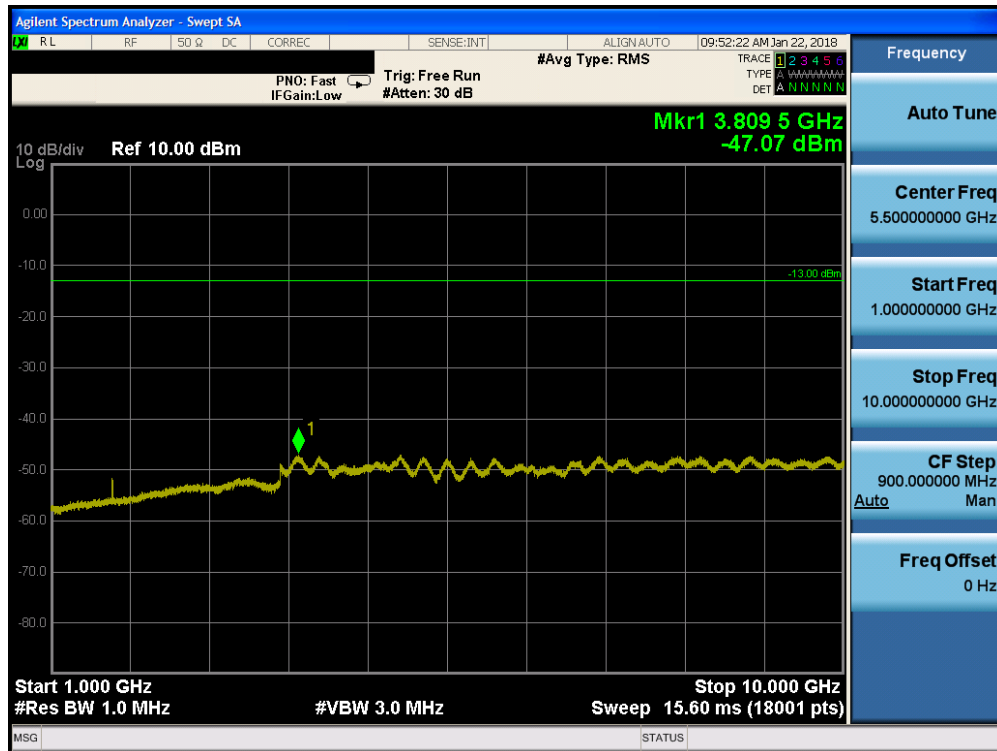
Plot 7-124. Conducted Spurious Plot (Band 26 - 3.0MHz QPSK - RB Size 1, RB Offset 0 - High Channel)
