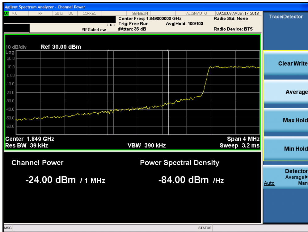
Plot 7-249. Lower Extended Band Edge Plot (Band 25 - 1.4MHz QPSK - Full RB Configuration)
