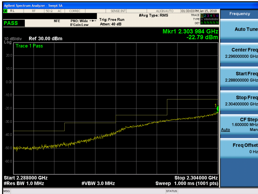
Plot 7-301. Lower Extended Band Edge Plot (Band 30 - 10.0MHz QPSK - Full RB Configuration)
