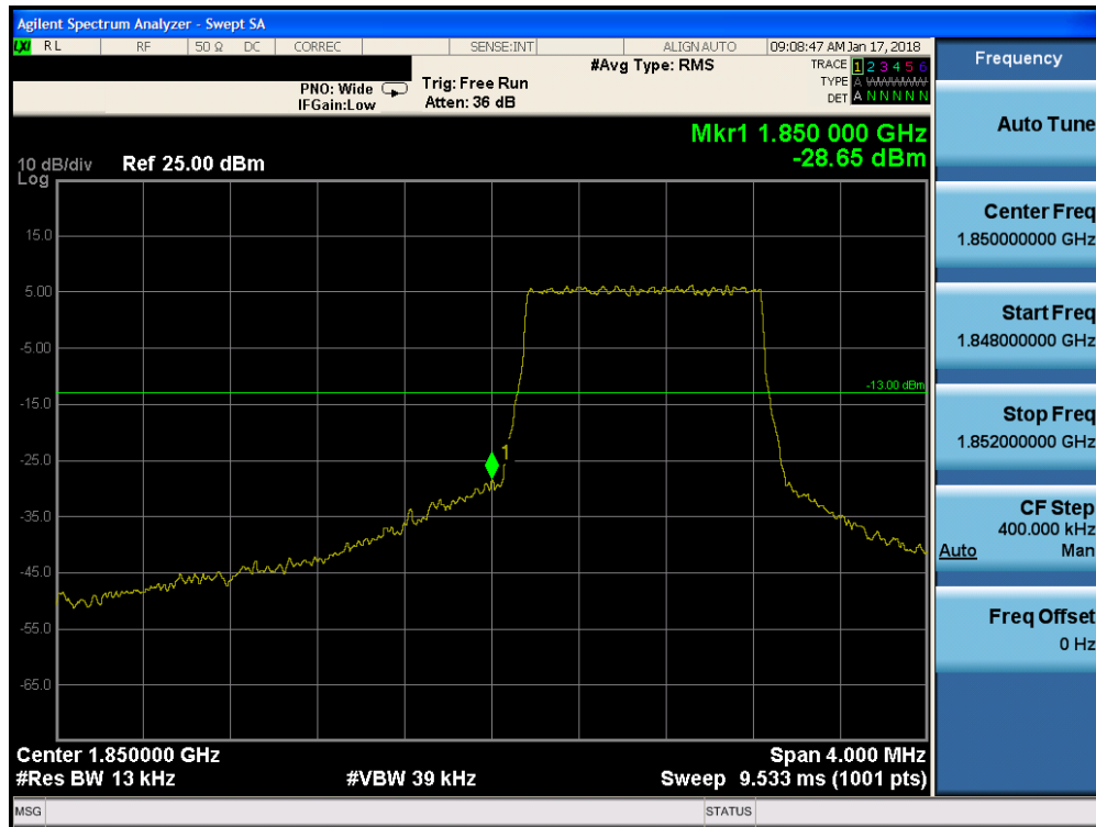
Plot 7-248. Lower Band Edge Plot (Band 25 - 1.4MHz QPSK - Full RB Configuration)
