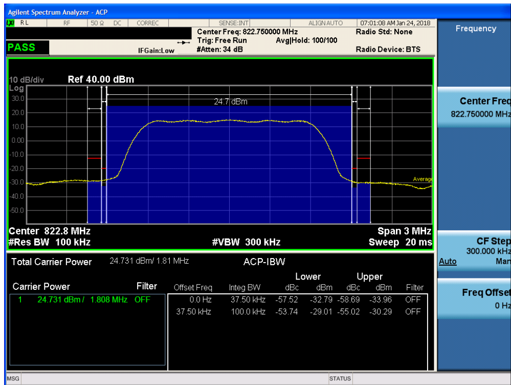
Plot 7-20. Channel Edge Plot (Ch. 670)
