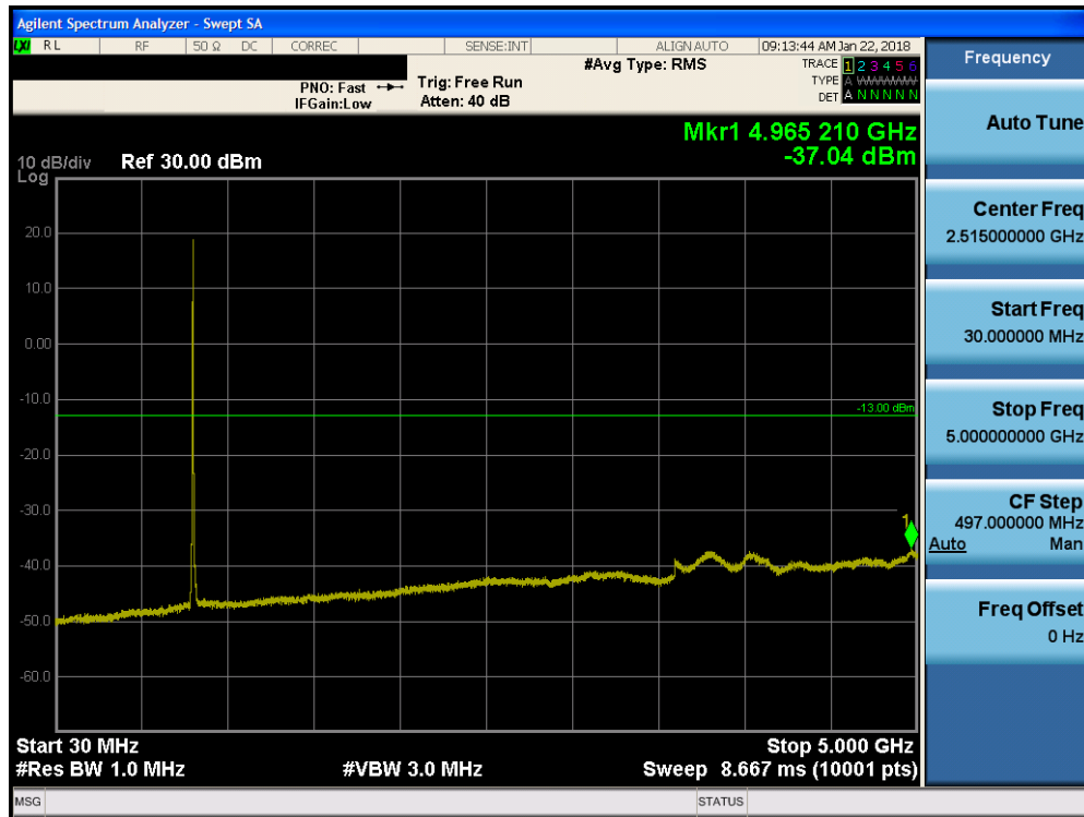
Plot 7-17. Conducted Spurious Plot (3MHz QPSK – RB Size 1, RB Offset 0 – High Channel)
