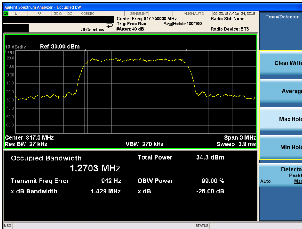
Plot 7-1. Occupied Bandwidth Plot (Ch. 450)
