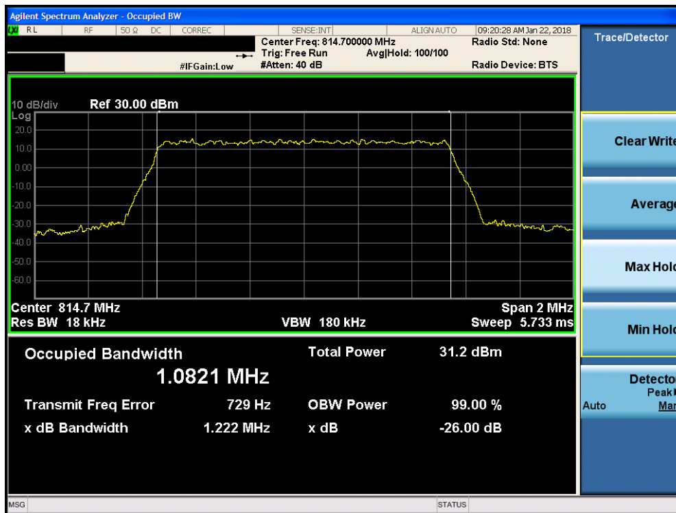
Plot 7-3. Occupied Bandwidth Plot (1.4MHz QPSK – RB Size 6– Low Channel)
