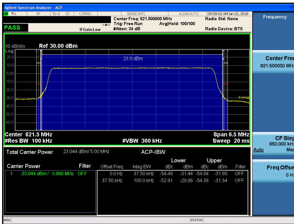
Plot 7-26. Channel Edge Plot (5MHz QPSK – RB Size 25 – High Channel)
