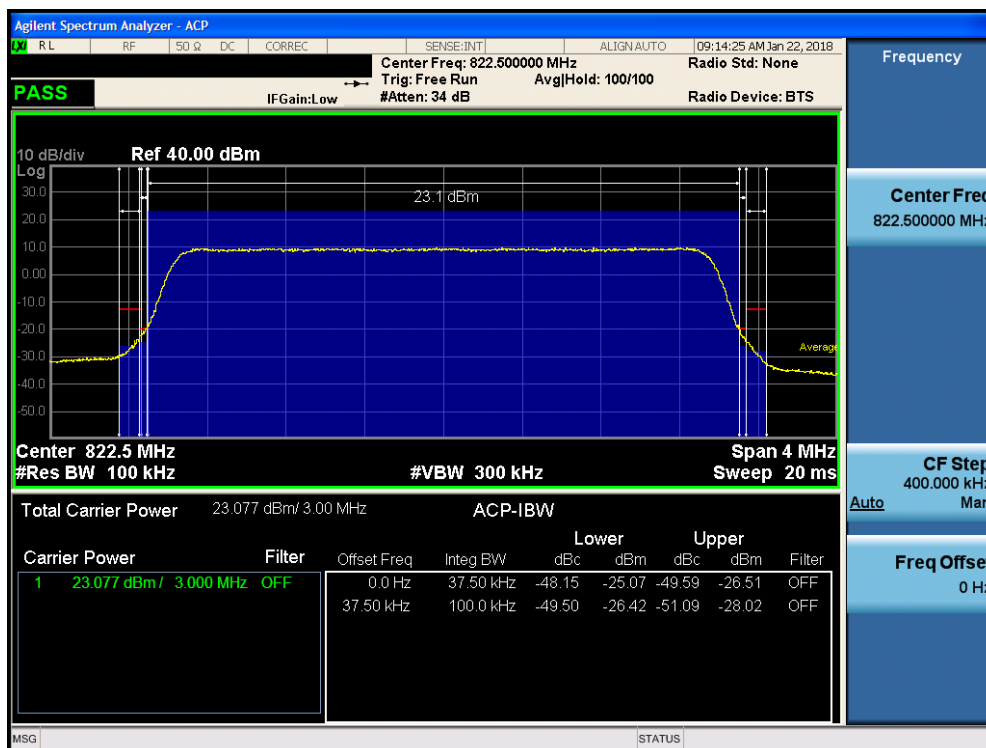
Plot 7-24. Channel Edge Plot (3MHz QPSK – RB Size 15 – High Channel)
