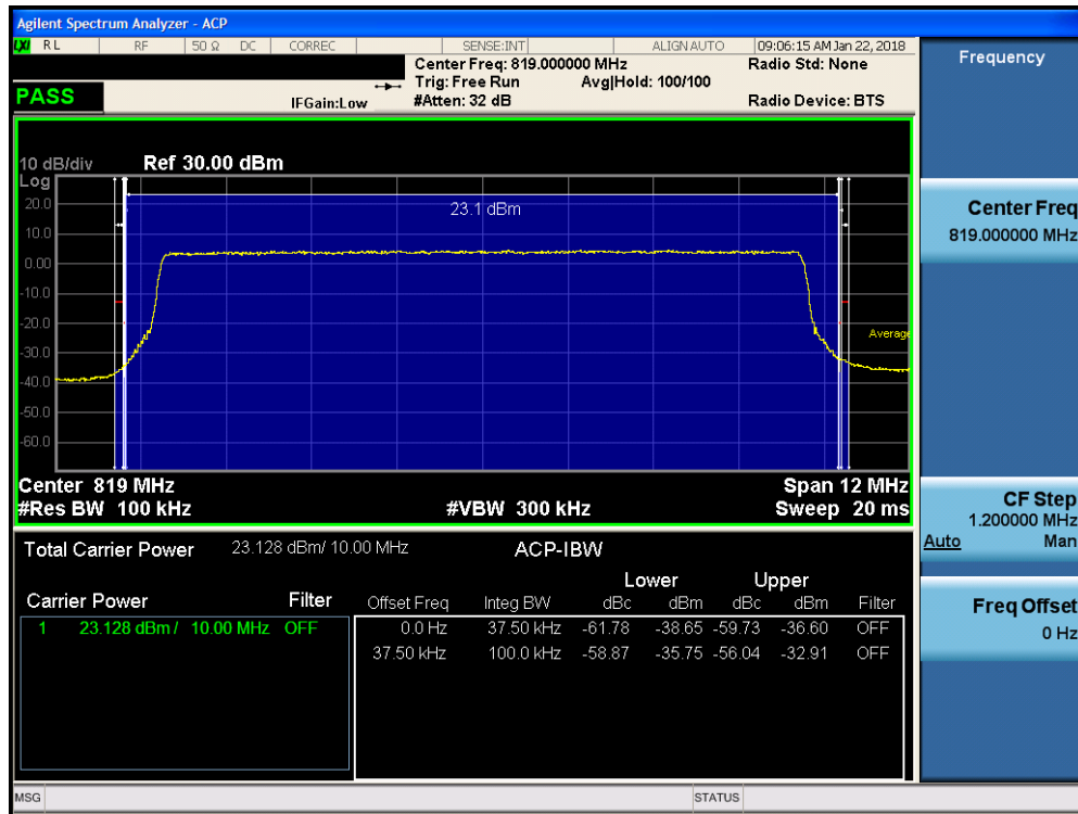
Plot 7-27. Channel Edge Plot (10MHz QPSK – RB Size 50)
