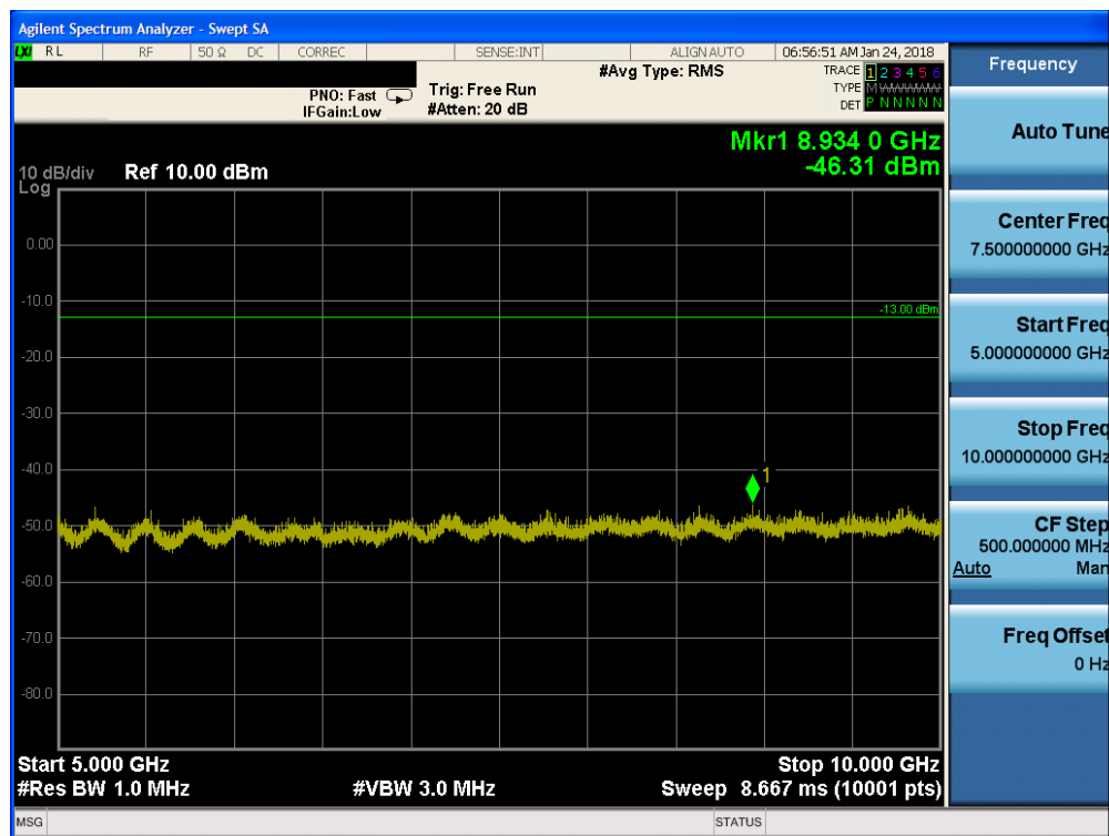
Plot 7-12. Conducted Spurious Plot (Ch. 450)
