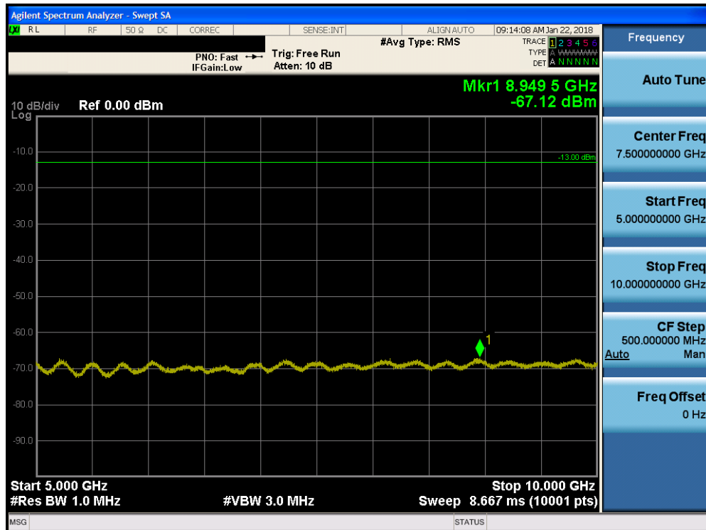
Plot 7-18. Conducted Spurious Plot (3MHz QPSK – RB Size 1, RB Offset 0 – High Channel)
