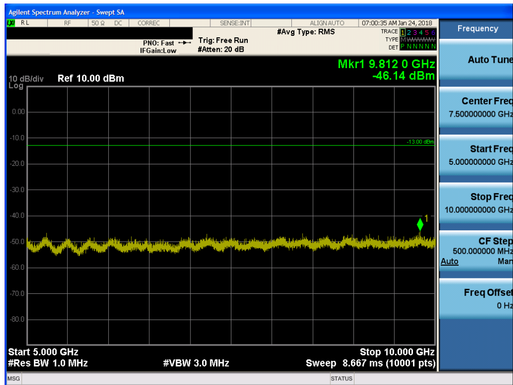
Plot 7-14. Conducted Spurious Plot (Ch. 670)
