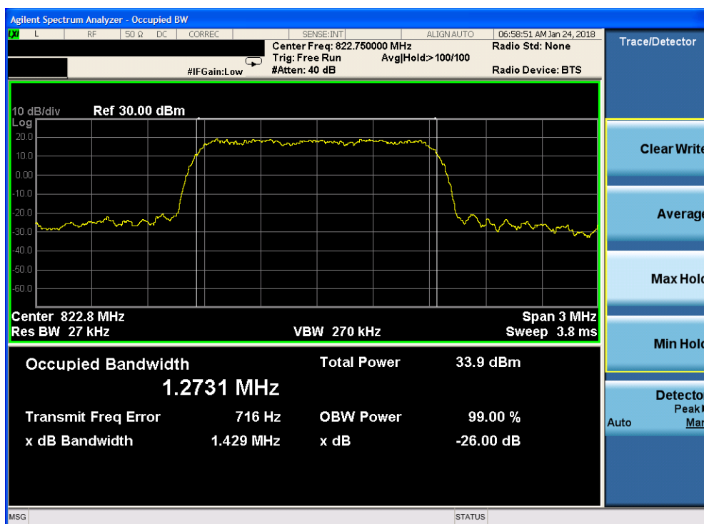
Plot 7-2. Occupied Bandwidth Plot (Ch. 670)
