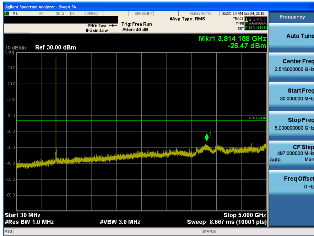
Plot 7-11. Conducted Spurious Plot (Ch. 450)
