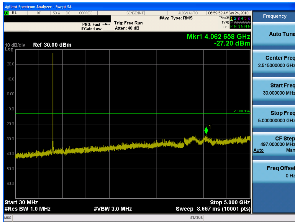
Plot 7-13. Conducted Spurious Plot (Ch. 670)
