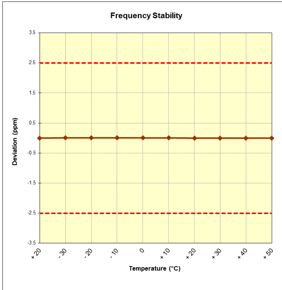
Figure 7-6. CDMA BC10 Frequency Stability Graph (Ch. 450)
