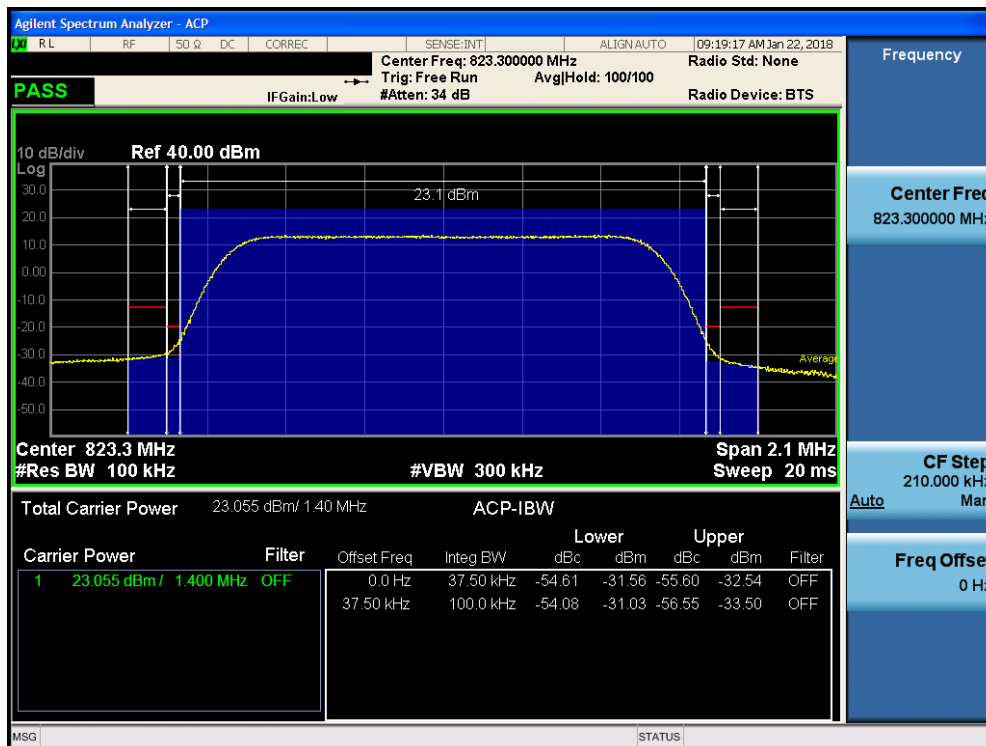
Plot 7-22. Channel Edge Plot (1.4MHz QPSK – RB Size 6 – High Channel)
