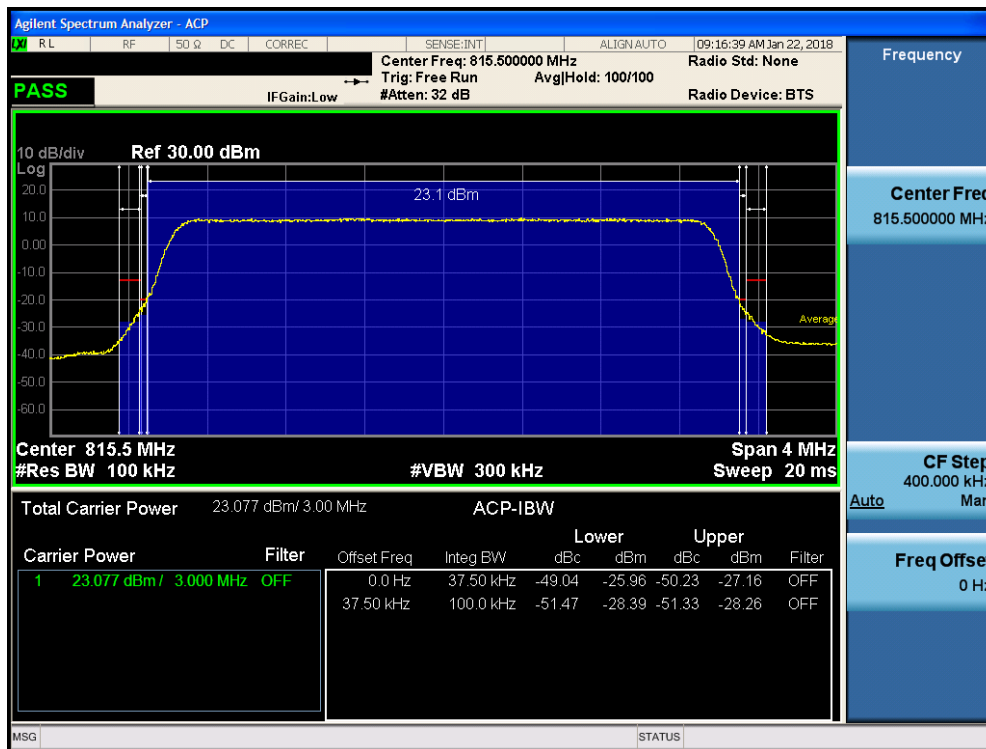
Plot 7-23. Channel Edge Plot (3MHz QPSK – RB Size 15– Low Channel)
