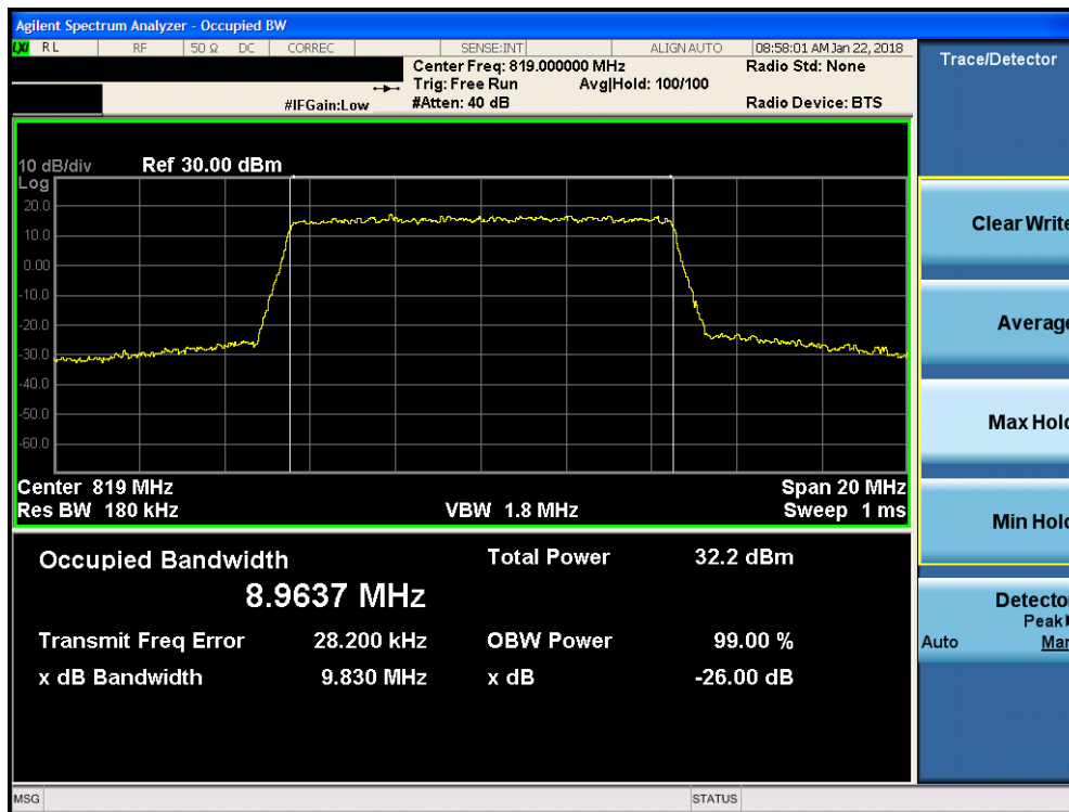
Plot 7-9. Occupied Bandwidth Plot (10MHz QPSK – RB Size 50)
