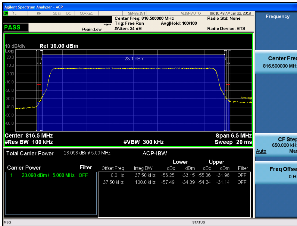
Plot 7-25. Channel Edge Plot (5MHz QPSK – RB Size 25– Low Channel)
