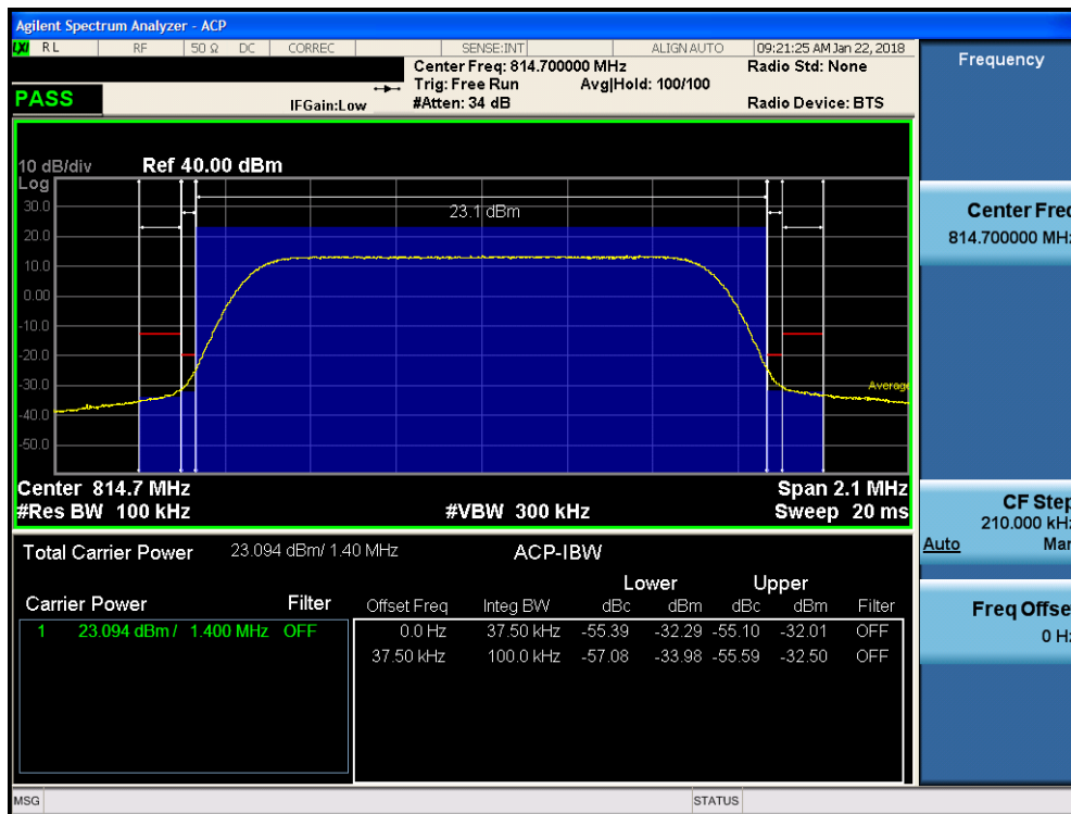
Plot 7-21. Channel Edge Plot (1.4MHz QPSK – RB Size 6– Low Channel)
