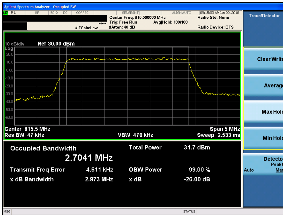
Plot 7-5. Occupied Bandwidth Plot (3MHz QPSK – RB Size 15– Low Channel)
