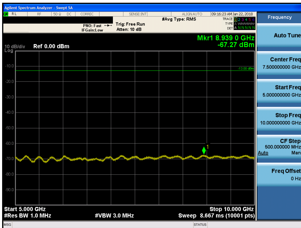
Plot 7-16. Conducted Spurious Plot (3MHz QPSK – RB Size 1, RB Offset 0 – Low Channel)
