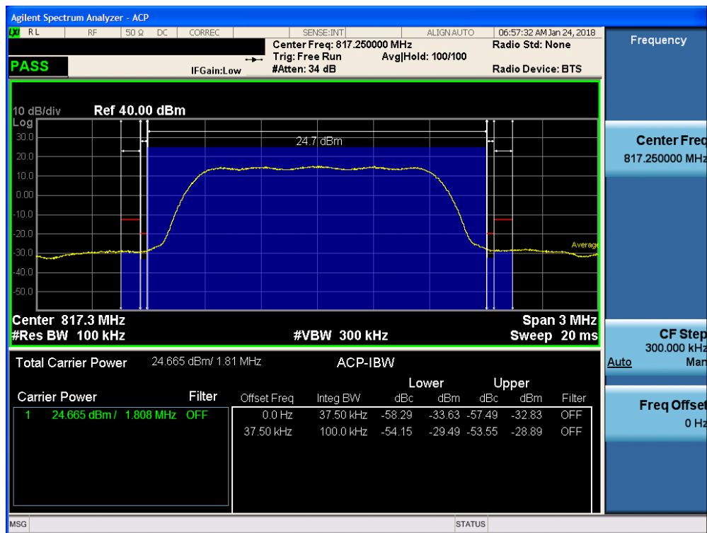
Plot 7-19. Channel Edge Plot (Ch. 450)
