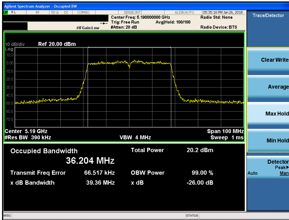
Plot 7-67. 26dB Bandwidth Plot MIMO ANT1 (40MHz BW 802.11n (UNII Band 1) – Ch. 38)
