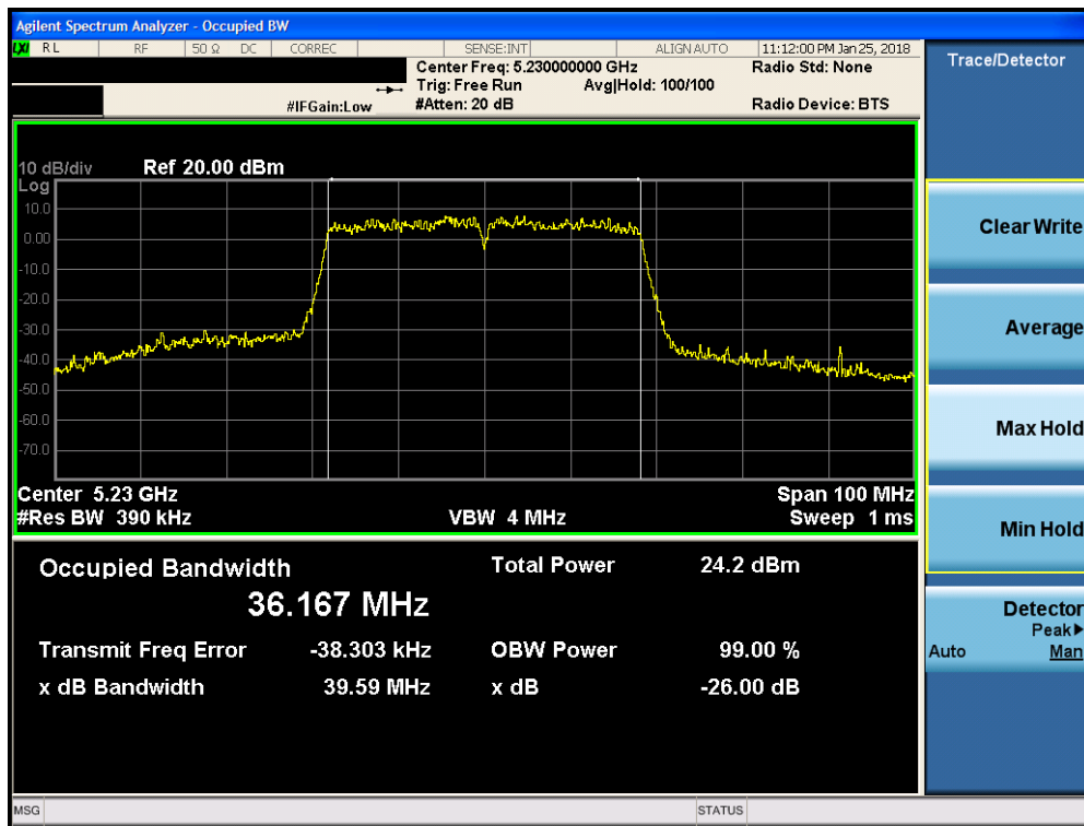
Plot 7-70. 26dB Bandwidth Plot MIMO ANT2 (40MHz BW 802.11n (UNII Band 1) – Ch. 46)
