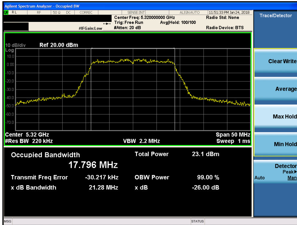
Plot 7-15. 26dB Bandwidth Plot FCC SISO ANT1 (20MHz BW 802.11n (UNII Band 2A) – Ch. 64)
