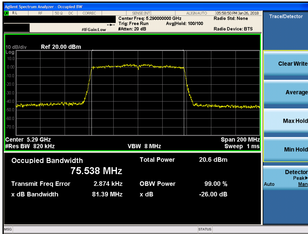
Plot 7-83. 26dB Bandwidth Plot MIMO ANT1 (80MHz BW 802.11ac (UNII Band 2A) – Ch. 58)
