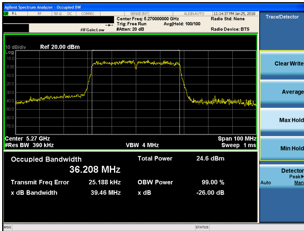
Plot 7-80. 26dB Bandwidth Plot MIMO ANT2 (40MHz BW 802.11n (UNII Band 2A) – Ch. 54)
