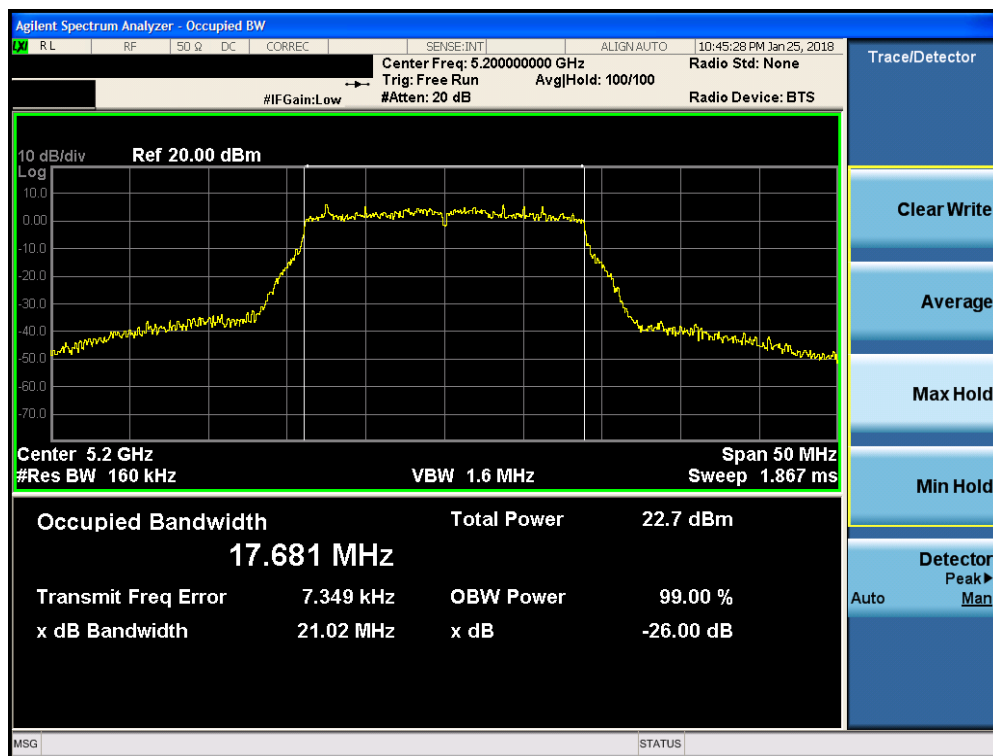
Plot 7-64. 26dB Bandwidth Plot MIMO ANT2 (20MHz BW 802.11n (UNII Band 1) – Ch. 40)
