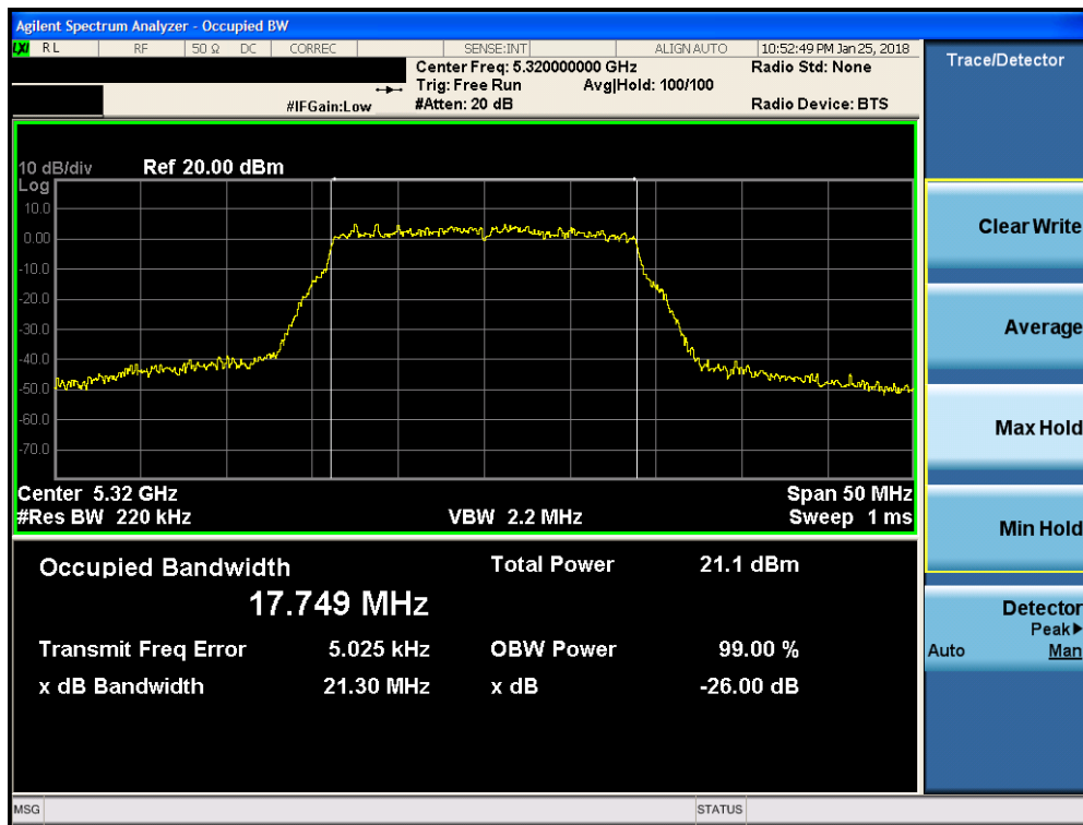
Plot 7-78. 26dB Bandwidth Plot MIMO ANT2 (20MHz BW 802.11n (UNII Band 2A) – Ch. 64)
