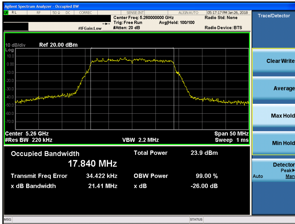
Plot 7-73. 26dB Bandwidth Plot MIMO ANT1 (20MHz BW 802.11n (UNII Band 2A) – Ch. 52)
