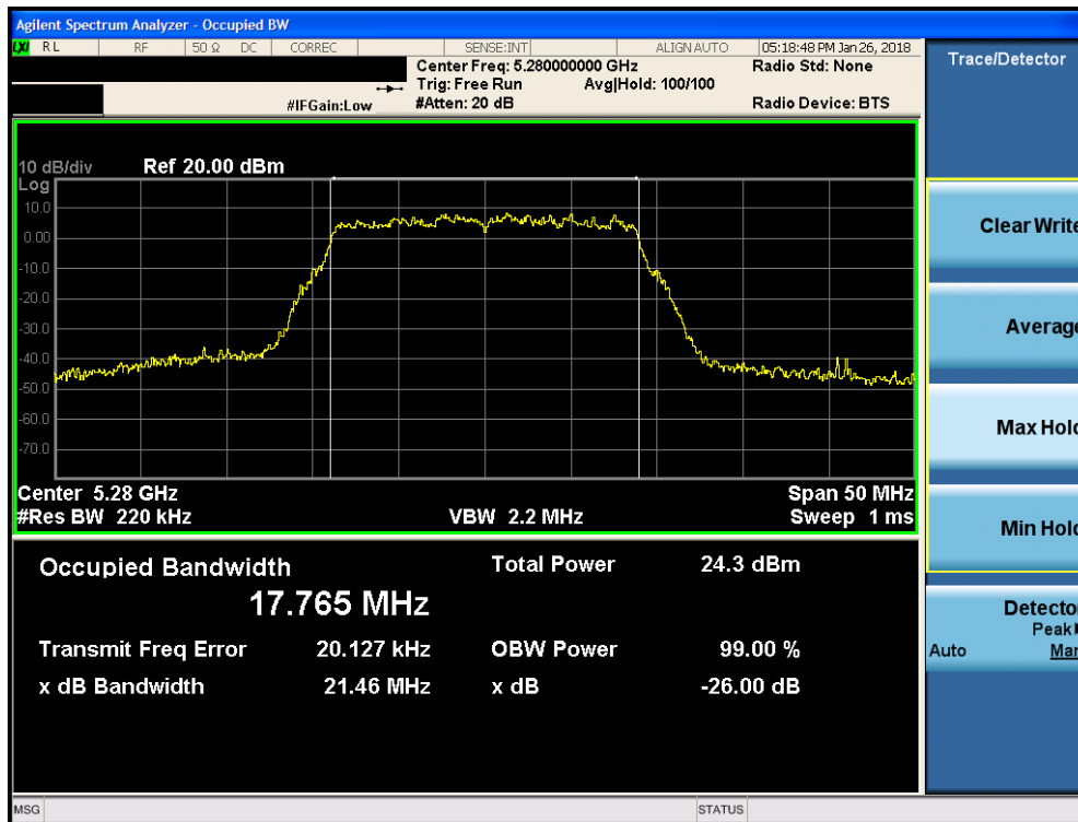
Plot 7-75. 26dB Bandwidth Plot MIMO ANT1 (20MHz BW 802.11n (UNII Band 2A) – Ch. 56)
