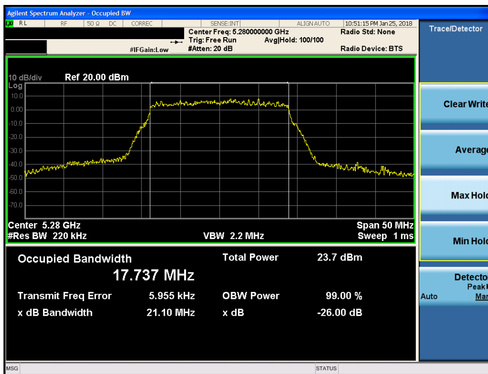
Plot 7-76. 26dB Bandwidth Plot MIMO ANT2 (20MHz BW 802.11n (UNII Band 2A) – Ch. 56)
