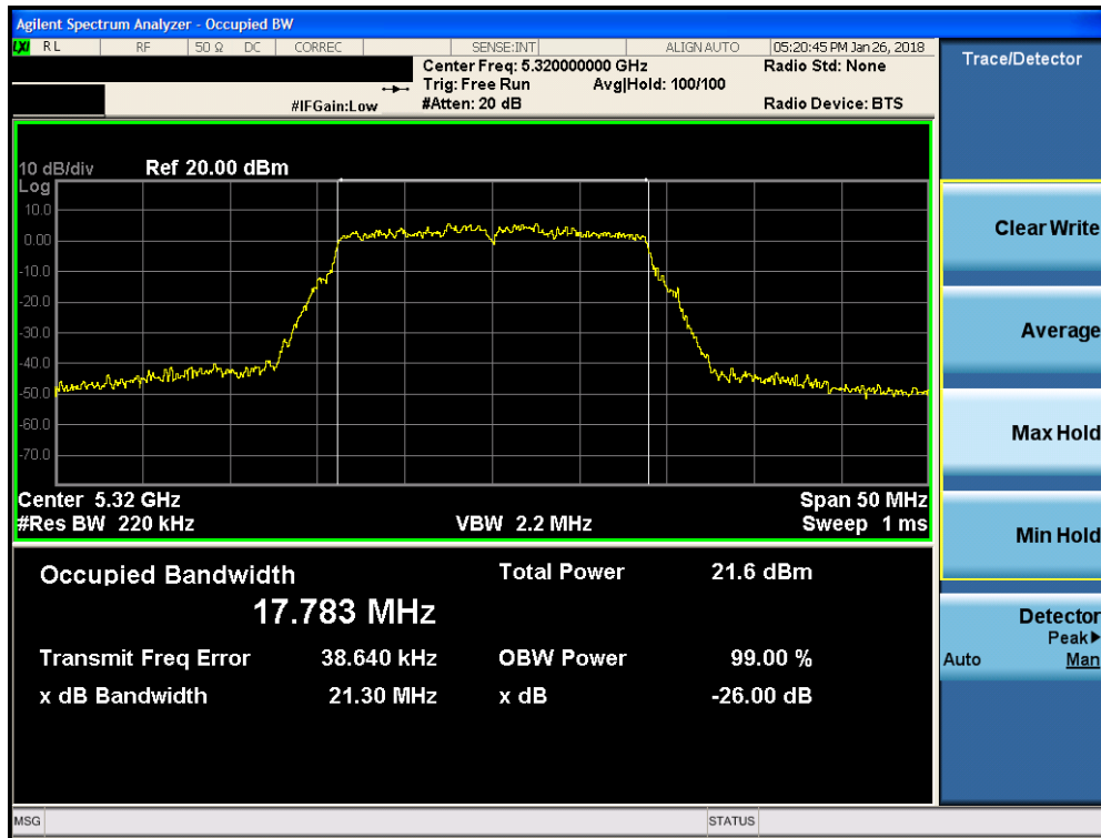
Plot 7-77. 26dB Bandwidth Plot MIMO ANT1 (20MHz BW 802.11n (UNII Band 2A) – Ch. 64)
