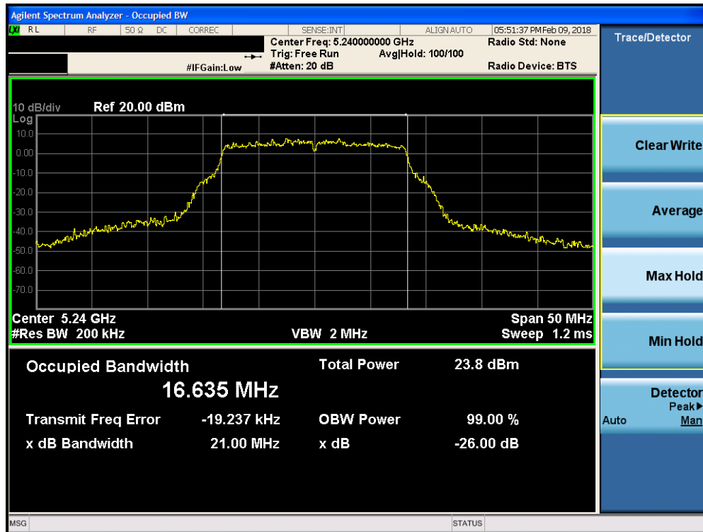
Plot 7-3. 26dB Bandwidth Plot FCC SISO ANT1 (802.11a (UNII Band 1) – Ch. 48)
