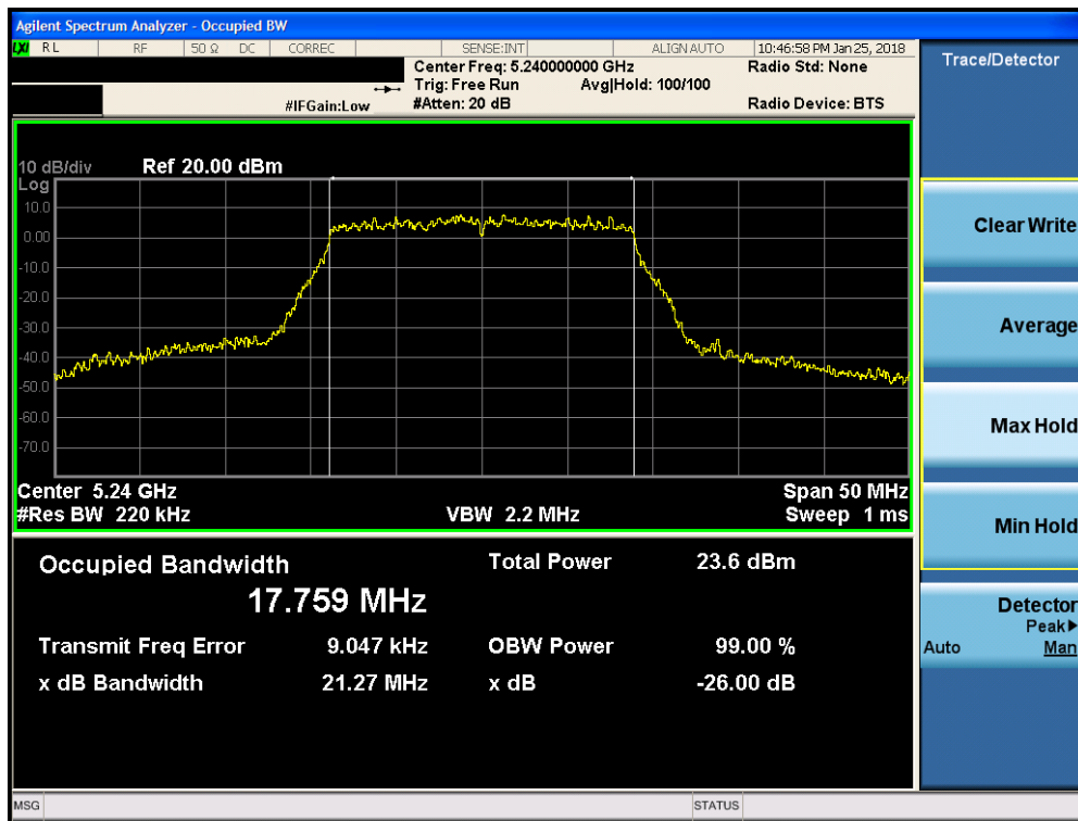
Plot 7-66. 26dB Bandwidth Plot MIMO ANT2 (20MHz BW 802.11n (UNII Band 1) – Ch. 48)
