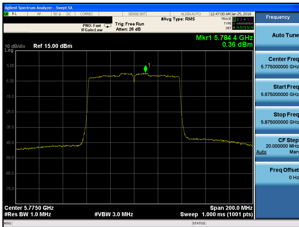
Plot 7-171. Power Spectral Density Plot FCC SISO ANT1 (80MHz BW 802.11ac (UNII Band 3) – Ch. 155)
