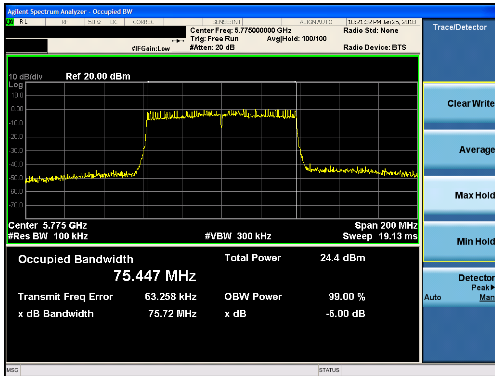
Plot 7-120. 6dB Bandwidth Plot FCC SISO ANT2 (80MHz BW 802.11ac (UNII Band 3) – Ch. 155)
