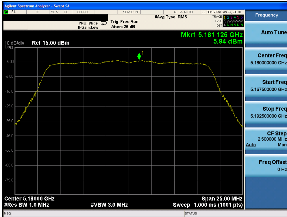
Plot 7-136. Power Spectral Density Plot FCC SISO ANT1 (20MHz BW 802.11n (UNII Band 1) – Ch. 36)
