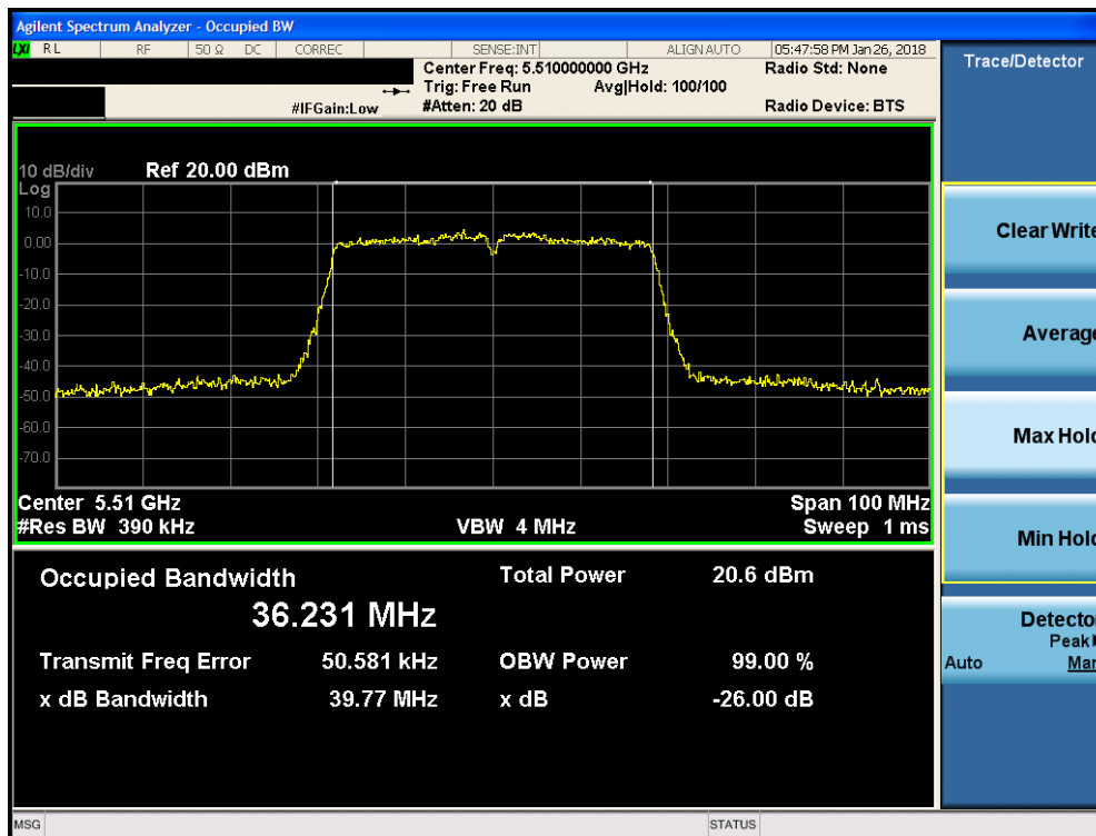
Plot 7-91. 26dB Bandwidth Plot MIMO ANT1 (40MHz BW 802.11n (UNII Band 2C) – Ch. 102)
