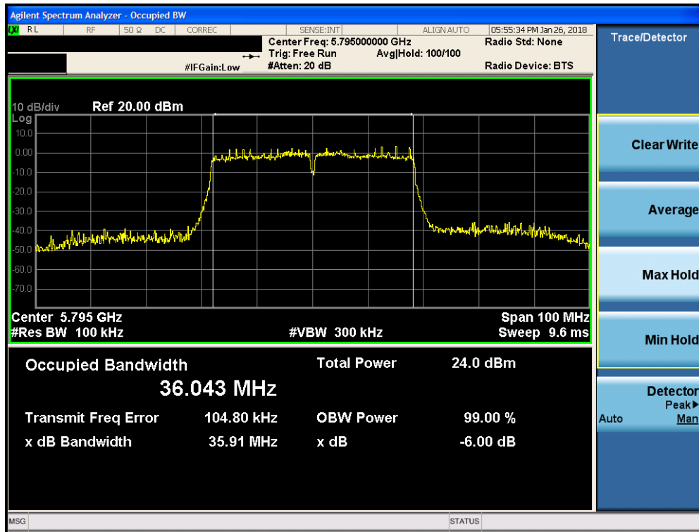
Plot 7-129. 6dB Bandwidth Plot MIMO ANT1 (40MHz BW 802.11n (UNII Band 3) – Ch. 159)
