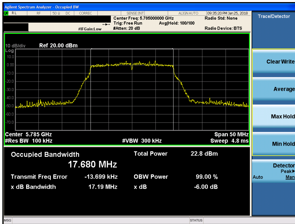
Plot 7-116. 6dB Bandwidth Plot FCC SISO ANT2 (20MHz BW 802.11n (UNII Band 3) – Ch. 157)
