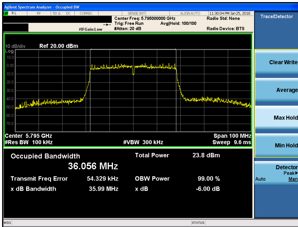
Plot 7-130. 6dB Bandwidth Plot MIMO ANT2 (40MHz BW 802.11n (UNII Band 3) – Ch. 159)
