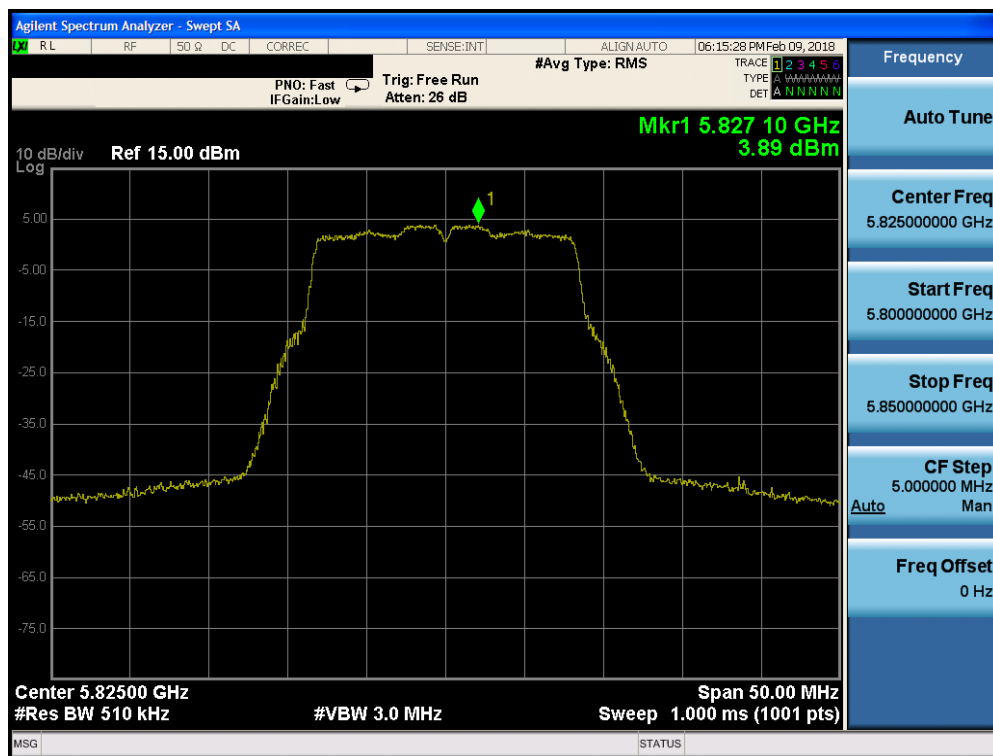
Plot 7-165. Power Spectral Density Plot FCC SISO ANT1 (802.11a (UNII Band 3) – Ch. 165)
