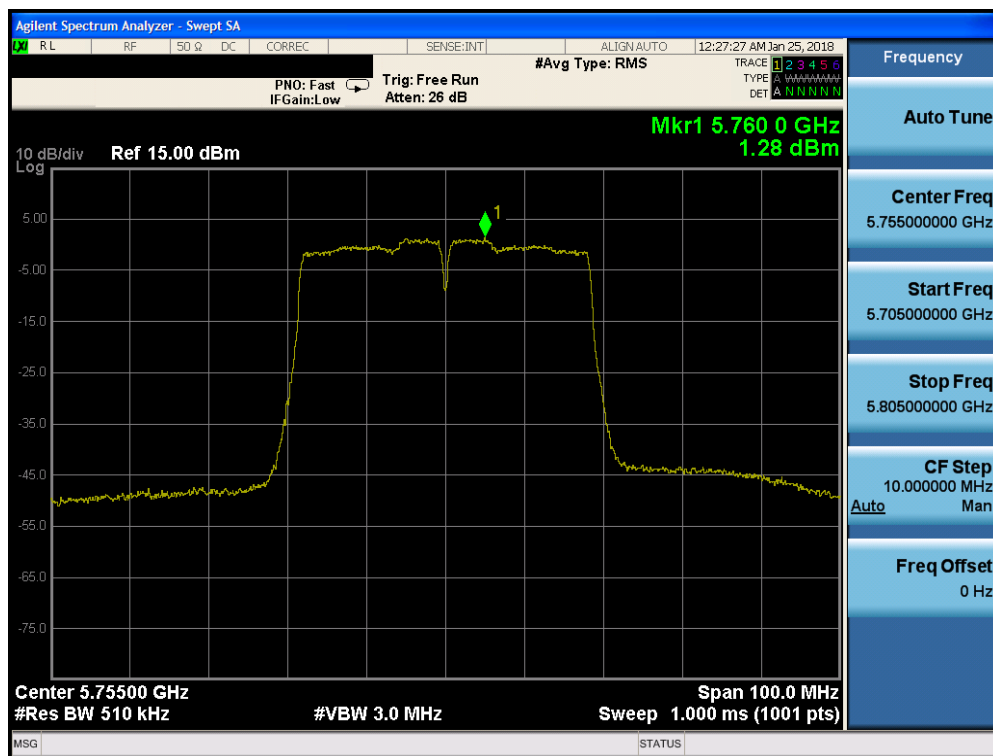
Plot 7-169. Power Spectral Density Plot FCC SISO ANT1 (40MHz BW 802.11n (UNII Band 3) – Ch. 151)
