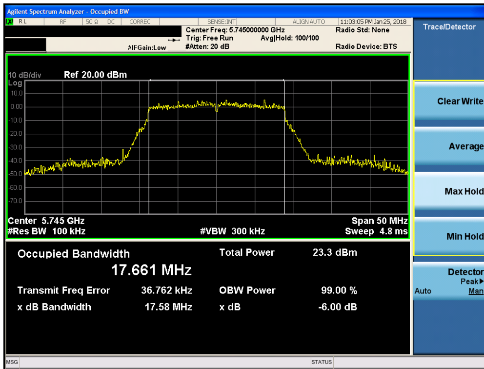
Plot 7-122. 6dB Bandwidth Plot MIMO ANT2 (20MHz BW 802.11n (UNII Band 3) – Ch. 149)
