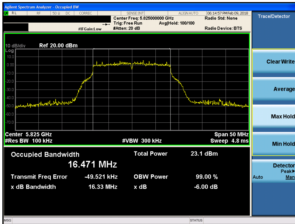
Plot 7-105. 6dB Bandwidth Plot FCC SISO ANT1 (802.11a (UNII Band 3) – Ch. 165)
