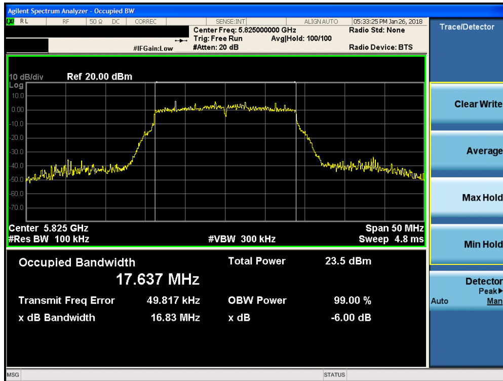
Plot 7-125. 6dB Bandwidth Plot MIMO ANT1 (20MHz BW 802.11n (UNII Band 3) – Ch. 165)
