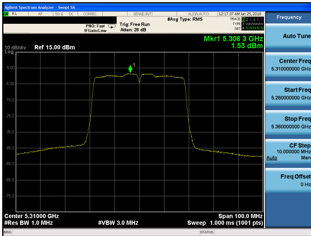
Plot 7-149. Power Spectral Density Plot FCC SISO ANT1 (40MHz BW 802.11n (UNII Band 2A) – Ch. 62)
