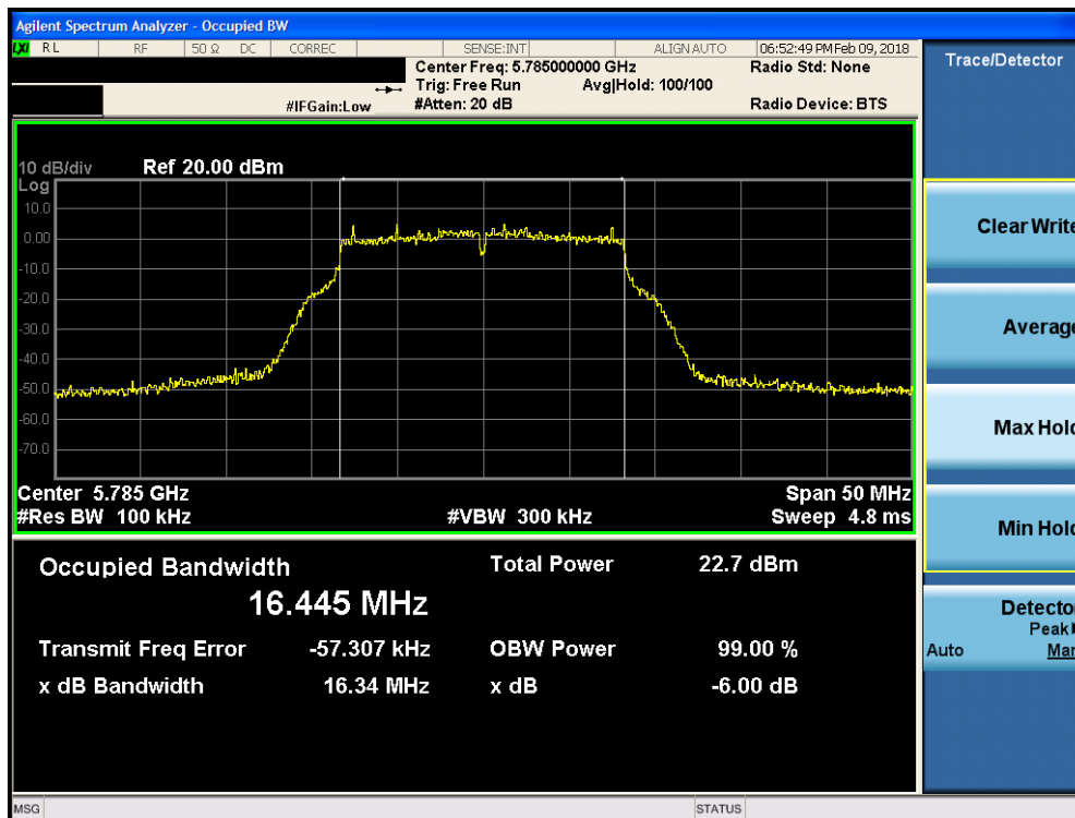
Plot 7-113. 6dB Bandwidth Plot FCC SISO ANT2 (802.11a (UNII Band 3) – Ch. 157)
