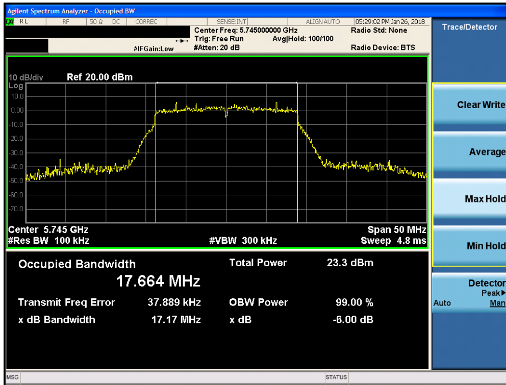
Plot 7-121. 6dB Bandwidth Plot MIMO ANT1 (20MHz BW 802.11n (UNII Band 3) – Ch. 149)
