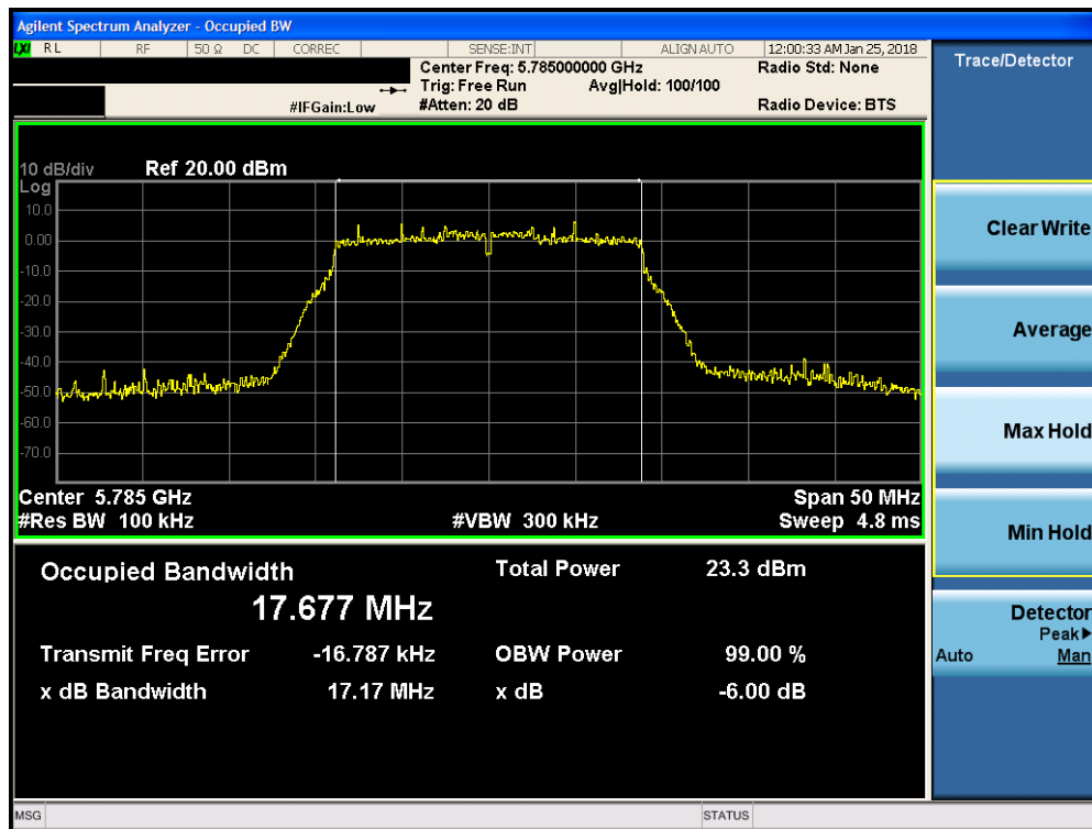
Plot 7-107. 6dB Bandwidth Plot FCC SISO ANT1 (20MHz BW 802.11n (UNII Band 3) – Ch. 157)
