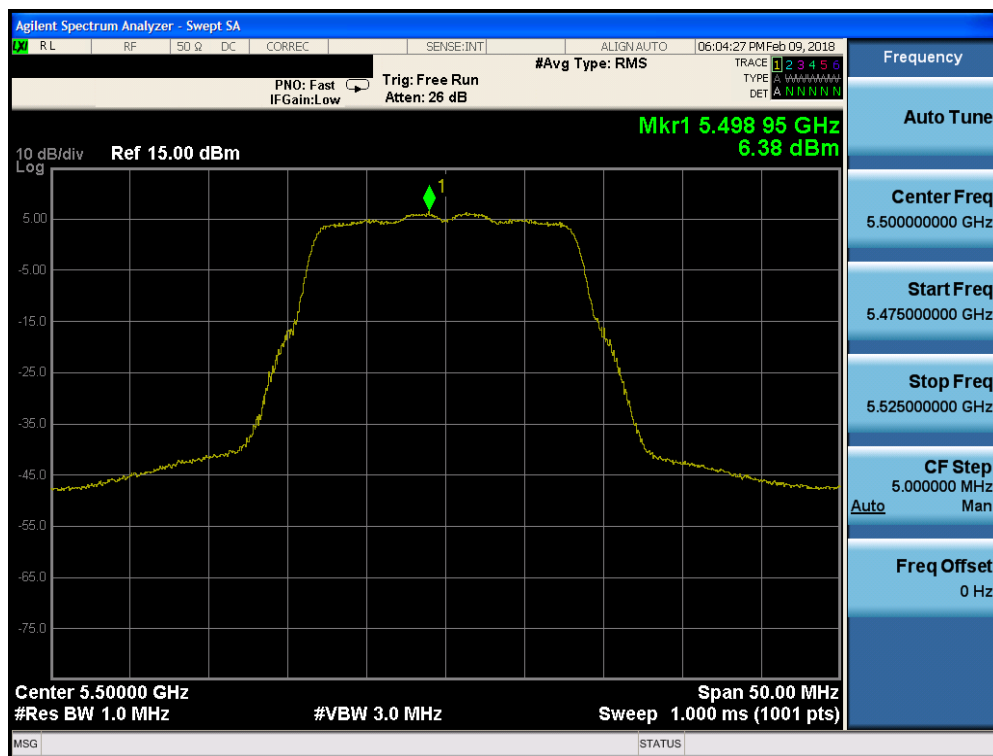
Plot 7-151. Power Spectral Density Plot FCC SISO ANT1 (802.11a (UNII Band 2C) – Ch. 100)
