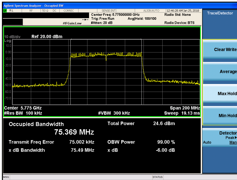
Plot 7-111. 6dB Bandwidth Plot FCC SISO ANT1 (80MHz BW 802.11ac (UNII Band 3) – Ch. 155)
