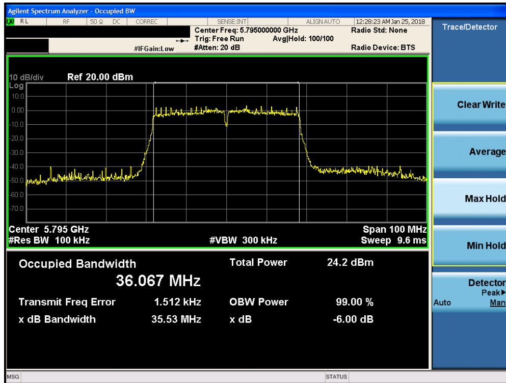
Plot 7-110. 6dB Bandwidth Plot FCC SISO ANT1 (40MHz BW 802.11n (UNII Band 3) – Ch. 159)
