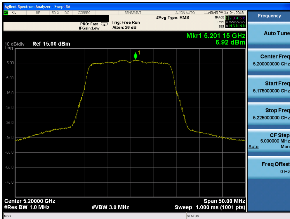
Plot 7-137. Power Spectral Density Plot FCC SISO ANT1 (20MHz BW 802.11n (UNII Band 1) – Ch. 40)
