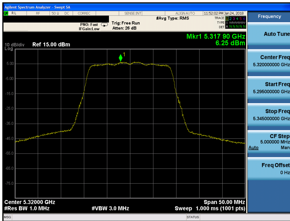
Plot 7-147. Power Spectral Density Plot FCC SISO ANT1 (20MHz BW 802.11n (UNII Band 2A) – Ch. 64)
