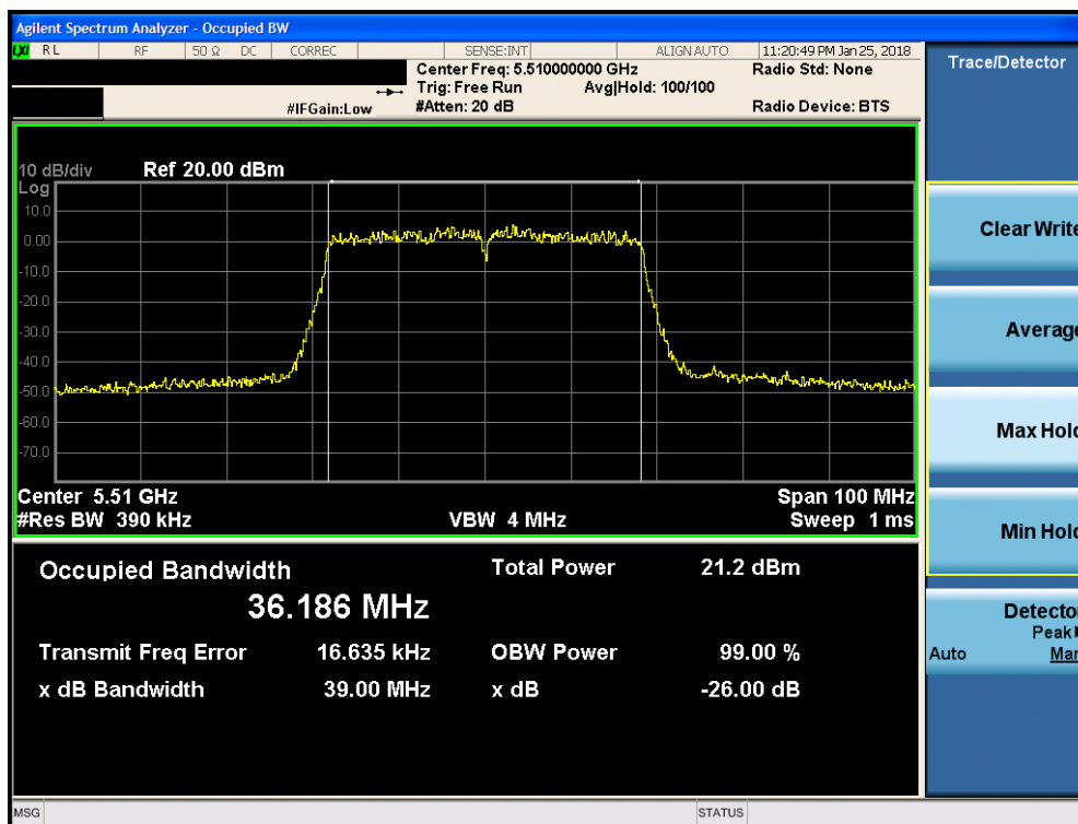
Plot 7-92. 26dB Bandwidth Plot MIMO ANT2 (40MHz BW 802.11n (UNII Band 2C) – Ch. 102)
