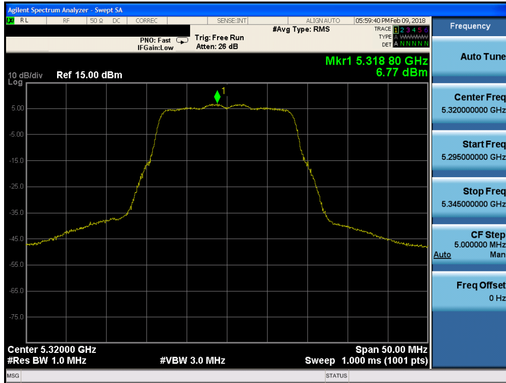
Plot 7-144. Power Spectral Density Plot FCC SISO ANT1 (802.11a (UNII Band 2A) – Ch. 64)
