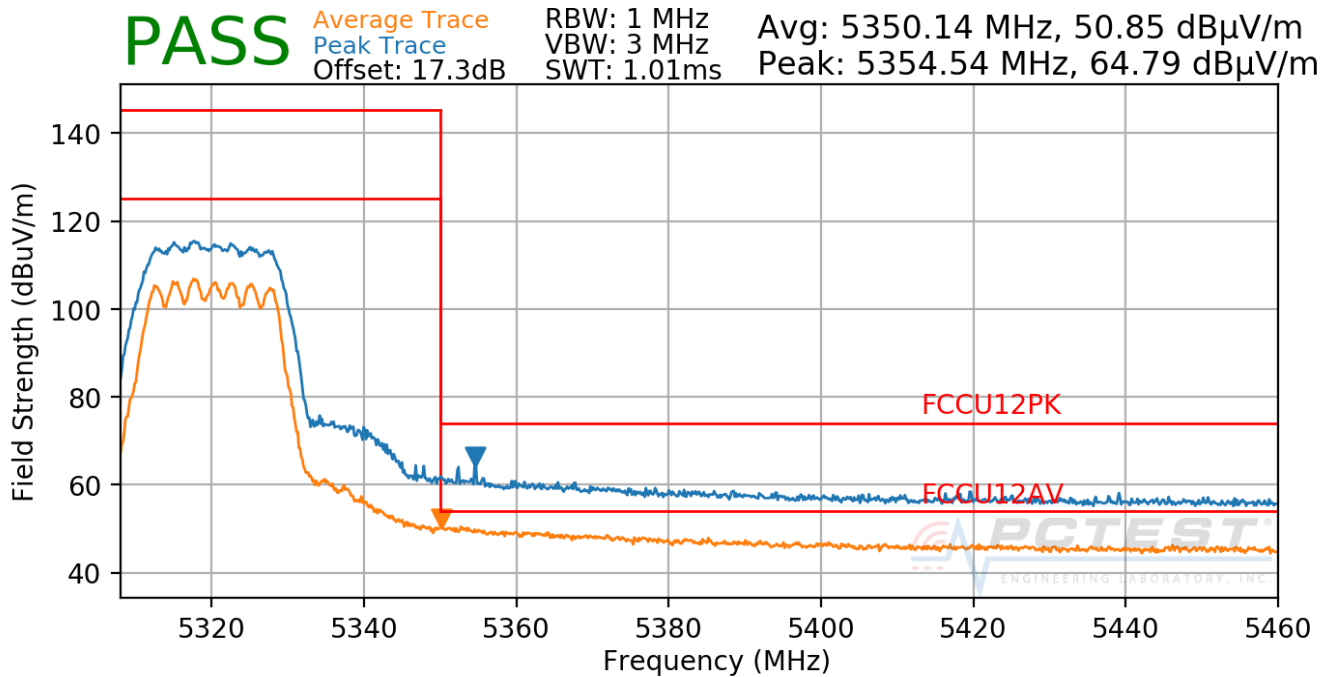
Plot 7-323. Radiated Upper Band Edge Plot MIMO (Average & Peak – UNII Band 2A)
