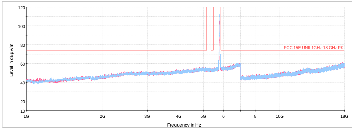
Plot 7-280. Radiated Spurious Plot above 1GHz SISO ANT1 (802.11n – U3 Ch. 157 H & V)
