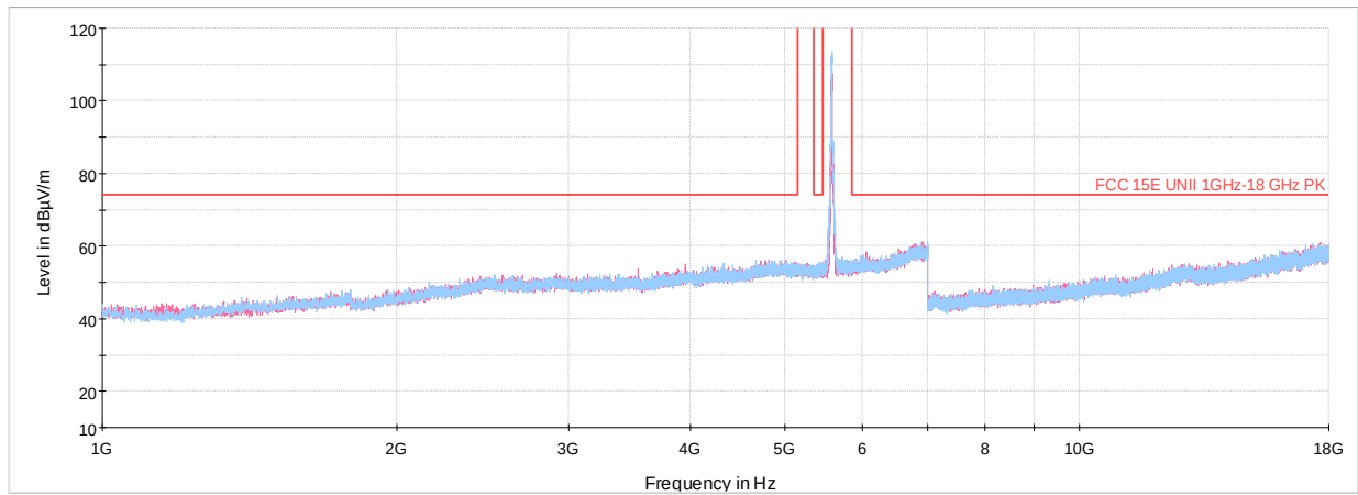
Plot 7-279. Radiated Spurious Plot above 1GHz SISO ANT1 (802.11n – U2C Ch. 116 H & V)
