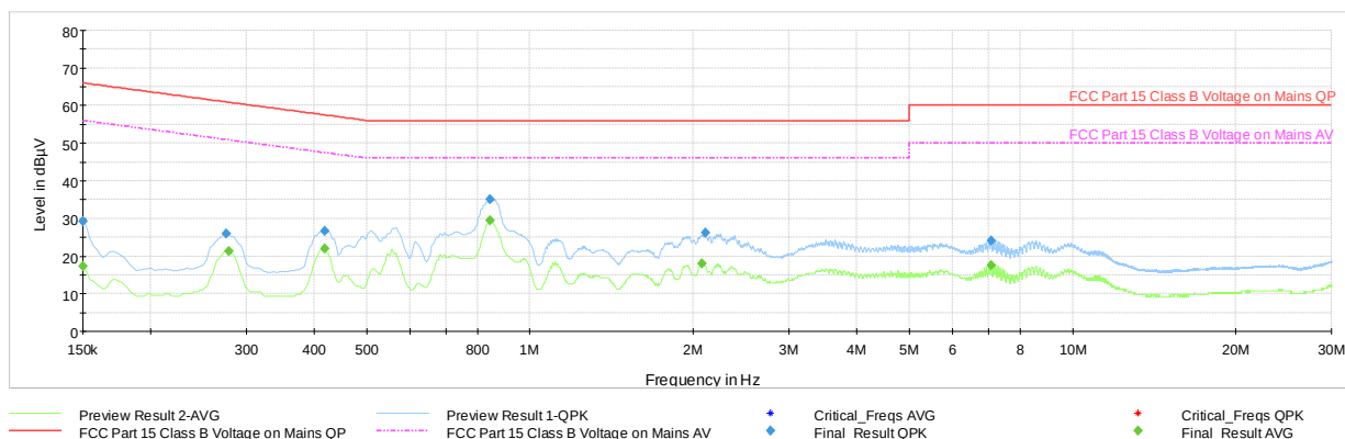
Plot 7-336. Line Conducted Plot with 802.11n UNII Band 1 (L1) SISO ANT1
