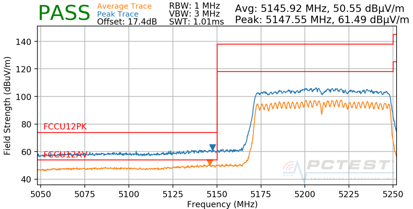
Plot 7-330. Radiated Lower Band Edge Plot MIMO (Average & Peak – UNII Band 1)
