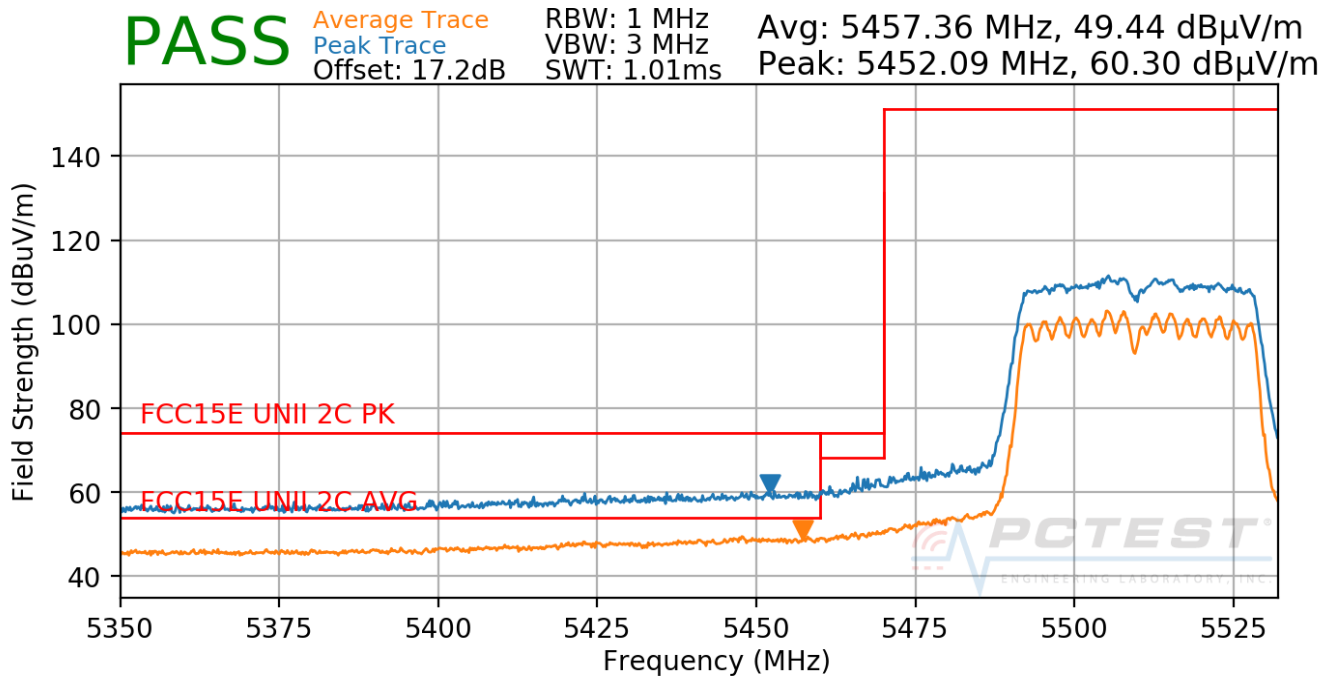
Plot 7-328. Radiated Lower Band Edge Plot MIMO (Average & Peak – UNII Band 2C)
