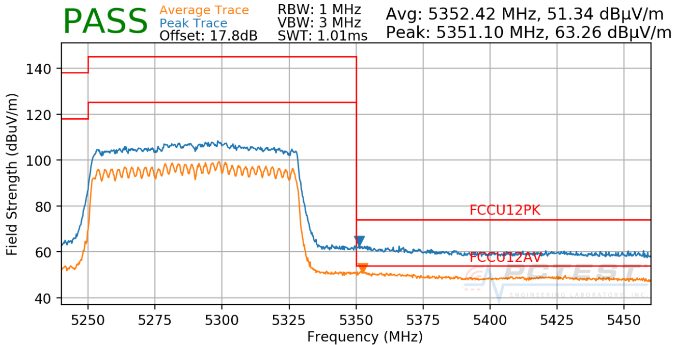
Plot 7-331. Radiated Upper Band Edge Plot MIMO (Average & Peak – UNII Band 2A)
