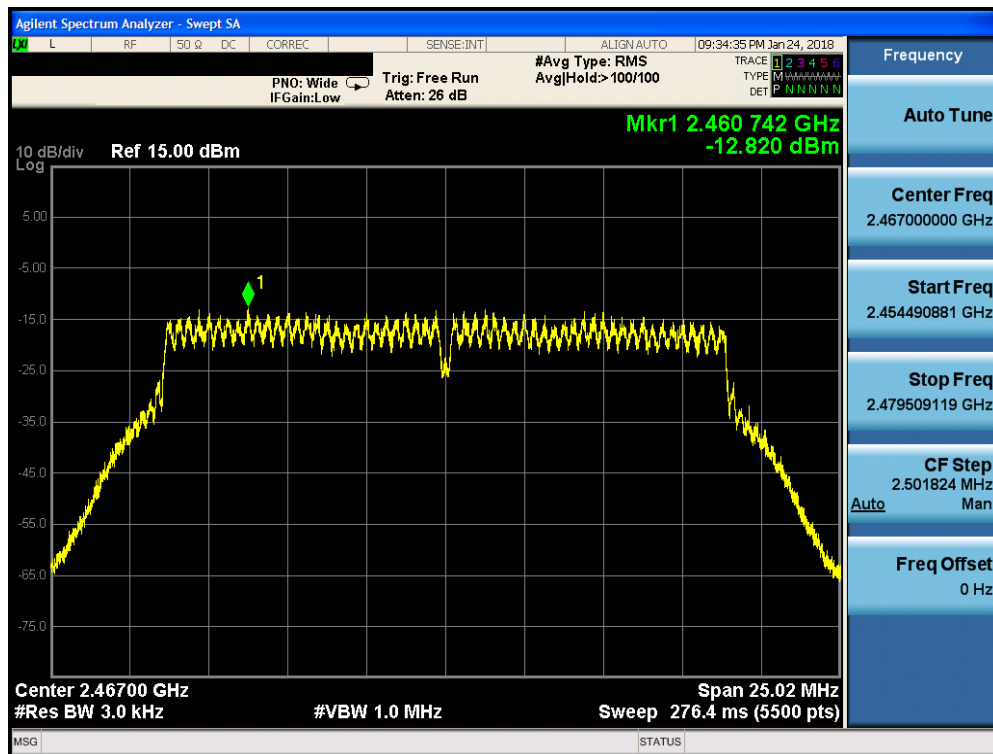
Plot 7-46. Power Spectral Density Plot SISO ANT1 (802.11n (2.4GHz) – Ch. 12)
