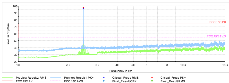
Plot #8 Radiated Emissions: 1-18 GHz
