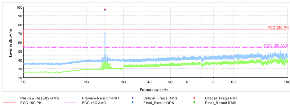
Plot #5 Radiated Emissions: 1-18 GHz
