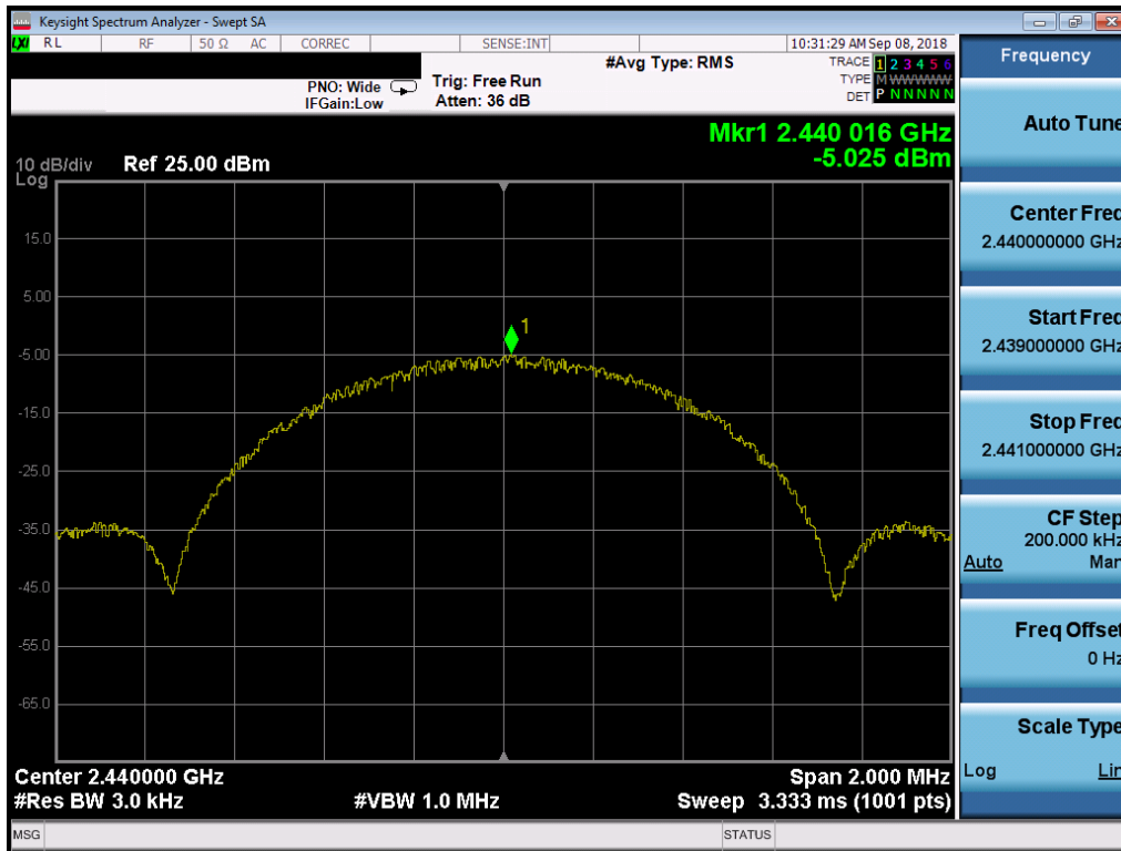
Plot 7-23. Power Spectral Density Plot (Bluetooth (LE), 1Mbps, iPA – Ch. 19, Antenna 0)
