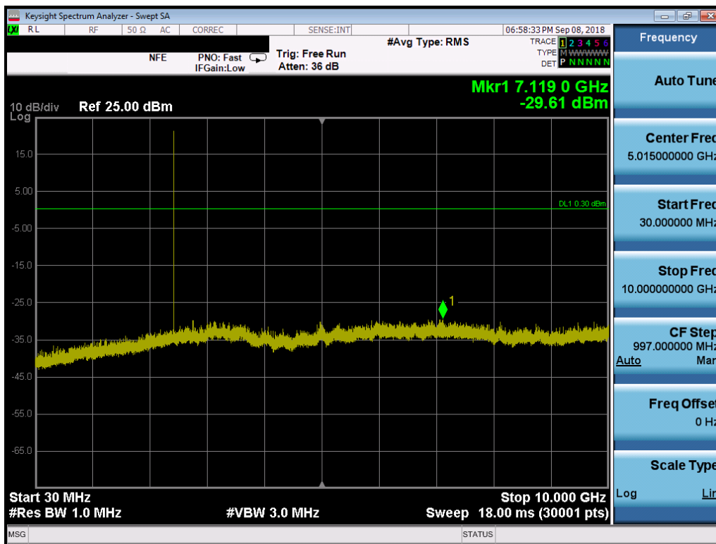
Plot 7-69. Conducted Spurious Plot (Bluetooth (LE), 1Mbps, ePA – Ch. 19, Antenna 1)
