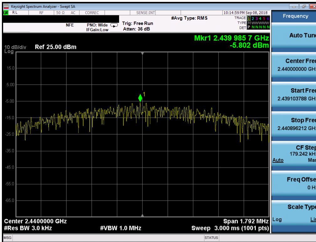
Plot 7-53. Power Spectral Density Plot (Bluetooth (LE), 2Mbps, iPA – Ch. 19, Antenna 2)
