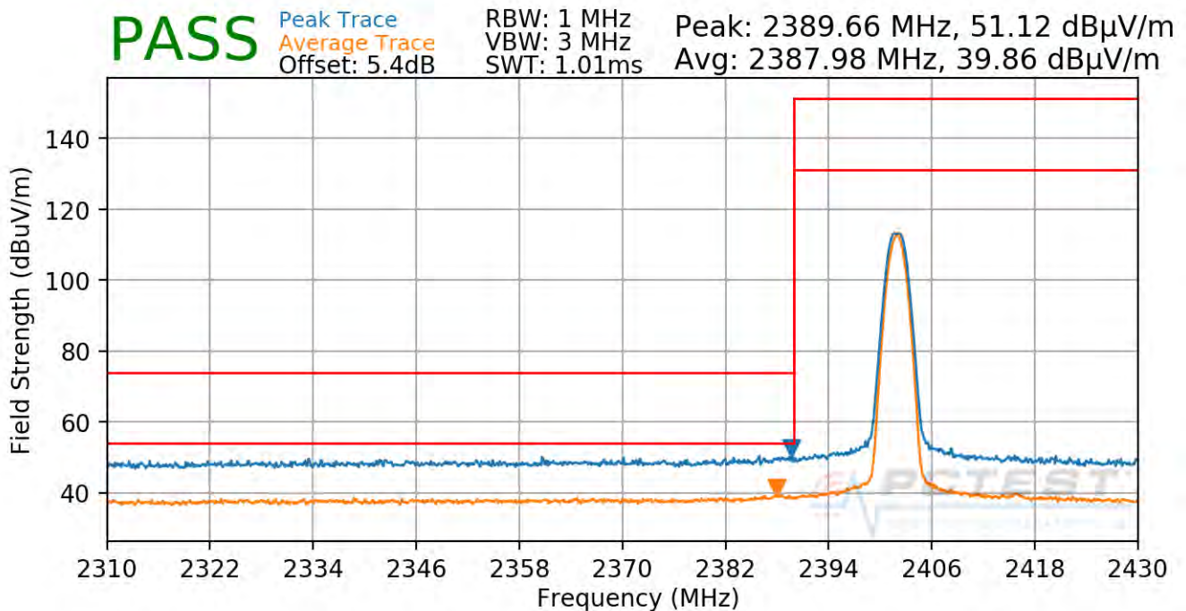
Plot 7-96. Radiated Restricted Lower Band Edge Measurement (Average & Peak), Antenna 1
