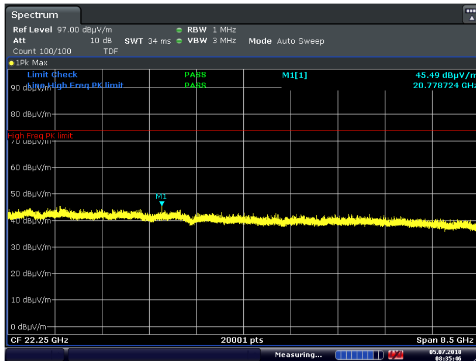
Plot 7-90. Radiated Spurious Plot above 18GHz (GFSK ePA, Pol. H) Antenna 1
