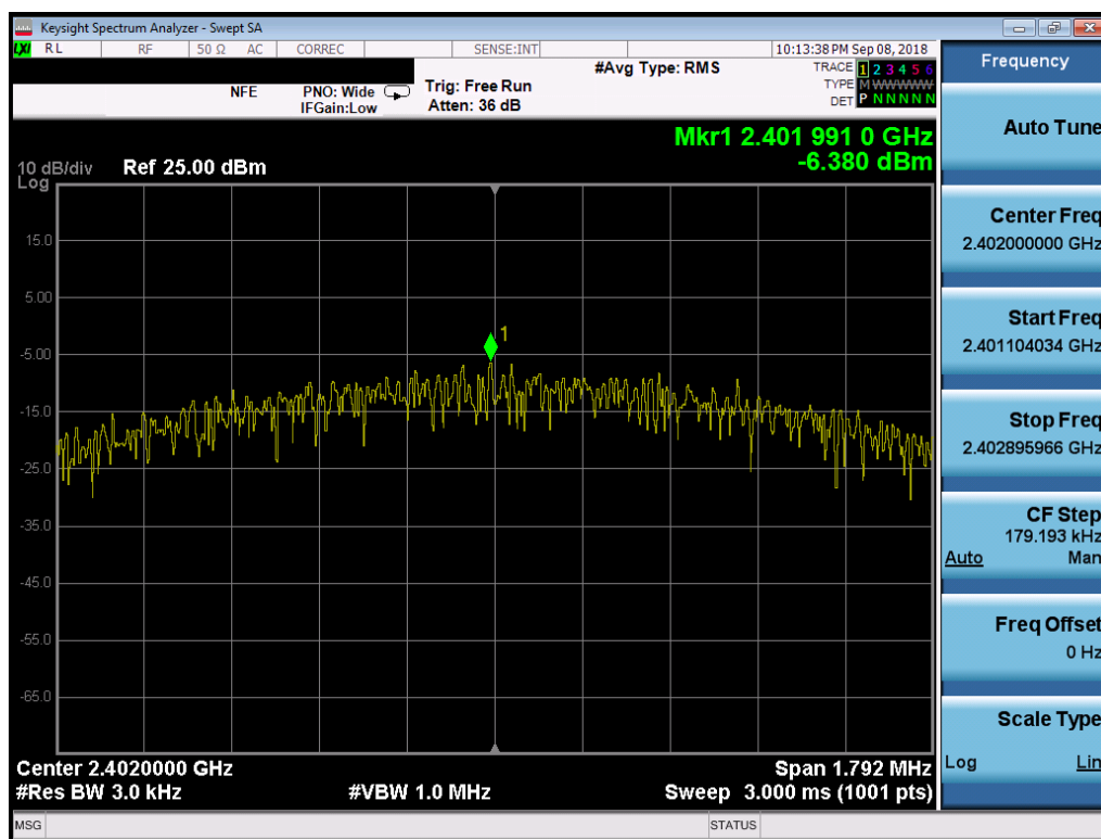
Plot 7-28. Power Spectral Density Plot (Bluetooth (LE), 2Mbps, iPA – Ch. 0, Antenna 0)
