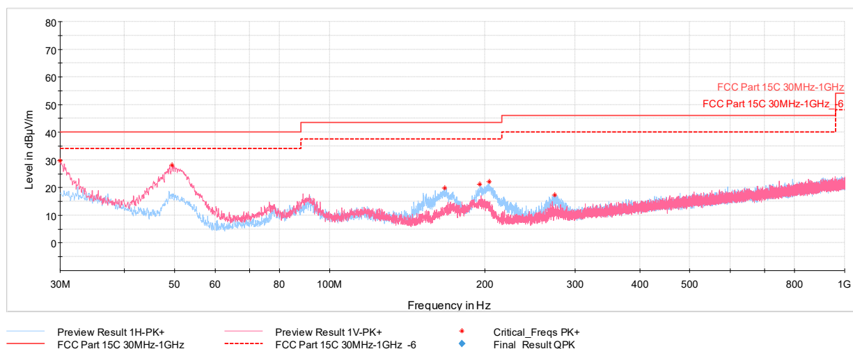
Plot 7-100. Radiated Spurious Plot below 1GHz (GFSK, ePA, Pol. H & V, with AC/DC Adapter)
