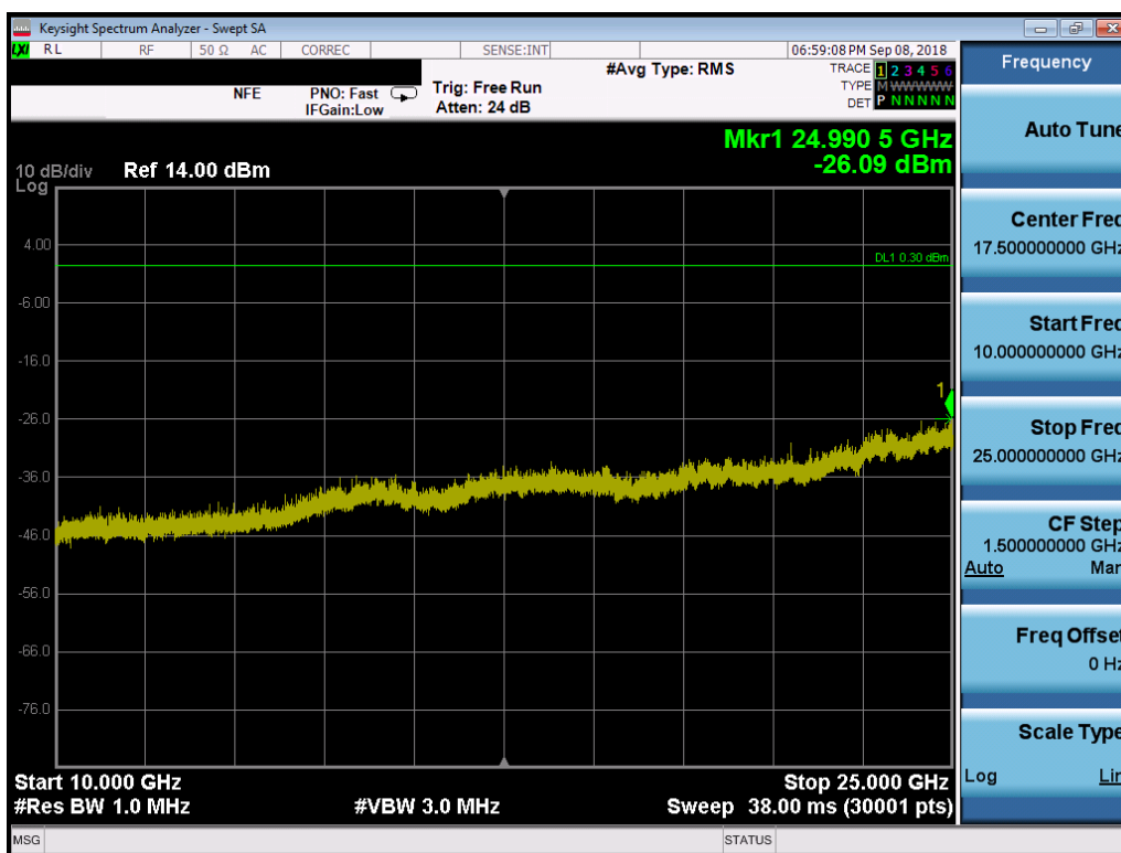
Plot 7-70. Conducted Spurious Plot (Bluetooth (LE), 1Mbps, ePA – Ch. 19, Antenna 1)
