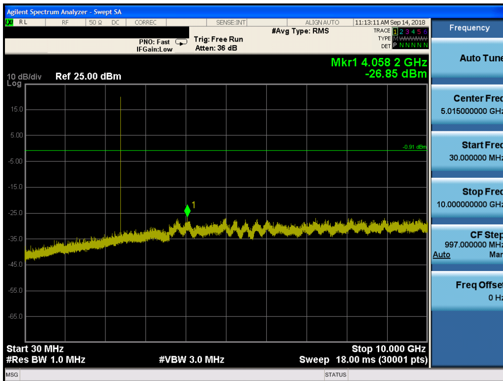
Plot 7-67. Conducted Spurious Plot (Bluetooth (LE), 1Mbps, ePA – Ch. 0, Antenna 1)
