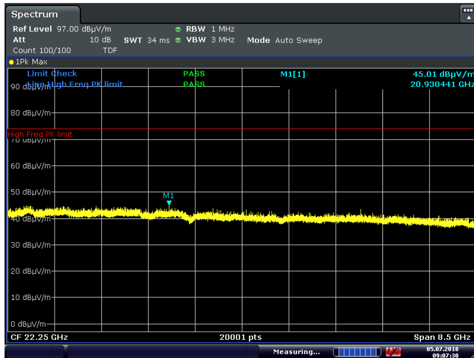
Plot 7-93. Radiated Spurious Plot above 18GHz (GFSK ePA, Pol. V) Antenna 2
