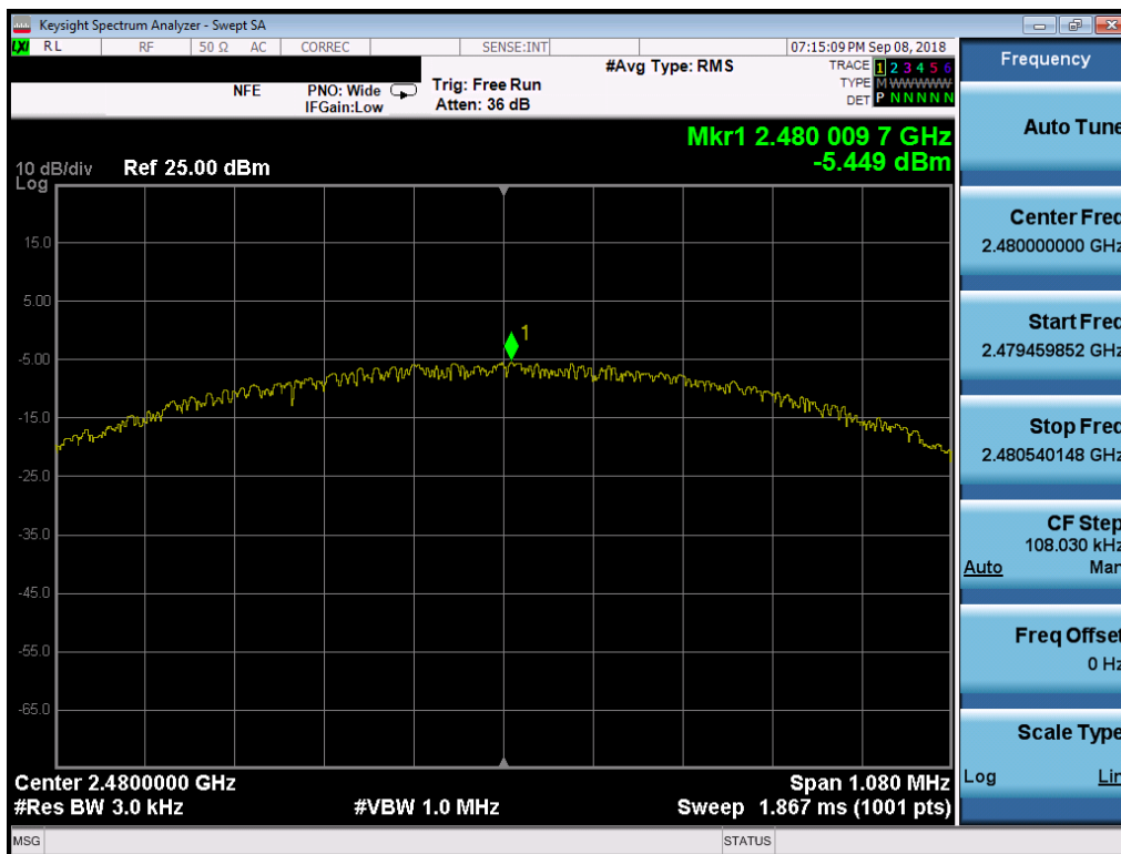
Plot 7-36. Power Spectral Density Plot (Bluetooth (LE), 1Mbps, iPA – Ch. 39, Antenna 1)
