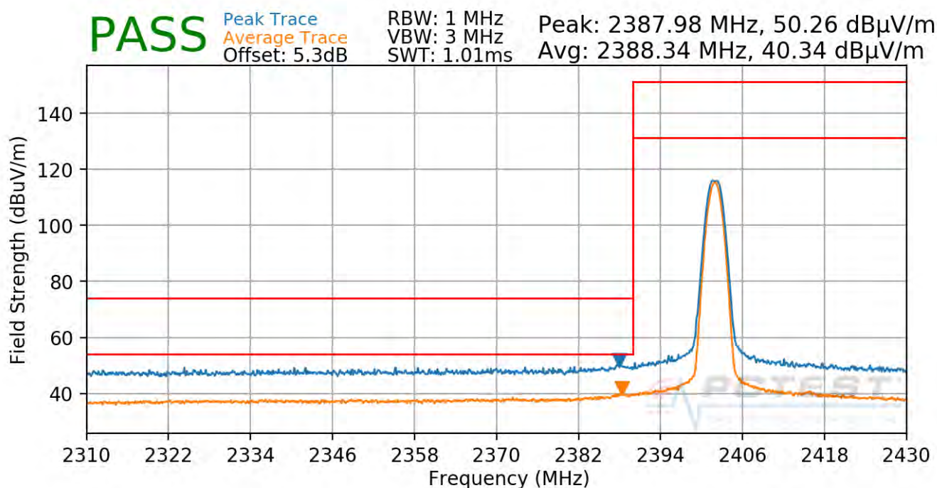
Plot 7-94. Radiated Restricted Lower Band Edge Measurement (Average & Peak), Antenna 0
