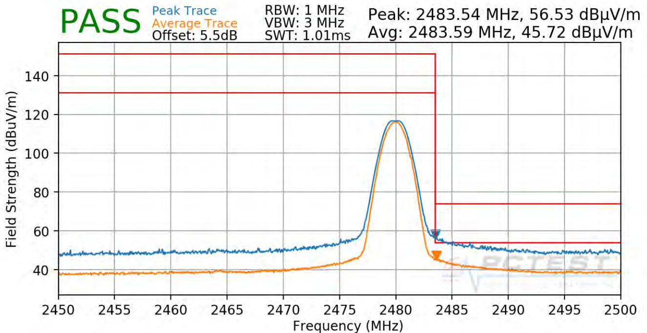
Plot 7-95. Radiated Restricted Upper Band Edge Measurement (Average & Peak), Antenna 0
