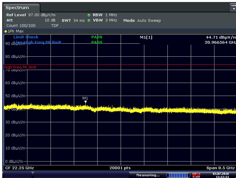
Plot 7-88. Radiated Spurious Plot above 18GHz (GFSK ePA, Pol. H) Antenna 0
