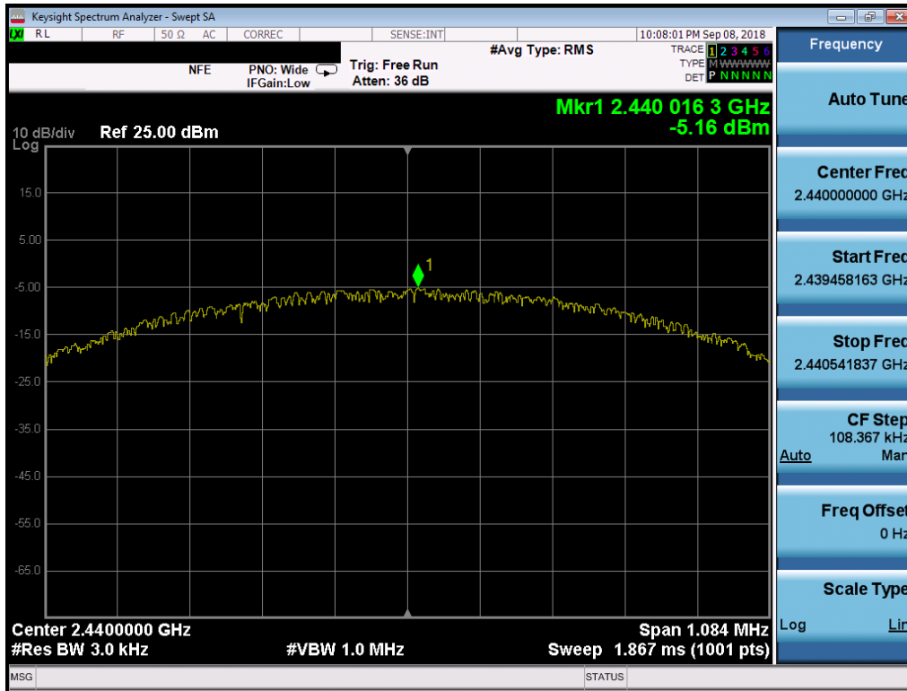
Plot 7-47. Power Spectral Density Plot (Bluetooth (LE), 1Mbps, iPA – Ch. 19, Antenna 2)
