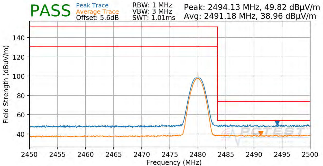
Plot 7-99. Radiated Restricted Upper Band Edge Measurement (Average & Peak), Antenna 2
