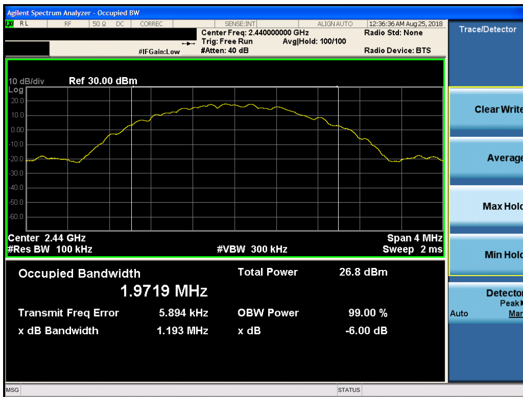
Plot 7-11. 6dB Bandwidth Plot (Bluetooth (LE), 2Mbps, ePA – Ch. 19, Antenna 1)
