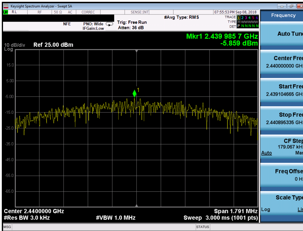
Plot 7-41. Power Spectral Density Plot (Bluetooth (LE), 2Mbps, iPA – Ch. 19, Antenna 1)
