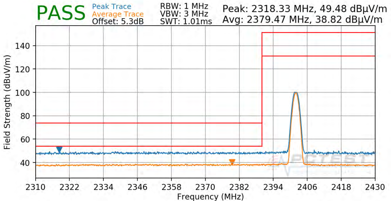
Plot 7-98. Radiated Restricted Lower Band Edge Measurement (Average & Peak), Antenna 2
