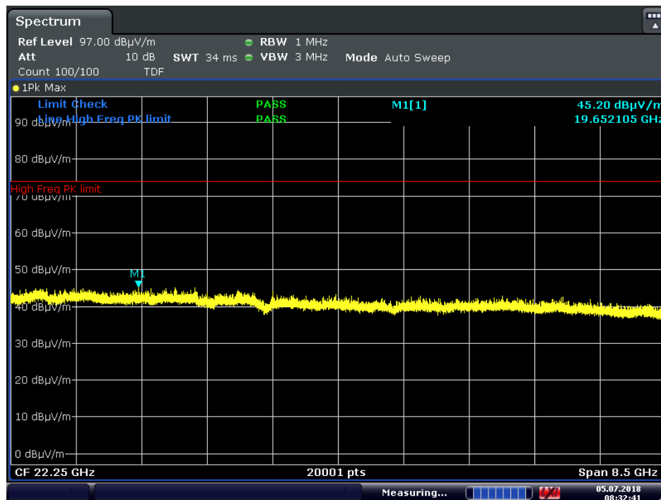
Plot 7-91. Radiated Spurious Plot above 18GHz (GFSK ePA, Pol. V) Antenna 1
