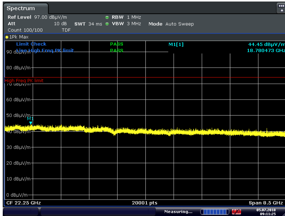
Plot 7-92. Radiated Spurious Plot above 18GHz (GFSK ePA, Pol. H) Antenna 2
