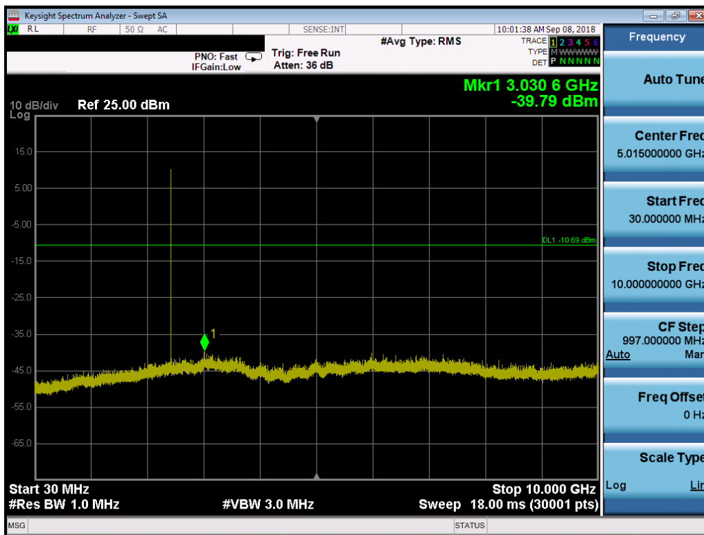
Plot 7-63. Conducted Spurious Plot (Bluetooth (LE), 1Mbps, ePA – Ch. 19, Antenna 0)
