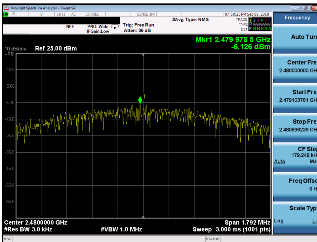
Plot 7-42. Power Spectral Density Plot (Bluetooth (LE), 2Mbps, iPA – Ch. 39, Antenna 1)
