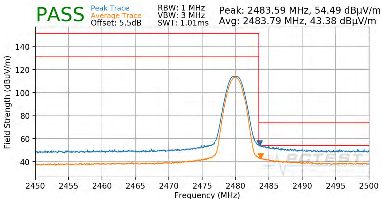
Plot 7-97. Radiated Restricted Upper Band Edge Measurement (Average & Peak), Antenna 1
