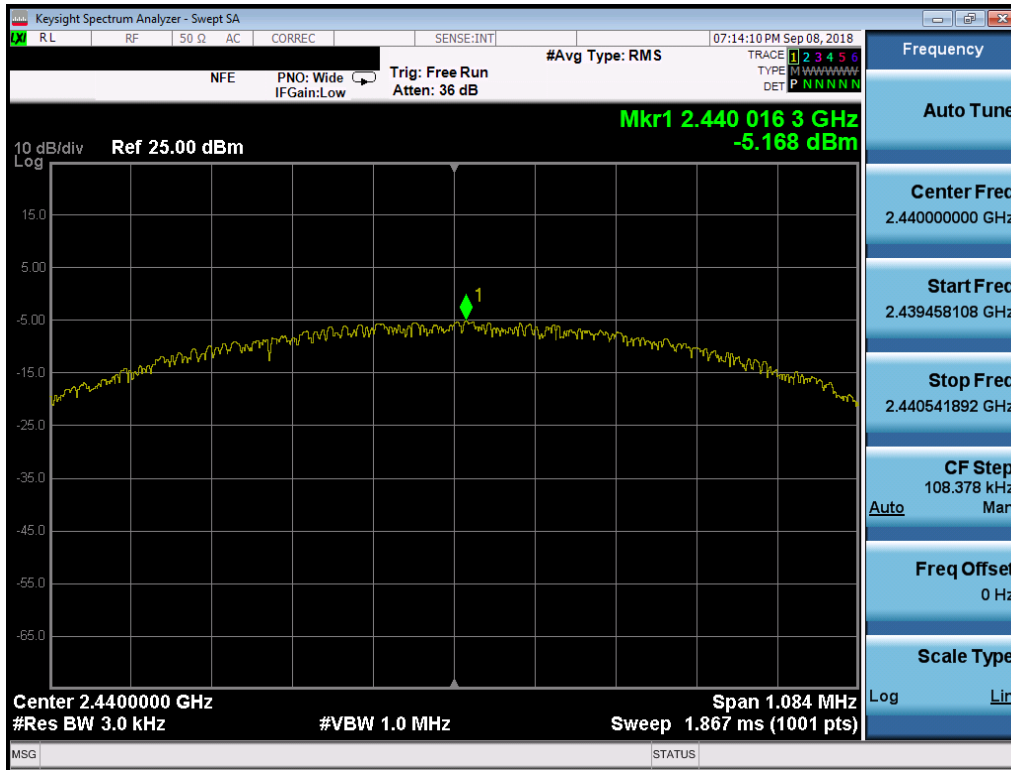
Plot 7-35. Power Spectral Density Plot (Bluetooth (LE), 1Mbps, iPA – Ch. 19, Antenna 1)
