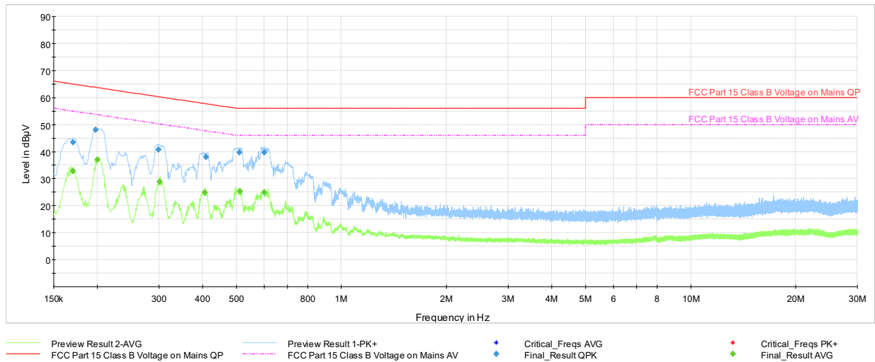
Plot 7-102. Line Conducted Plot with Bluetooth LE (GFSK ePA, N, with AC/DC Adapter)
