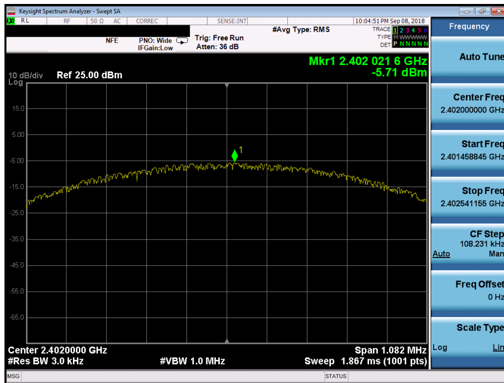
Plot 7-46. Power Spectral Density Plot (Bluetooth (LE), 1Mbps, iPA – Ch. 0, Antenna 2)
