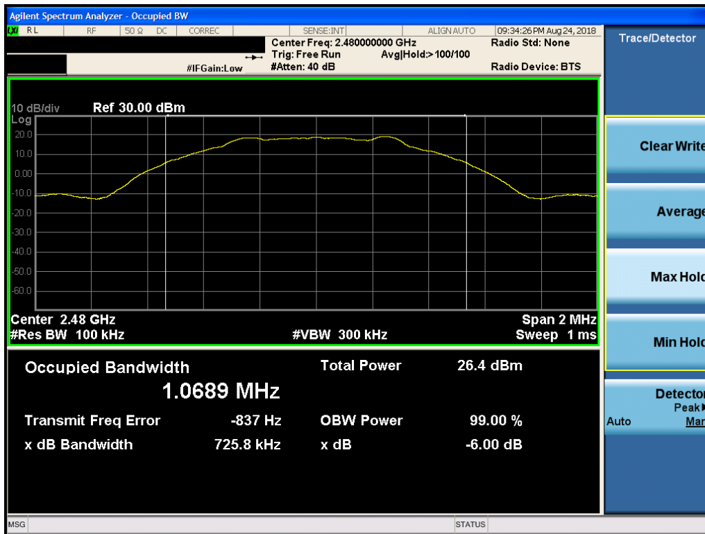
Plot 7-3. 6dB Bandwidth Plot (Bluetooth (LE), 1Mbps, ePA – Ch. 39, Antenna 0)
