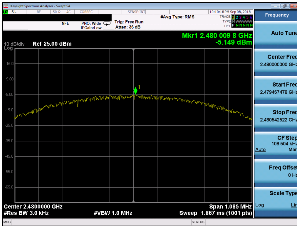
Plot 7-48. Power Spectral Density Plot (Bluetooth (LE), 1Mbps, iPA – Ch. 39, Antenna 2)
