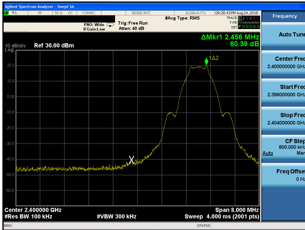
Plot 7-55. Band Edge Plot (Bluetooth (LE), ePA – Ch. 0, Antenna 0)
