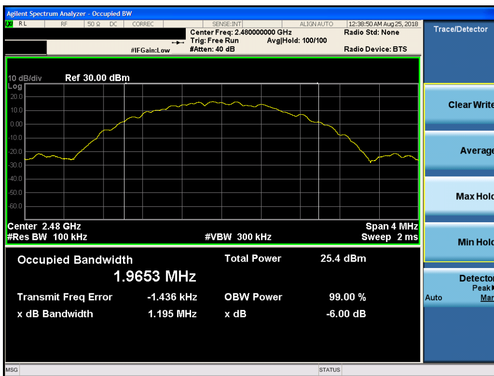
Plot 7-12. 6dB Bandwidth Plot (Bluetooth (LE), 2Mbps, ePA – Ch. 39, Antenna 1)
