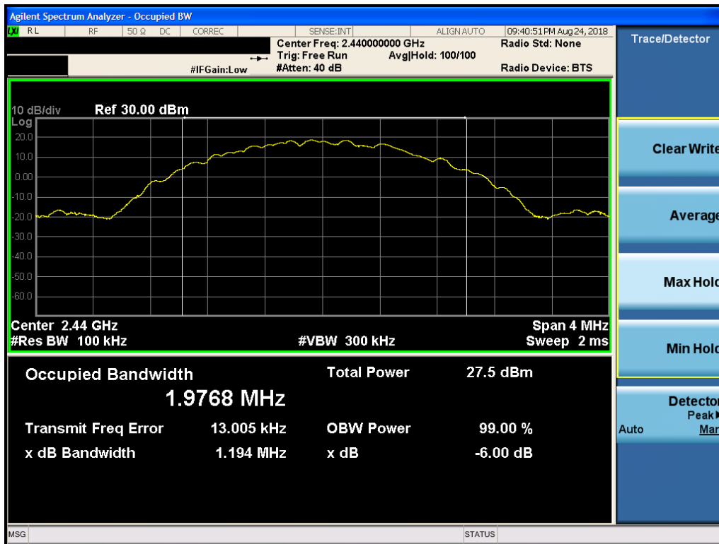
Plot 7-5. 6dB Bandwidth Plot (Bluetooth (LE), 2Mbps, ePA – Ch. 19, Antenna 0)
