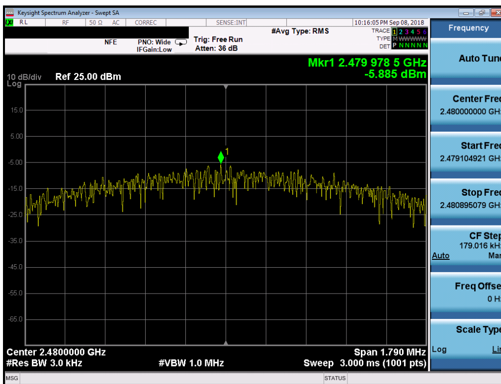
Plot 7-54. Power Spectral Density Plot (Bluetooth (LE), 2Mbps, iPA – Ch. 39, Antenna 2)
