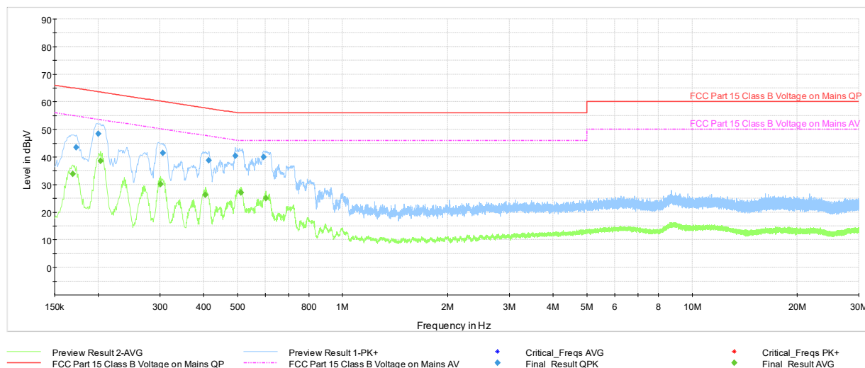
Plot 7-101. Line Conducted Plot with Bluetooth LE (GFSK ePA, L1, with AC/DC Adapter)
