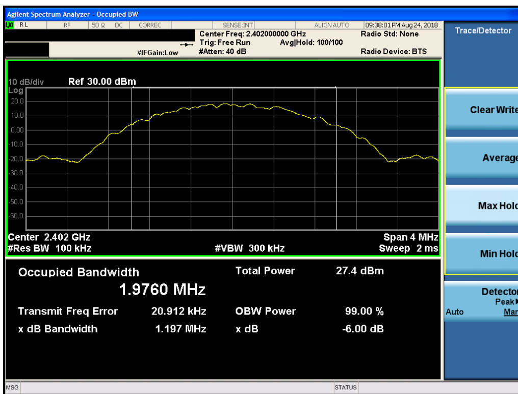
Plot 7-16. 6dB Bandwidth Plot (Bluetooth (LE), 2Mbps, ePA – Ch. 0, Antenna 2)
