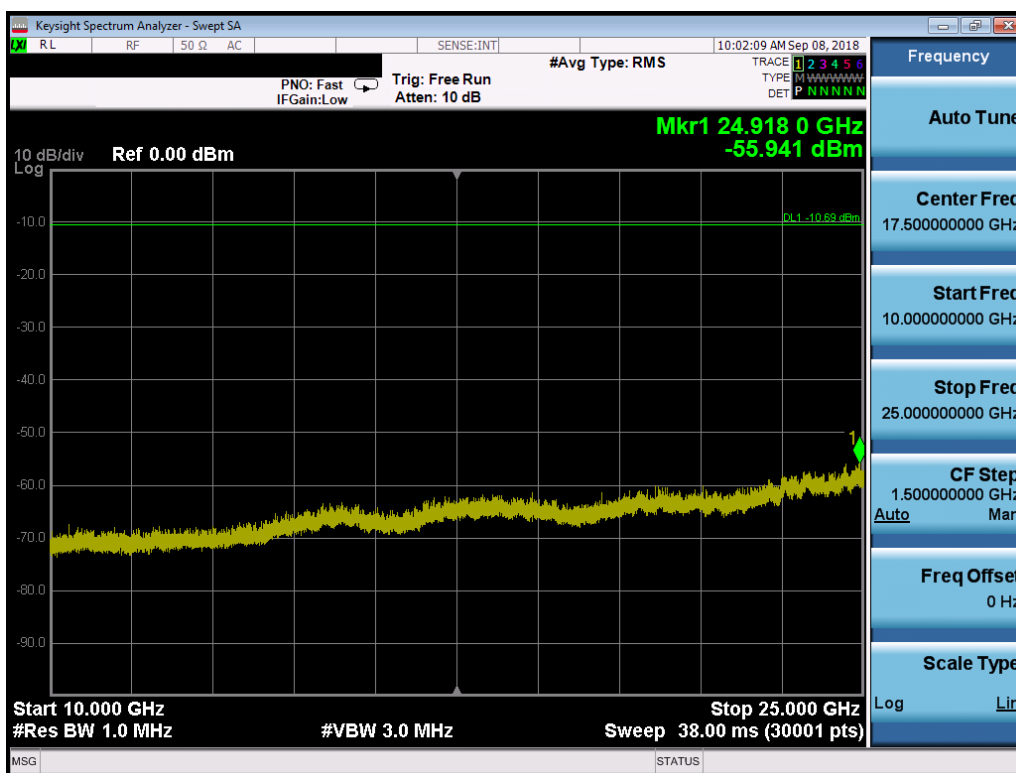
Plot 7-64. Conducted Spurious Plot (Bluetooth (LE), 1Mbps, ePA – Ch. 19, Antenna 0)
