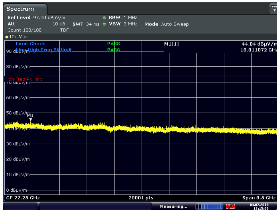
Plot 7-89. Radiated Spurious Plot above 18GHz (GFSK ePA, Pol. V) Antenna 0
