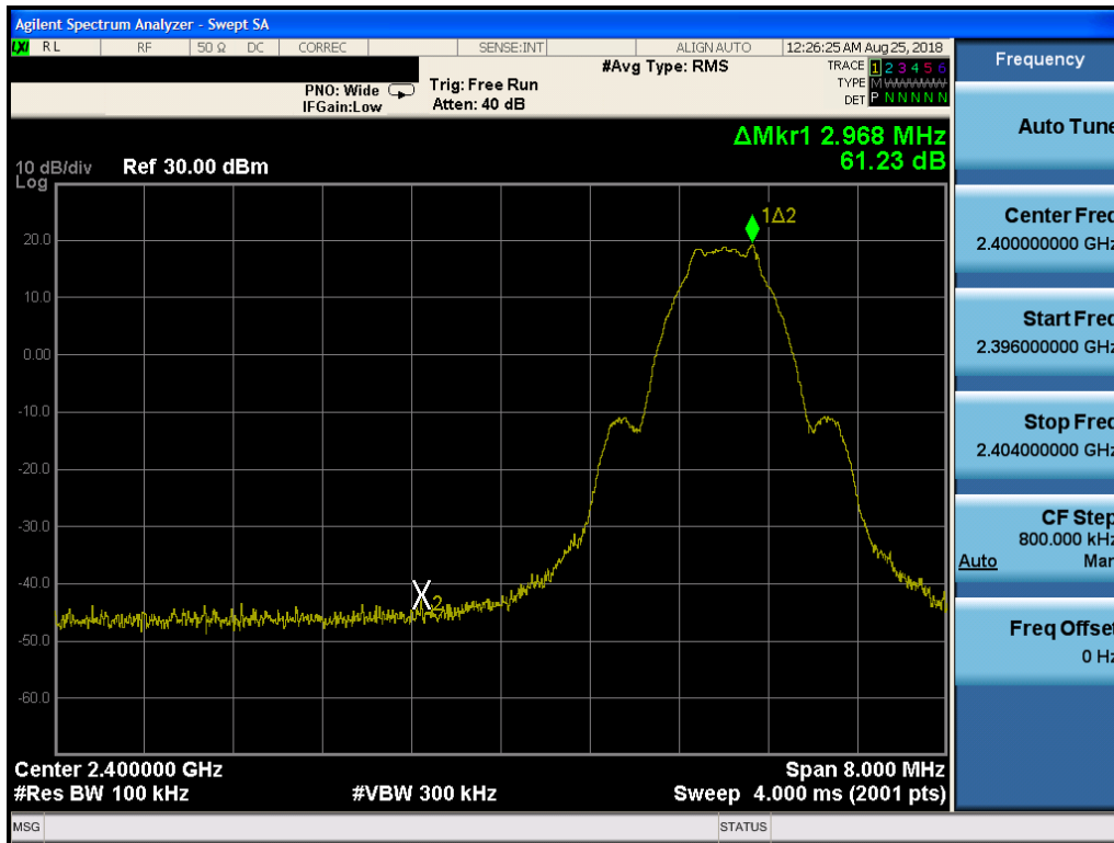
Plot 7-57. Band Edge Plot (Bluetooth (LE), ePA – Ch. 0, Antenna 1)
