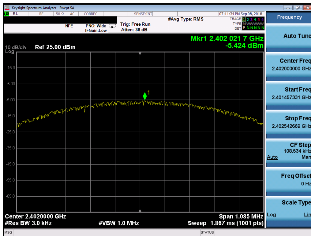
Plot 7-34. Power Spectral Density Plot (Bluetooth (LE), 1Mbps, iPA – Ch. 0, Antenna 1)
