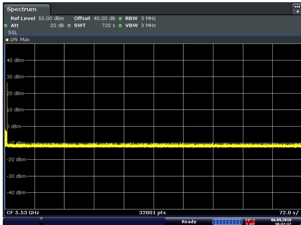
Figure 9-111 5530MHz - Monitoring 10 minutes (80MHz)
