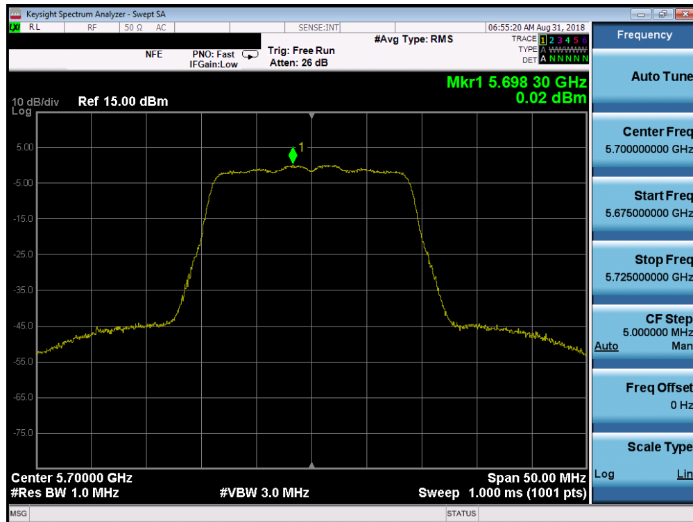
Plot 7-67. Power Spectral Density Plot SISO CORE 0 (20MHz BW 802.11n (UNII Band 2C) – Ch. 140)
