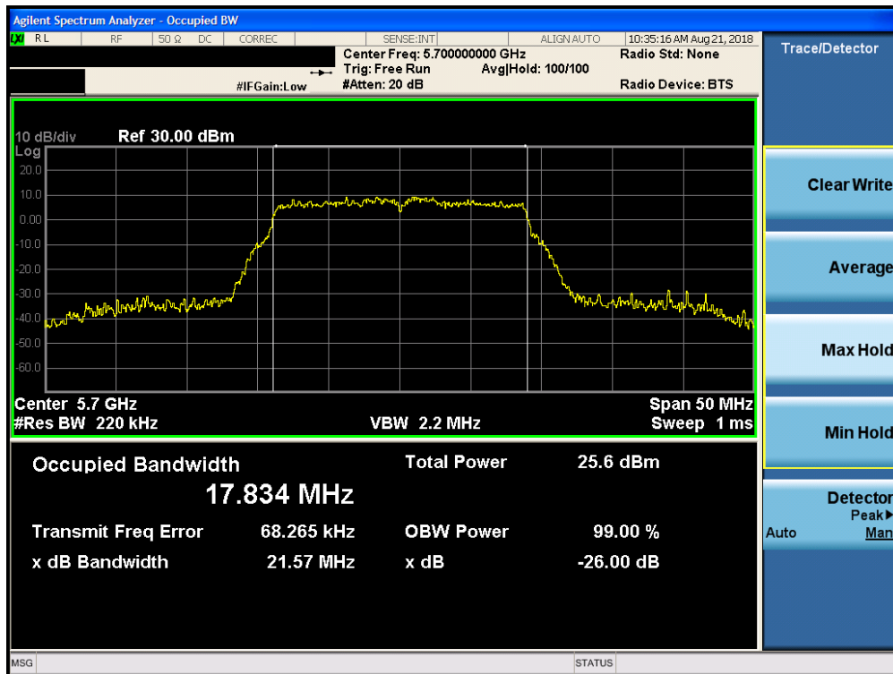
Plot 7-35. 26dB Bandwidth Plot SISO CORE 1 (20MHz BW 802.11n (UNII Band 2C) – Ch. 140)
