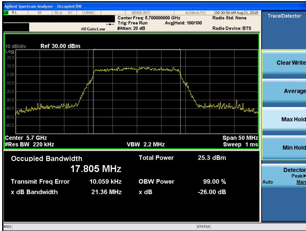
Plot 7-15. 26dB Bandwidth Plot SISO CORE 0 (20MHz BW 802.11n (UNII Band 2C) – Ch. 140)
