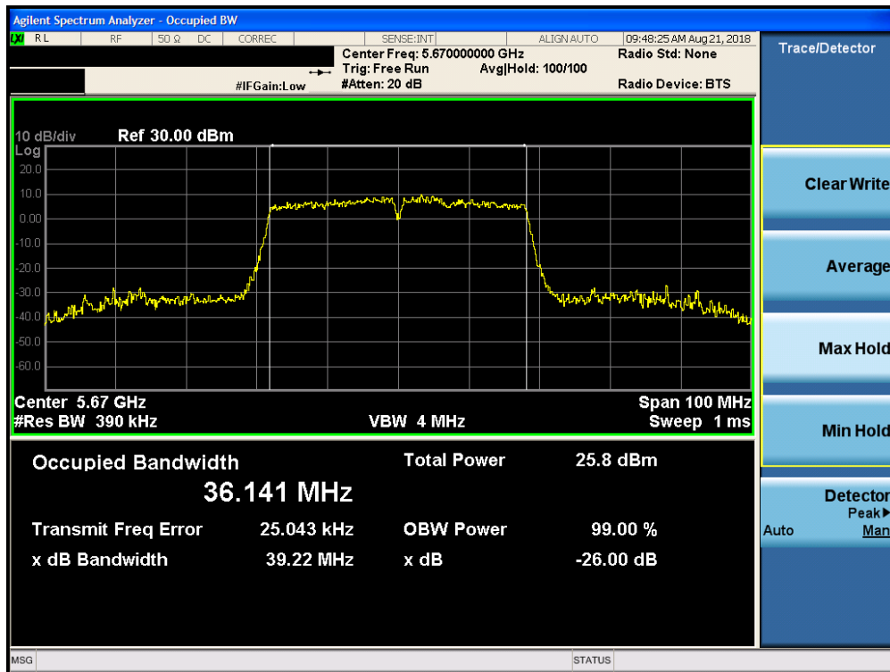
Plot 7-18. 26dB Bandwidth Plot SISO CORE 0 (40MHz BW 802.11n (UNII Band 2C) – Ch. 134)
