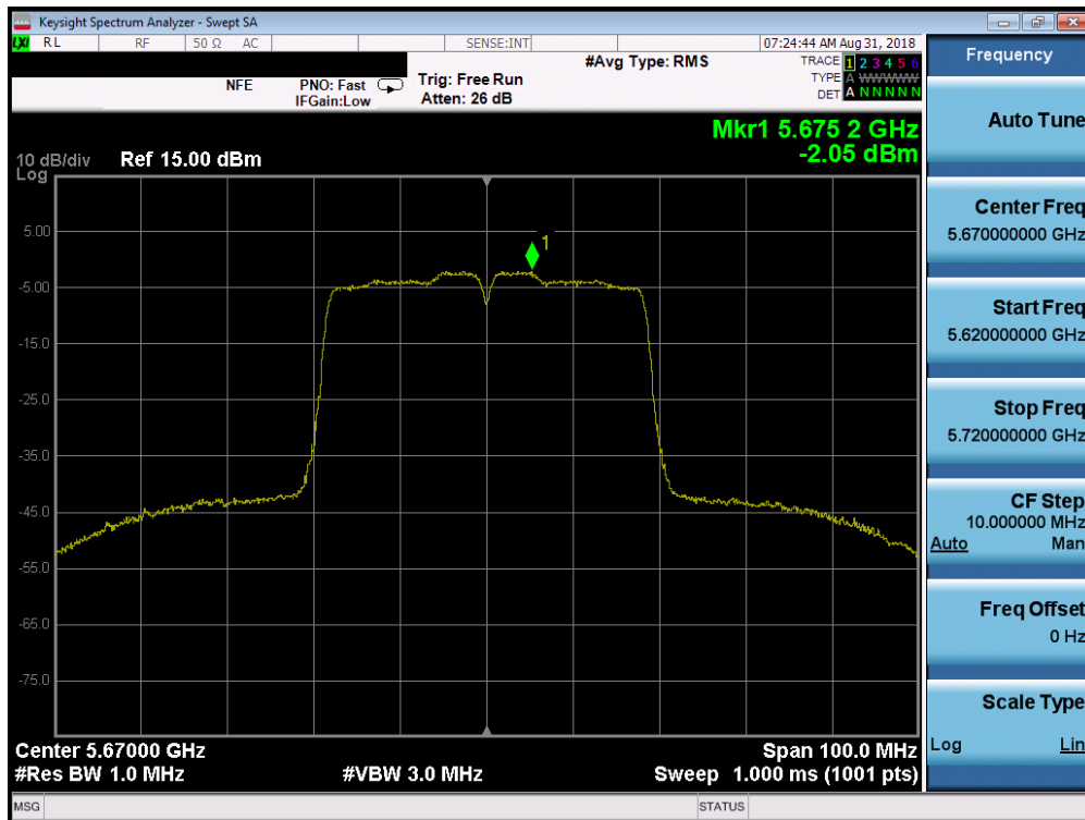
Plot 7-70. Power Spectral Density Plot SISO CORE 0 (40MHz BW 802.11n (UNII Band 2C) – Ch. 134)
