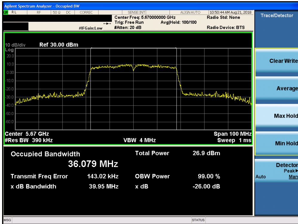
Plot 7-38. 26dB Bandwidth Plot SISO CORE 1 (40MHz BW 802.11n (UNII Band 2C) – Ch. 134)
