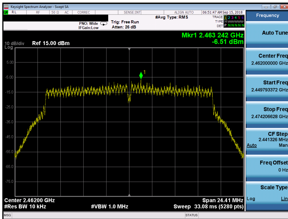
Plot 7-65. Power Spectral Density Plot CDD Core 0 (802.11n – Ch. 11)
