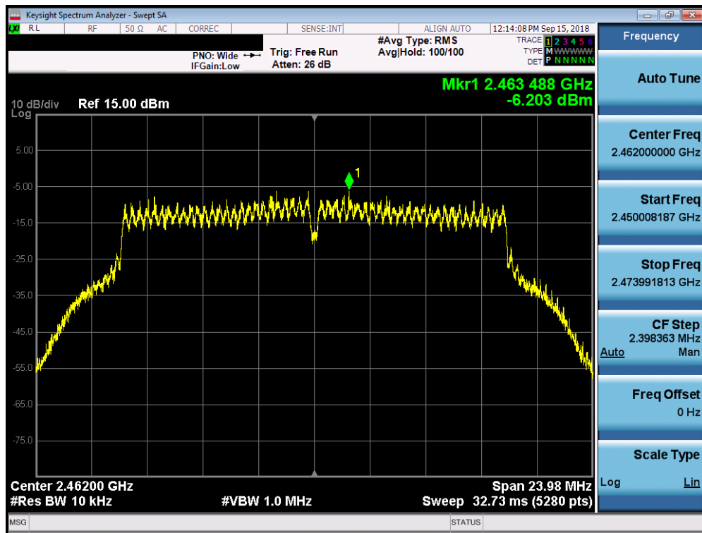
Plot 7-71. Power Spectral Density Plot CDD Core 0 (802.11g – Ch. 11)
