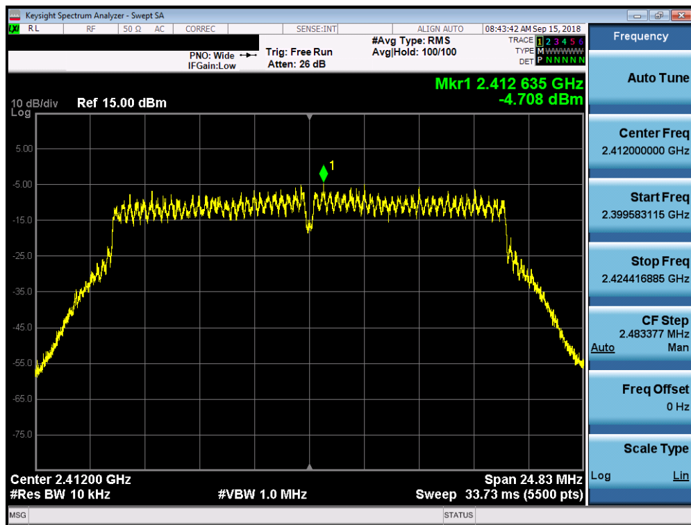
Plot 7-73. Power Spectral Density Plot CDD Core 0 (802.11n – Ch. 1)
