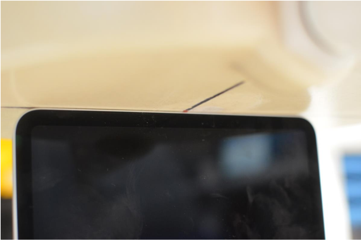
SAR Test Setup Photo 4: Bottom Edge at 0 mm
