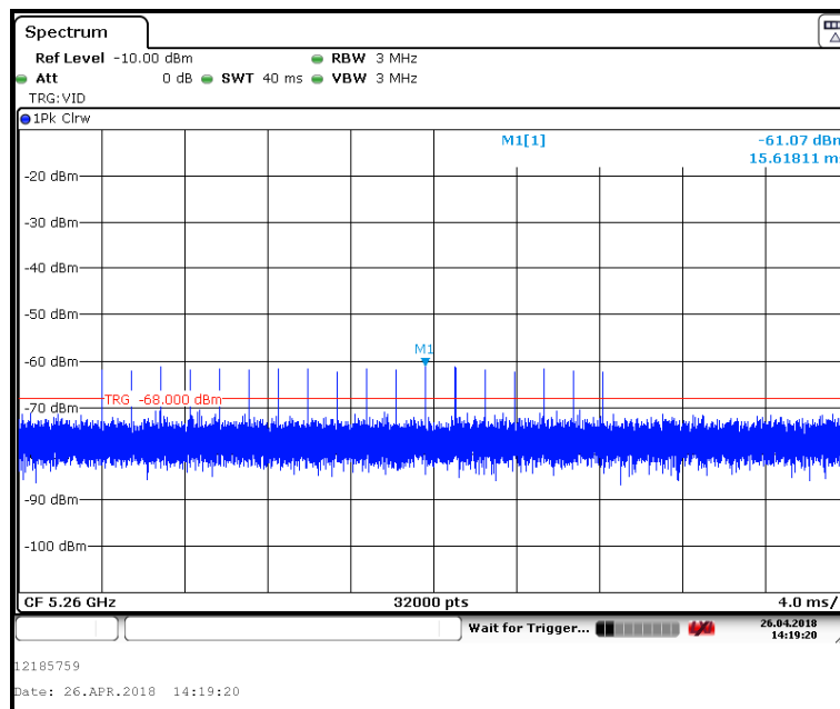
Radar Type 0 – full 18 pulse waveform – Setup 2 (client to client)
