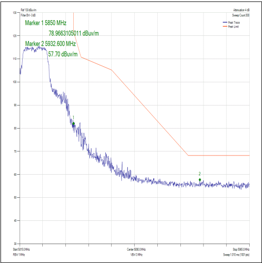
Figure 402 – Channel 165 - Authorised Band Edge
