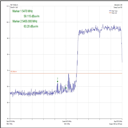
Figure 438 – Channel 106 - Authorised Band Edge
