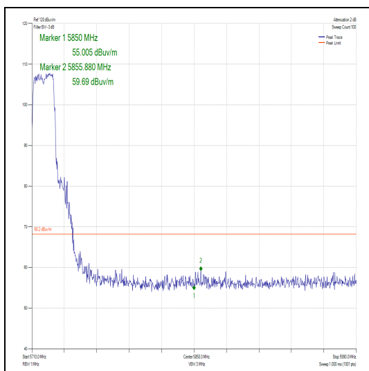
Figure 455 – Channel 144 - Authorised Band Edge
