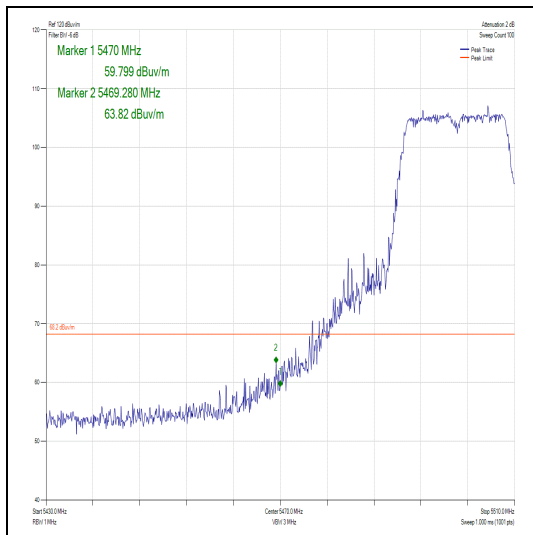
Figure 453 – Channel 100 - Authorised Band Edge
