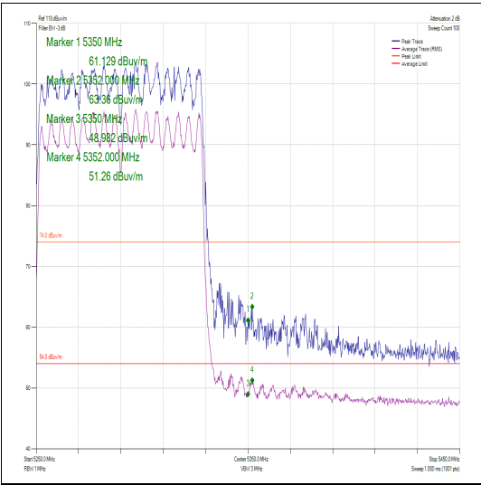
Figure 540 – Channel 58 - Restricted Band Edge
