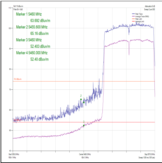
Figure 553 – Channel 106 - Restricted Band Edge
