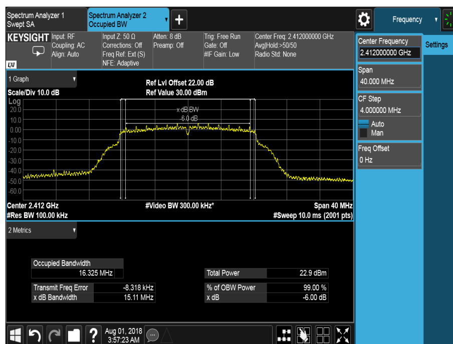
Figure 4 - 2412 MHz – 6 dB Bandwidth and 99% Occupied Bandwidth
