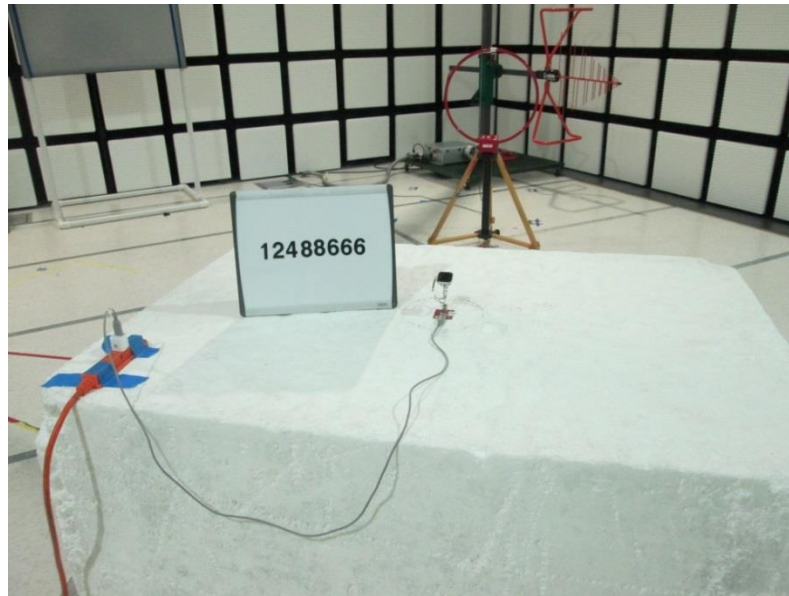
RADIATED EMISSIONS BELOW 30MHz (Front – With Watch)
