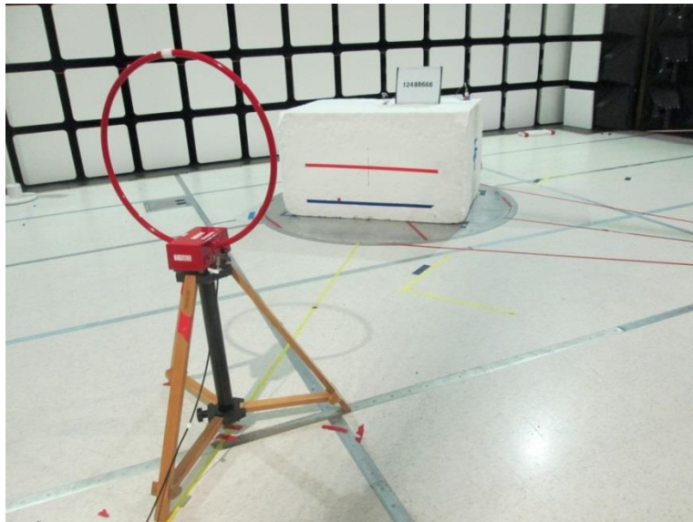
RADIATED EMISSIONS BELOW 30MHz (Back - With Watch)
