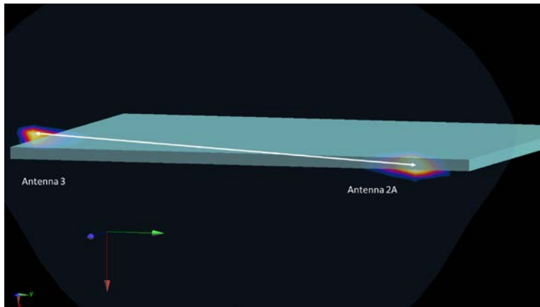
Figure 11-25 Right Edge Spatial Separation for Antenna 3 and Antenna 2A
