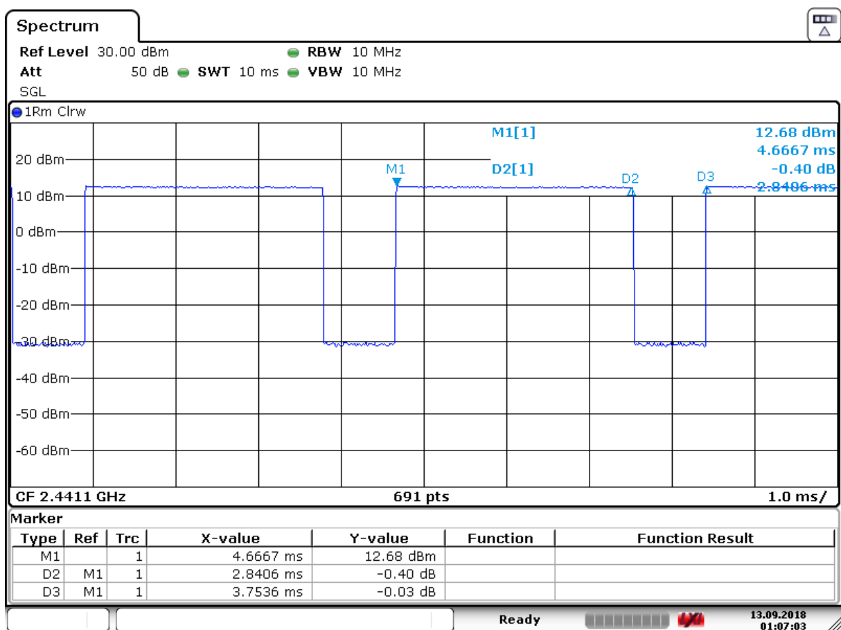
Figure 8-7 Bluetooth Transmission Plot & Duty Cycle Calculation – Ant 5 Variant 1
