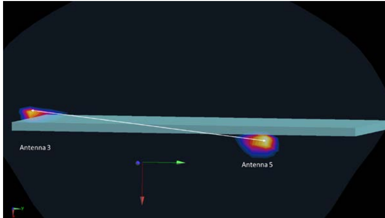
Figure 11-24 Right Edge Spatial Separation for Antenna 3 and Antenna 5
