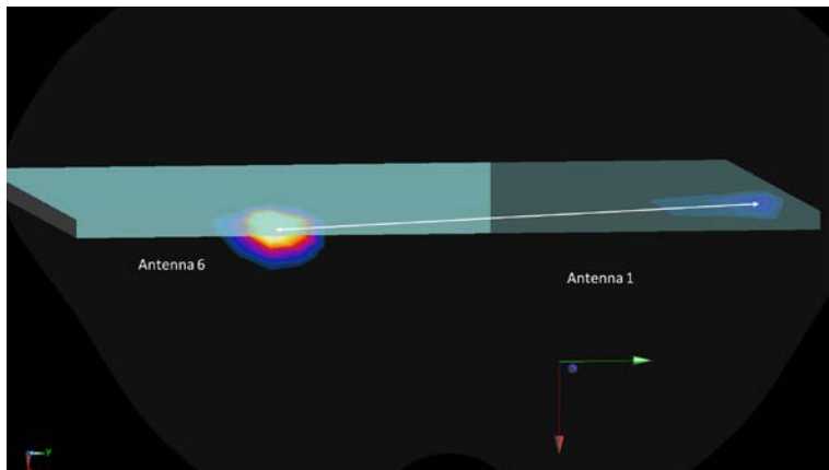
Figure 11-26 Right Edge Spatial Separation for Antenna 1 and Antenna 6
