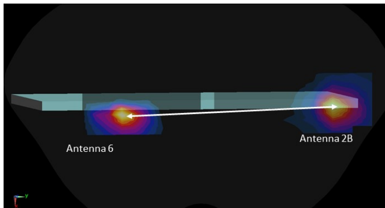
Figure 11-28 Right Edge Spatial Separation for Antenna 2B and Antenna 6
