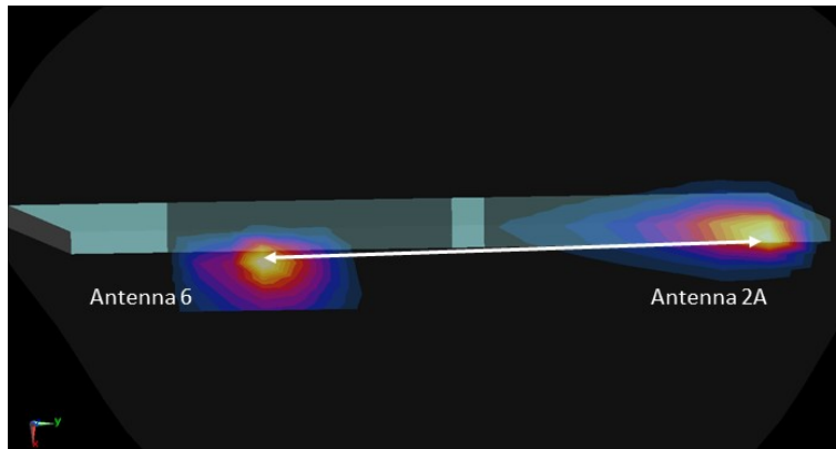
Figure 11-27 Right Edge Spatial Separation for Antenna 2A and Antenna 6
