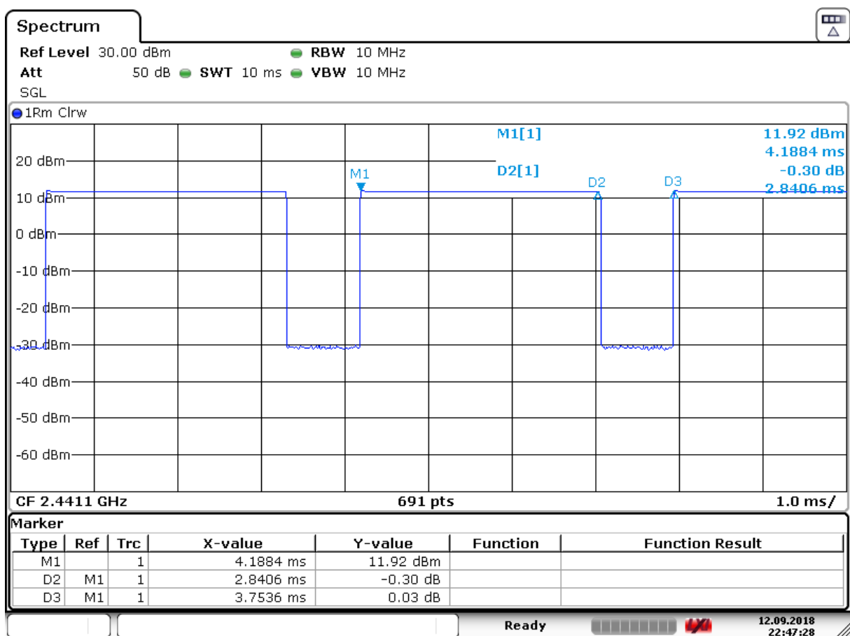
Figure 8-9 Bluetooth Transmission Plot & Duty Cycle Calculation – Ant 2a Variant 2
