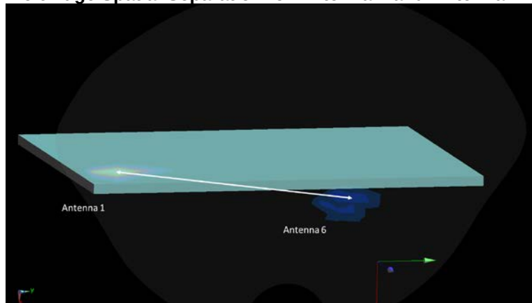
Figure 11-31 Left Edge Spatial Separation for Antenna 1 and Antenna 6
