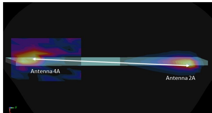
Figure 11-20 Right Edge Spatial Separation for Antenna 4A and Antenna 2A
