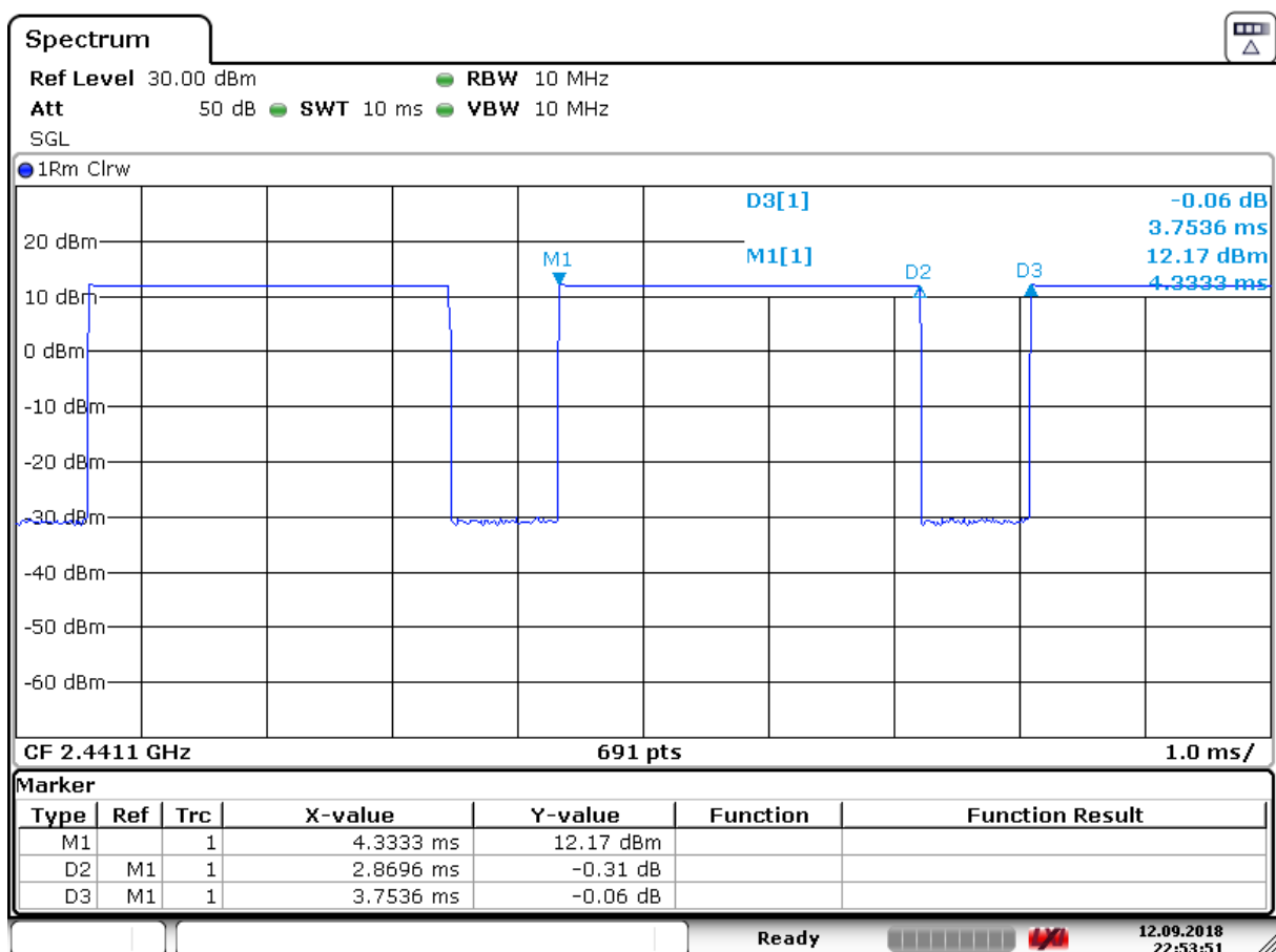
Figure 8-8 Bluetooth Transmission Plot & Duty Cycle Calculation – Ant 4a Variant 2
