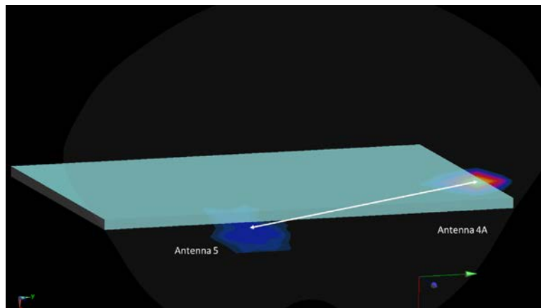
Figure 11-32 Left Edge Spatial Separation for Antenna 4A and Antenna 5
