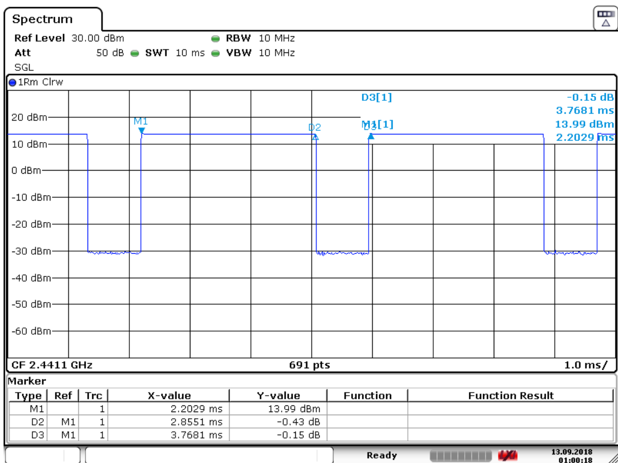
Figure 8-6 Bluetooth Transmission Plot & Duty Cycle Calculation – Ant 2a Variant 1
