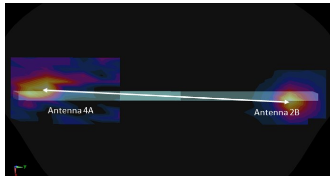
Figure 11-19 Right Edge Spatial Separation for Antenna 4A and Antenna 2B
