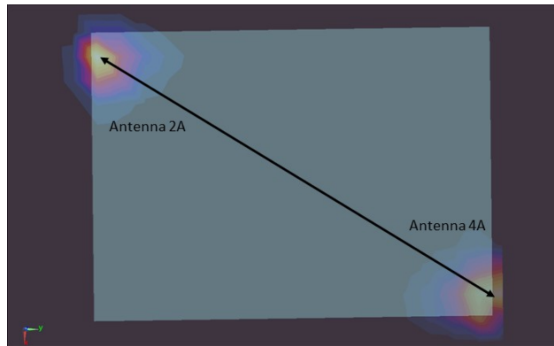
Figure 11-3 Back Side Spatial Separation for Antenna 4A and Antenna 2A
