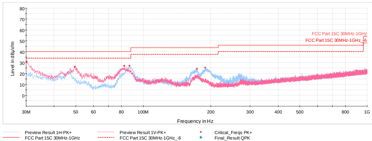
Plot 7-4. Radiated Spurious Plot above 30MHz (Pol. H & V)
