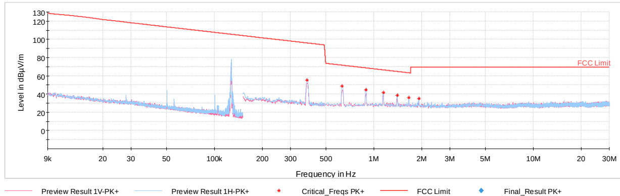
Plot 7-3. Radiated Spurious Plot from 9kHz – 30MHz (Loop Antenna X & Y)
