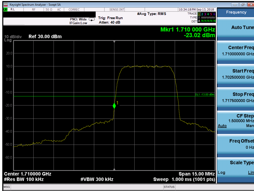
Plot 7-59. Band Edge Plot (AWS WCDMA Mode - Low Channel)
