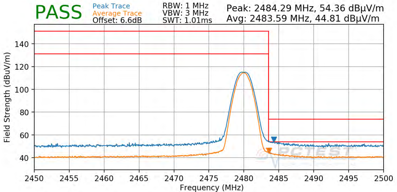
Plot 7-96. Radiated Restricted Upper Band Edge Measurement ANT1 (Average & Peak)
