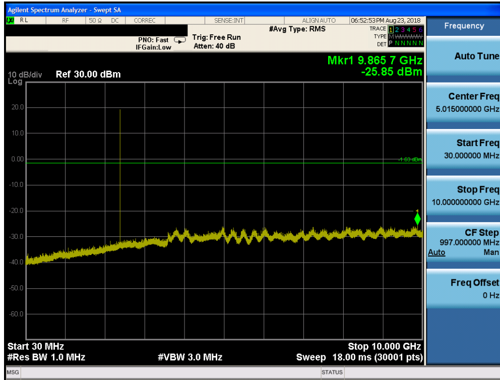
Plot 7-61. Conducted Spurious Plot ANT0 (Bluetooth (LE), 1Mbps, ePA – Ch. 0)
