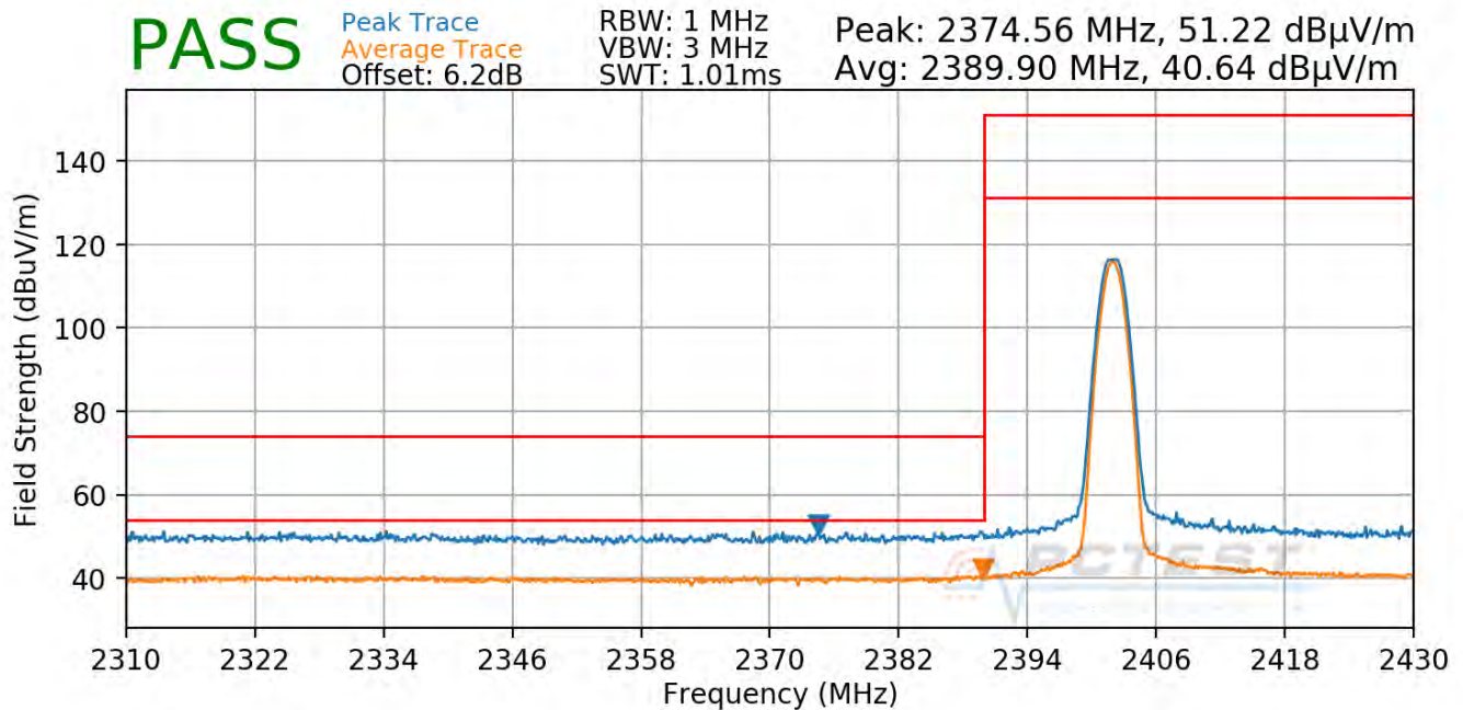
Plot 7-91. Radiated Restricted Lower Band Edge Measurement ANT0 (Average & Peak)
