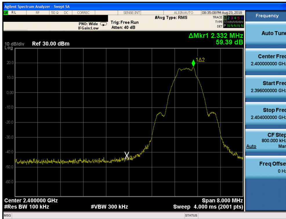
Plot 7-57. Band Edge Plot ANT1 (Bluetooth (LE), ePA – Ch. 0)
