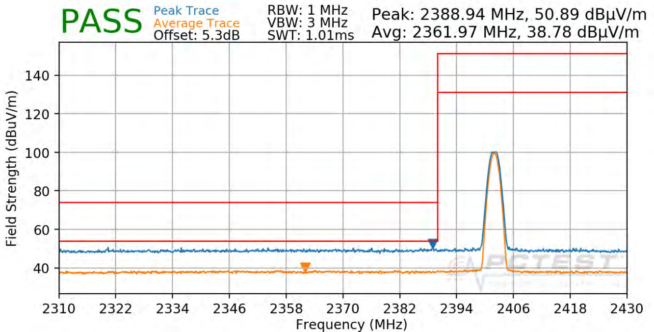
Plot 7-99. Radiated Restricted Lower Band Edge Measurement ANT2 (Average & Peak)
