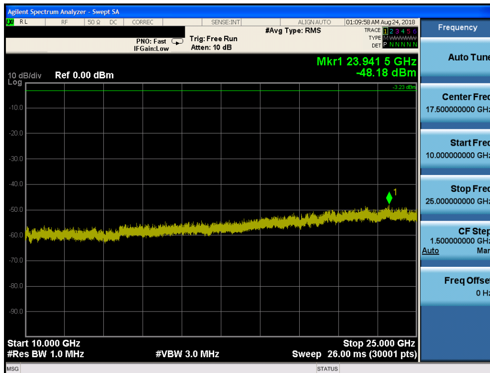
Plot 7-74. Conducted Spurious Plot ANT2 (Bluetooth (LE), 1Mbps, ePA – Ch. 0)
