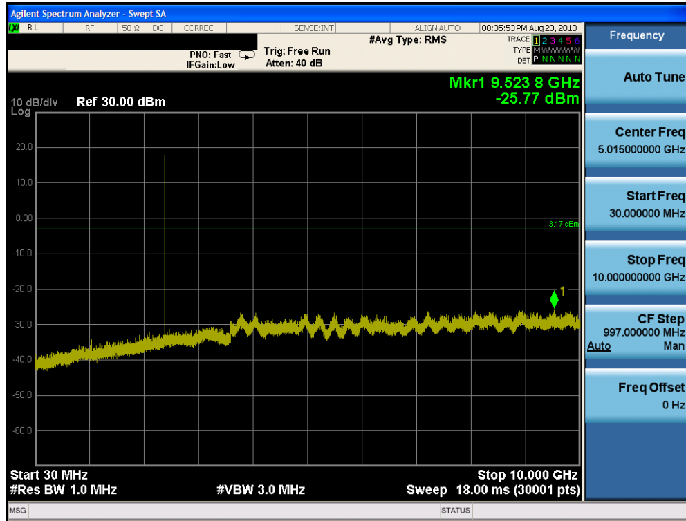
Plot 7-67. Conducted Spurious Plot ANT1 (Bluetooth (LE), 1Mbps, ePA – Ch. 0)
