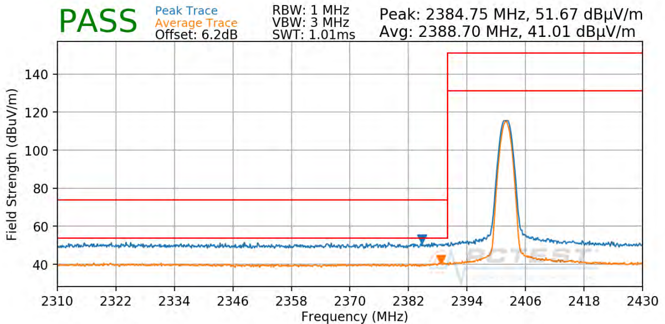
Plot 7-94. Radiated Restricted Lower Band Edge Measurement ANT1 (Average & Peak)
