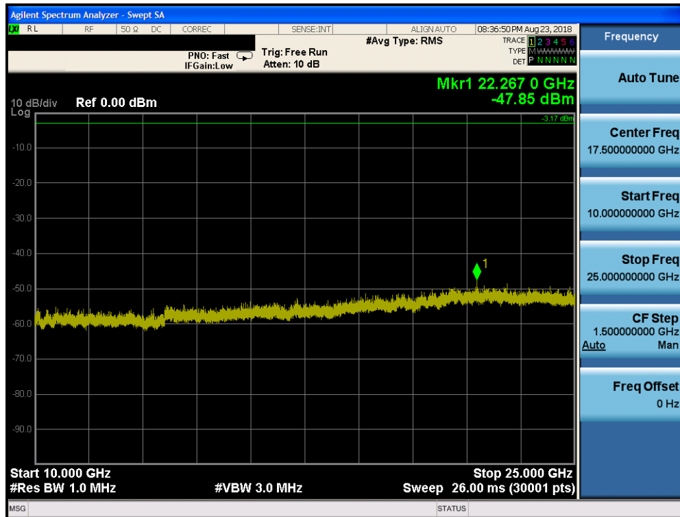
Plot 7-68. Conducted Spurious Plot ANT1 (Bluetooth (LE), 1Mbps, ePA – Ch. 0)
