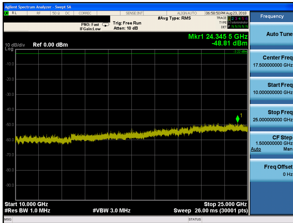
Plot 7-66. Conducted Spurious Plot ANT0 (Bluetooth (LE), 1Mbps, ePA – Ch. 39)
