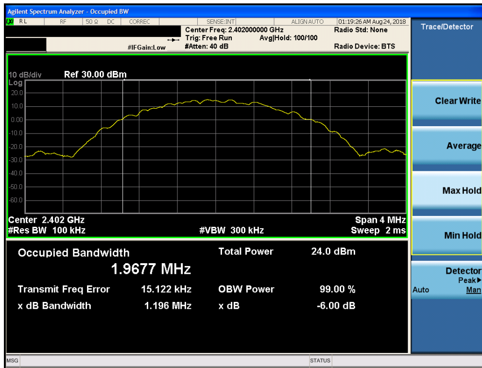
Plot 7-16. 6dB Bandwidth Plot ANT2 (Bluetooth (LE), 2Mbps, ePA – Ch. 0)
