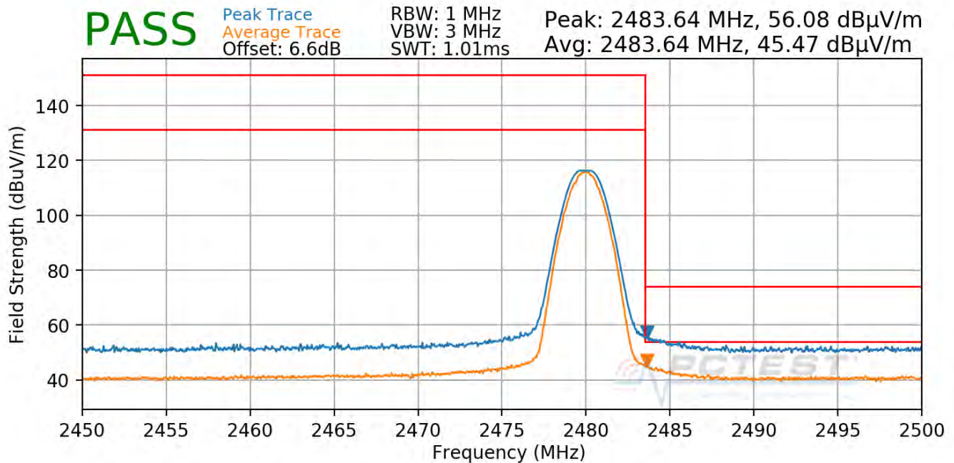
Plot 7-93. Radiated Restricted Upper Band Edge Measurement ANT0 (Average & Peak)
