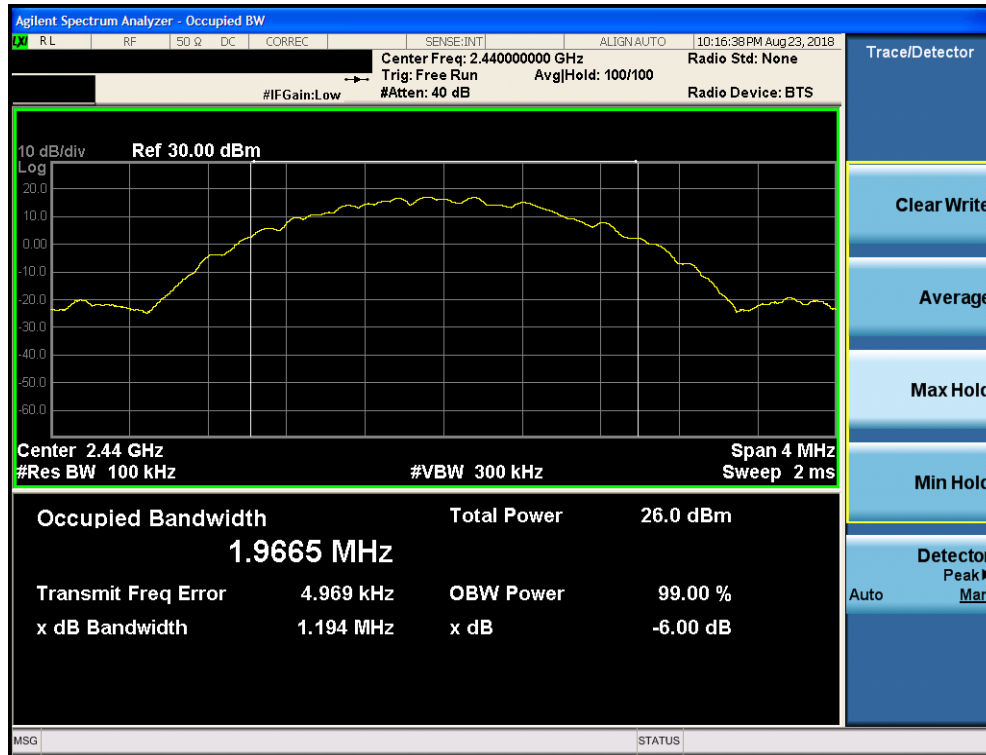
Plot 7-11. 6dB Bandwidth Plot ANT1 (Bluetooth (LE), 2Mbps, ePA – Ch. 19)
