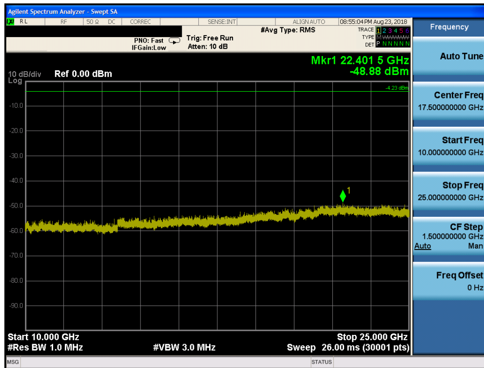
Plot 7-72. Conducted Spurious Plot ANT1 (Bluetooth (LE), 1Mbps, ePA – Ch. 39)
