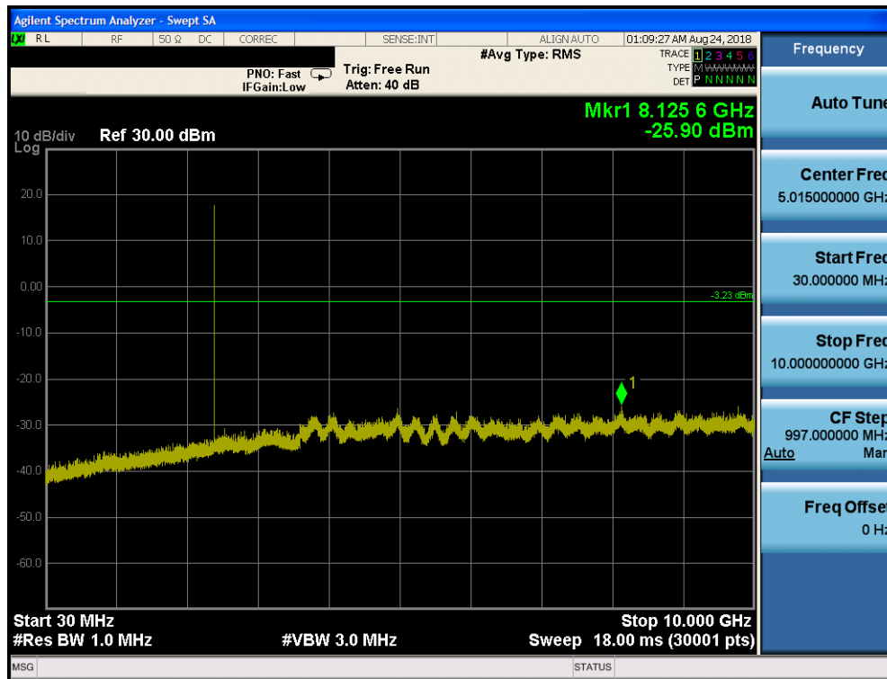
Plot 7-73. Conducted Spurious Plot ANT2 (Bluetooth (LE), 1Mbps, ePA – Ch. 0)
