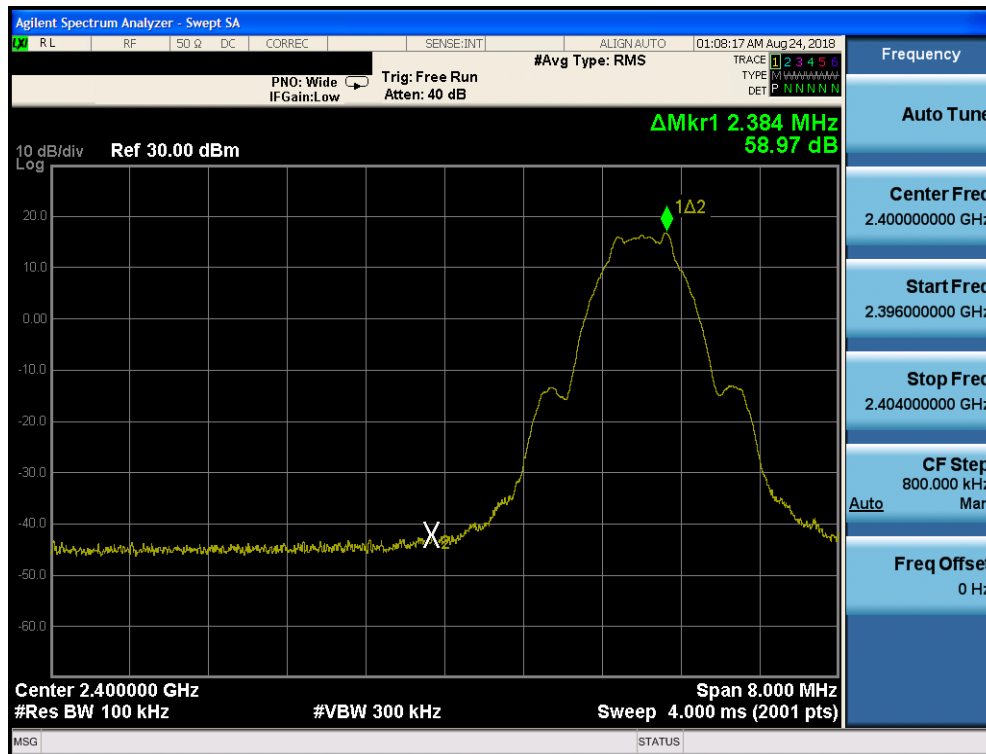
Plot 7-59. Band Edge Plot ANT2 (Bluetooth (LE), ePA – Ch. 0)
