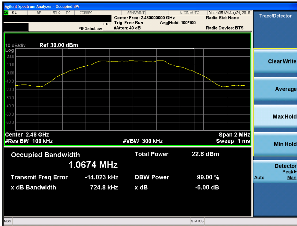
Plot 7-15. 6dB Bandwidth Plot ANT2 (Bluetooth (LE), 1Mbps, ePA – Ch. 39)
