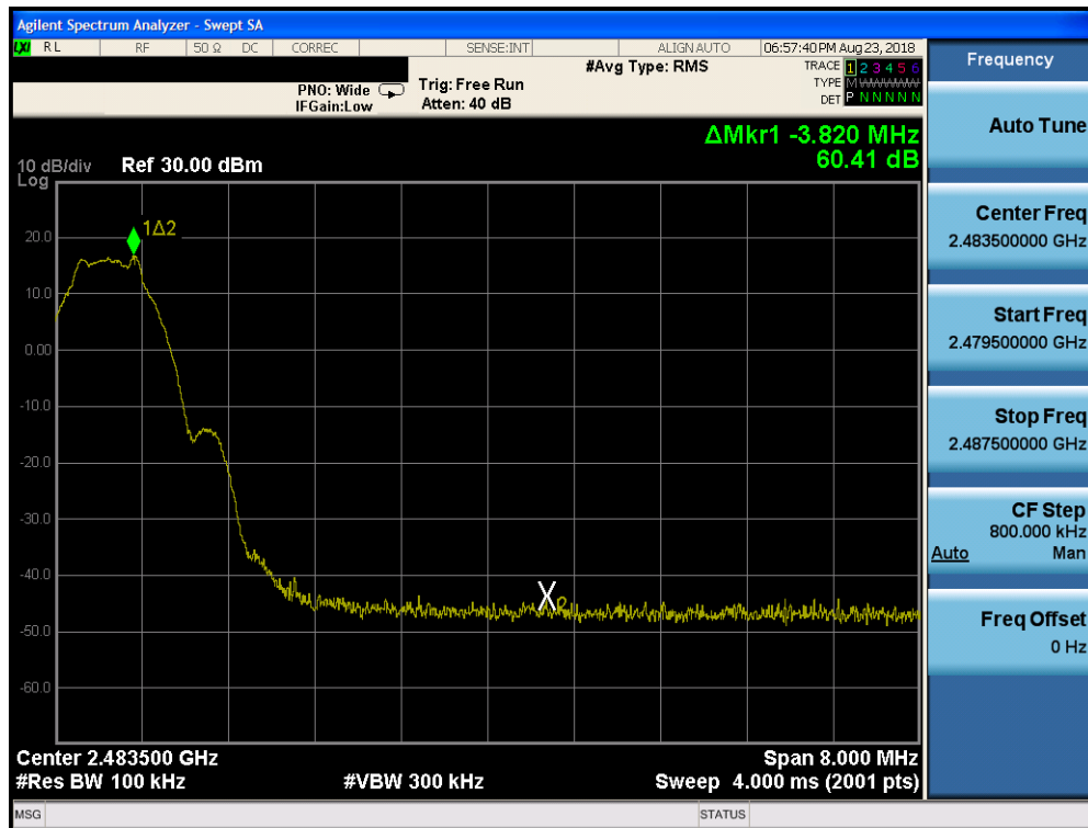
Plot 7-56. Band Edge Plot ANT0 (Bluetooth (LE), ePA - Ch. 39)
