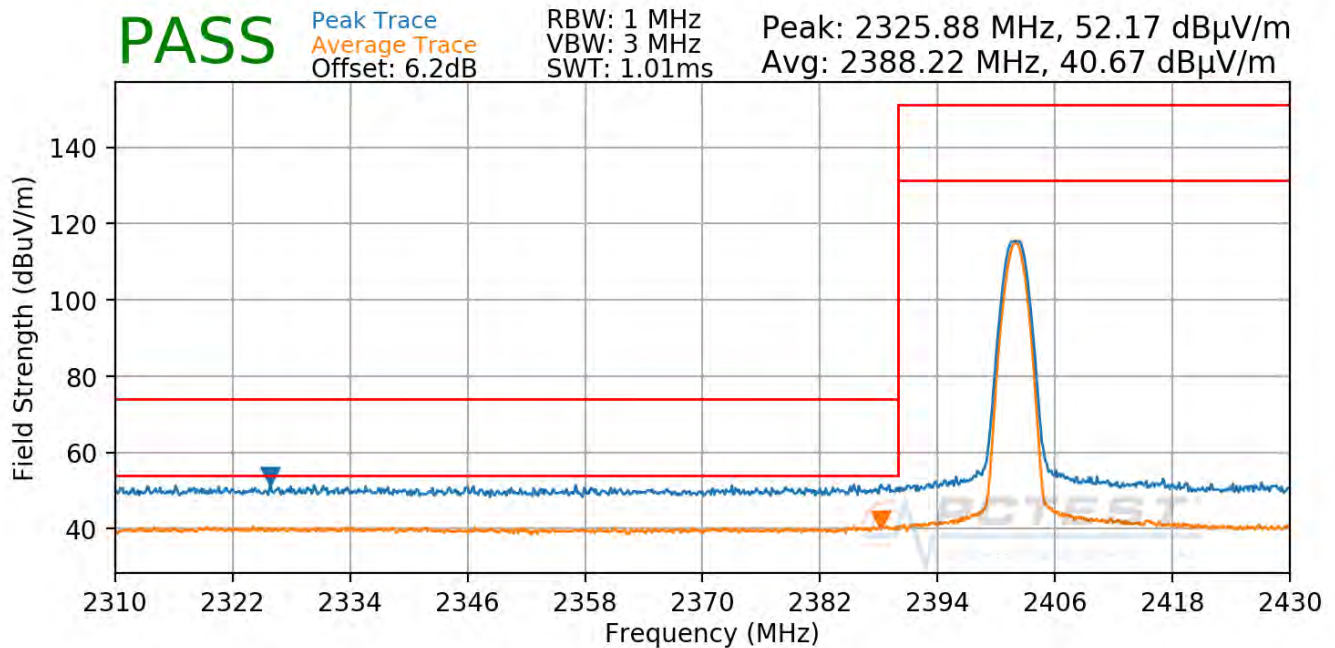
Plot 7-95. Radiated Restricted Lower Band Edge Measurement ANT1 (Average & Peak)
