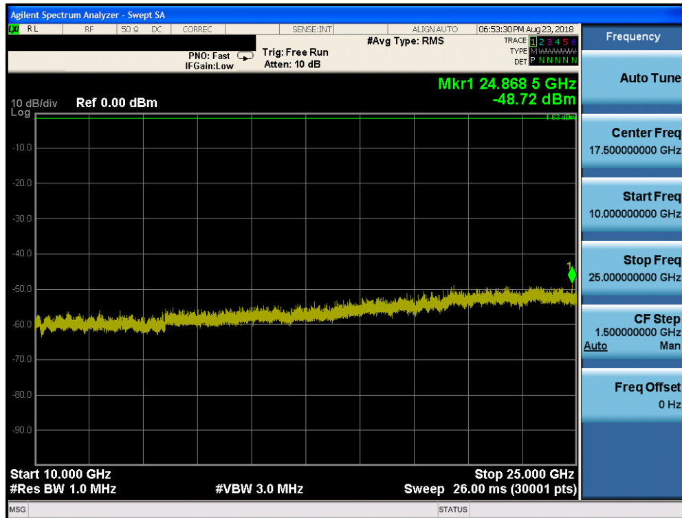
Plot 7-62. Conducted Spurious Plot ANT0 (Bluetooth (LE), 1Mbps, ePA – Ch. 0)
