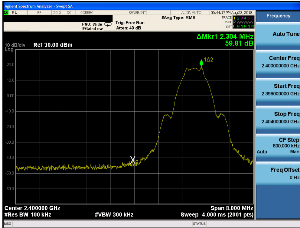
Plot 7-55. Band Edge Plot ANT0 (Bluetooth (LE), ePA - Ch. 0)
