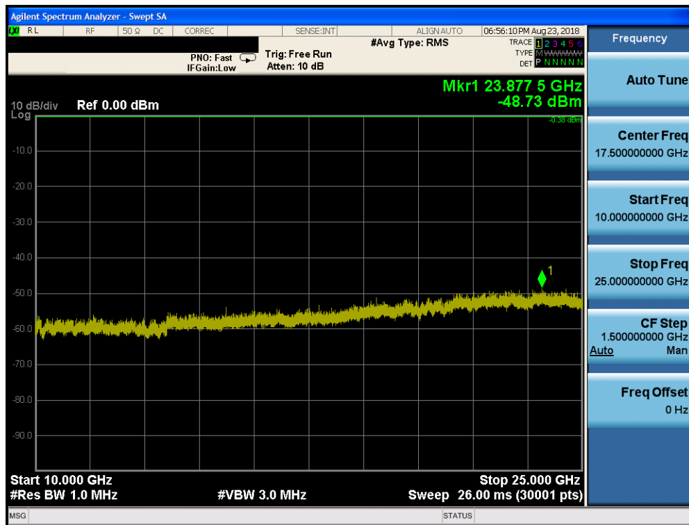
Plot 7-64. Conducted Spurious Plot ANT0 (Bluetooth (LE), 1Mbps, ePA – Ch. 19)
