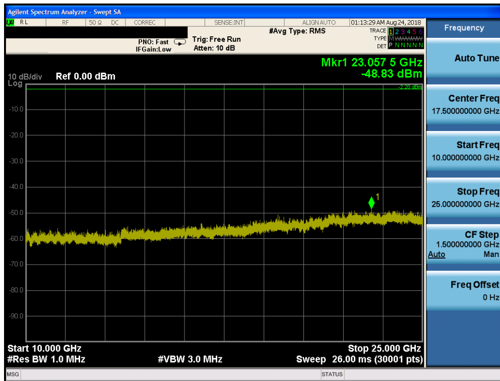
Plot 7-76. Conducted Spurious Plot ANT2 (Bluetooth (LE), 1Mbps, ePA – Ch. 19)
