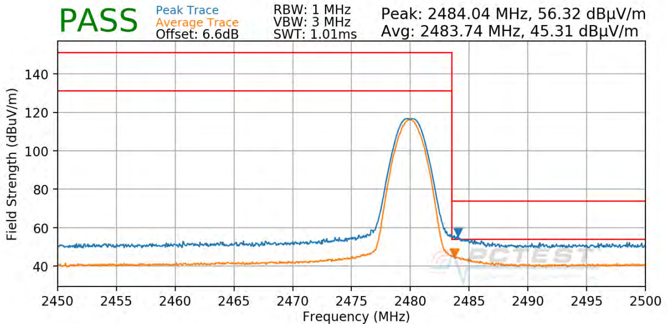
Plot 7-92. Radiated Restricted Upper Band Edge Measurement ANT0 (Average & Peak)
