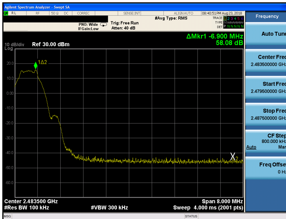
Plot 7-58. Band Edge Plot ANT1 (Bluetooth (LE), ePA – Ch. 39)
