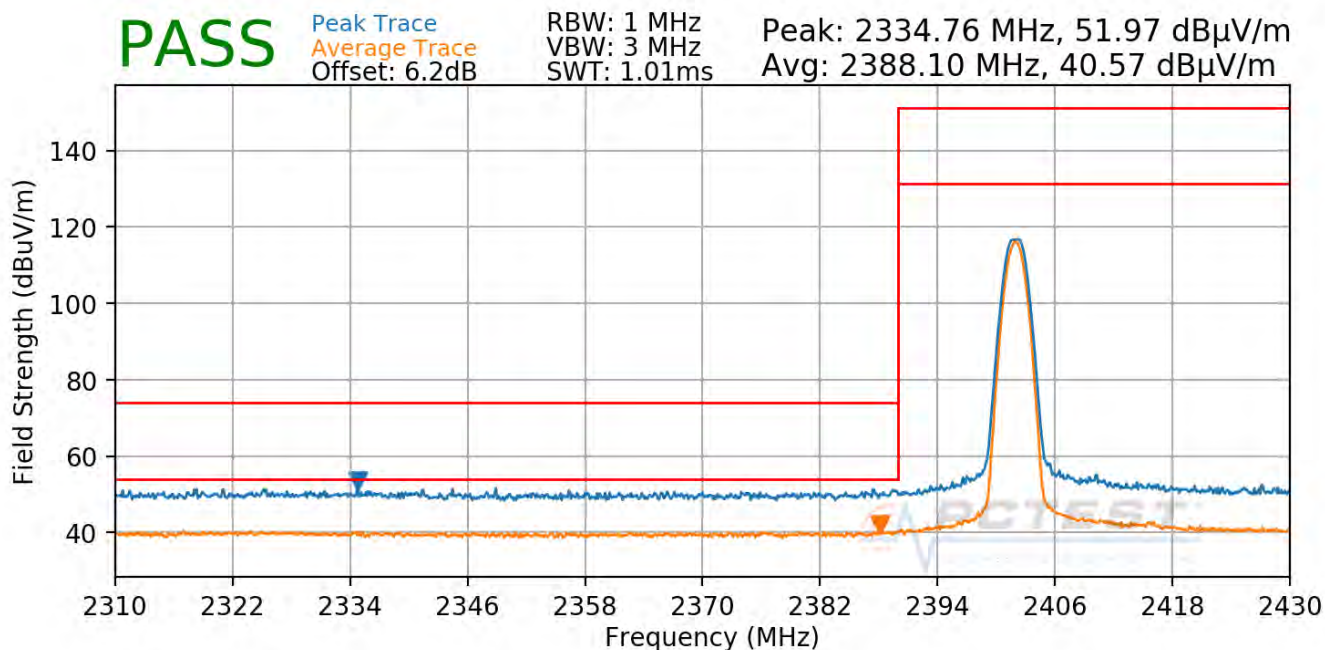
Plot 7-90. Radiated Restricted Lower Band Edge Measurement ANT0 (Average & Peak)
