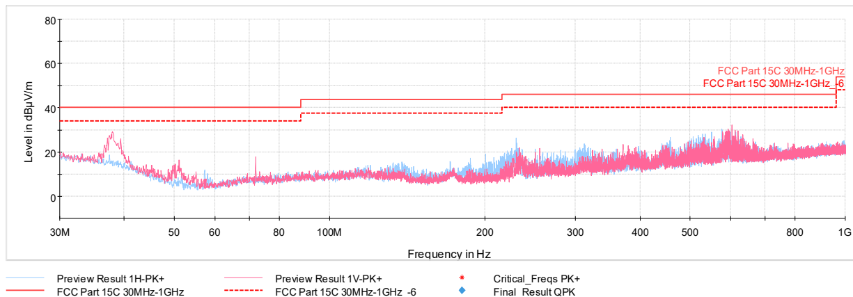
Plot 7-102. Radiated Spurious Plot below 1GHz (1Mbps, ePA, Pol. H & V, with Laptop)
