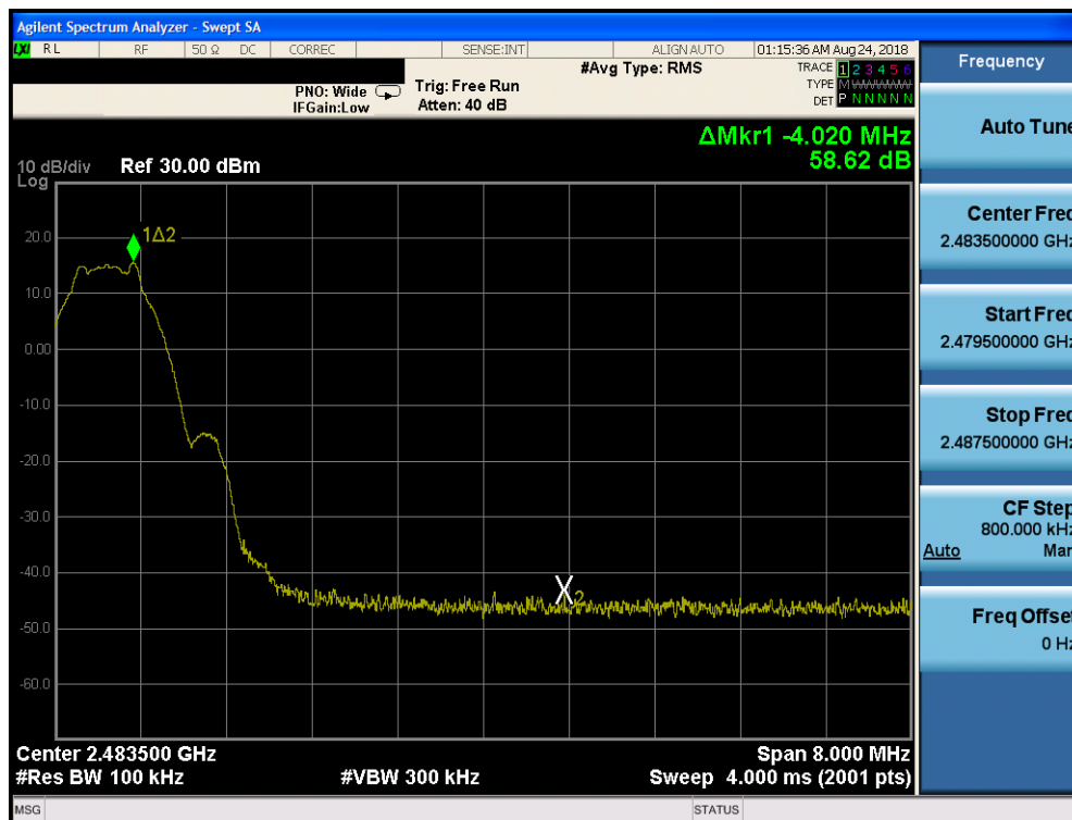
Plot 7-60. Band Edge Plot ANT2 (Bluetooth (LE), ePA – Ch. 39)
