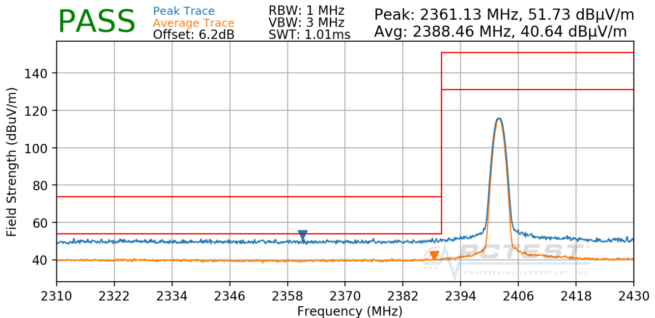
Plot 7-105. Radiated Restricted Lower Band Edge Measurement ANT1 (Average & Peak)
