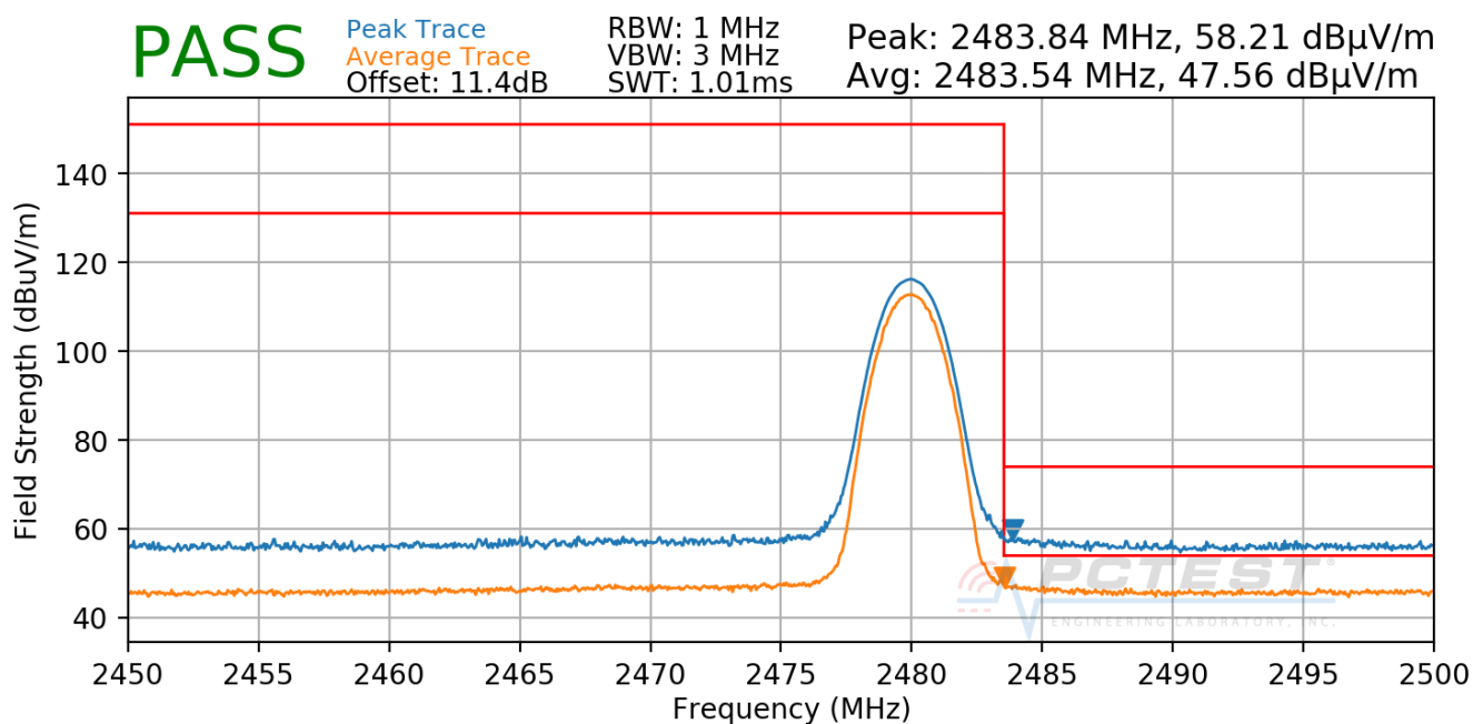
Plot 7-104. Radiated Restricted Upper Band Edge Measurement ANT0 (Average & Peak)
