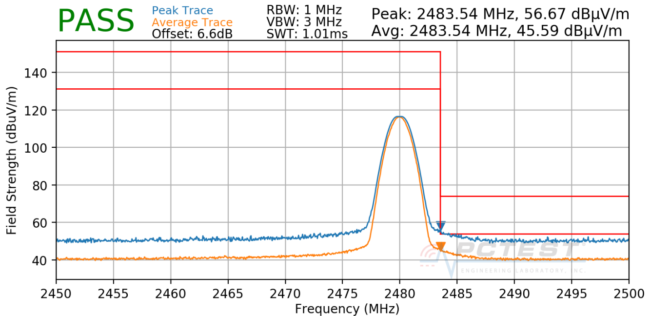
Plot 7-103. Radiated Restricted Upper Band Edge Measurement ANT0 (Average & Peak)
