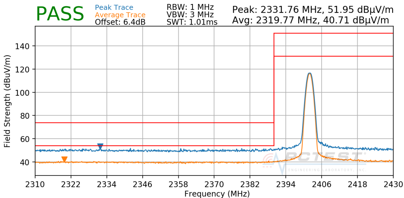
Plot 7-101. Radiated Restricted Lower Band Edge Measurement ANT0 (Average & Peak)
