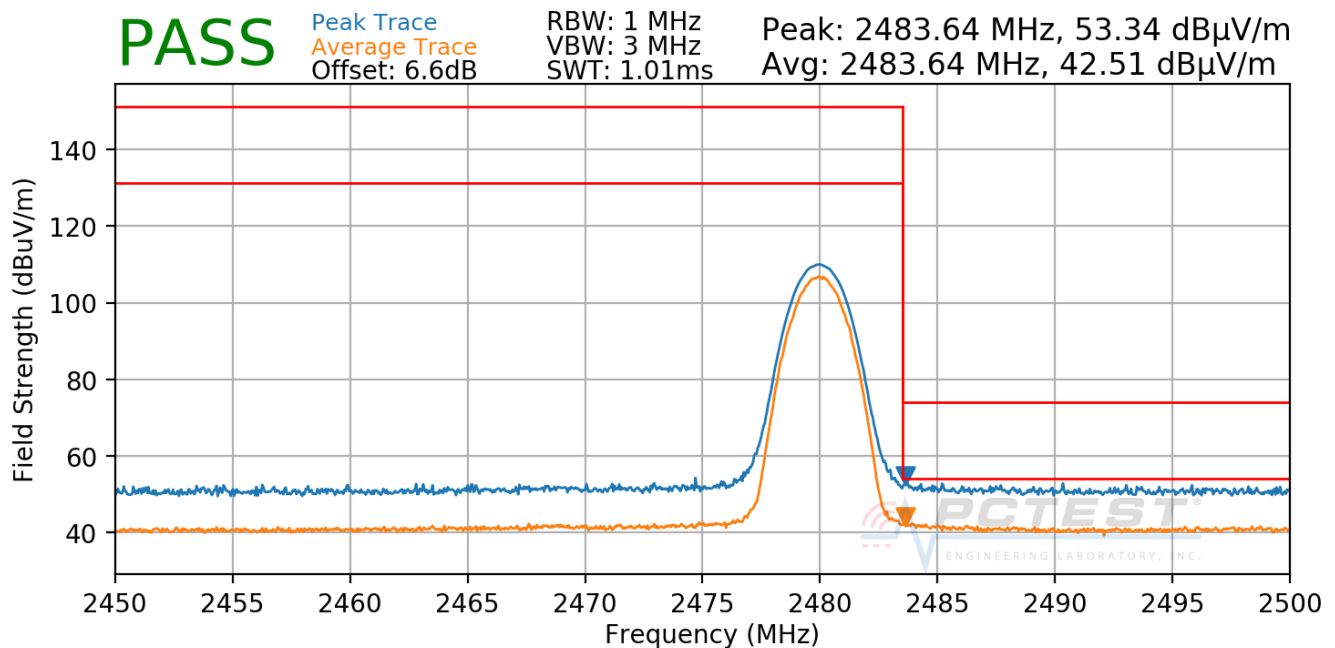
Plot 7-108. Radiated Restricted Upper Band Edge Measurement ANT1 (Average & Peak)
