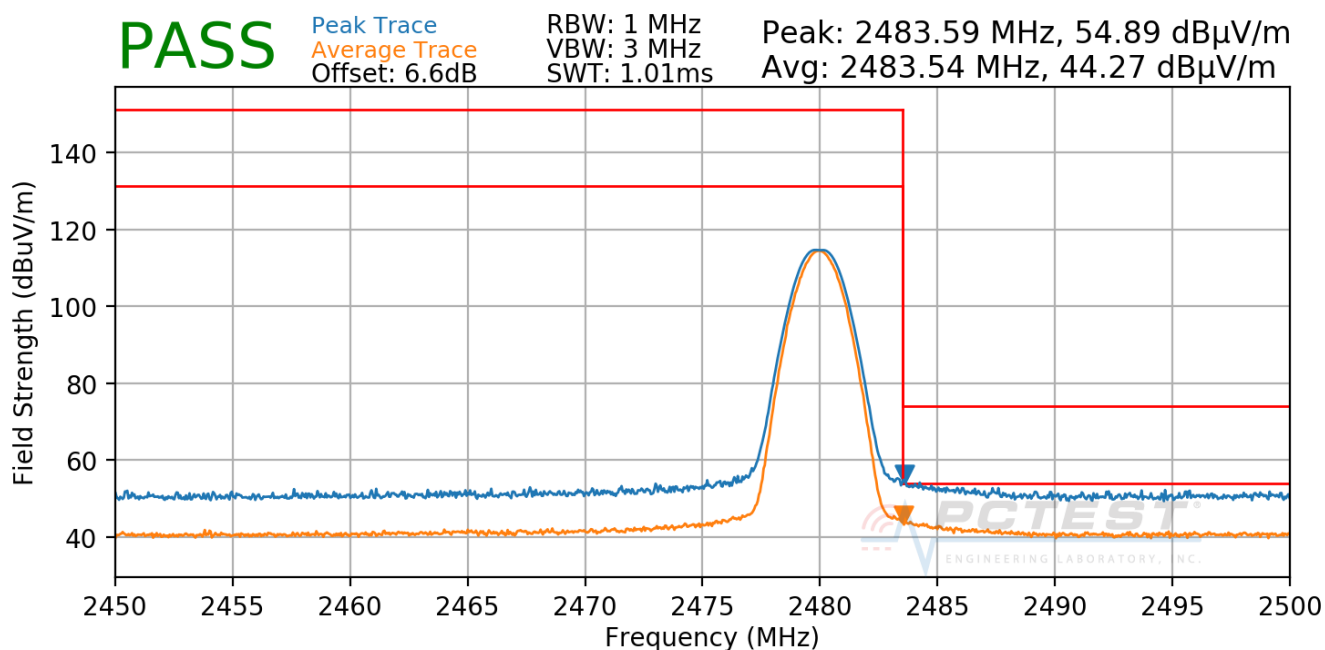
Plot 7-107. Radiated Restricted Upper Band Edge Measurement ANT1 (Average & Peak)
