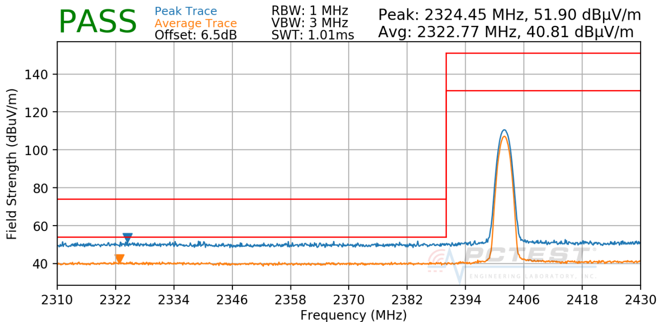
Plot 7-102. Radiated Restricted Lower Band Edge Measurement ANT0 (Average & Peak)
