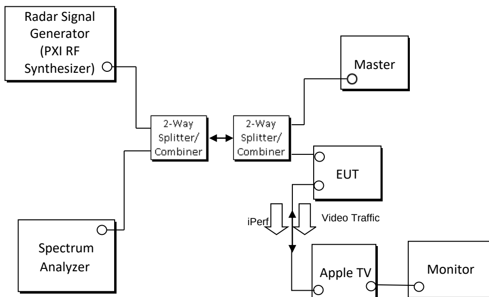
Figure 5-3. Test Setup (Mode 3)
