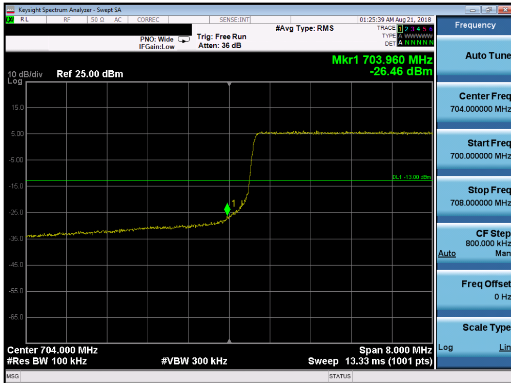
Plot 7-202. Lower Band Edge Plot (Band 17 – 10.0MHz QPSK – RB Size 50)
