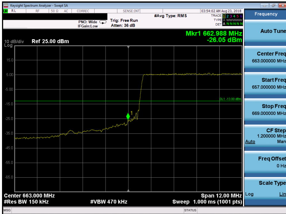
Plot 7-188. Lower Band Edge Plot (Band 71 - 15.0MHz QPSK - RB Size 75)
