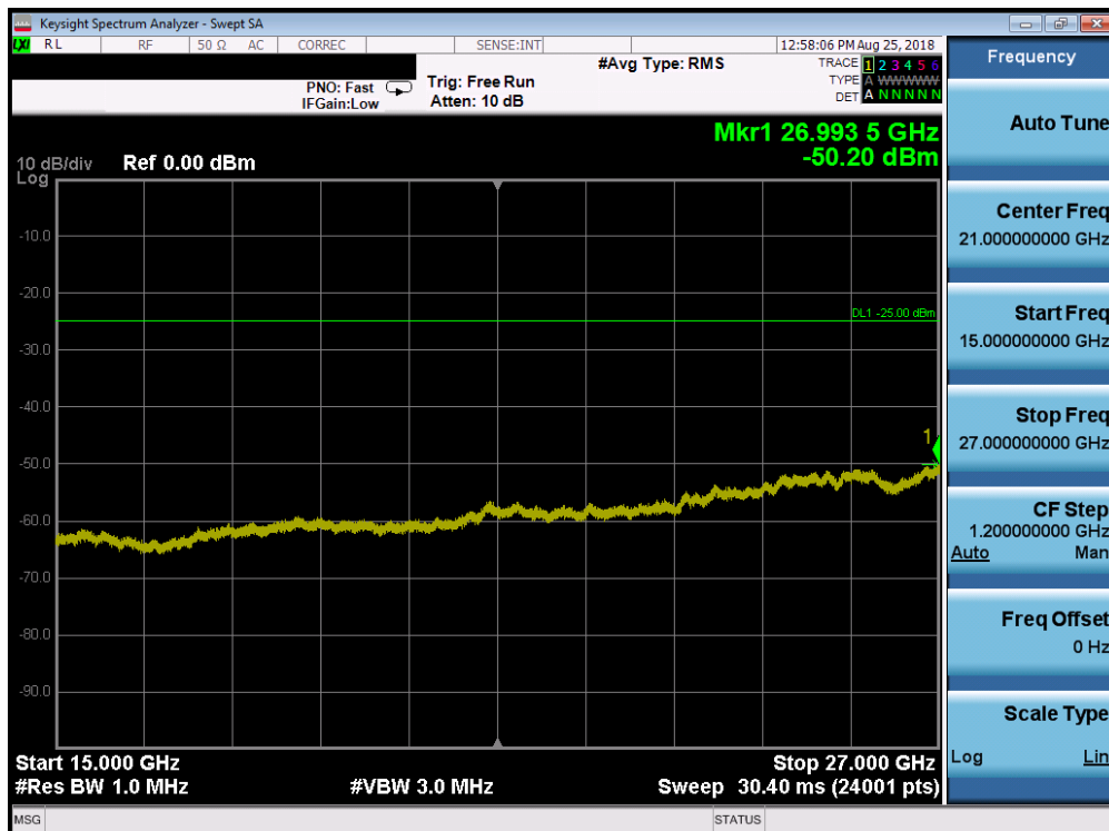
Plot 7-171. Conducted Spurious Plot (Band 7 – 20.0MHz QPSK – RB Size 1, RB Offset 0 – Mid Channel)
