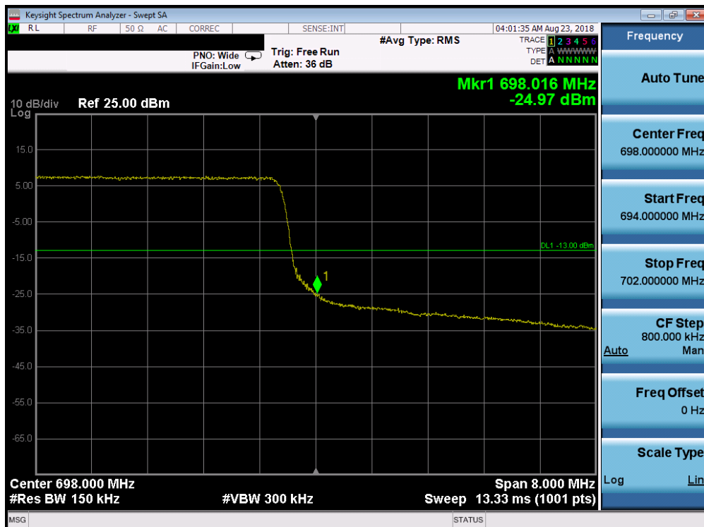
Plot 7-187. Upper Band Edge Plot (Band 71 - 10.0MHz QPSK - RB Size 50)
