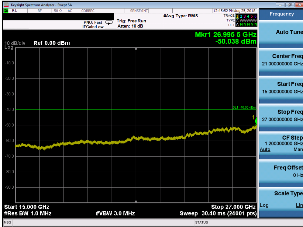
Plot 7-165. Conducted Spurious Plot (Band 30 – 10.0MHz QPSK – RB Size 1, RB Offset 0 – Mid Channel)
