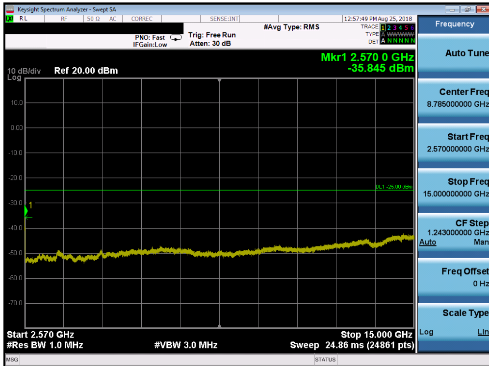
Plot 7-170. Conducted Spurious Plot (Band 7 – 20.0MHz QPSK – RB Size 1, RB Offset 0 – Mid Channel)
