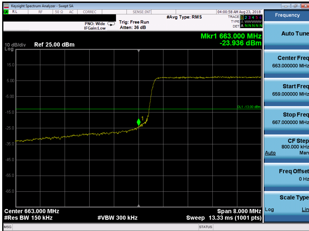
Plot 7-186. Lower Band Edge Plot (Band 71 - 10.0MHz QPSK - RB Size 50)
