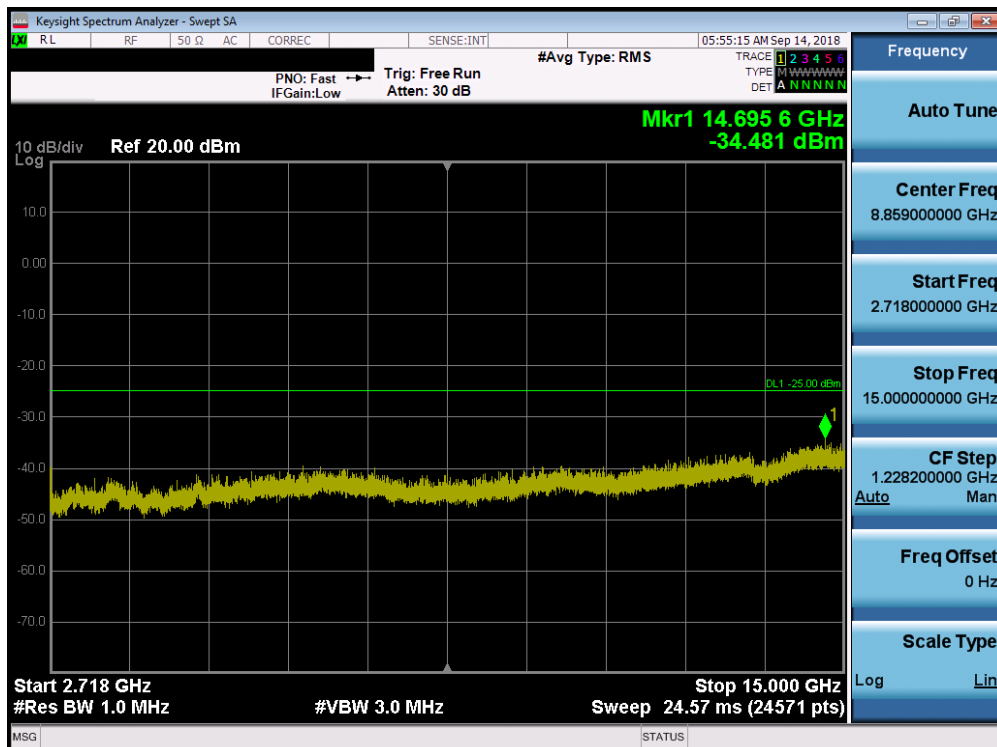
Plot 7-182. Conducted Spurious Plot (Band 41 – 20.0MHz QPSK – RB Size 1, RB Offset 0 – High Channel)
