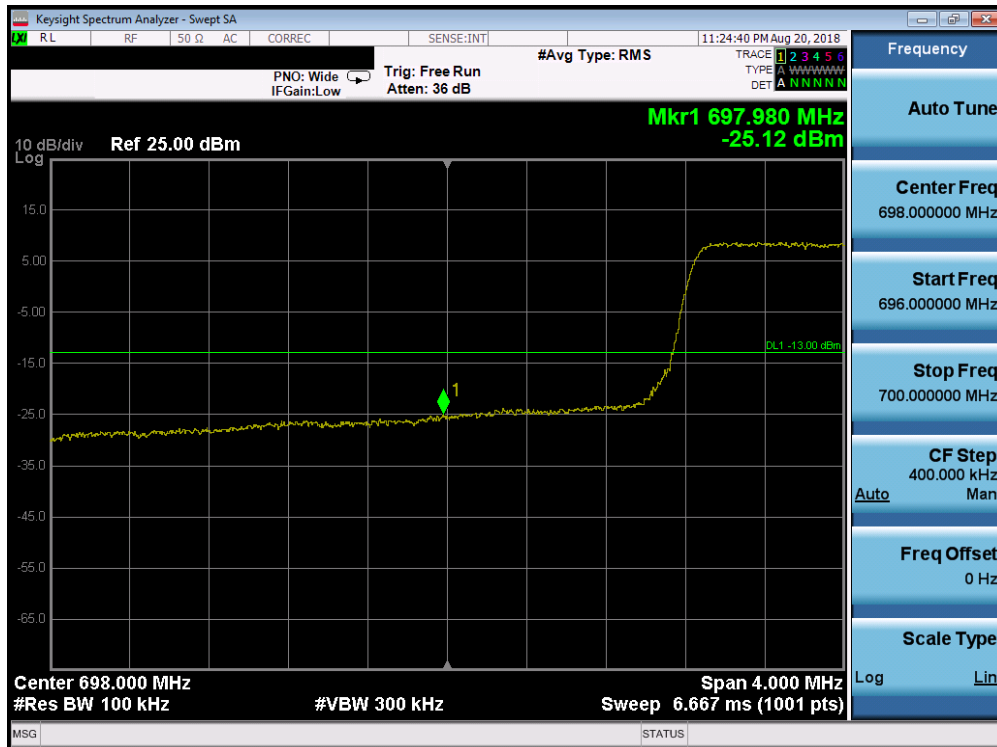
Plot 7-196. Lower Band Edge Plot (Band 12 – 5.0MHz QPSK – RB Size 25)
