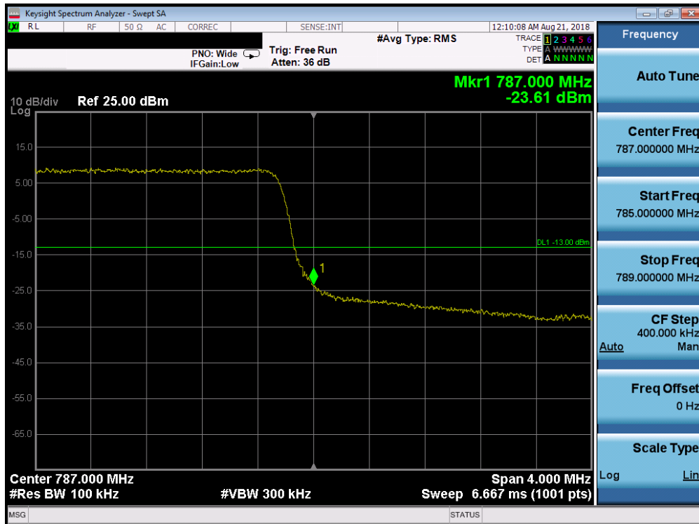
Plot 7-206. Upper Band Edge Plot (Band 13 – 5.0MHz QPSK – RB Size 25)
