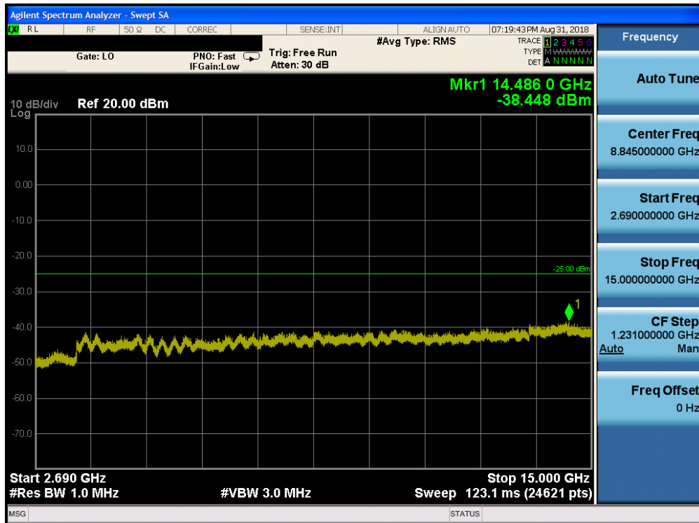
Plot 7-179. Conducted Spurious Plot (Band 41 – 20.0MHz QPSK – RB Size 1, RB Offset 0 – Mid Channel)
