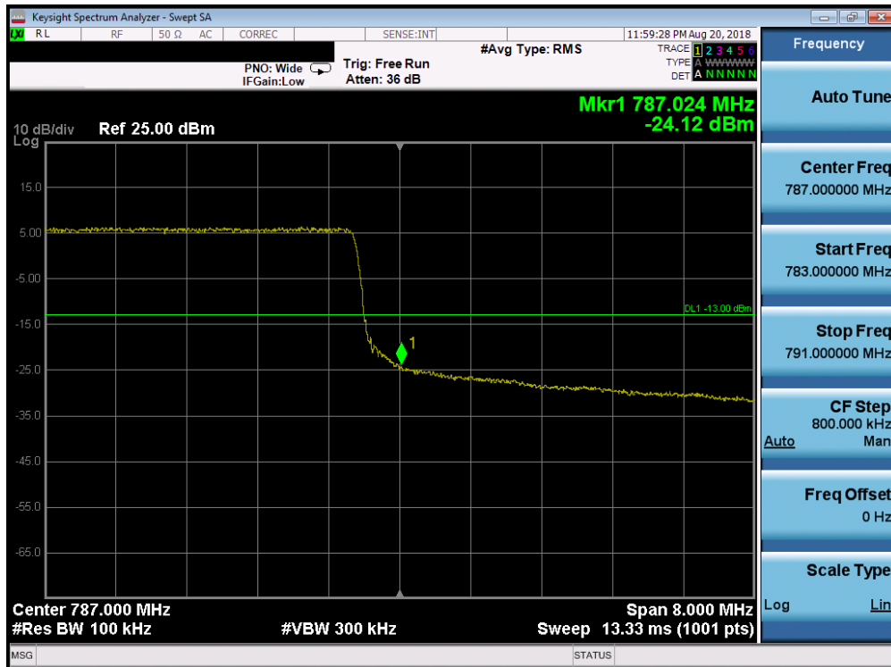
Plot 7-210. Upper Band Edge Plot (Band 13 – 10.0MHz QPSK – RB Size 50)
