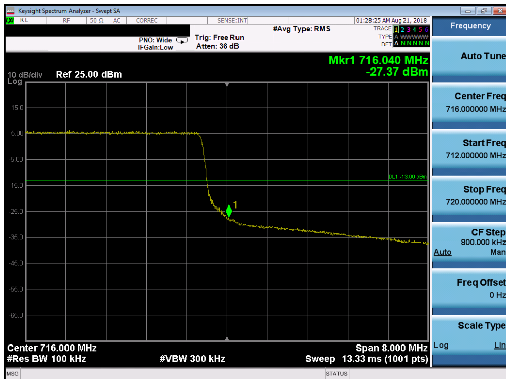
Plot 7-203. Upper Band Edge Plot (Band 17 – 10.0MHz QPSK – RB Size 50)
