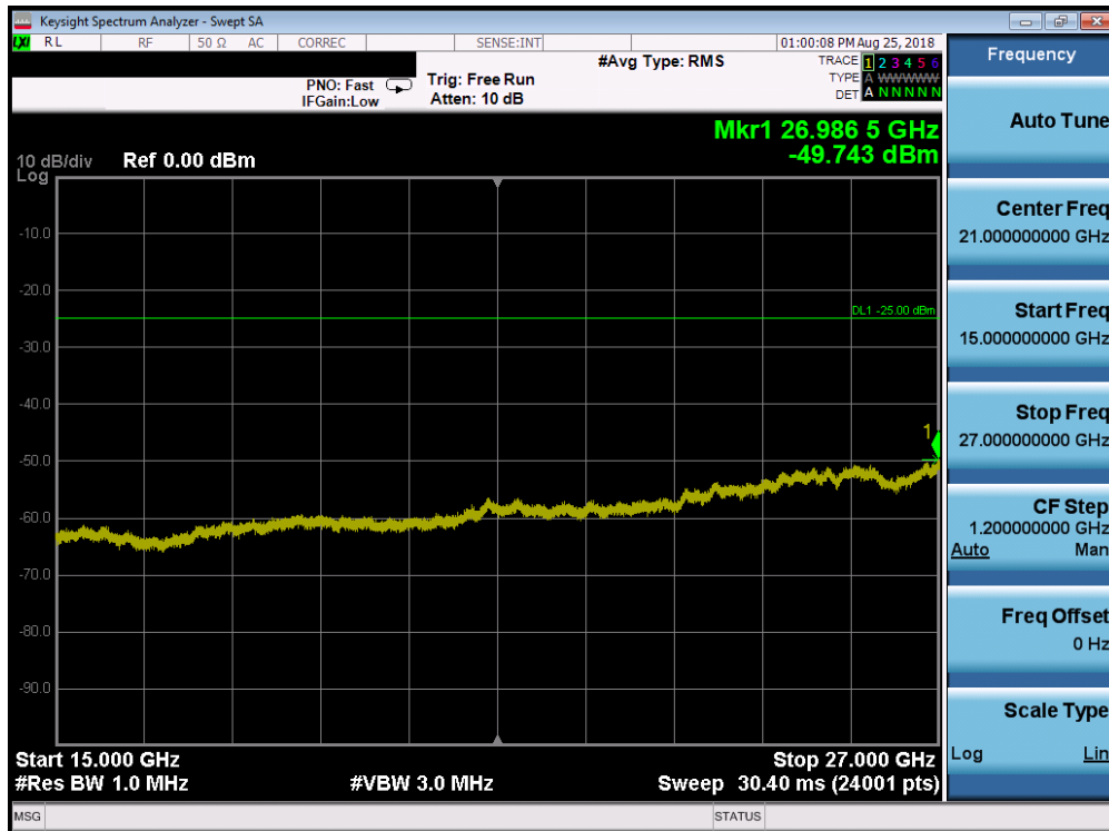
Plot 7-168. Conducted Spurious Plot (Band 7 – 20.0MHz QPSK – RB Size 1, RB Offset 0 – Low Channel)
