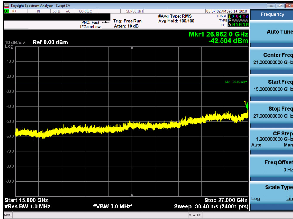
Plot 7-183. Conducted Spurious Plot (Band 41 – 20.0MHz QPSK – RB Size 1, RB Offset 0 – High Channel)
