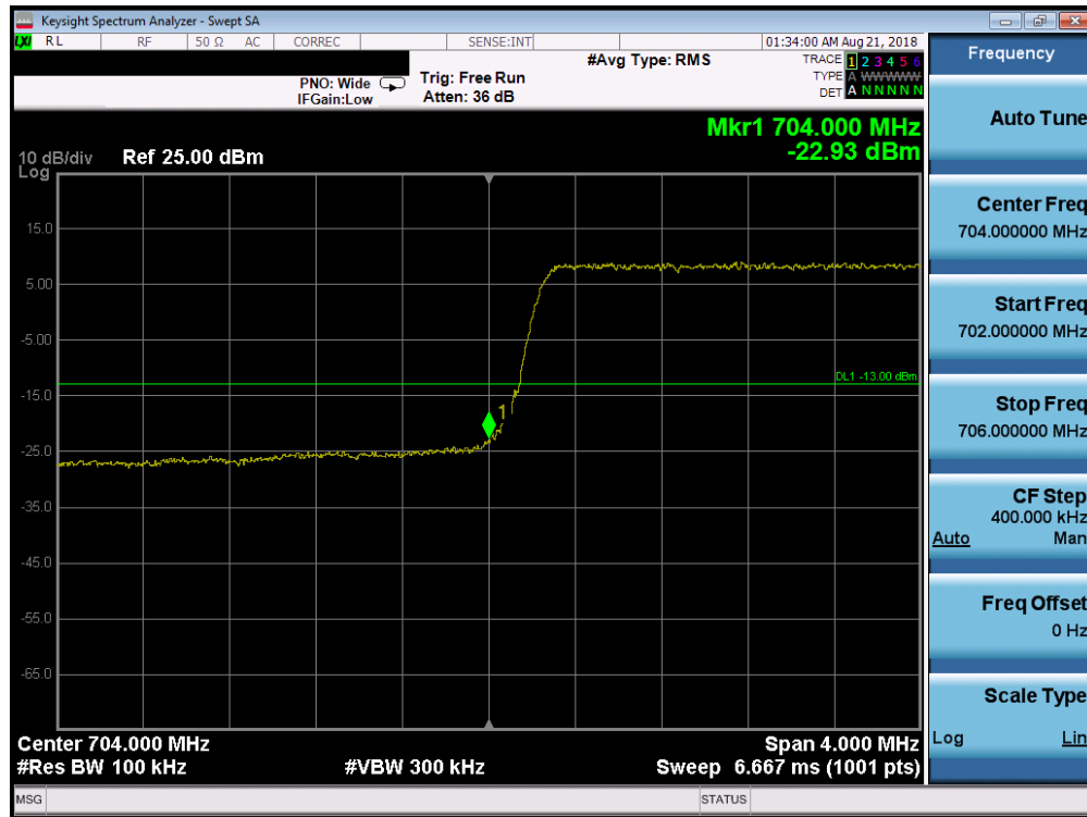
Plot 7-200. Lower Band Edge Plot (Band 17 – 5.0MHz QPSK – RB Size 25)
