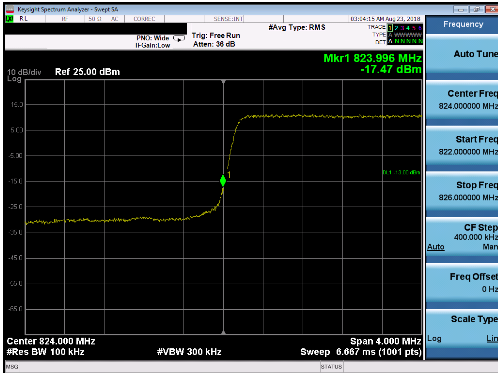
Plot 7-214. Lower Band Edge Plot (Band 5 - 3.0MHz QPSK - RB Size 15)
