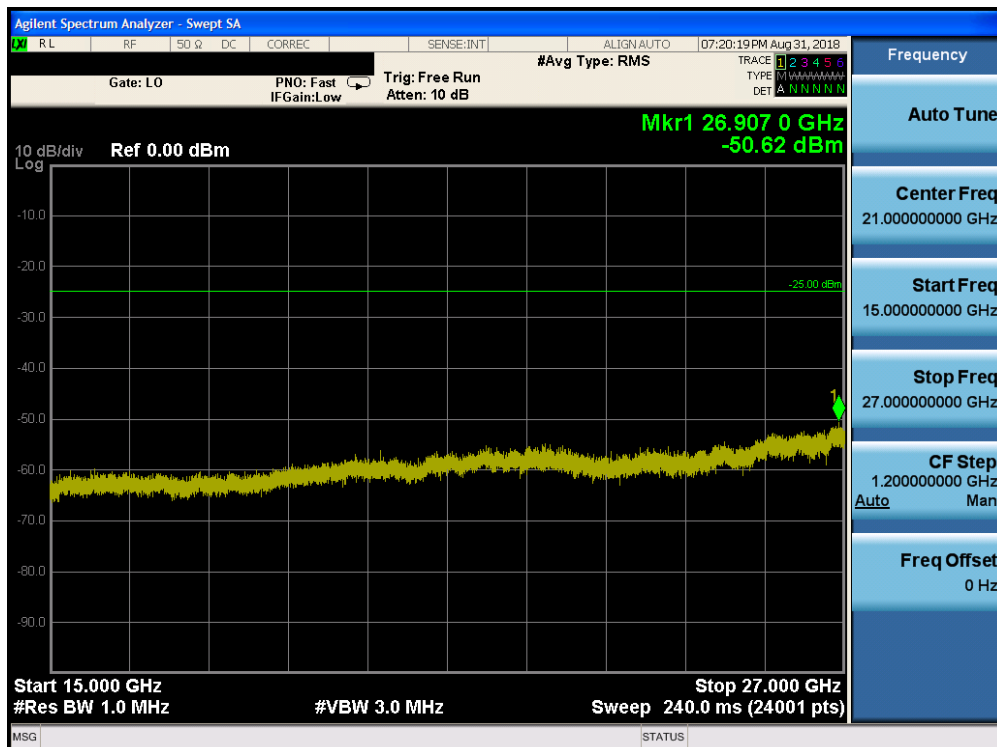
Plot 7-180. Conducted Spurious Plot (Band 41 – 20.0MHz QPSK – RB Size 1, RB Offset 0 – Mid Channel)
