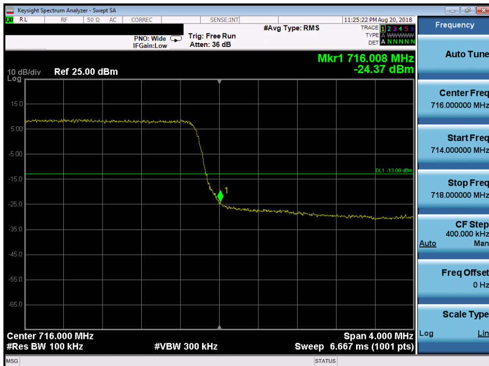
Plot 7-197. Upper Band Edge Plot (Band 12 – 5.0MHz QPSK – RB Size 25)
