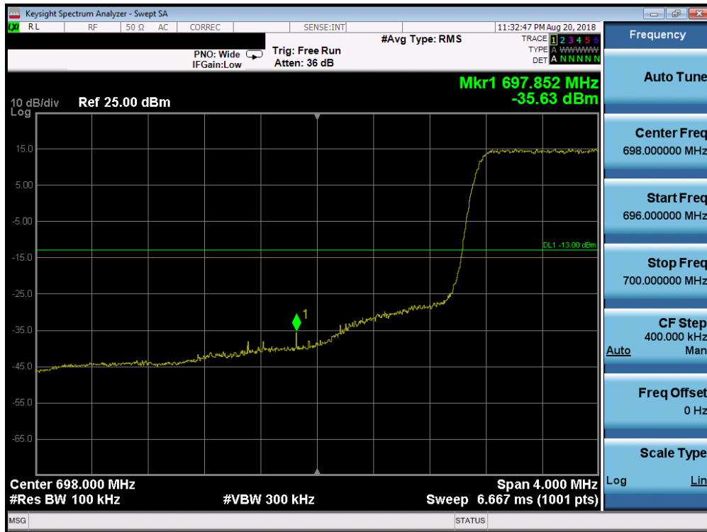
Plot 7-192. Lower Band Edge Plot (Band 12 – 1.4MHz QPSK – RB Size 6)
