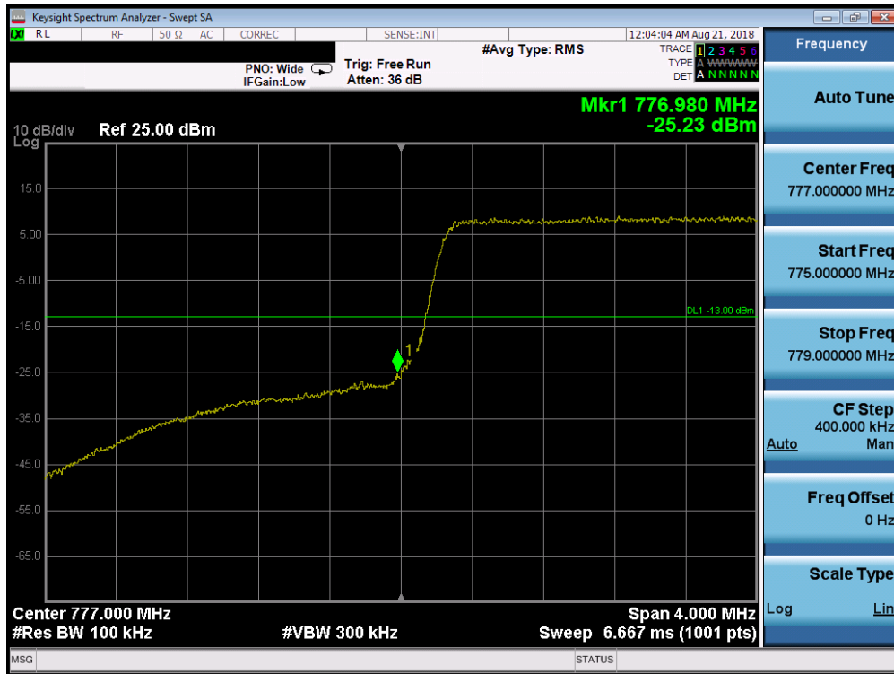
Plot 7-204. Lower Band Edge Plot (Band 13 – 5.0MHz QPSK – RB Size 25)
