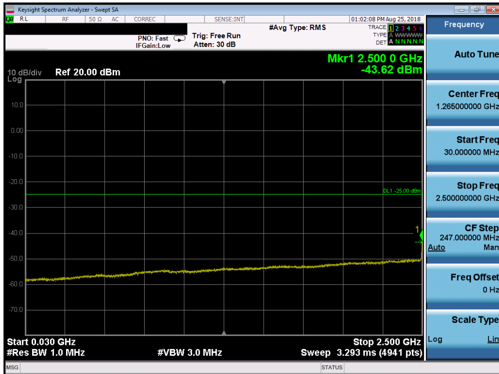
Plot 7-172. Conducted Spurious Plot (Band 7 – 20.0MHz QPSK – RB Size 1, RB Offset 0 – High Channel)
