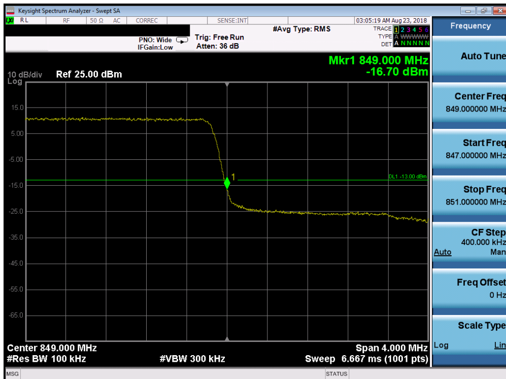
Plot 7-215. Upper Band Edge Plot (Band 5 - 3.0MHz QPSK - RB Size 15)
