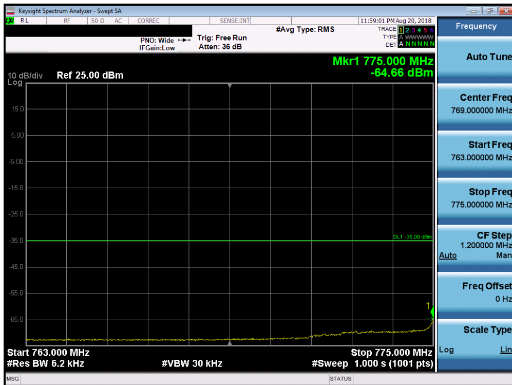
Plot 7-209. Lower Emission Mask Edge Plot (Band 13 – 10.0MHz QPSK – RB Size 50)
