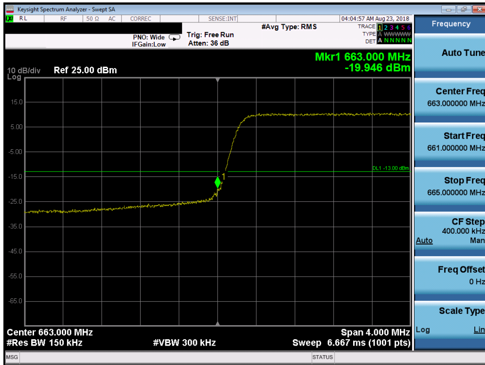
Plot 7-184. Lower Band Edge Plot (Band 71 - 5.0MHz QPSK - RB Size 25)
