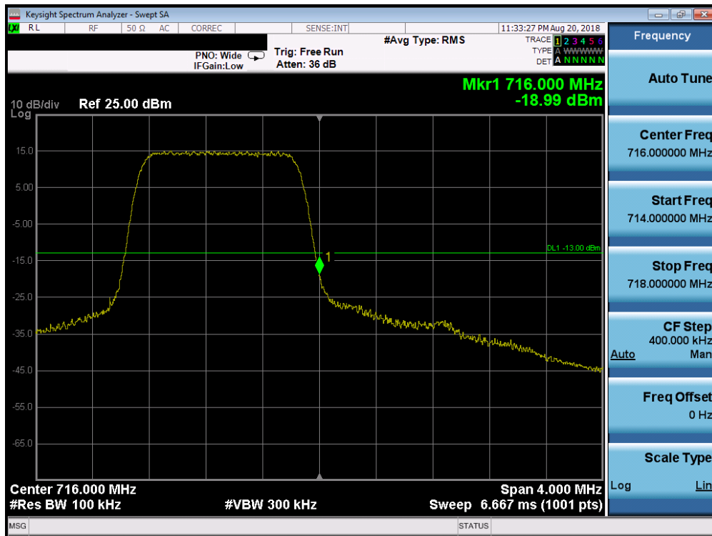
Plot 7-193. Upper Band Edge Plot (Band 12 – 1.4MHz QPSK – RB Size 6)
