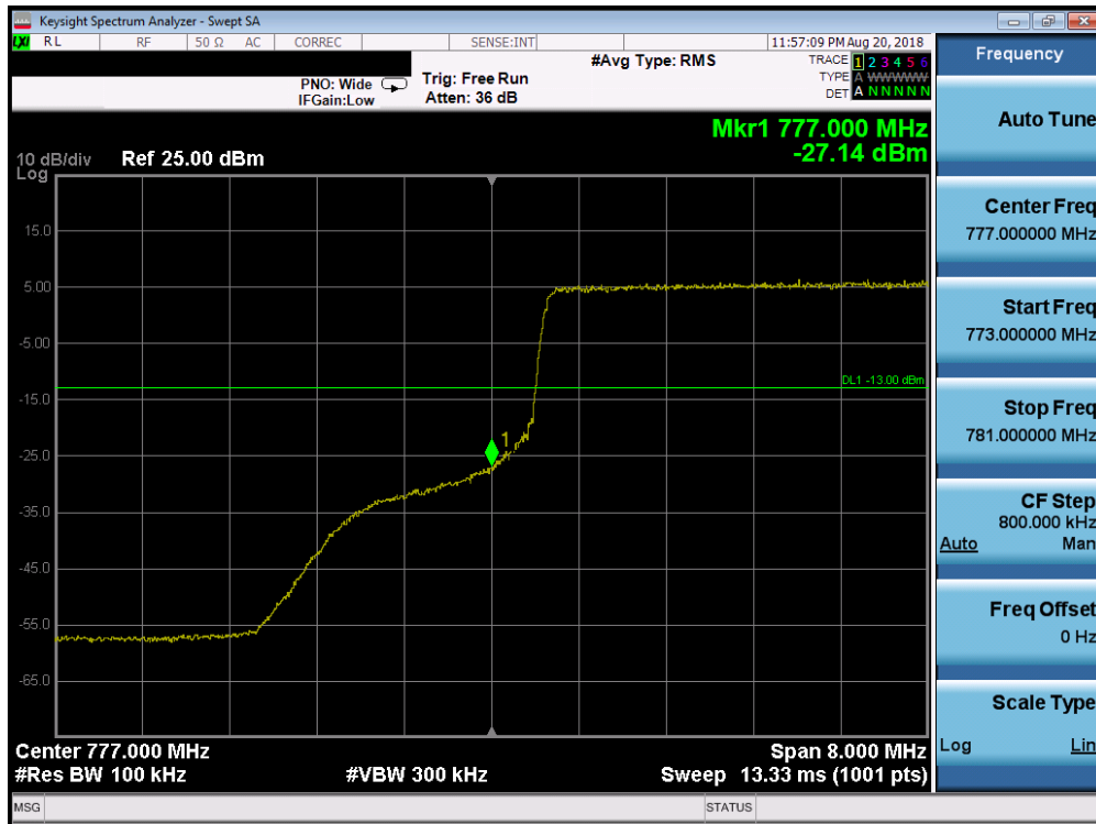
Plot 7-208. Lower Band Edge Plot (Band 13 – 10.0MHz QPSK – RB Size 50)
