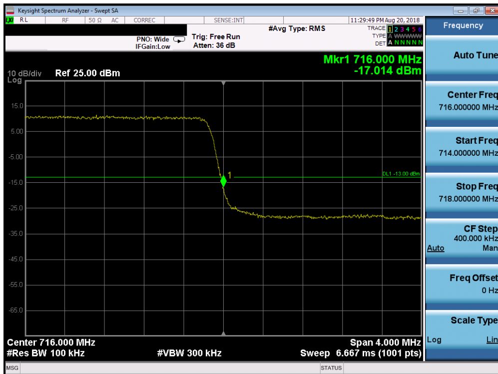
Plot 7-195. Upper Band Edge Plot (Band 12 – 3.0MHz QPSK – RB Size 15)
