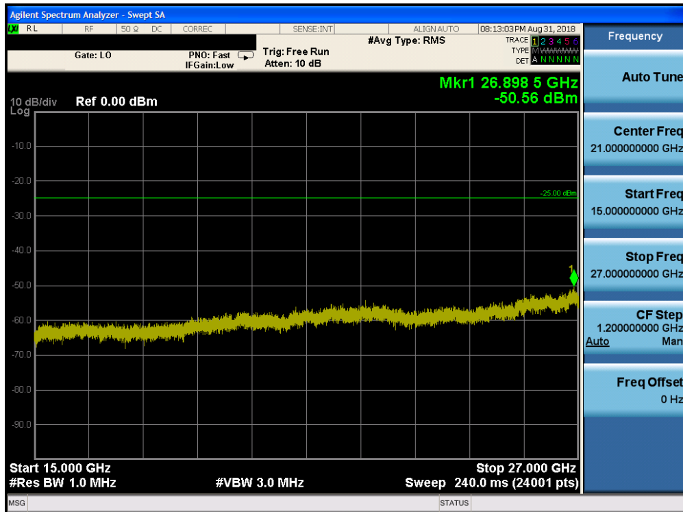
Plot 7-177. Conducted Spurious Plot (Band 41 – 20.0MHz QPSK – RB Size 1, RB Offset 0 – Low Channel)
