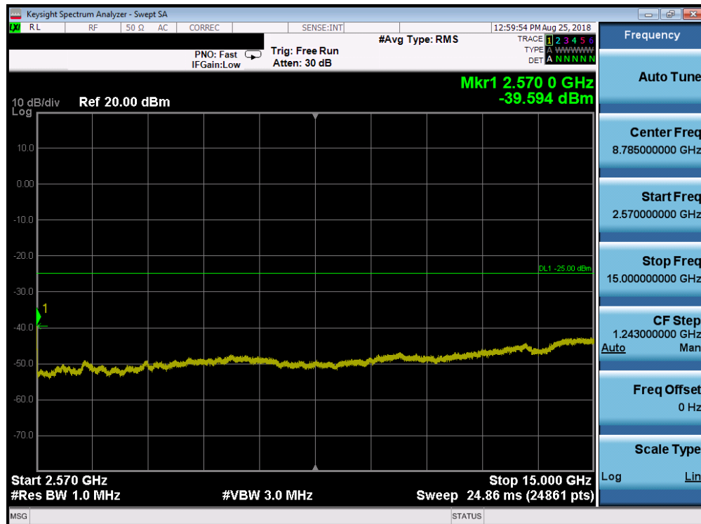
Plot 7-167. Conducted Spurious Plot (Band 7 – 20.0MHz QPSK – RB Size 1, RB Offset 0 – Low Channel)
