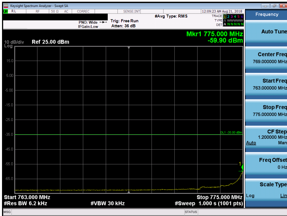
Plot 7-205. Lower Emission Mask Edge Plot (Band 13 – 5.0MHz QPSK – RB Size 25)
