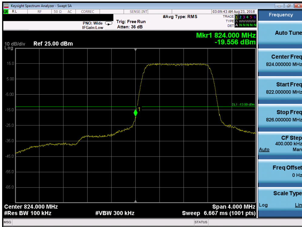
Plot 7-212. Lower Band Edge Plot (Band 5 – 1.4MHz QPSK – RB Size 6)
