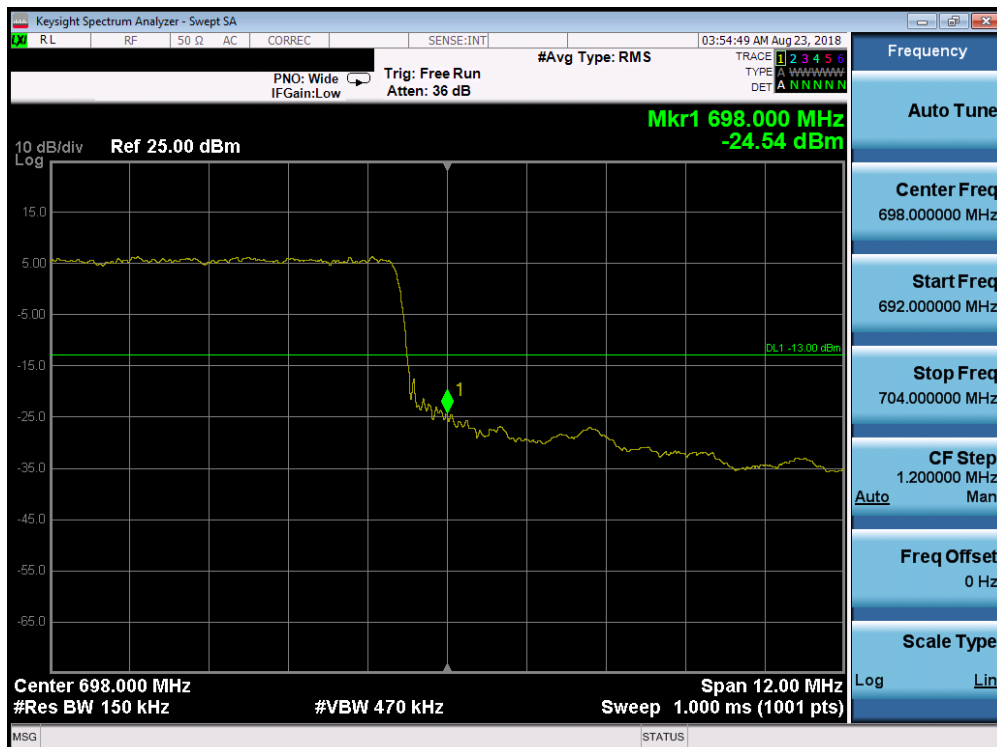
Plot 7-189. Upper Band Edge Plot (Band 71 - 15.0MHz QPSK - RB Size 75)
