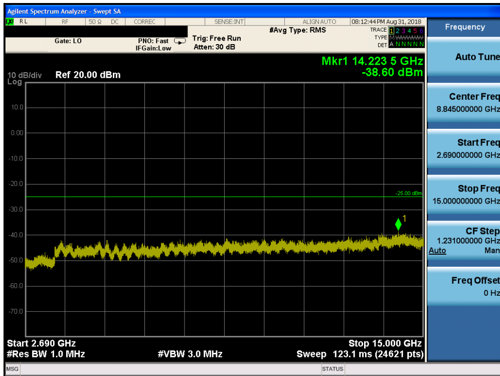
Plot 7-176. Conducted Spurious Plot (Band 41 – 20.0MHz QPSK – RB Size 1, RB Offset 0 – Low Channel)
