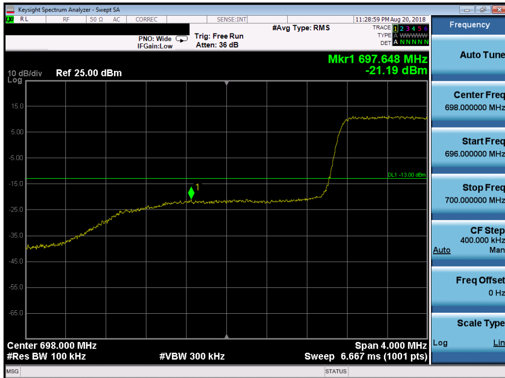
Plot 7-194. Lower Band Edge Plot (Band 12 – 3.0MHz QPSK – RB Size 15)
