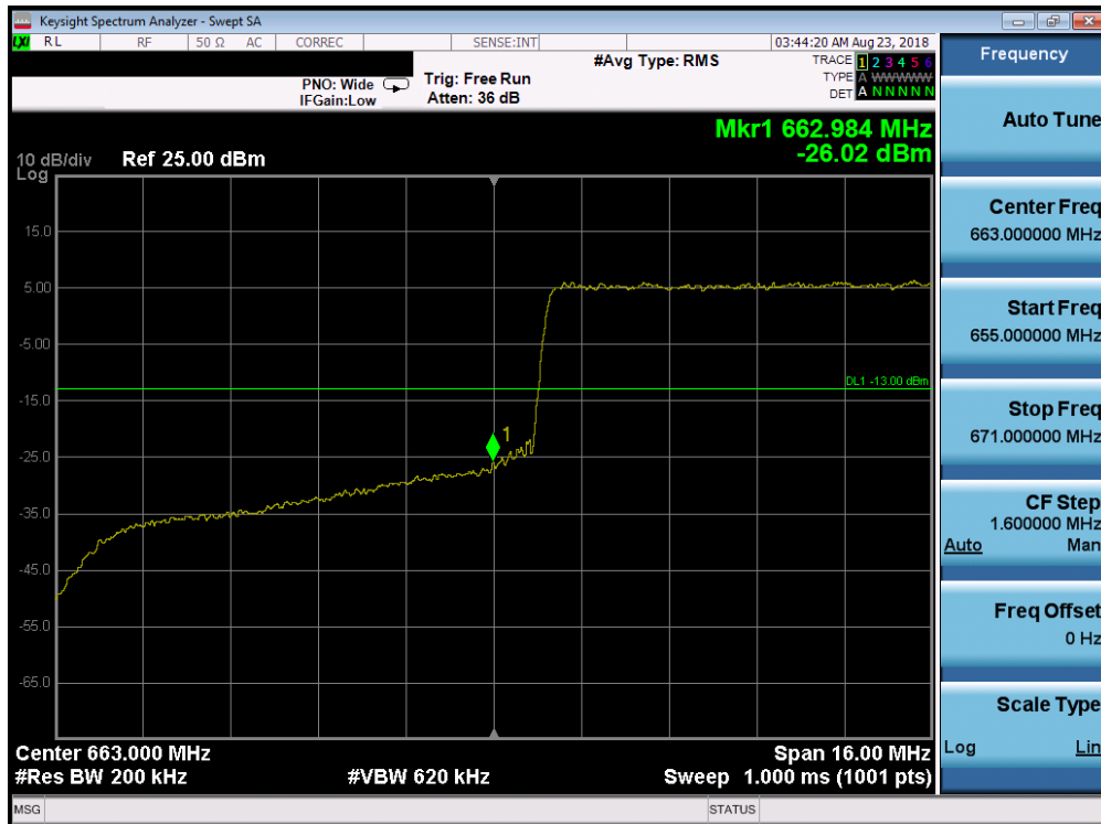
Plot 7-190. Lower Band Edge Plot (Band 71 – 20.0MHz QPSK – RB Size 100)
