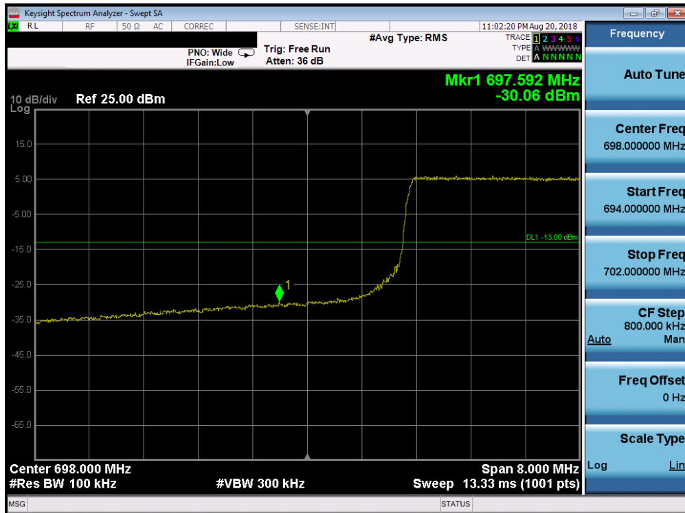
Plot 7-198. Lower Band Edge Plot (Band 12 – 10.0MHz QPSK – RB Size 50)
