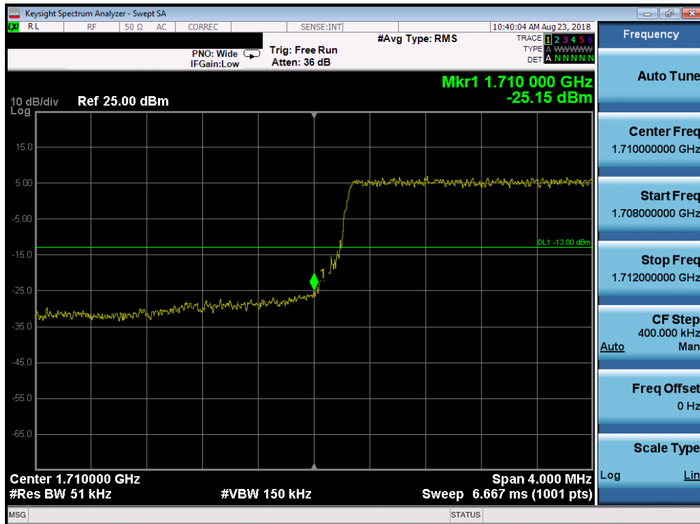
Plot 7-238. Lower Band Edge Plot (Band 4 – 5.0MHz QPSK – RB Size 25)
