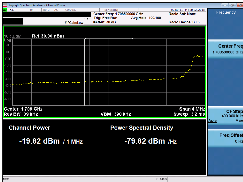
Plot 7-239. Lower Extended Band Edge Plot (Band 4 – 5.0MHz QPSK – RB Size 25)
