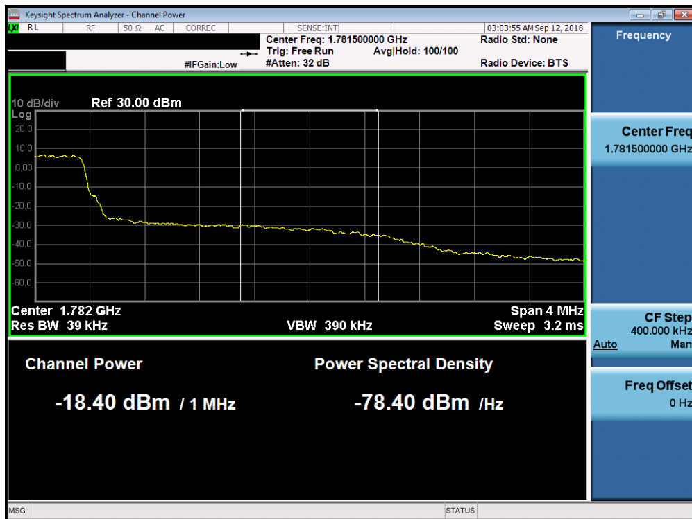
Plot 7-261. Upper Extended Band Edge Plot (Band 66 – 3.0MHz QPSK – RB Size 15)
