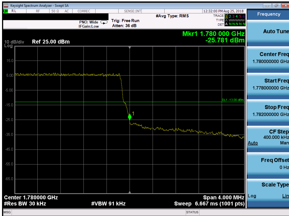
Plot 7-260. Upper Band Edge Plot (Band 66 – 3.0MHz QPSK – RB Size 15)
